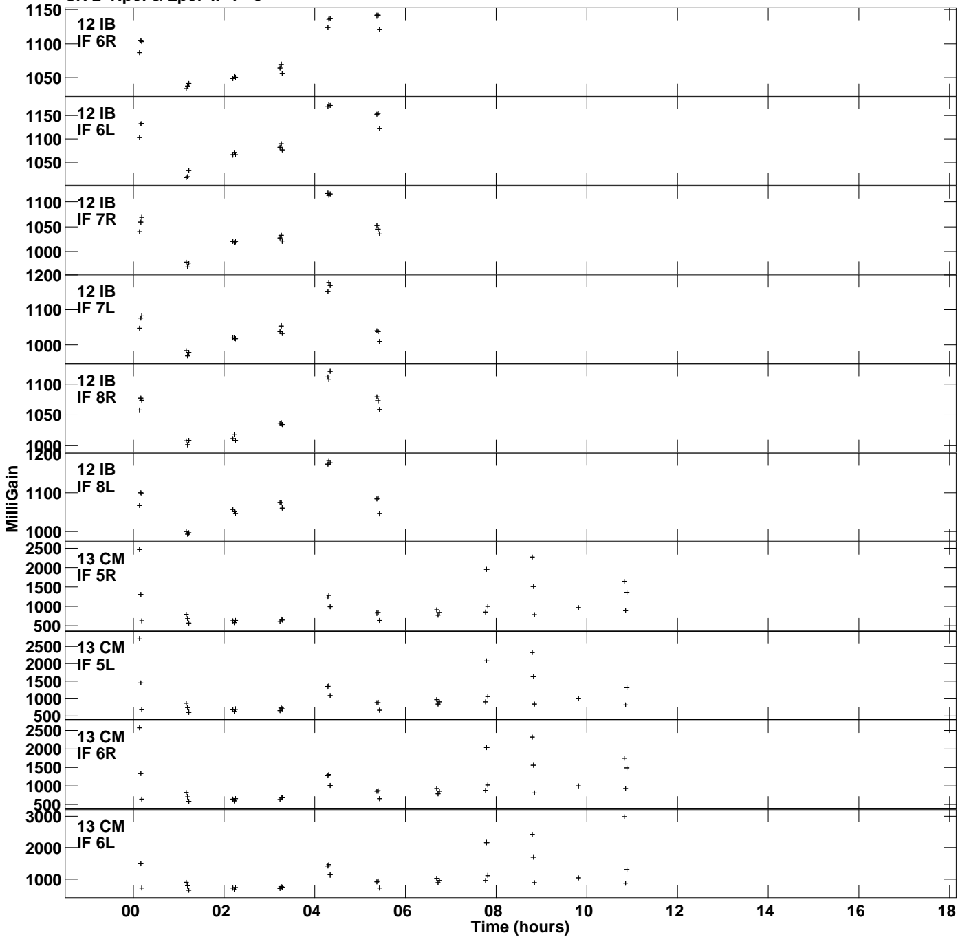
Plot file version 18 created 25-APR-2023 18:46:27 Gain amp vs UTC time for OQ208.MULTI.1 SN 2 Rpol & Lpol IF 1 - 8
