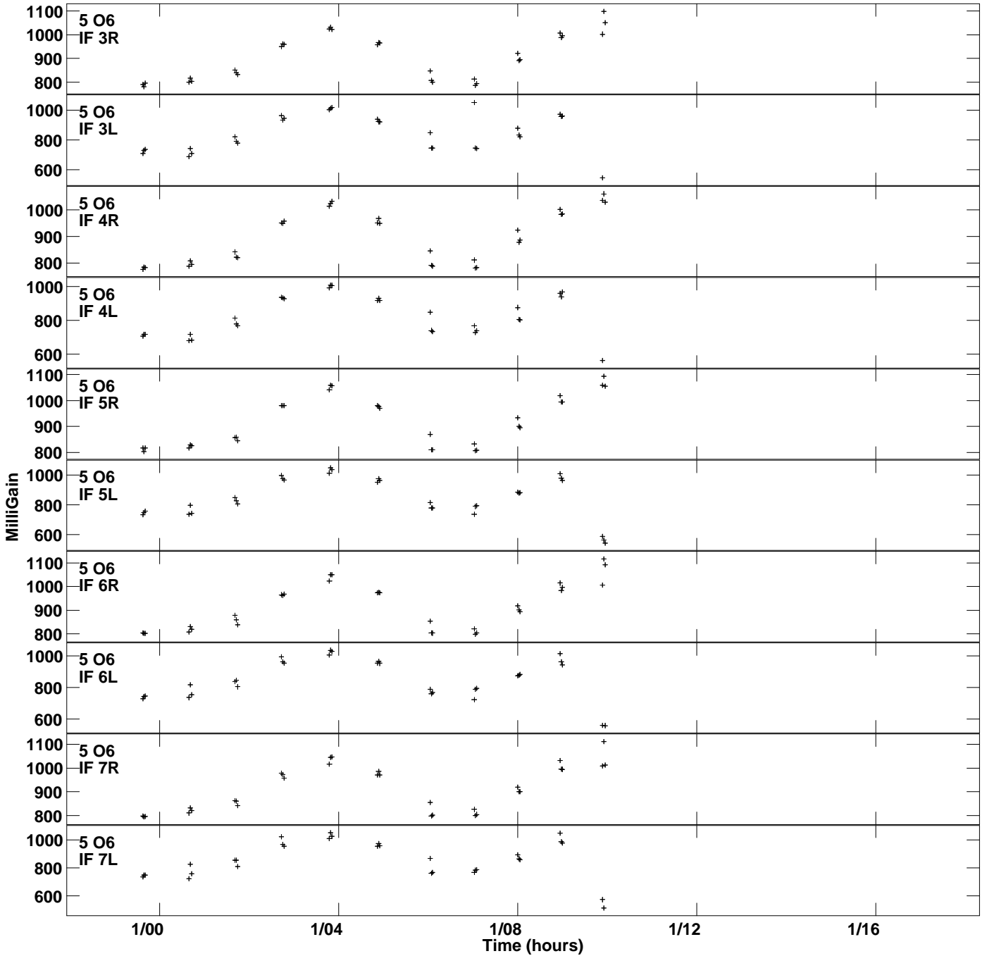
Plot file version 7 created 03-MAY-2023 12:14:24 Gain amp vs UTC time for OQ208.MULTI.1 SN 2 Rpol & Lpol IF 1 - 8
