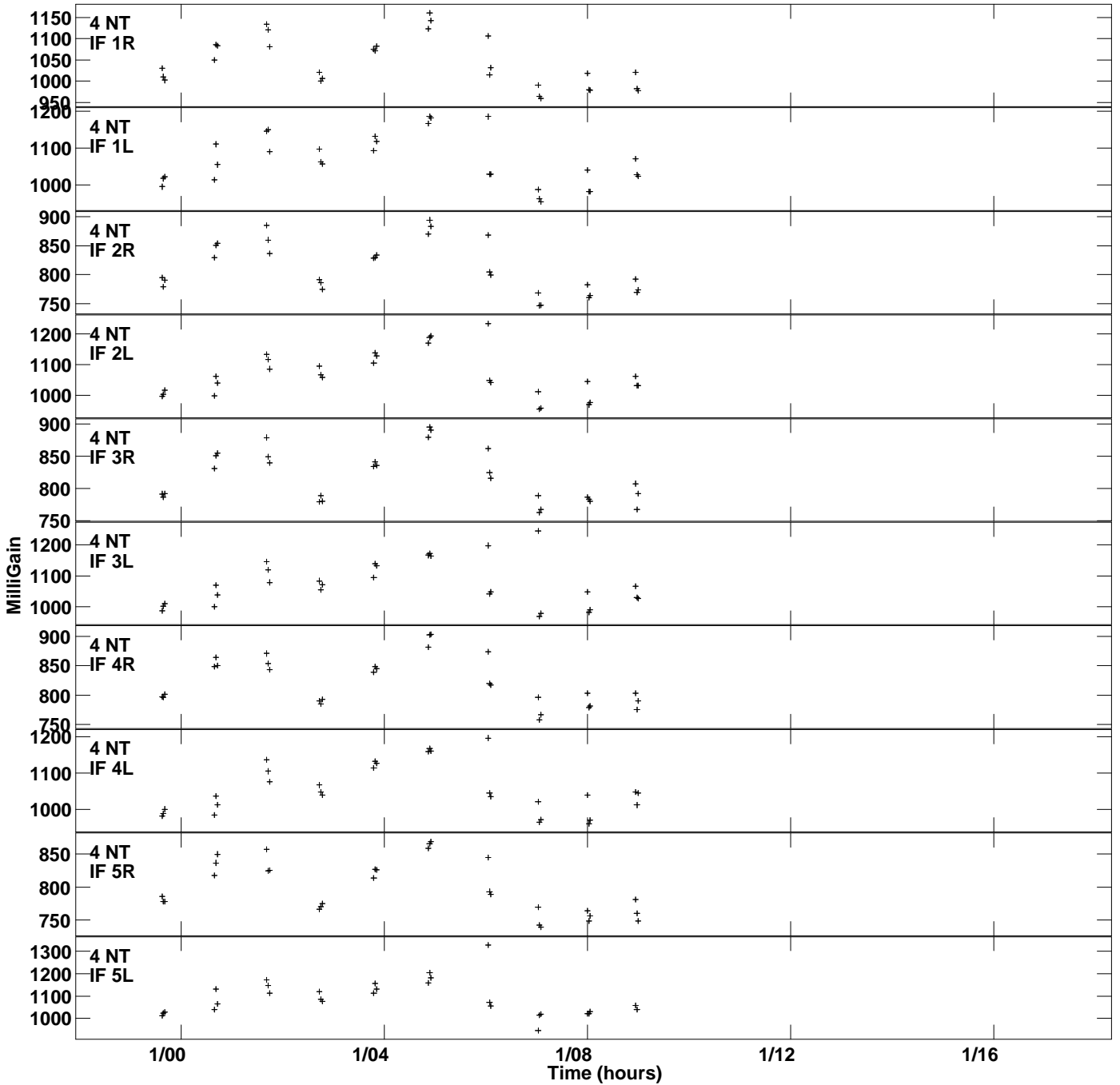
Plot file version 5 created 03-MAY-2023 12:14:24 Gain amp vs UTC time for OQ208.MULTI.1 SN 2 Rpol & Lpol IF 1 - 8
