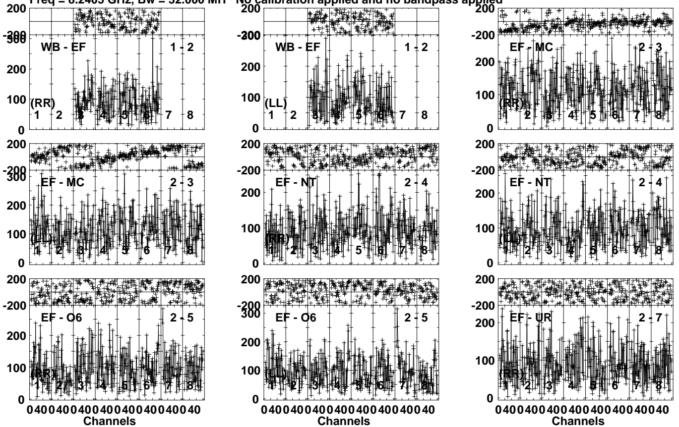
Lower frame: Micro Ampl Jy Top frame: Phas deg Vector averaged cross-power spectrum Several baselines displayed Timerange: 01/05:42:11 to 01/05:44:39
