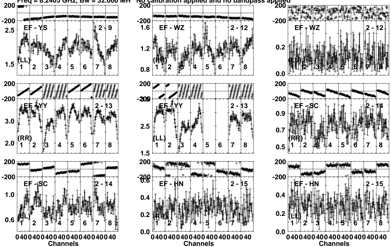
Lower frame: Milli Ampl Jy Top frame: Phas deg Vector averaged cross-power spectrum Several baselines displayed Timerange: 01/09:58:56 to 01/10:00:24
