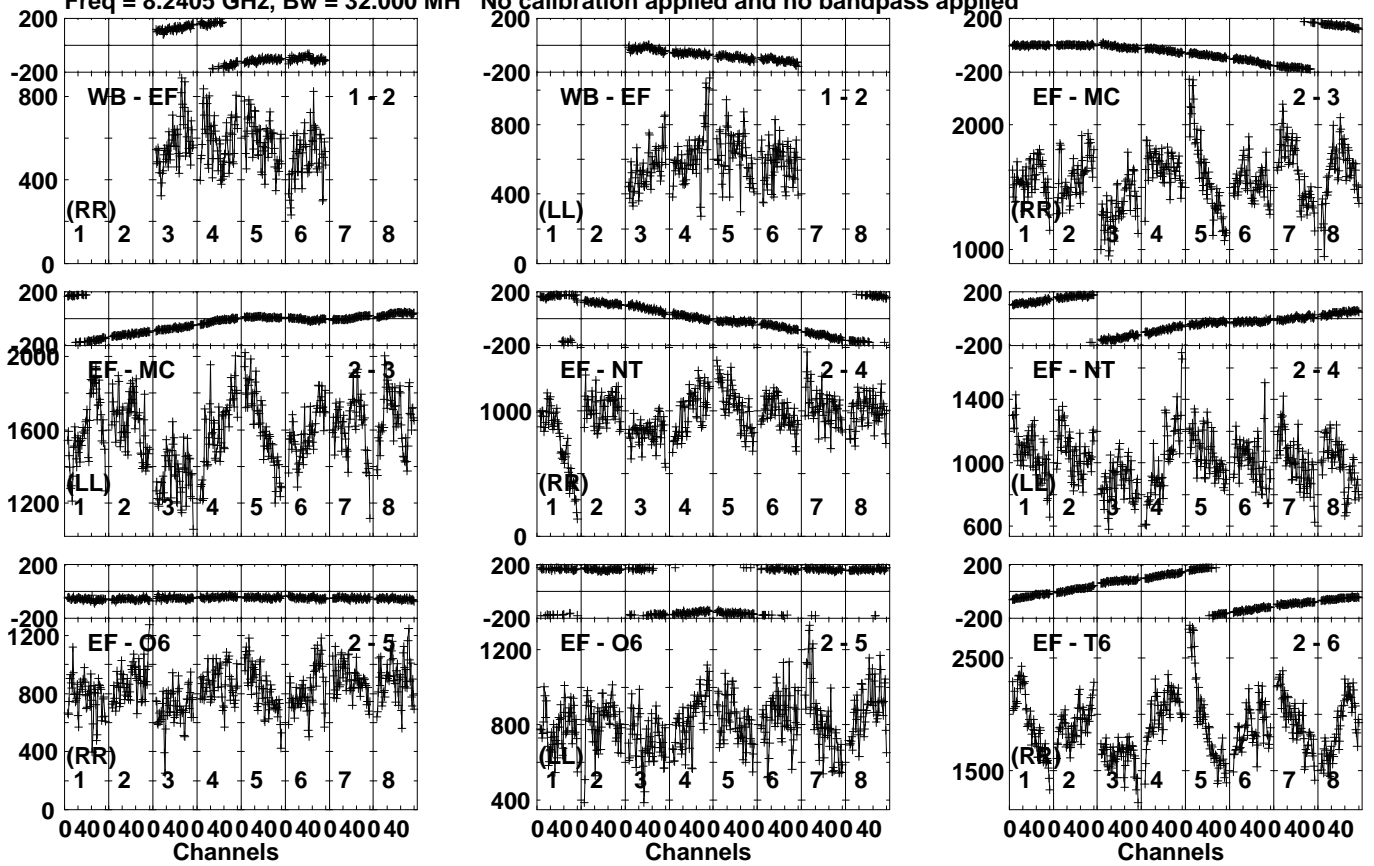
Lower frame: Micro Ampl Jy Top frame: Phas deg Vector averaged cross-power spectrum Several baselines displayed Timerange: 01/02:39:36 to 01/02:40:34
