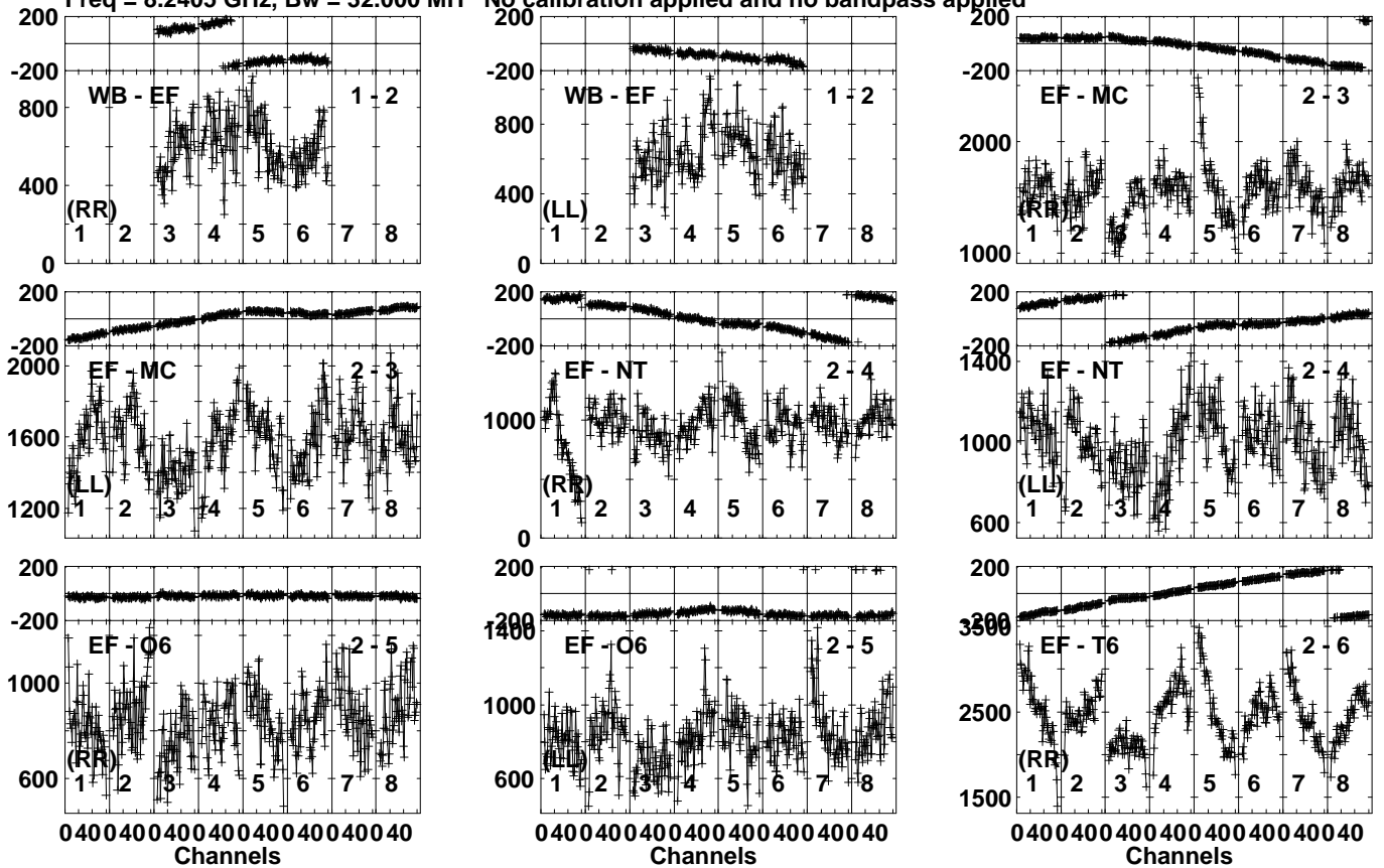
Lower frame: Micro Ampl Jy Top frame: Phas deg Vector averaged cross-power spectrum Several baselines displayed Timerange: 01/02:35:12 to 01/02:36:10
