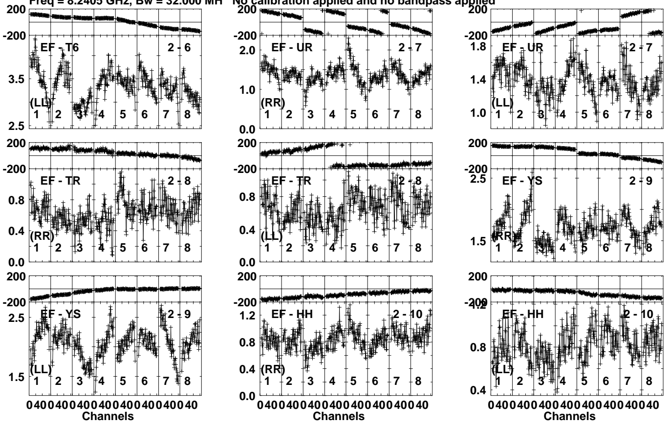
Lower frame: Milli Ampl Jy Top frame: Phas deg Vector averaged cross-power spectrum Several baselines displayed Timerange: 01/00:35:57 to 01/00:36:56
