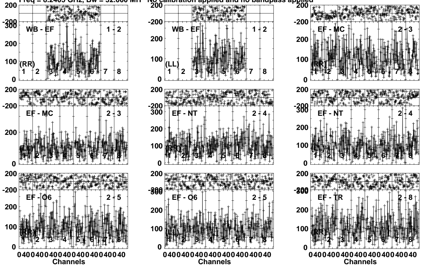
Lower frame: Micro Ampl Jy Top frame: Phas deg Vector averaged cross-power spectrum Several baselines displayed Timerange: 01/09:35:07 to 01/09:37:05
