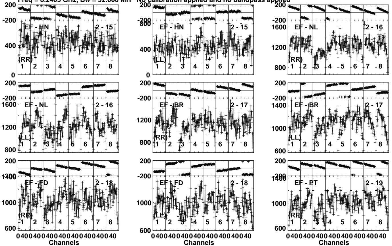
Lower frame: Micro Ampl Jy Top frame: Phas deg Vector averaged cross-power spectrum Several baselines displayed Timerange: 01/09:42:00 to 01/09:43:28
