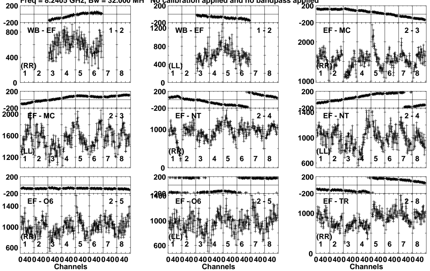
Lower frame: Micro Ampl Jy Top frame: Phas deg Vector averaged cross-power spectrum Several baselines displayed Timerange: 01/06:40:12 to 01/06:41:42
