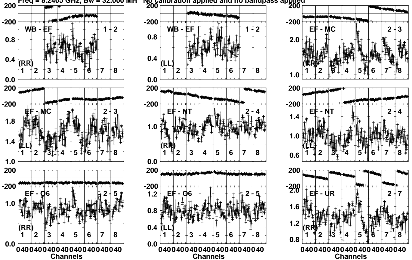
Lower frame: Milli Ampl Jy Top frame: Phas deg Vector averaged cross-power spectrum Several baselines displayed Timerange: 01/02:54:12 to 01/02:55:11
