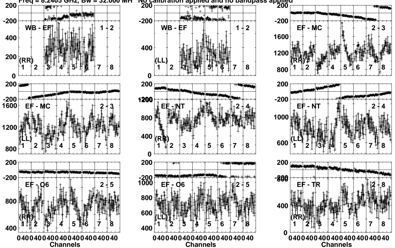
Lower frame: Micro Ampl Jy Top frame: Phas deg Vector averaged cross-power spectrum Several baselines displayed Timerange: 01/09:46:24 to 01/09:47:52
