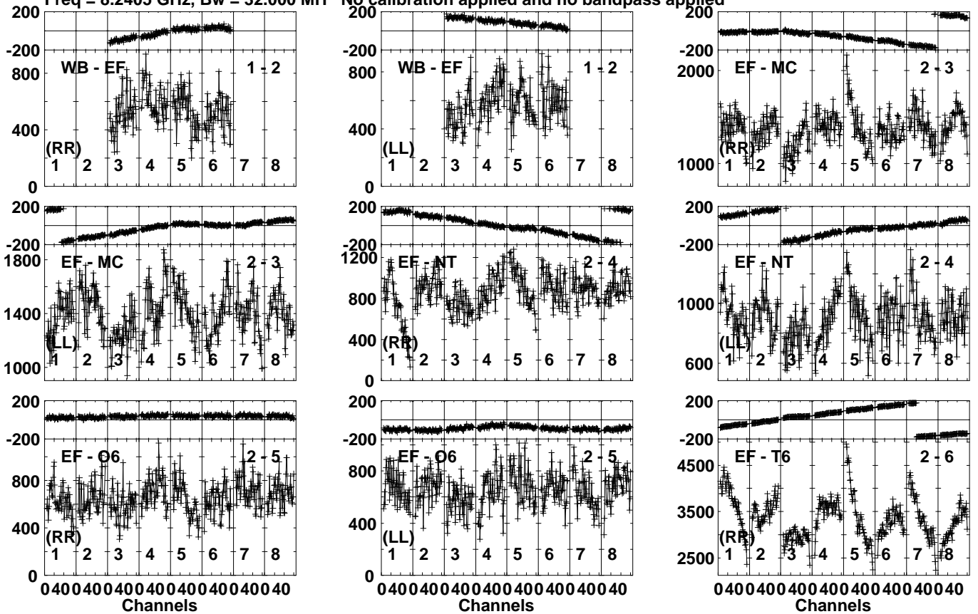
Lower frame: Micro Ampl Jy Top frame: Phas deg Vector averaged cross-power spectrum Several baselines displayed Timerange: 01/00:00:51 to 01/00:01:50
