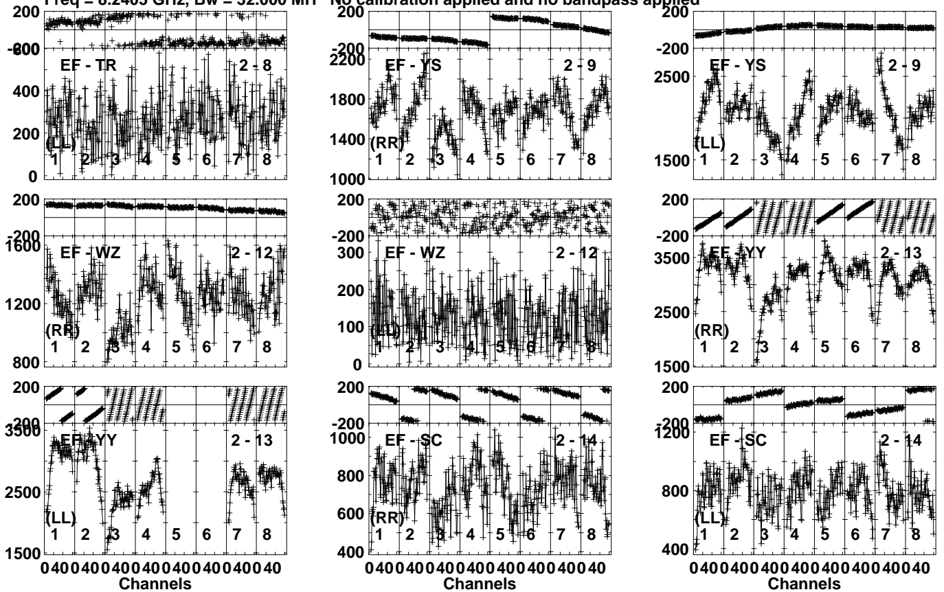
Lower frame: Micro Ampl Jy Top frame: Phas deg Vector averaged cross-power spectrum Several baselines displayed Timerange: 01/09:15:30 to 01/09:17:00
