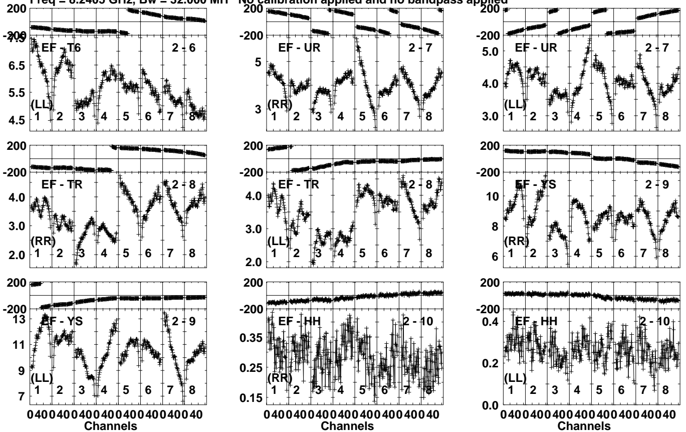
Lower frame: Milli Ampl Jy Top frame: Phas deg Vector averaged cross-power spectrum Several baselines displayed Timerange: 00/23:36:41 to 00/23:41:41
