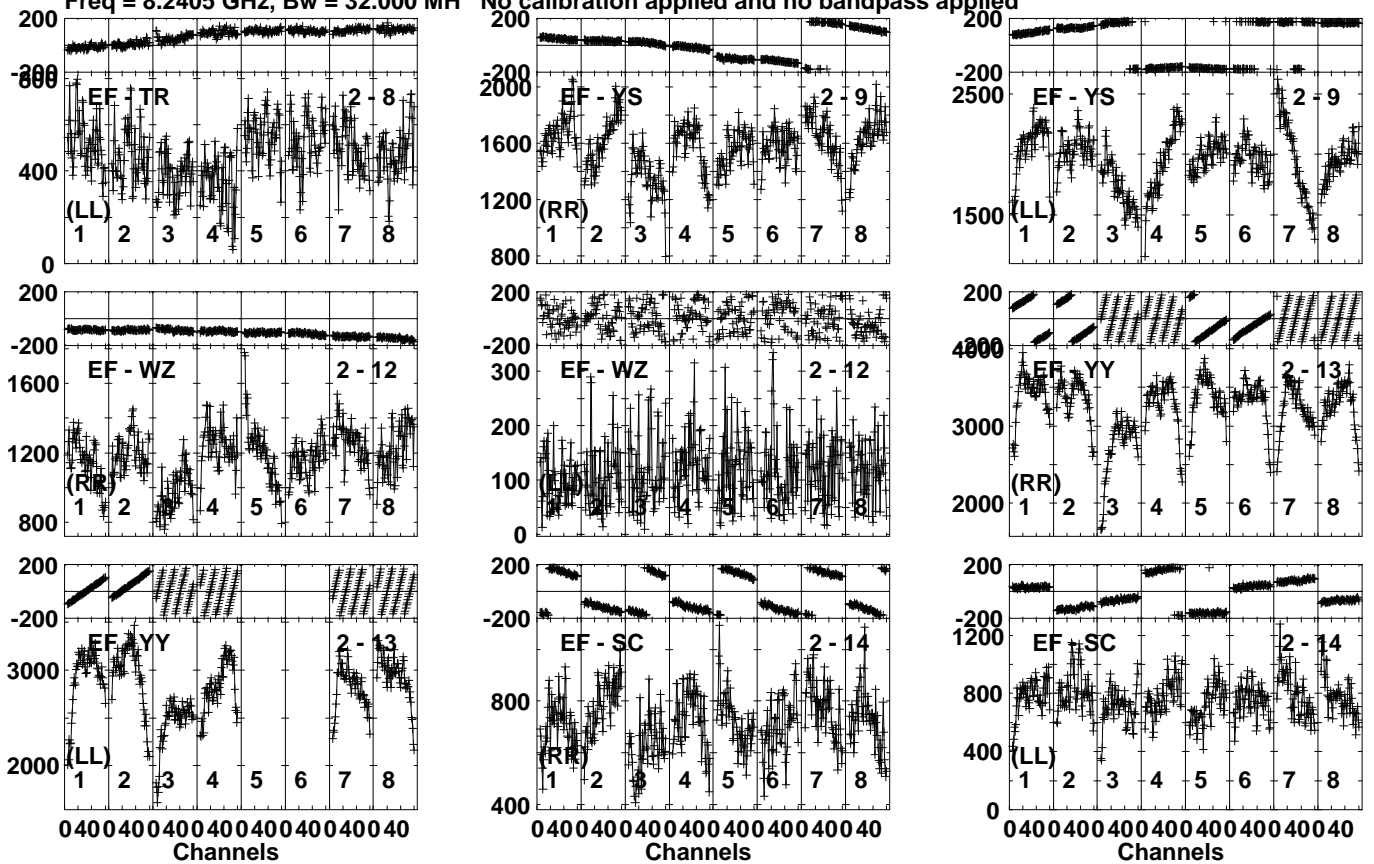
Lower frame: Micro Ampl Jy Top frame: Phas deg Vector averaged cross-power spectrum Several baselines displayed Timerange: 01/10:03:20 to 01/10:04:49
