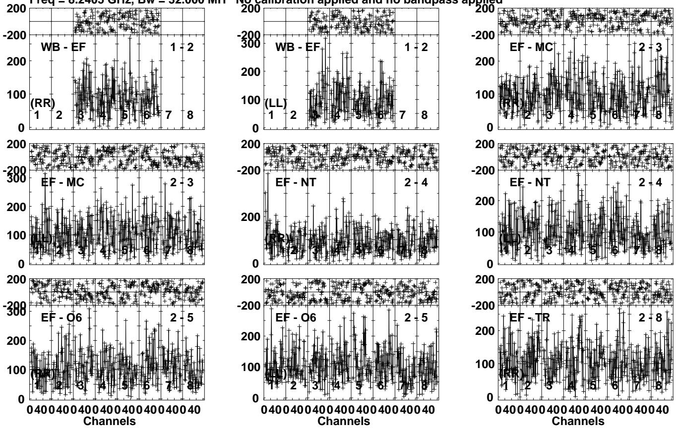
Lower frame: Micro Ampl Jy Top frame: Phas deg Vector averaged cross-power spectrum Several baselines displayed Timerange: 01/10:14:04 to 01/10:16:04
