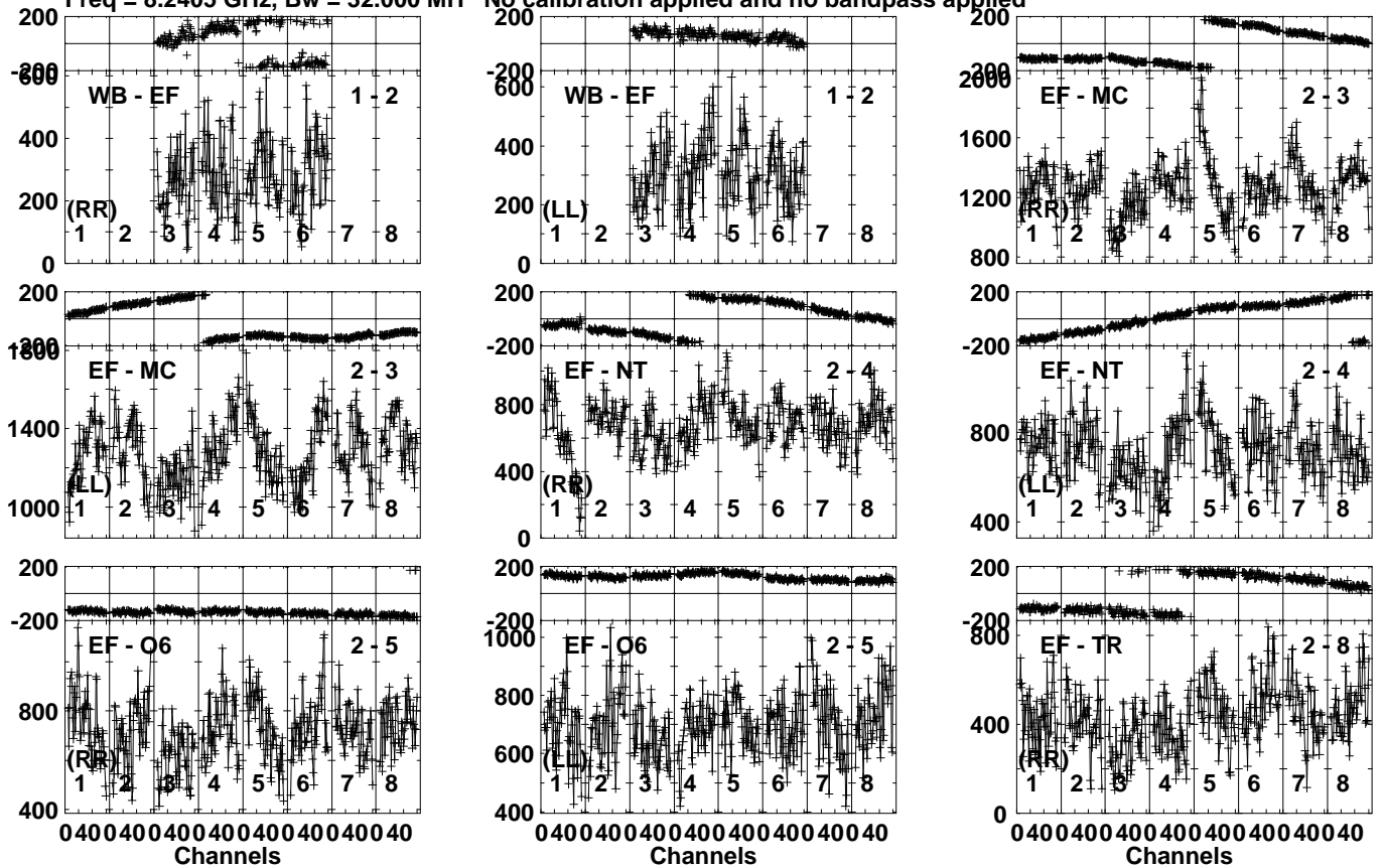
Lower frame: Micro Ampl Jy Top frame: Phas deg Vector averaged cross-power spectrum Several baselines displayed Timerange: 01/09:28:46 to 01/09:30:14
