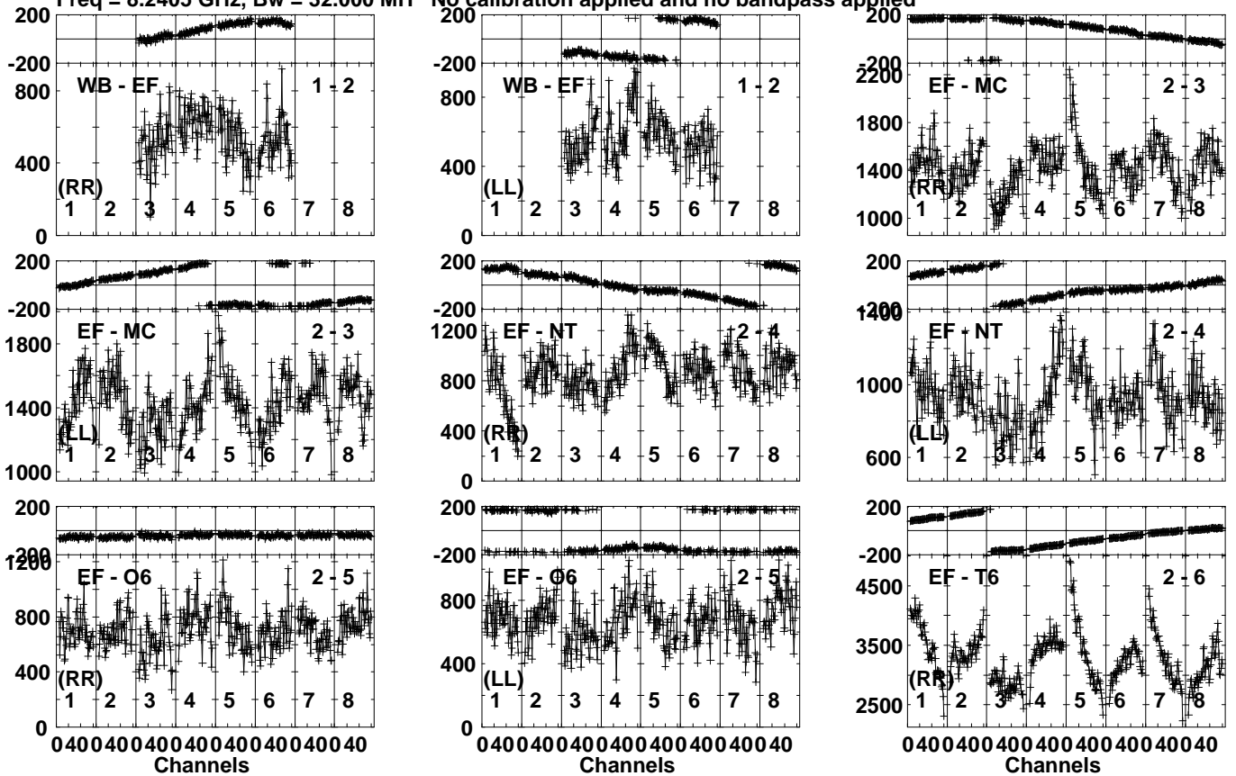
Lower frame: Micro Ampl Jy Top frame: Phas deg Vector averaged cross-power spectrum Several baselines displayed Timerange: 01/00:22:47 to 01/00:23:46
