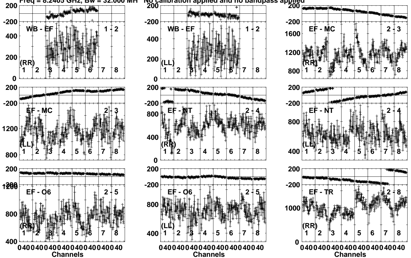
Lower frame: Micro Ampl Jy Top frame: Phas deg Vector averaged cross-power spectrum Several baselines displayed Timerange: 01/10:12:09 to 01/10:13:37
