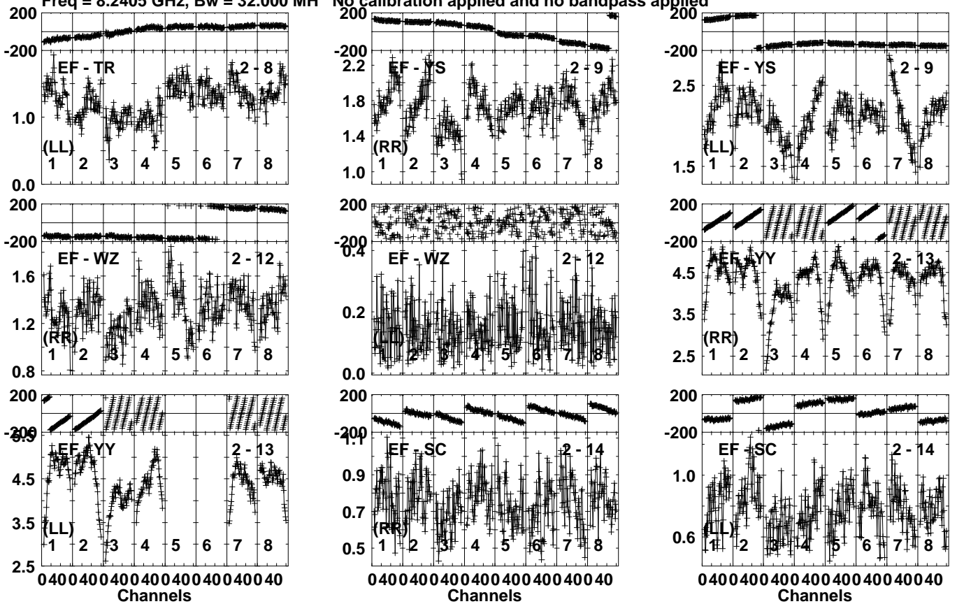
Lower frame: Milli Ampl Jy Top frame: Phas deg Vector averaged cross-power spectrum Several baselines displayed Timerange: 01/08:53:25 to 01/08:54:23
