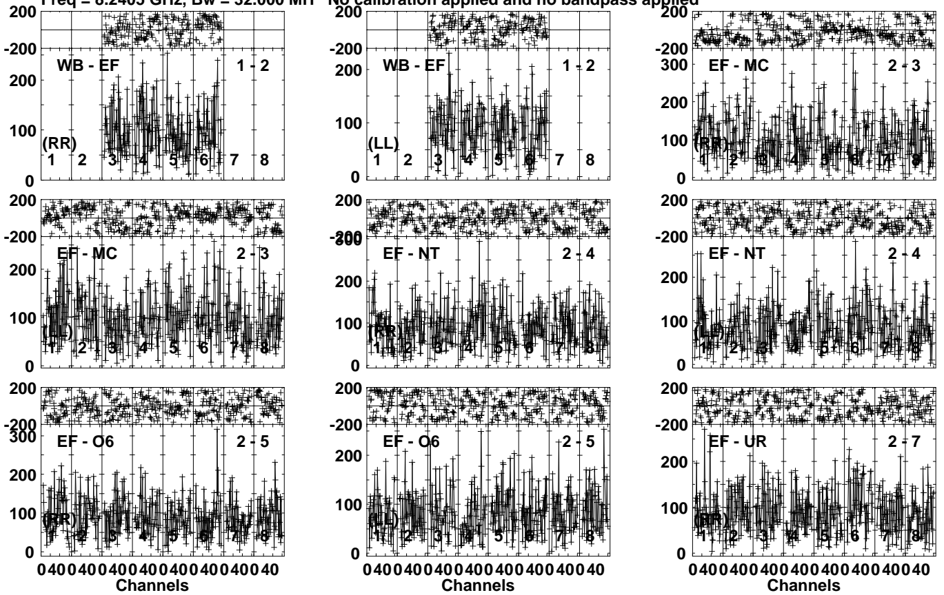
Lower frame: Micro Ampl Jy Top frame: Phas deg Vector averaged cross-power spectrum Several baselines displayed Timerange: 01/04:21:51 to 01/04:24:21
