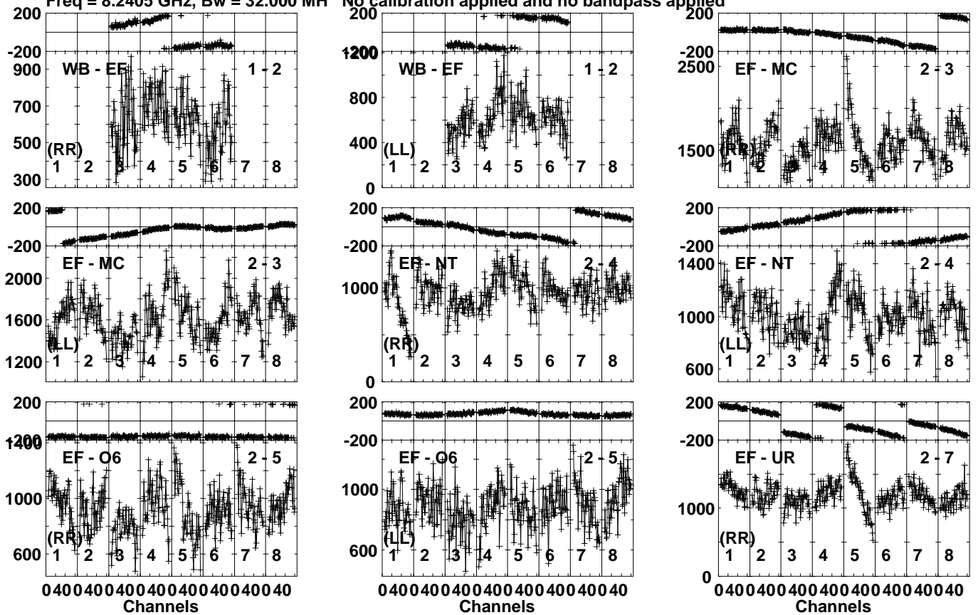
Lower frame: Micro Ampl Jy Top frame: Phas deg Vector averaged cross-power spectrum Several baselines displayed Timerange: 01/04:29:28 to 01/04:30:27
