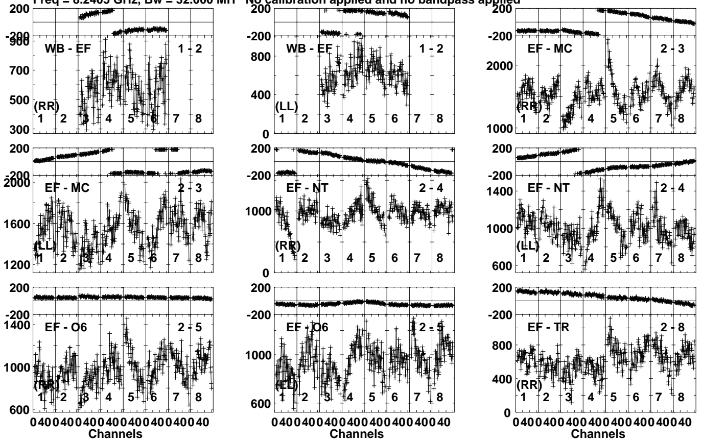
Lower frame: Micro Ampl Jy Top frame: Phas deg Vector averaged cross-power spectrum Several baselines displayed Timerange: 01/06:17:40 to 01/06:19:08
