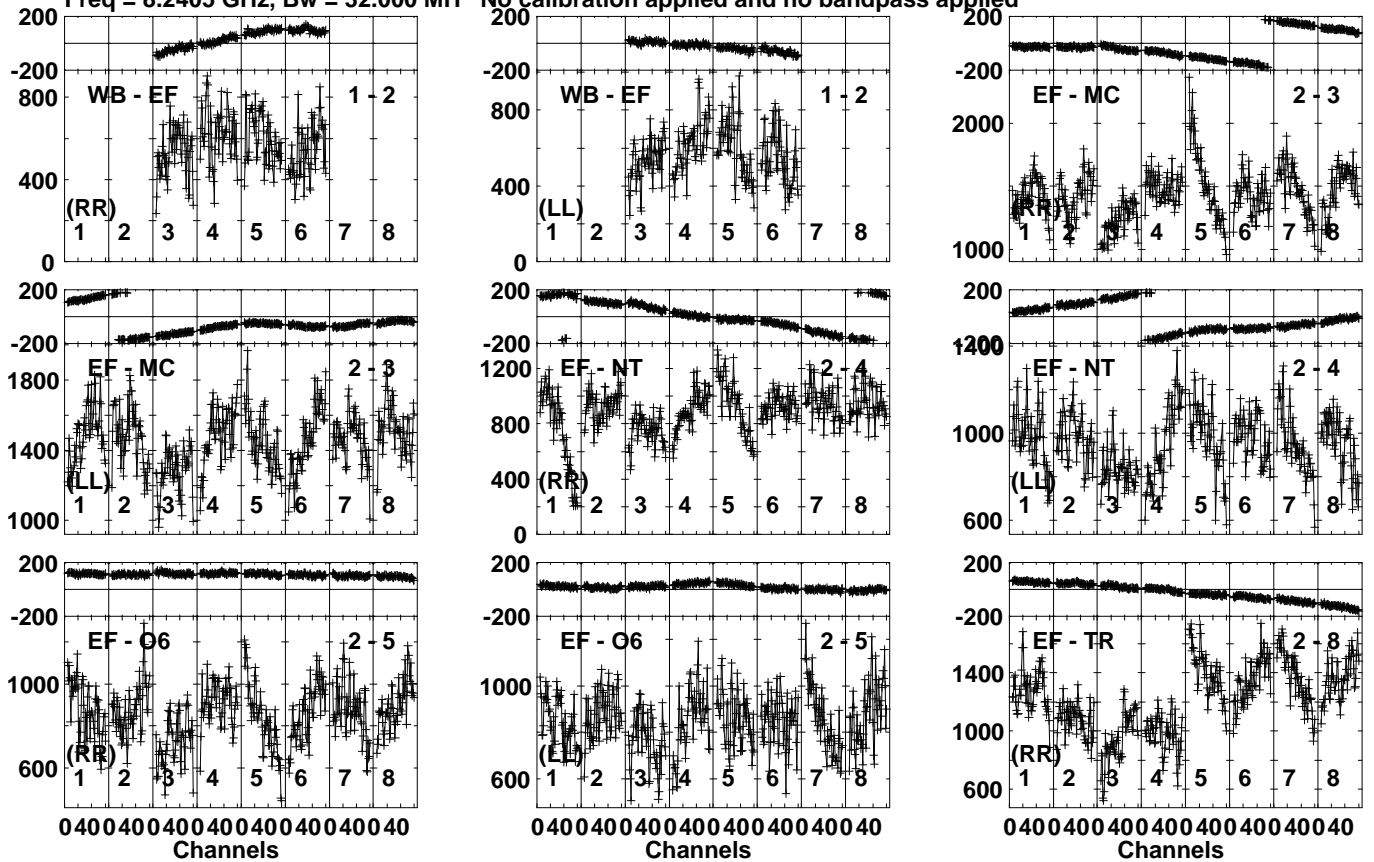
Lower frame: Micro Ampl Jy Top frame: Phas deg Vector averaged cross-power spectrum Several baselines displayed Timerange: 01/07:47:40 to 01/07:49:10
