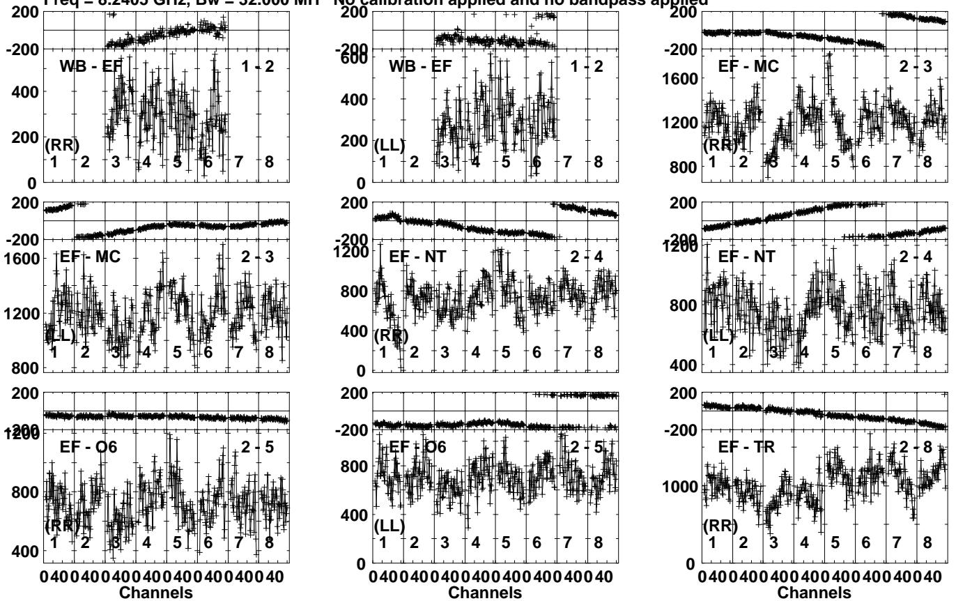
Lower frame: Micro Ampl Jy Top frame: Phas deg Vector averaged cross-power spectrum Several baselines displayed Timerange: 01/09:50:49 to 01/09:51:47
