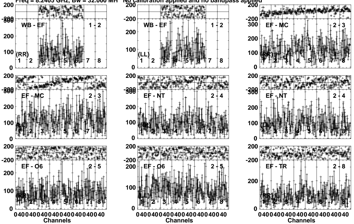
Lower frame: Micro Ampl Jy Top frame: Phas deg Vector averaged cross-power spectrum Several baselines displayed Timerange: 01/05:46:44 to 01/05:49:13
