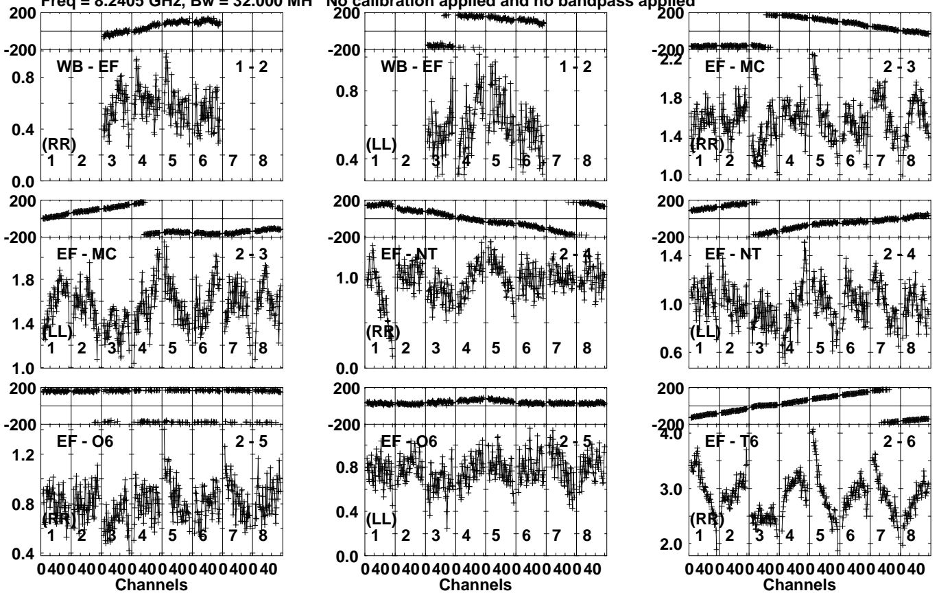
Lower frame: Milli Ampl Jy Top frame: Phas deg Vector averaged cross-power spectrum Several baselines displayed Timerange: 01/01:55:46 to 01/01:56:45
