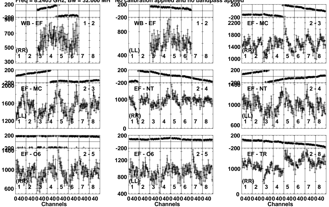
Lower frame: Micro Ampl Jy Top frame: Phas deg Vector averaged cross-power spectrum Several baselines displayed Timerange: 01/07:16:26 to 01/07:17:54
