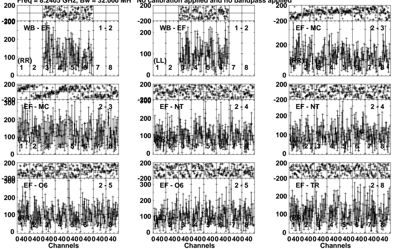
Lower frame: Micro Ampl Jy Top frame: Phas deg Vector averaged cross-power spectrum Several baselines displayed Timerange: 01/07:22:53 to 01/07:24:52
