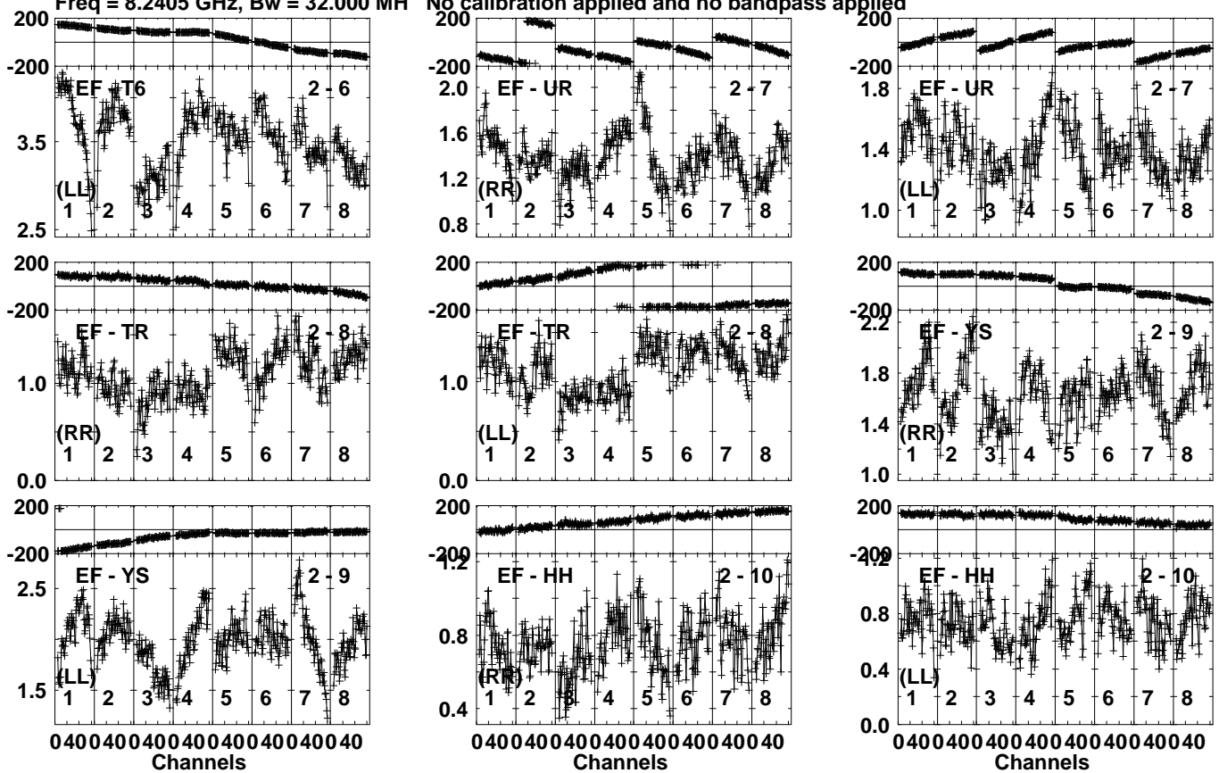
Lower frame: Milli Ampl Jy Top frame: Phas deg Vector averaged cross-power spectrum Several baselines displayed Timerange: 00/23:52:05 to 00/23:53:04
