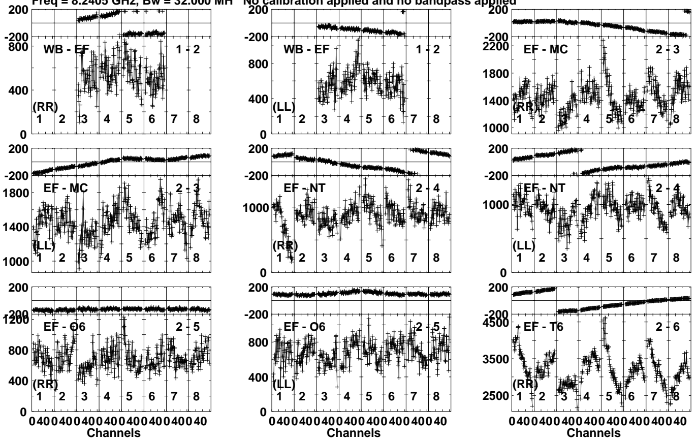
Lower frame: Micro Ampl Jy Top frame: Phas deg Vector averaged cross-power spectrum Several baselines displayed Timerange: 01/00:35:57 to 01/00:36:56
