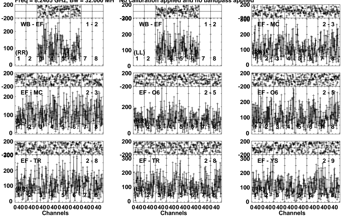
Lower frame: Micro Ampl Jy Top frame: Phas deg Vector averaged cross-power spectrum Several baselines displayed Timerange: 01/10:22:54 to 01/10:24:53
