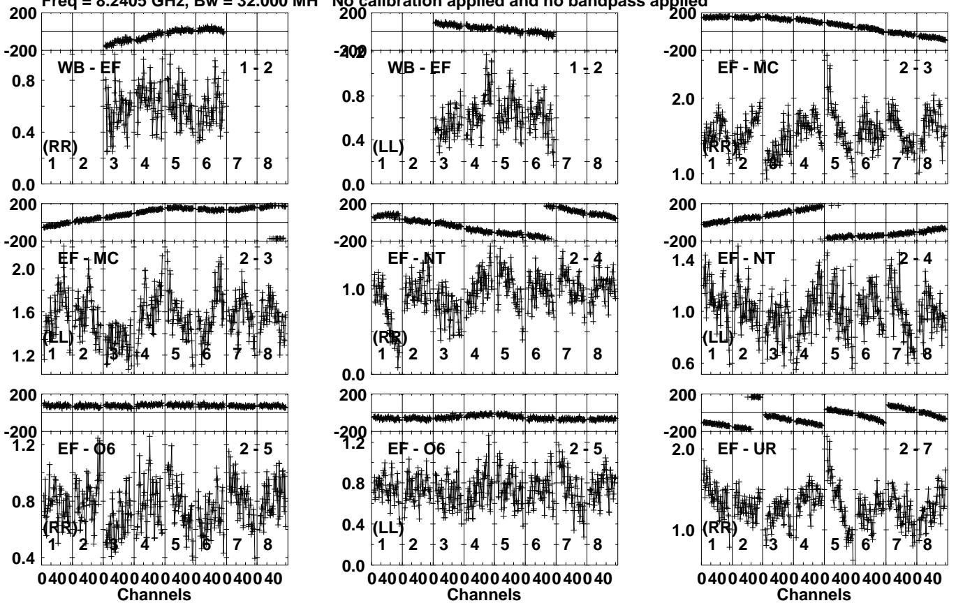
Lower frame: Milli Ampl Jy Top frame: Phas deg Vector averaged cross-power spectrum Several baselines displayed Timerange: 01/03:25:21 to 01/03:26:19
