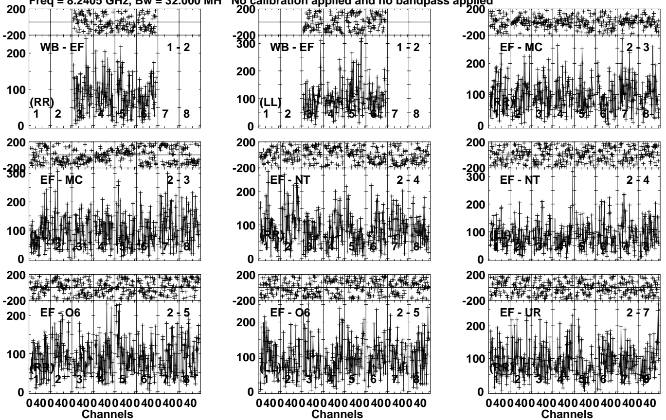
Lower frame: Micro Ampl Jy Top frame: Phas deg Vector averaged cross-power spectrum Several baselines displayed Timerange: 01/04:12:46 to 01/04:15:16
