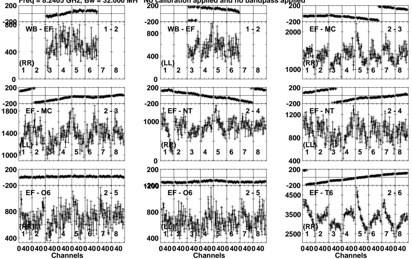
Lower frame: Micro Ampl Jy Top frame: Phas deg Vector averaged cross-power spectrum Several baselines displayed Timerange: 01/00:05:15 to 01/00:06:13
