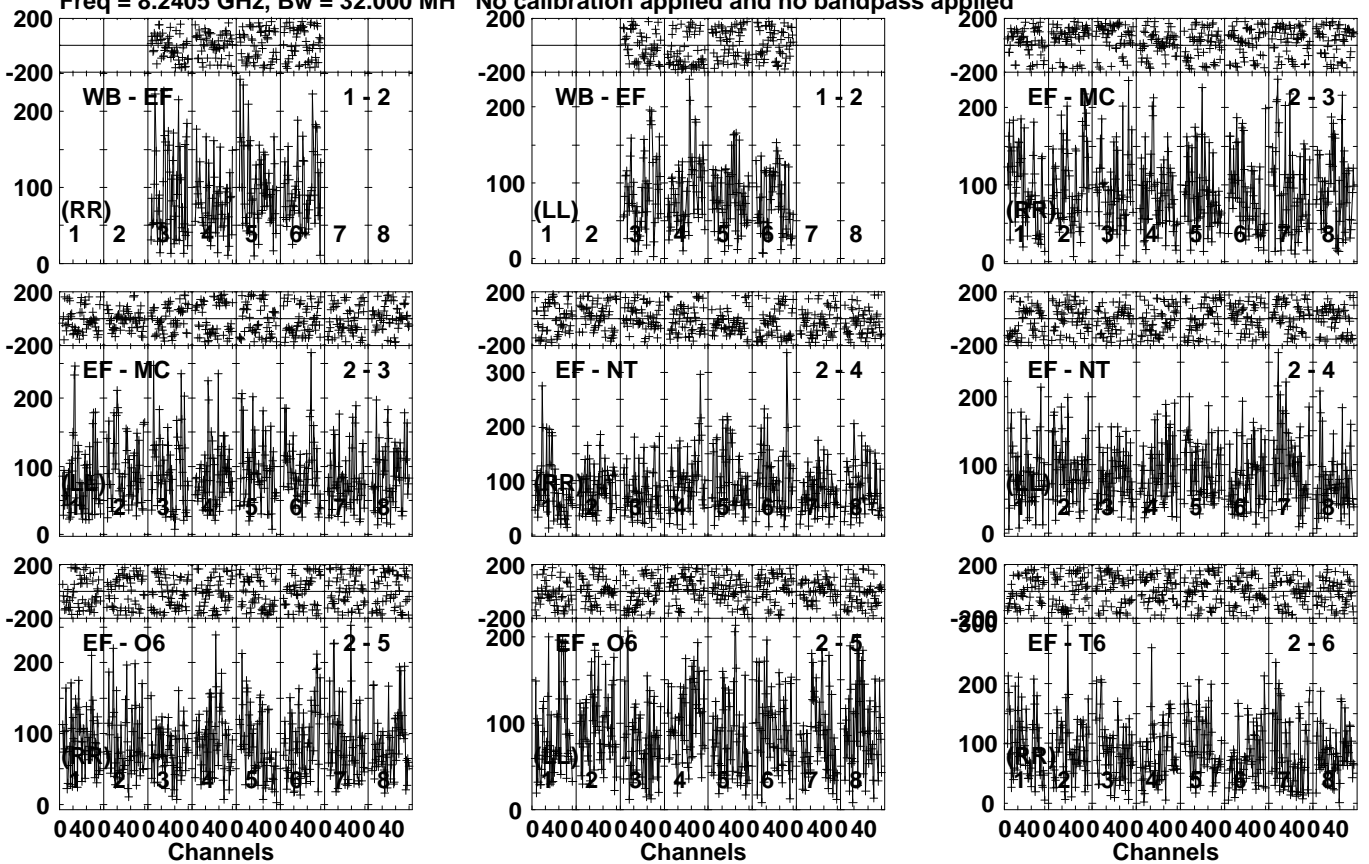
Lower frame: Micro Ampl Jy Top frame: Phas deg Vector averaged cross-power spectrum Several baselines displayed Timerange: 01/02:27:50 to 01/02:30:20
