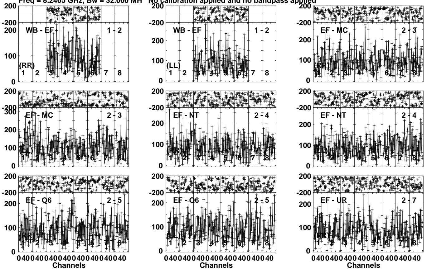
Lower frame: Micro Ampl Jy Top frame: Phas deg Vector averaged cross-power spectrum Several baselines displayed Timerange: 01/04:26:24 to 01/04:28:54
