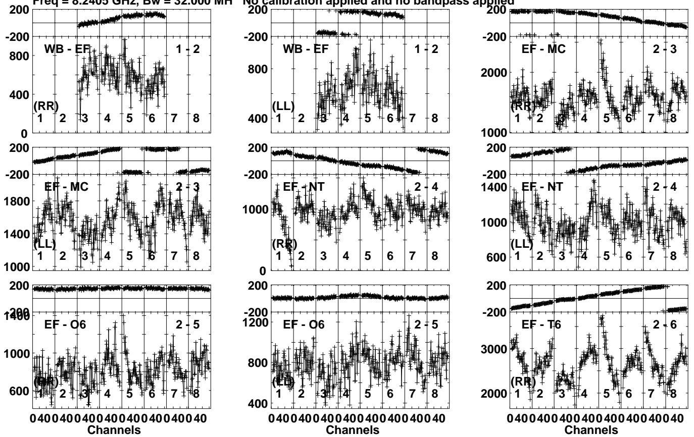
Lower frame: Micro Ampl Jy Top frame: Phas deg Vector averaged cross-power spectrum Several baselines displayed Timerange: 01/02:04:31 to 01/02:05:30
