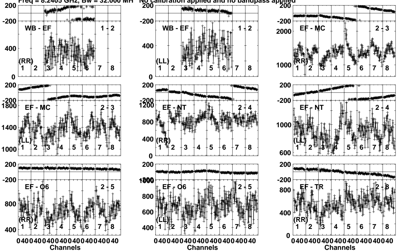
Lower frame: Micro Ampl Jy Top frame: Phas deg Vector averaged cross-power spectrum Several baselines displayed Timerange: 01/08:44:34 to 01/08:46:02
