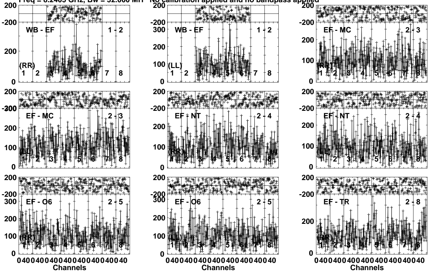
Lower frame: Micro Ampl Jy Top frame: Phas deg Vector averaged cross-power spectrum Several baselines displayed Timerange: 01/09:39:32 to 01/09:41:31
