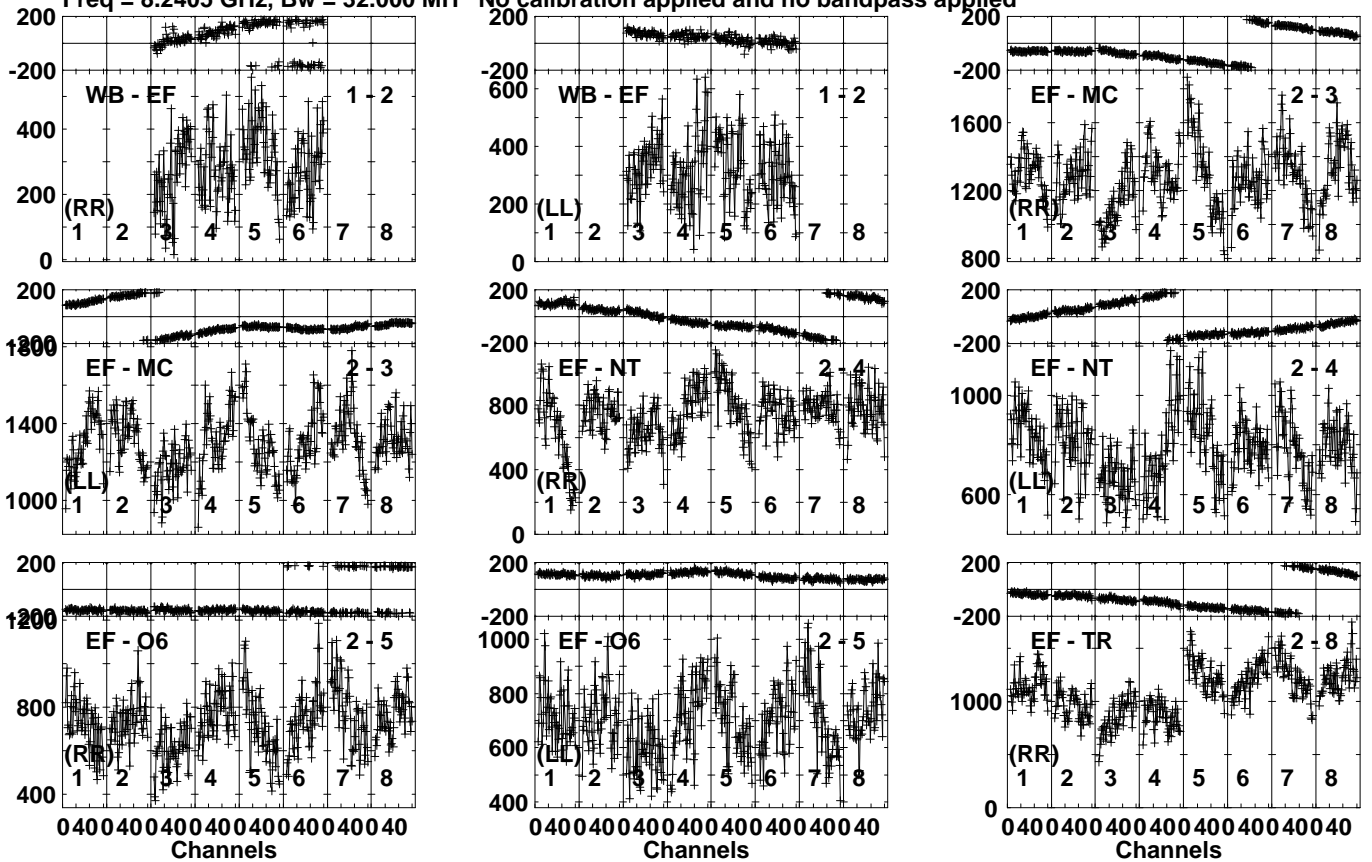
Lower frame: Micro Ampl Jy Top frame: Phas deg Vector averaged cross-power spectrum Several baselines displayed Timerange: 01/09:24:20 to 01/09:25:50
