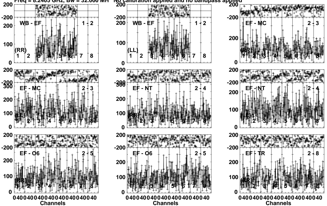
Lower frame: Micro Ampl Jy Top frame: Phas deg Vector averaged cross-power spectrum Several baselines displayed Timerange: 01/05:51:16 to 01/05:53:46
