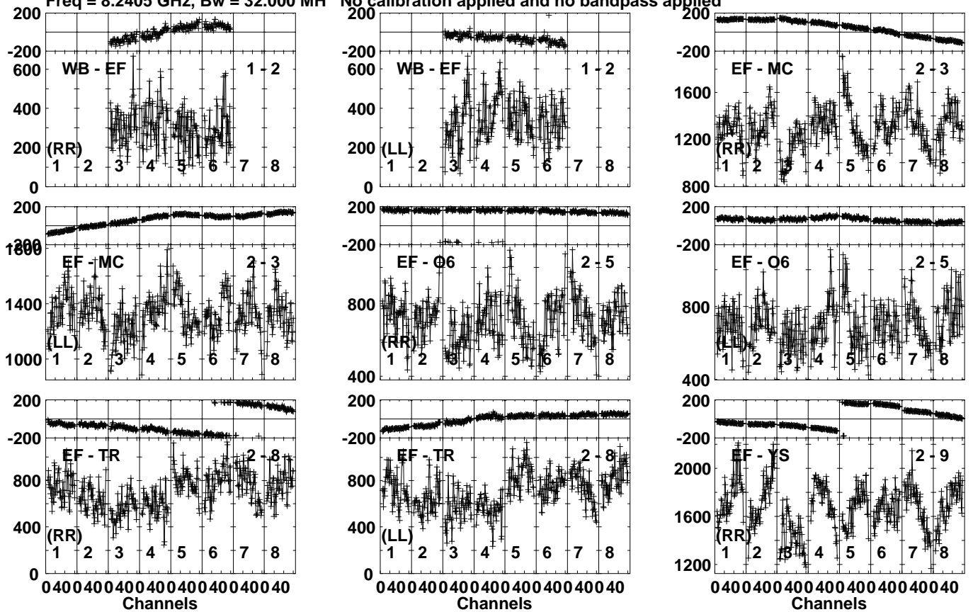
Lower frame: Micro Ampl Jy Top frame: Phas deg Vector averaged cross-power spectrum Several baselines displayed Timerange: 01/09:11:06 to 01/09:12:34
