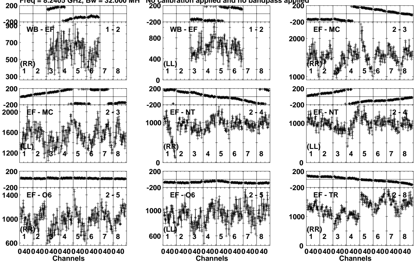
Lower frame: Micro Ampl Jy Top frame: Phas deg Vector averaged cross-power spectrum Several baselines displayed Timerange: 01/06:22:11 to 01/06:23:40
