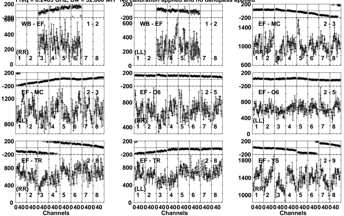
Lower frame: Micro Ampl Jy Top frame: Phas deg Vector averaged cross-power spectrum Several baselines displayed Timerange: 01/10:20:57 to 01/10:22:25
