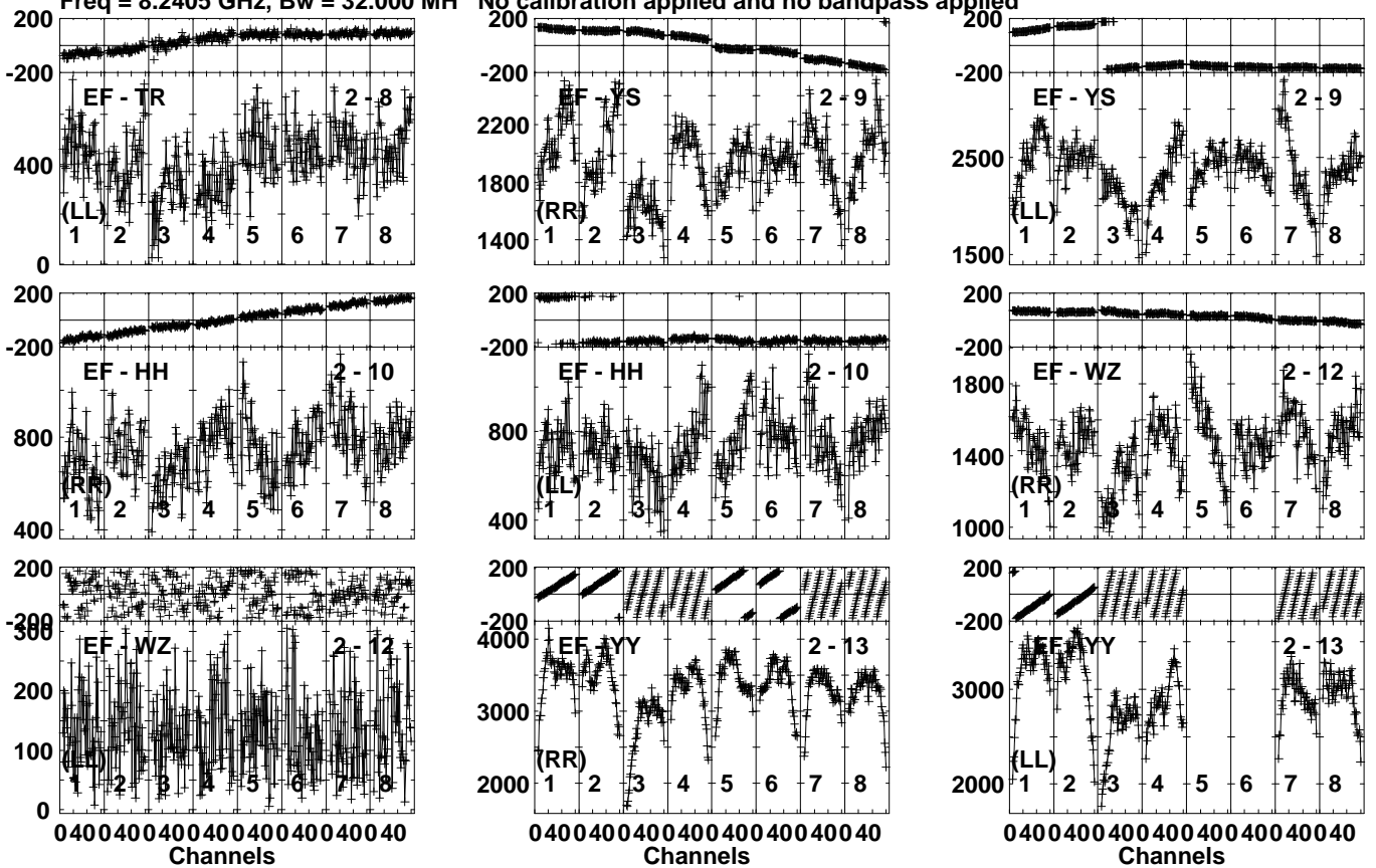
Lower frame: Micro Ampl Jy Top frame: Phas deg Vector averaged cross-power spectrum Several baselines displayed Timerange: 01/07:25:21 to 01/07:26:50
