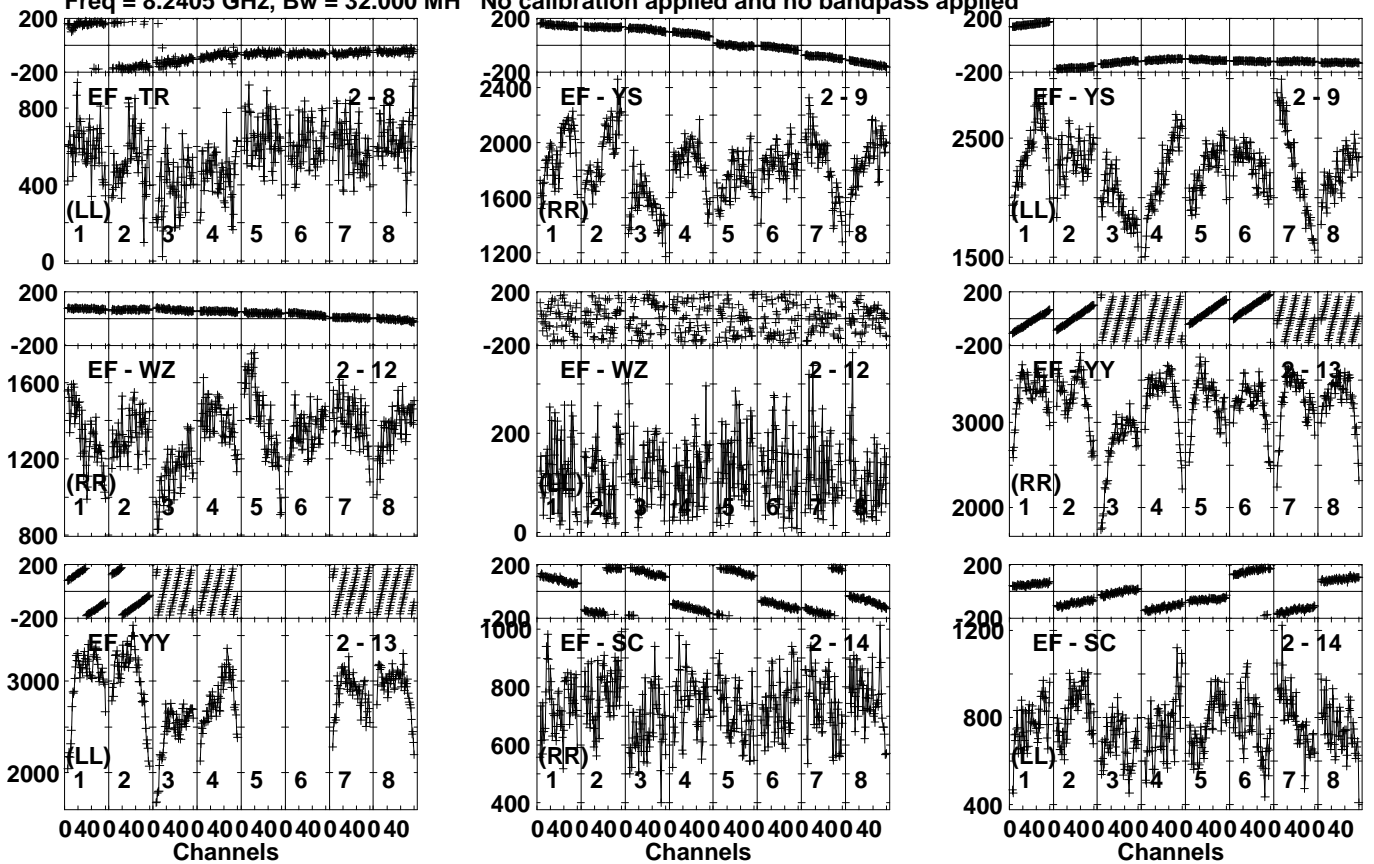
Lower frame: Micro Ampl Jy Top frame: Phas deg Vector averaged cross-power spectrum Several baselines displayed Timerange: 01/08:13:32 to 01/08:15:00
