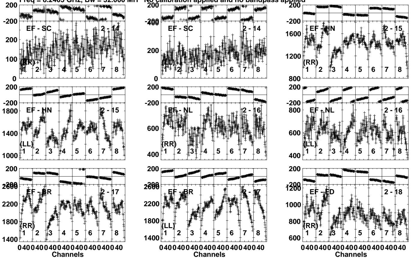
Lower frame: Micro Ampl Jy Top frame: Phas deg Vector averaged cross-power spectrum Several baselines displayed Timerange: 01/06:01:45 to 01/06:06:44
