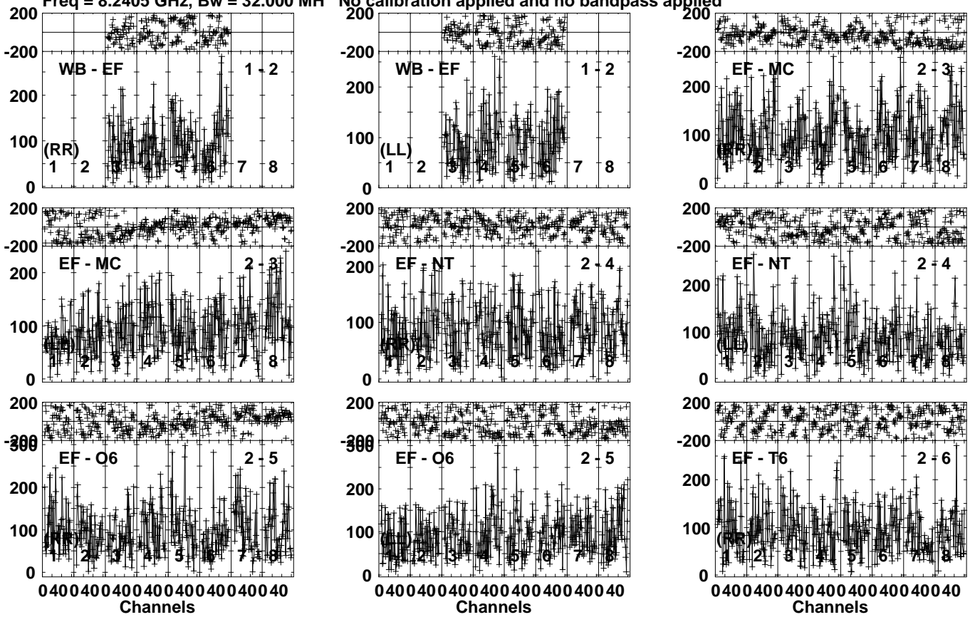
Lower frame: Micro Ampl Jy Top frame: Phas deg Vector averaged cross-power spectrum Several baselines displayed Timerange: 01/00:46:35 to 01/00:49:05
