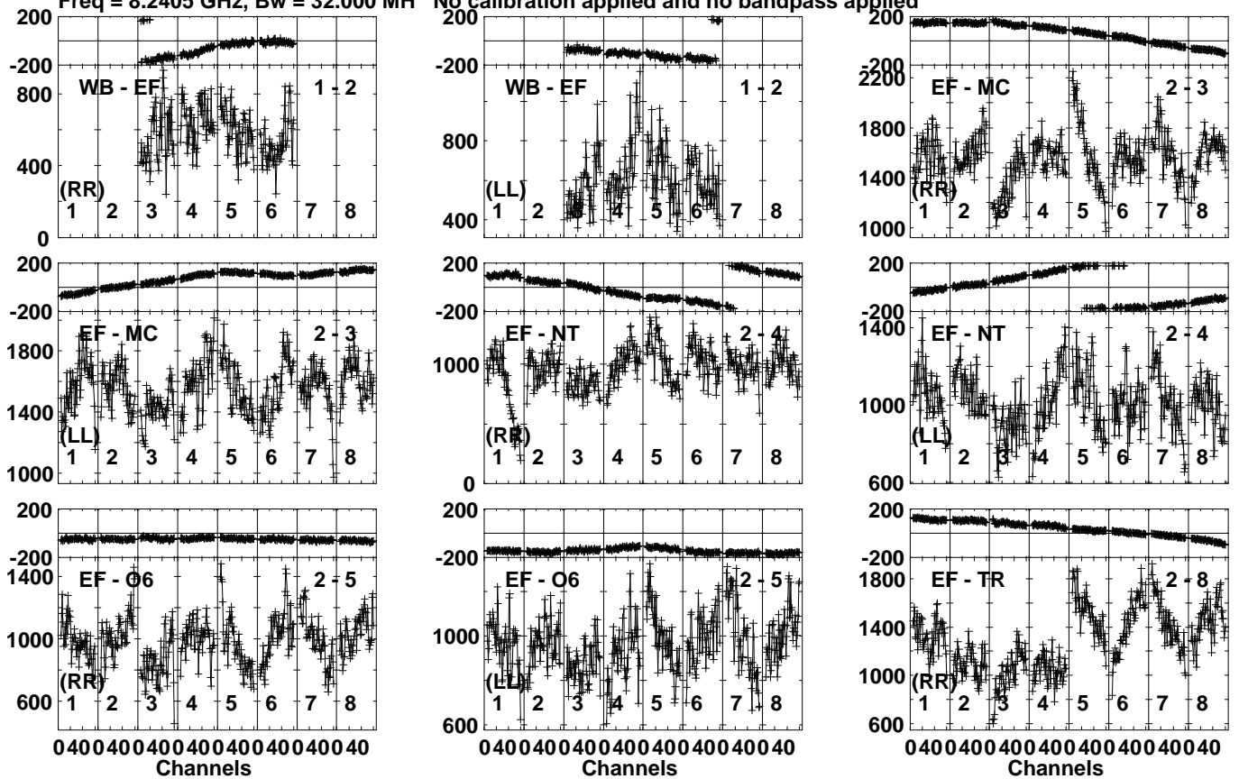
Lower frame: Micro Ampl Jy Top frame: Phas deg Vector averaged cross-power spectrum Several baselines displayed Timerange: 01/06:35:42 to 01/06:37:11
