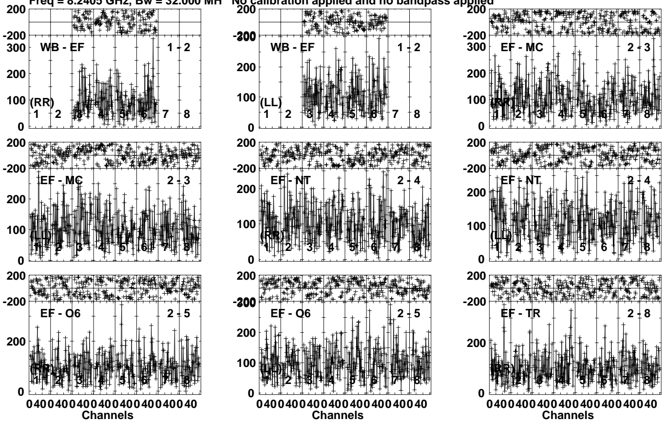
Lower frame: Micro Ampl Jy Top frame: Phas deg Vector averaged cross-power spectrum Several baselines displayed Timerange: 01/06:28:41 to 01/06:30:40
