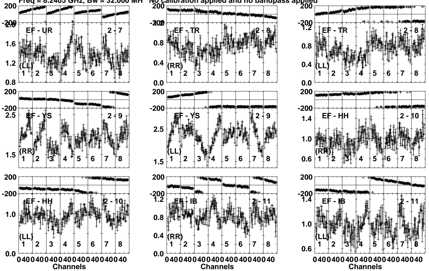
Lower frame: Milli Ampl Jy Top frame: Phas deg Vector averaged cross-power spectrum Several baselines displayed Timerange: 01/02:58:38 to 01/02:59:37
