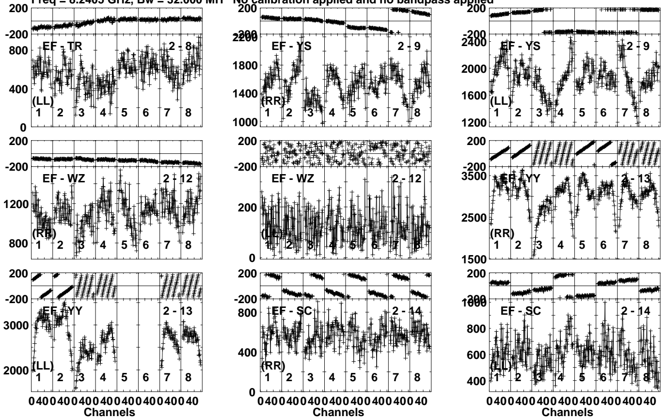
Lower frame: Micro Ampl Jy Top frame: Phas deg Vector averaged cross-power spectrum Several baselines displayed Timerange: 01/10:16:33 to 01/10:18:01
