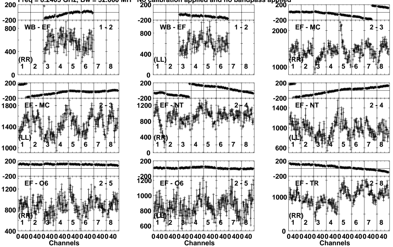
Lower frame: Micro Ampl Jy Top frame: Phas deg Vector averaged cross-power spectrum Several baselines displayed Timerange: 01/07:38:46 to 01/07:40:14
