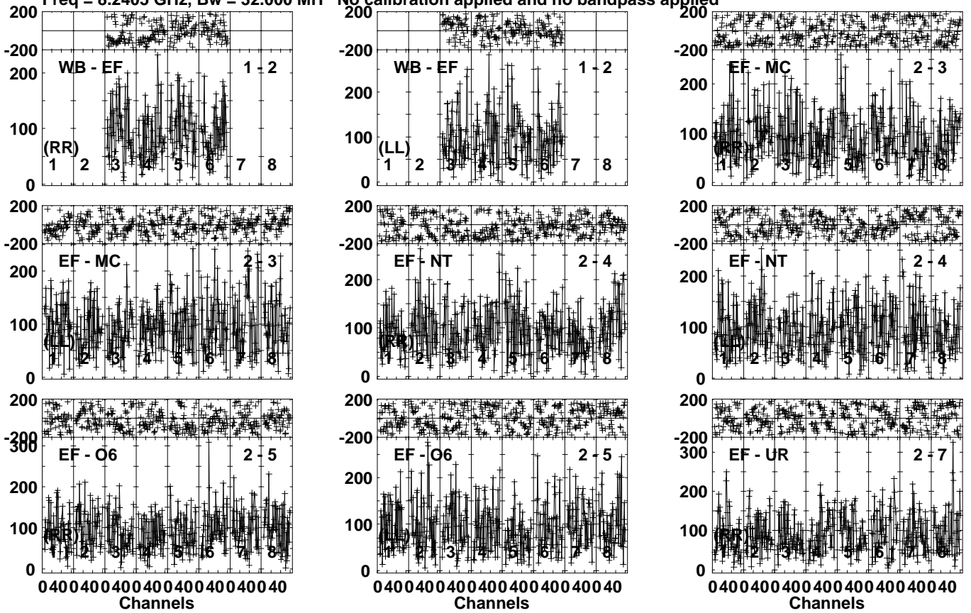
Lower frame: Micro Ampl Jy Top frame: Phas deg Vector averaged cross-power spectrum Several baselines displayed Timerange: 01/03:22:22 to 01/03:24:50
