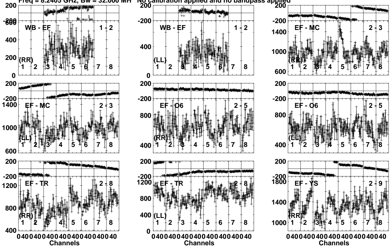
Lower frame: Micro Ampl Jy Top frame: Phas deg Vector averaged cross-power spectrum Several baselines displayed Timerange: 01/10:25:21 to 01/10:26:49
