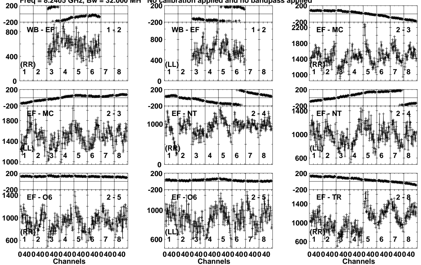
Lower frame: Micro Ampl Jy Top frame: Phas deg Vector averaged cross-power spectrum Several baselines displayed Timerange: 01/07:29:49 to 01/07:31:19
