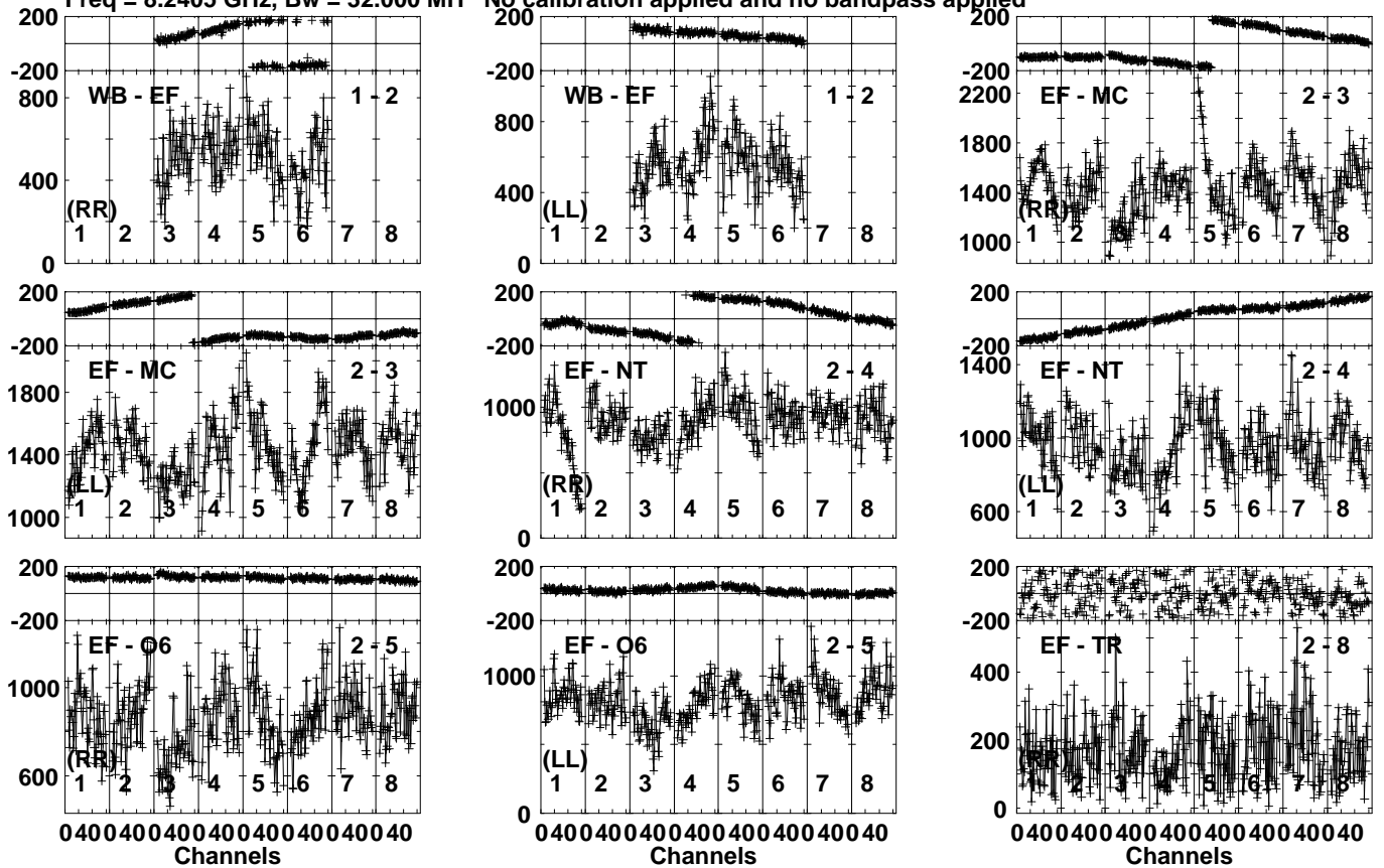
Lower frame: Micro Ampl Jy Top frame: Phas deg Vector averaged cross-power spectrum Several baselines displayed Timerange: 01/07:56:34 to 01/07:57:33
