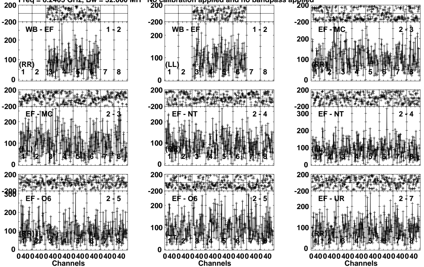
Lower frame: Micro Ampl Jy Top frame: Phas deg Vector averaged cross-power spectrum Several baselines displayed Timerange: 01/04:40:05 to 01/04:42:35
