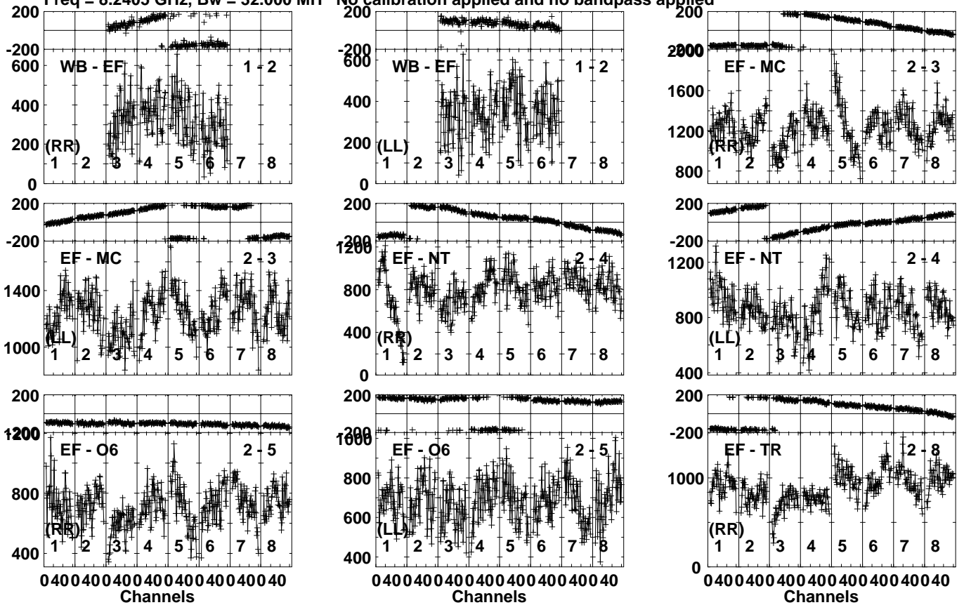
Lower frame: Micro Ampl Jy Top frame: Phas deg Vector averaged cross-power spectrum Several baselines displayed Timerange: 01/09:33:10 to 01/09:34:38
