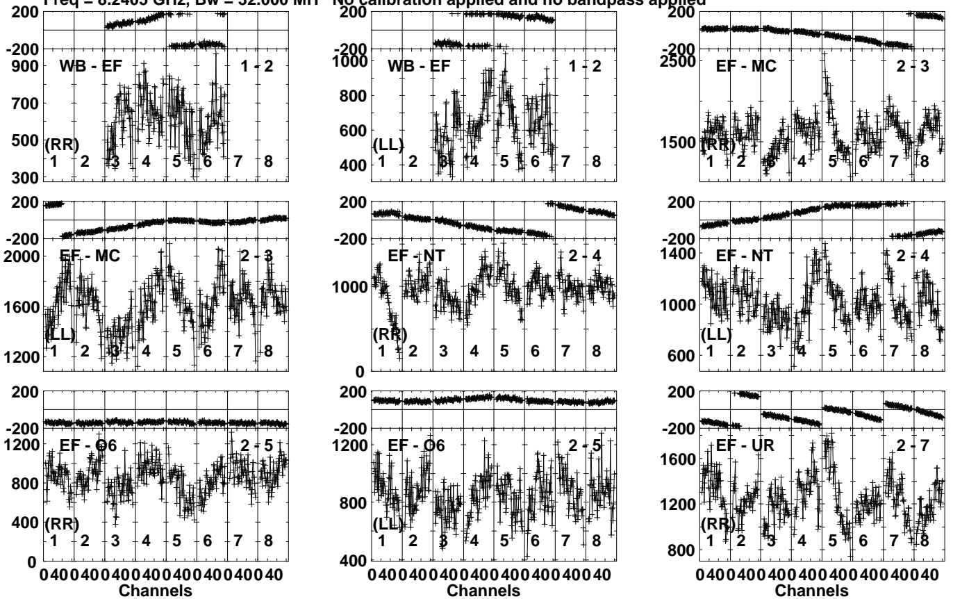
Lower frame: Micro Ampl Jy Top frame: Phas deg Vector averaged cross-power spectrum Several baselines displayed Timerange: 01/04:20:22 to 01/04:21:21
