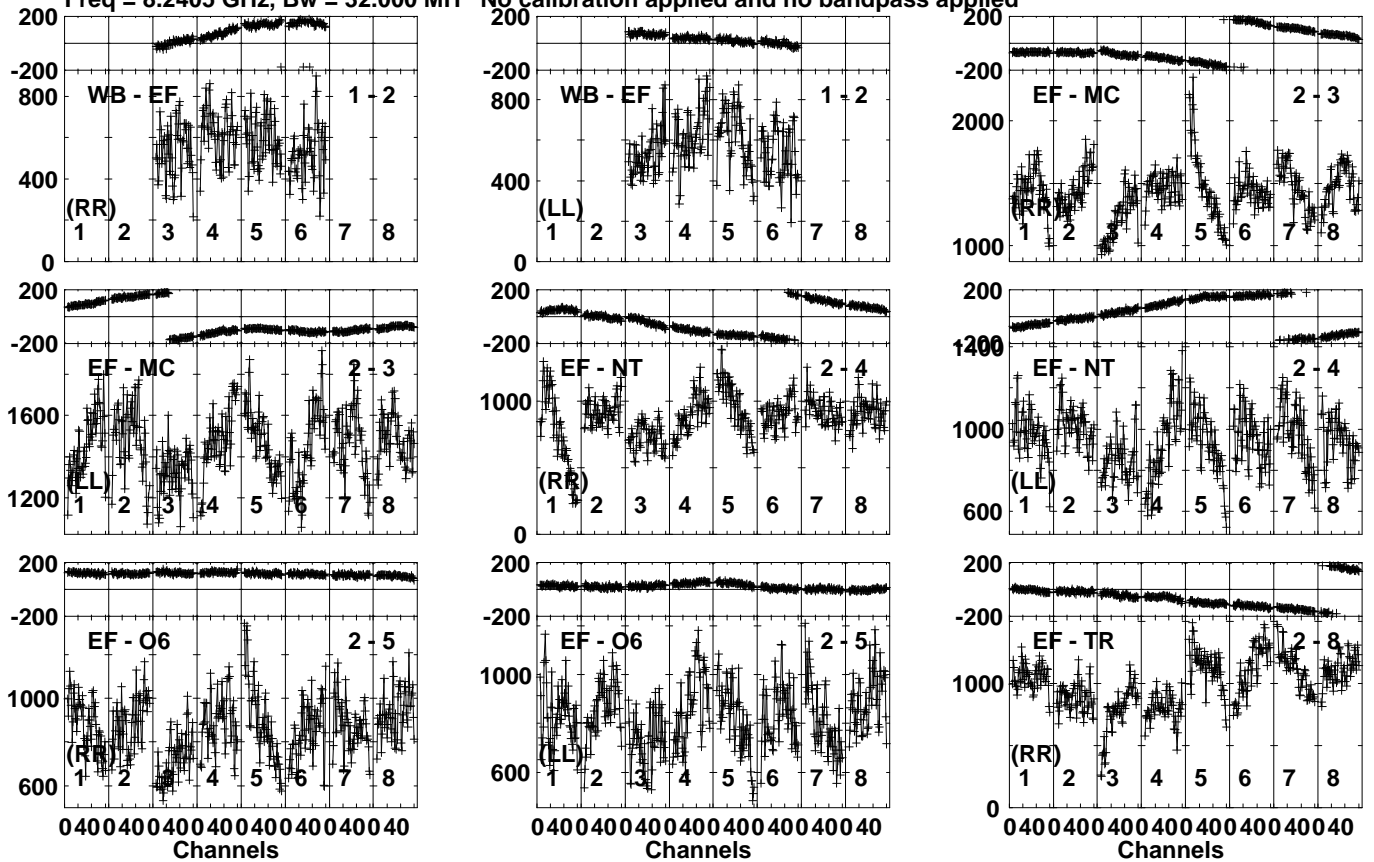
Lower frame: Micro Ampl Jy Top frame: Phas deg Vector averaged cross-power spectrum Several baselines displayed Timerange: 01/07:52:08 to 01/07:53:36
