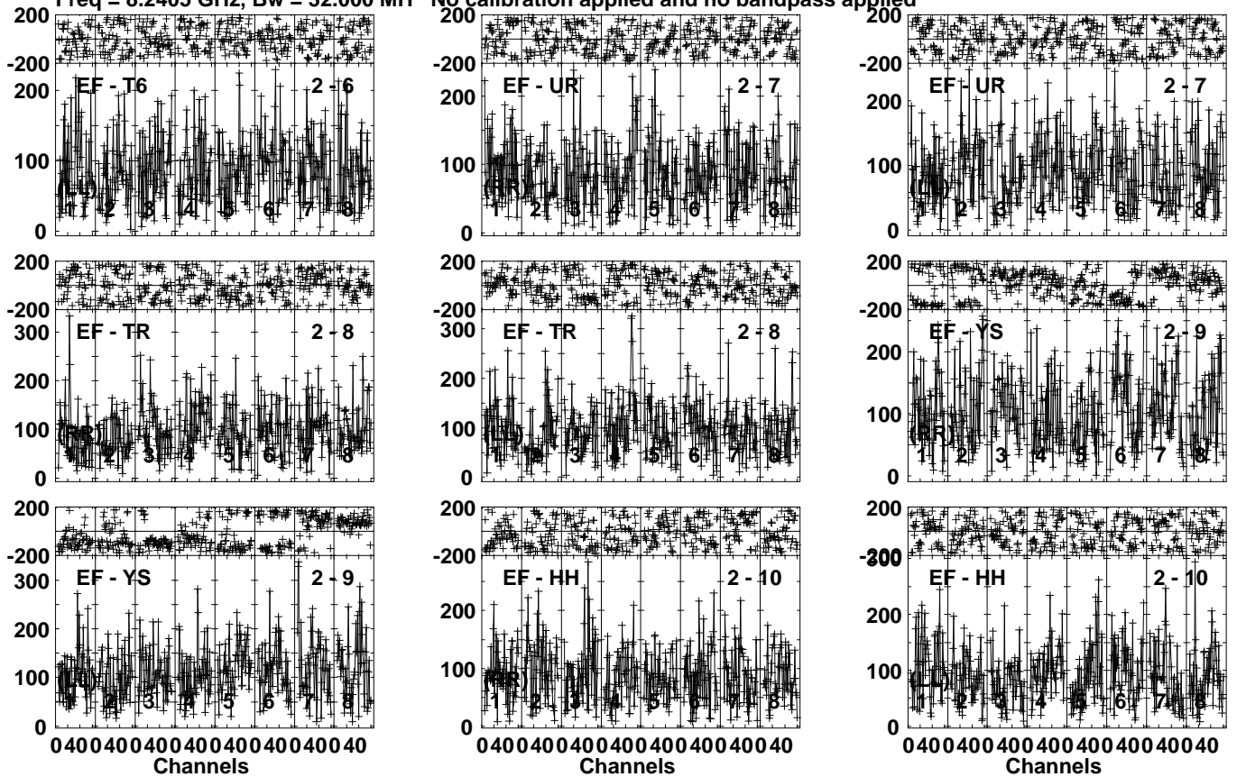
Lower frame: Micro Ampl Jy Top frame: Phas deg Vector averaged cross-power spectrum Several baselines displayed Timerange: 01/02:05:57 to 01/02:08:27
