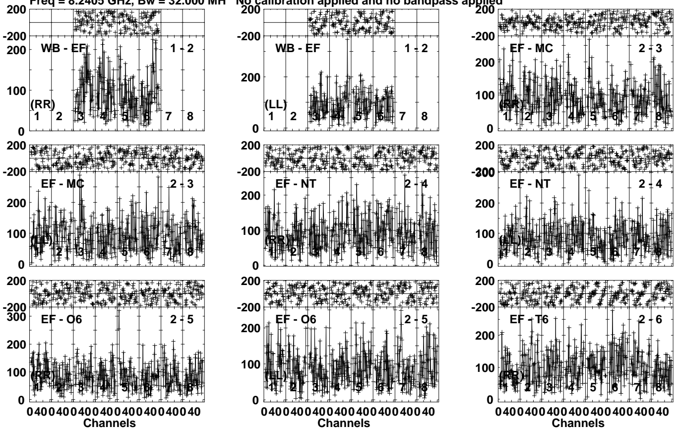
Lower frame: Micro Ampl Jy Top frame: Phas deg Vector averaged cross-power spectrum Several baselines displayed Timerange: 00/23:49:08 to 00/23:51:36
