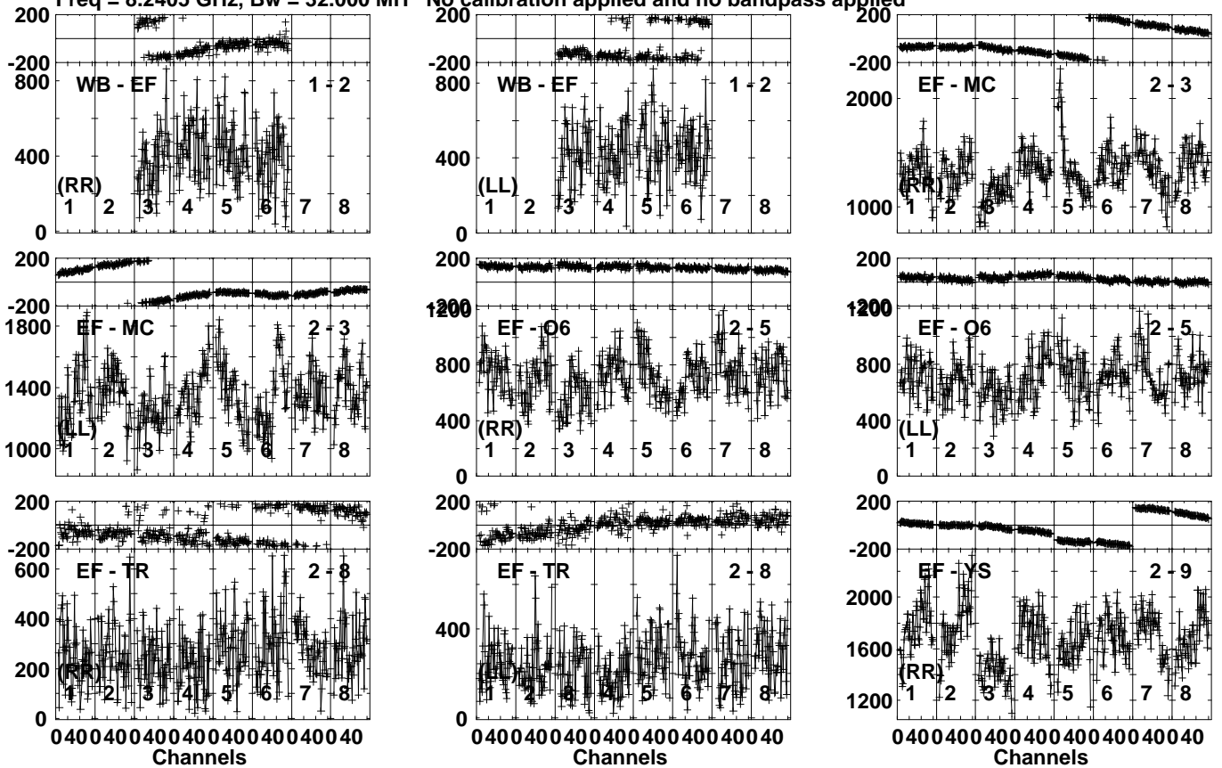
Lower frame: Micro Ampl Jy Top frame: Phas deg Vector averaged cross-power spectrum Several baselines displayed Timerange: 01/09:02:16 to 01/09:03:44
