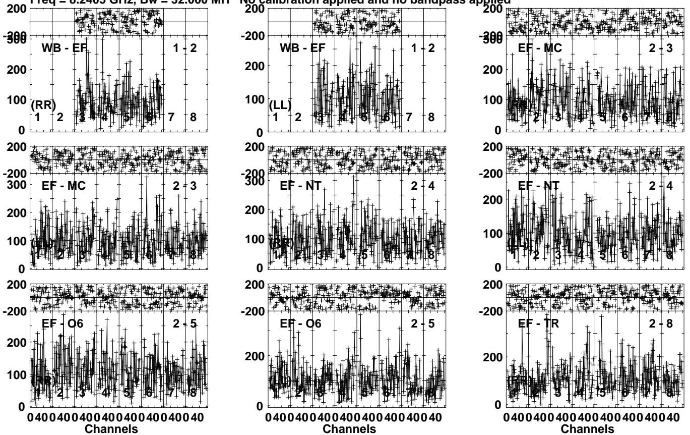
Lower frame: Micro Ampl Jy Top frame: Phas deg Vector averaged cross-power spectrum Several baselines displayed Timerange: 01/10:09:40 to 01/10:11:39
