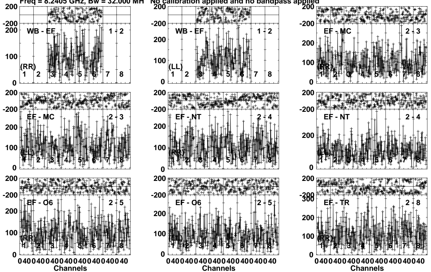
Lower frame: Micro Ampl Jy Top frame: Phas deg Vector averaged cross-power spectrum Several baselines displayed Timerange: 01/09:30:42 to 01/09:32:42
