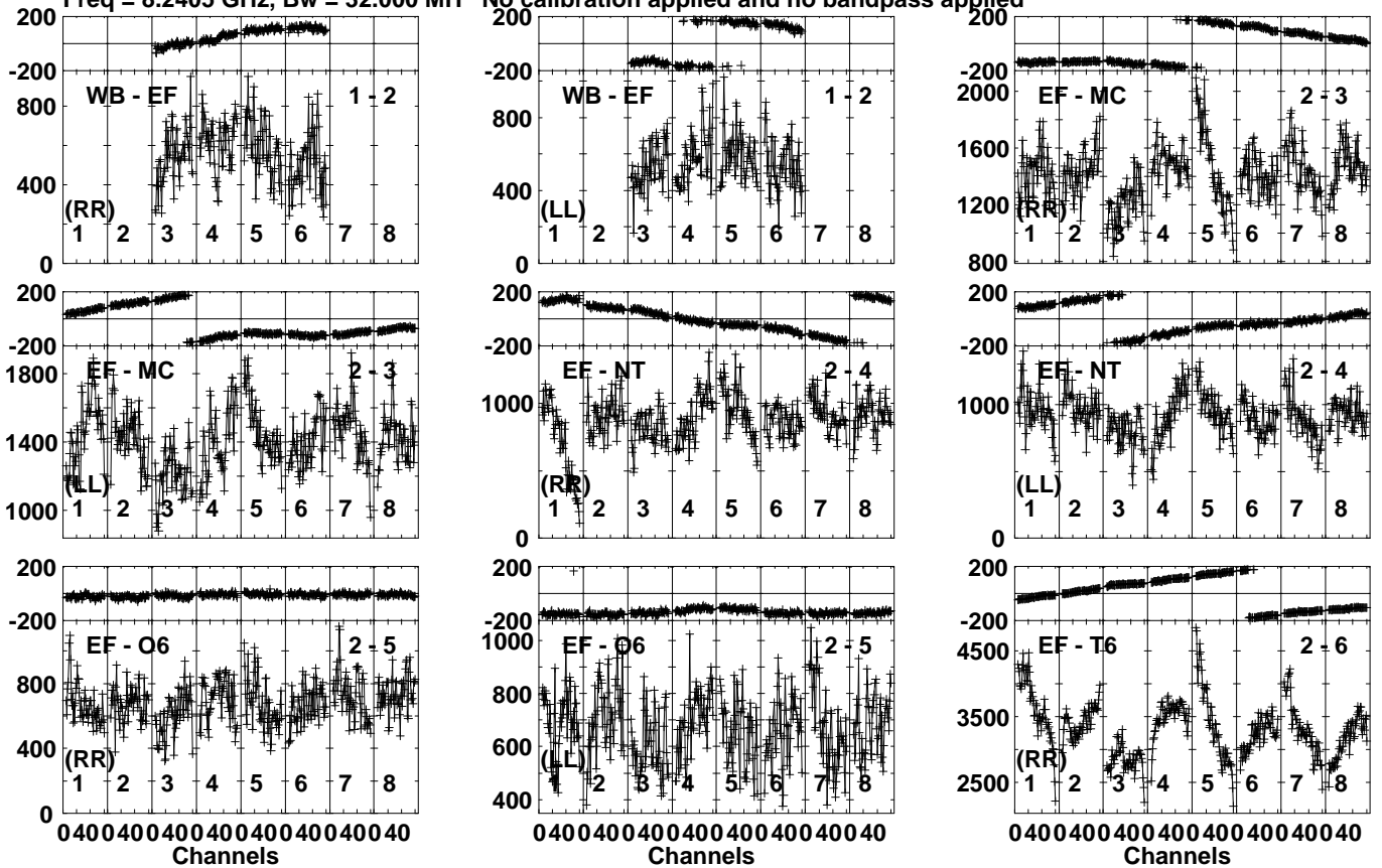
Lower frame: Micro Ampl Jy Top frame: Phas deg Vector averaged cross-power spectrum Several baselines displayed Timerange: 01/00:14:02 to 01/00:15:01
