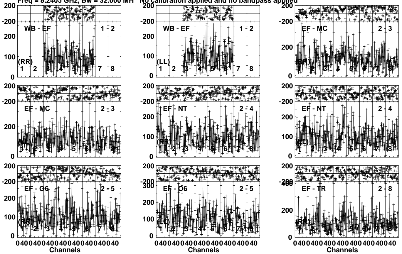
Lower frame: Micro Ampl Jy Top frame: Phas deg Vector averaged cross-power spectrum Several baselines displayed Timerange: 01/07:45:12 to 01/07:47:11
