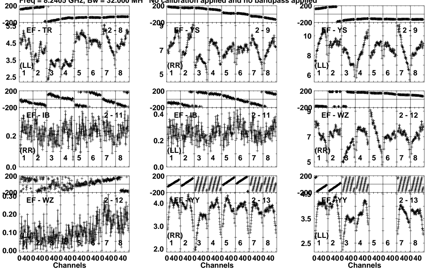
Lower frame: Milli Ampl Jy Top frame: Phas deg Vector averaged cross-power spectrum Several baselines displayed Timerange: 01/06:01:45 to 01/06:06:44
