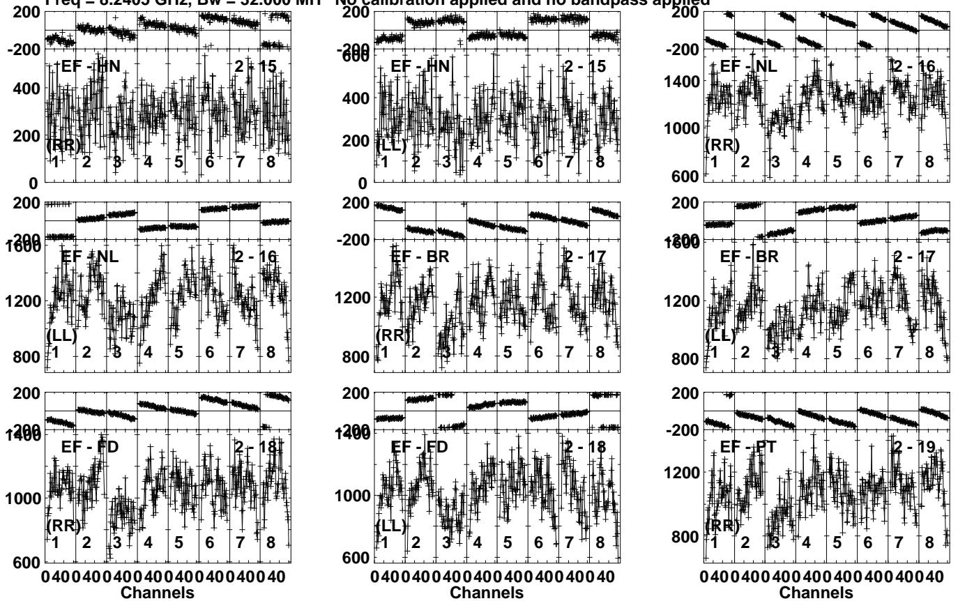
Lower frame: Micro Ampl Jy Top frame: Phas deg Vector averaged cross-power spectrum Several baselines displayed Timerange: 01/10:07:44 to 01/10:09:13
