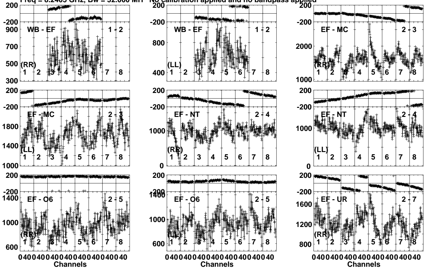
Lower frame: Micro Ampl Jy Top frame: Phas deg Vector averaged cross-power spectrum Several baselines displayed Timerange: 01/04:38:35 to 01/04:39:33
