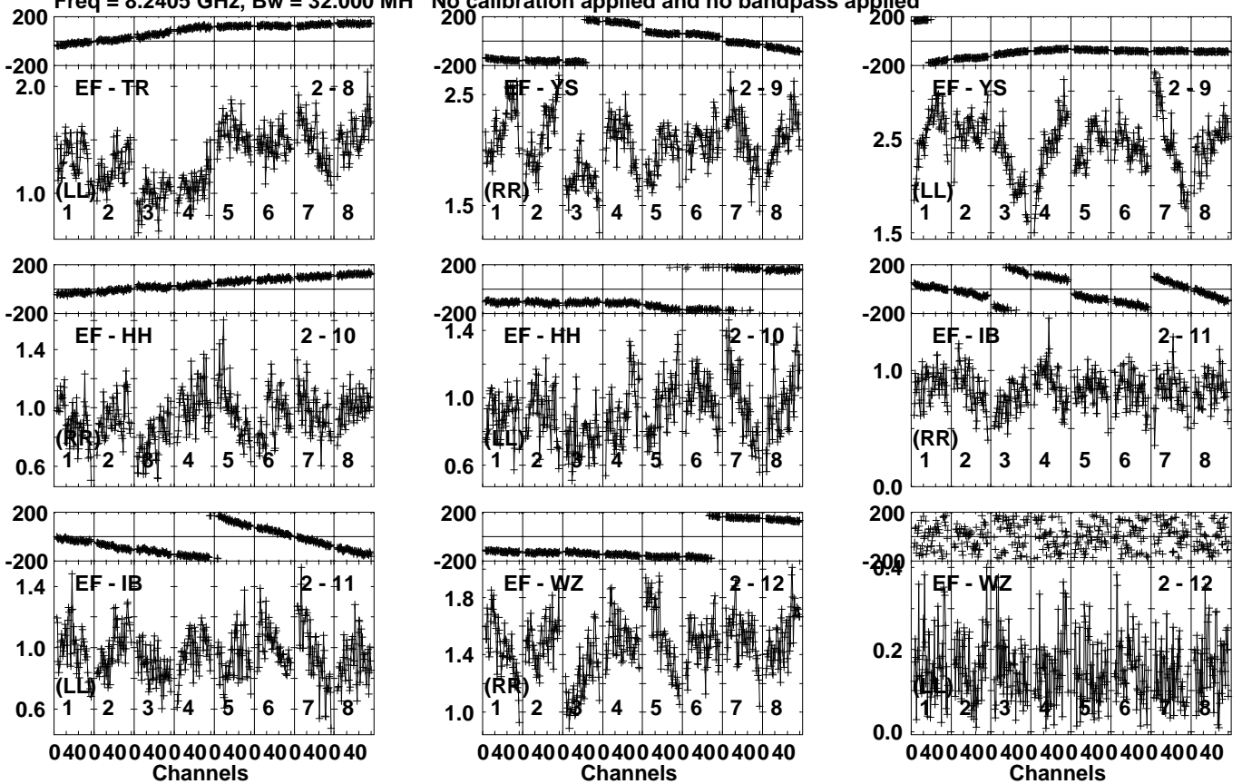
Lower frame: Milli Ampl Jy Top frame: Phas deg Vector averaged cross-power spectrum Several baselines displayed Timerange: 01/06:08:35 to 01/06:10:04
