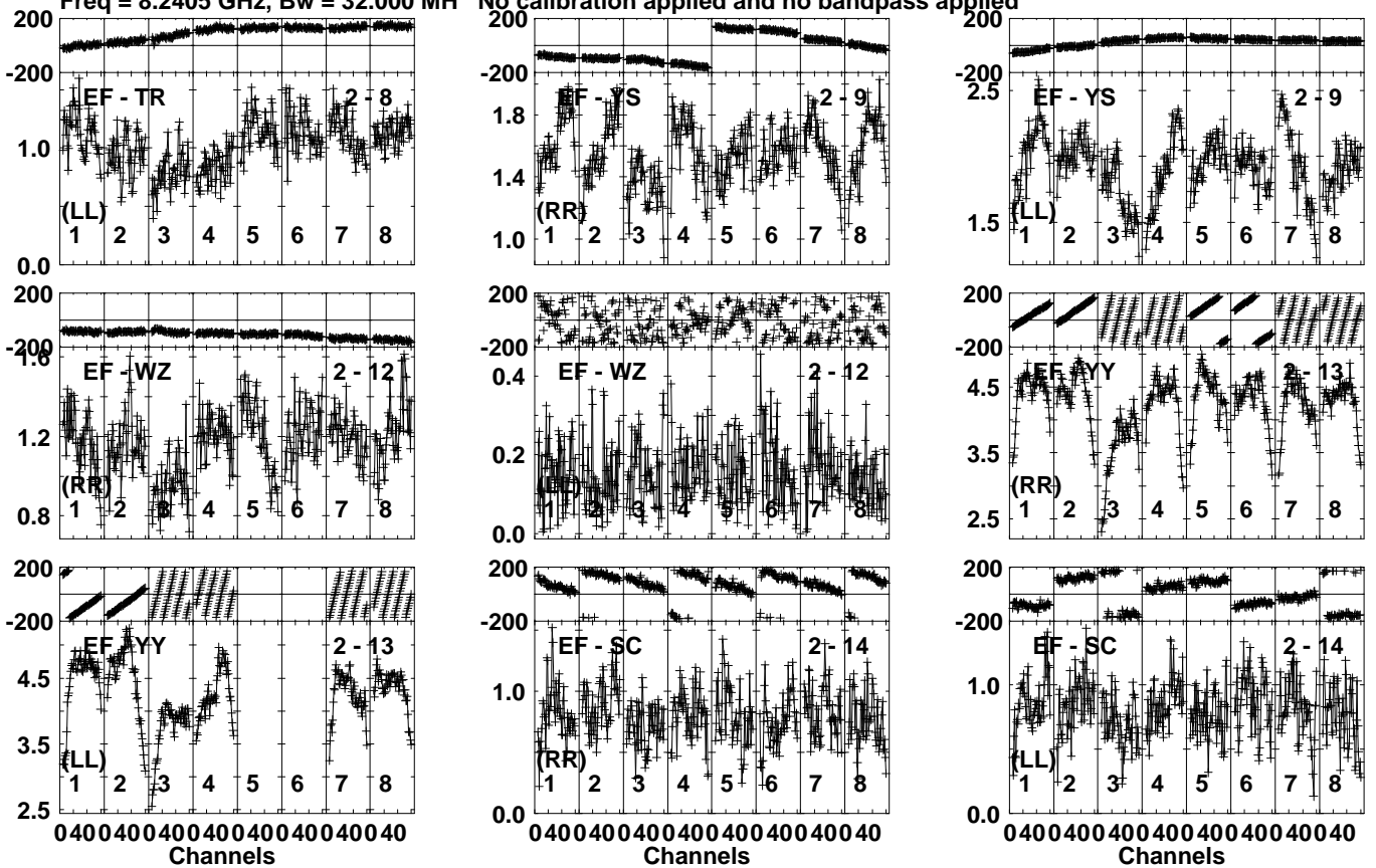
Lower frame: Milli Ampl Jy Top frame: Phas deg Vector averaged cross-power spectrum Several baselines displayed Timerange: 01/09:50:49 to 01/09:51:47
