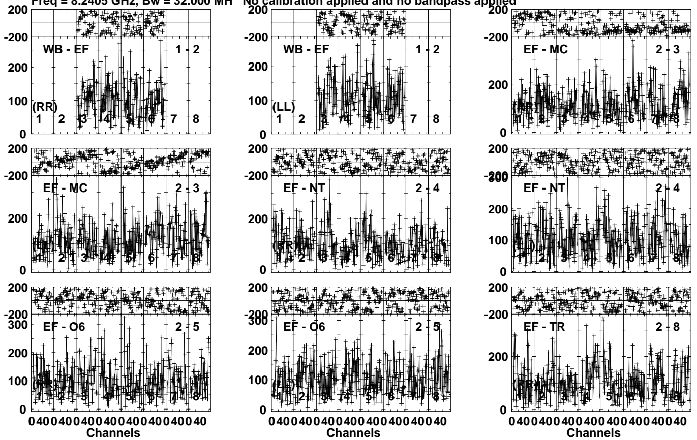
Lower frame: Micro Ampl Jy Top frame: Phas deg Vector averaged cross-power spectrum Several baselines displayed Timerange: 01/06:51:11 to 01/06:53:11
