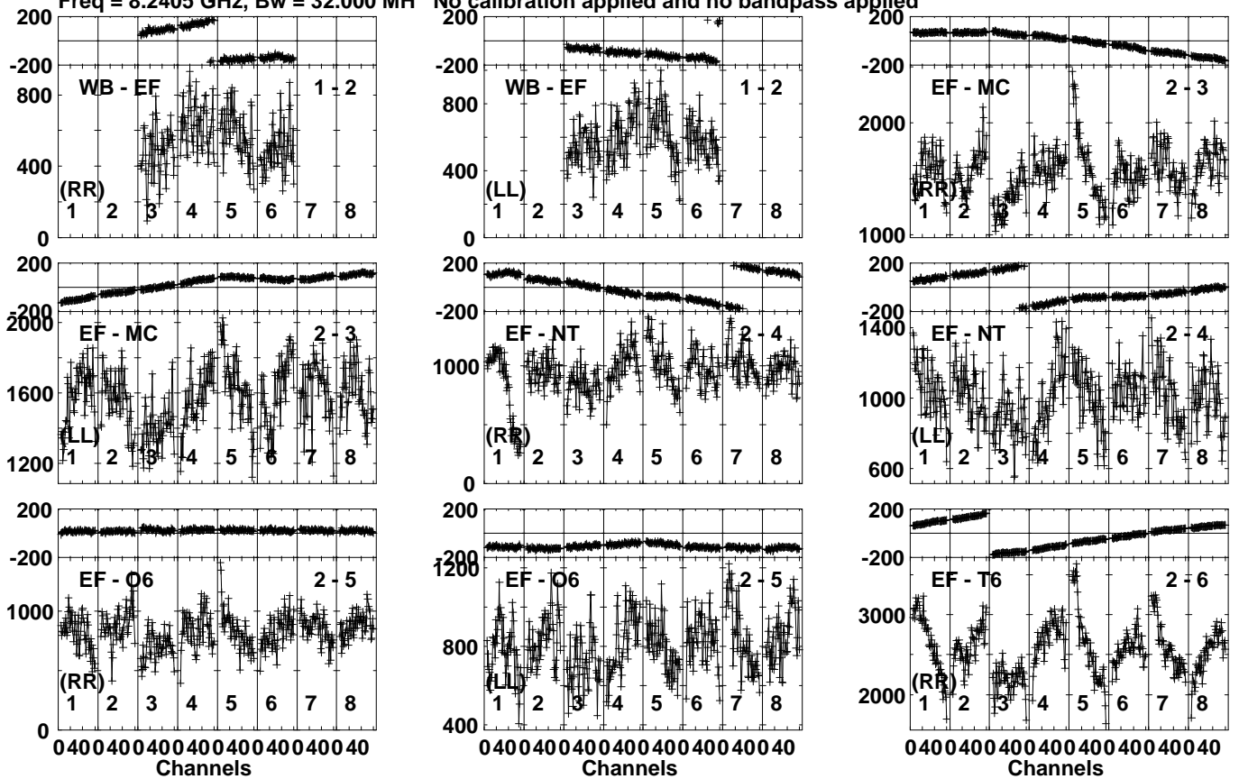
Lower frame: Micro Ampl Jy Top frame: Phas deg Vector averaged cross-power spectrum Several baselines displayed Timerange: 01/02:26:24 to 01/02:27:23
