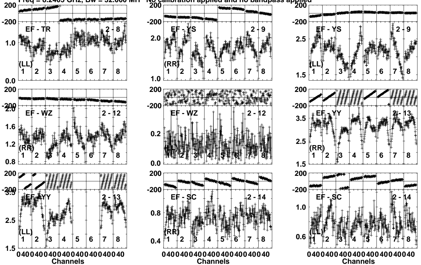
Lower frame: Milli Ampl Jy Top frame: Phas deg Vector averaged cross-power spectrum Several baselines displayed Timerange: 01/08:40:08 to 01/08:41:36
