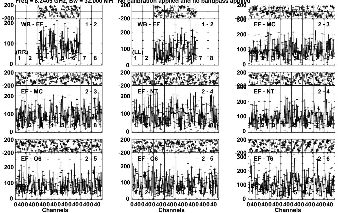
Lower frame: Micro Ampl Jy Top frame: Phas deg Vector averaged cross-power spectrum Several baselines displayed Timerange: 01/00:19:50 to 01/00:22:20
