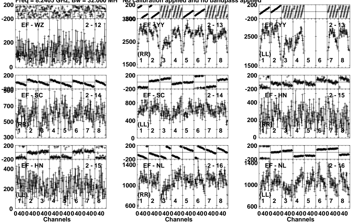
Lower frame: Micro Ampl Jy Top frame: Phas deg Vector averaged cross-power spectrum Several baselines displayed Timerange: 01/10:29:45 to 01/10:31:13
