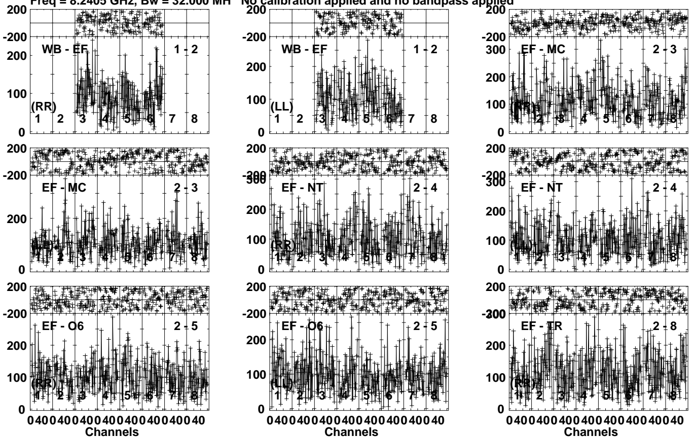
Lower frame: Micro Ampl Jy Top frame: Phas deg Vector averaged cross-power spectrum Several baselines displayed Timerange: 01/08:42:05 to 01/08:44:04
