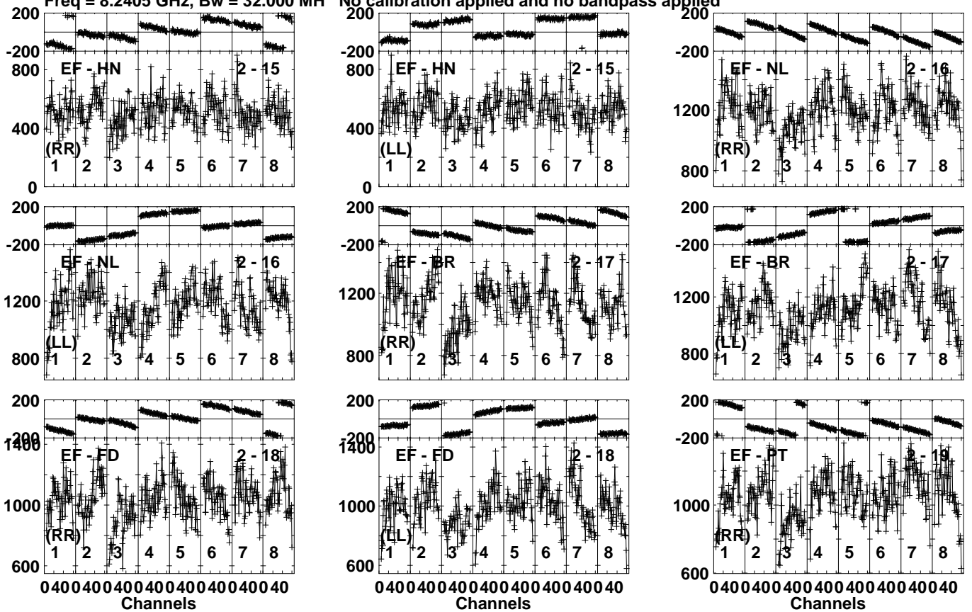
Lower frame: Micro Ampl Jy Top frame: Phas deg Vector averaged cross-power spectrum Several baselines displayed Timerange: 01/09:37:34 to 01/09:39:03
