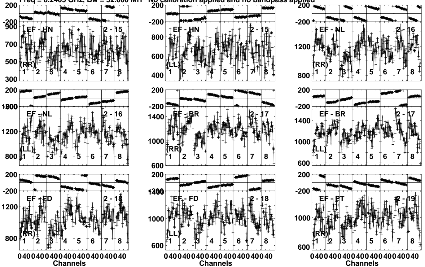
Lower frame: Micro Ampl Jy Top frame: Phas deg Vector averaged cross-power spectrum Several baselines displayed Timerange: 01/08:49:00 to 01/08:50:28
