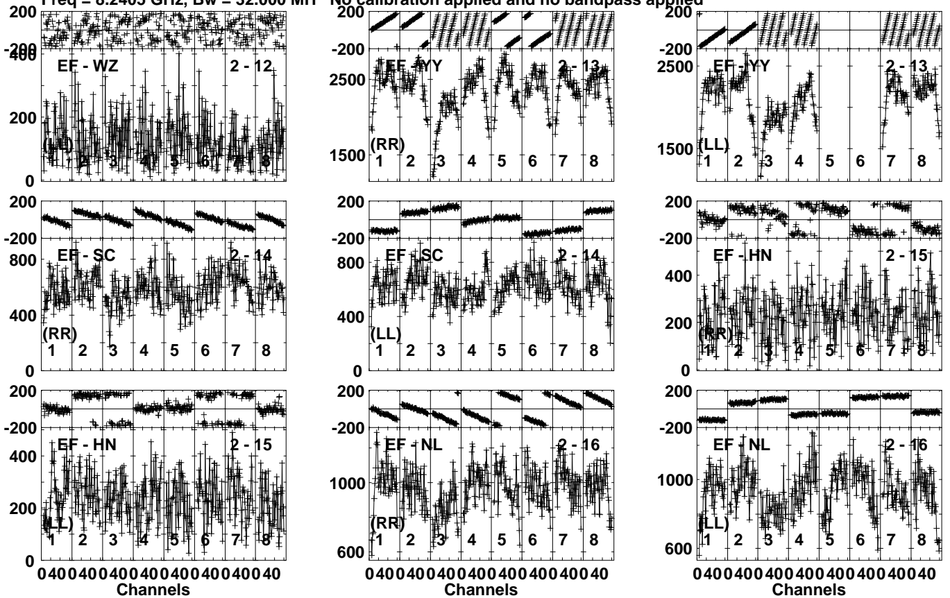
Lower frame: Micro Ampl Jy Top frame: Phas deg Vector averaged cross-power spectrum Several baselines displayed Timerange: 01/10:42:58 to 01/10:44:26
