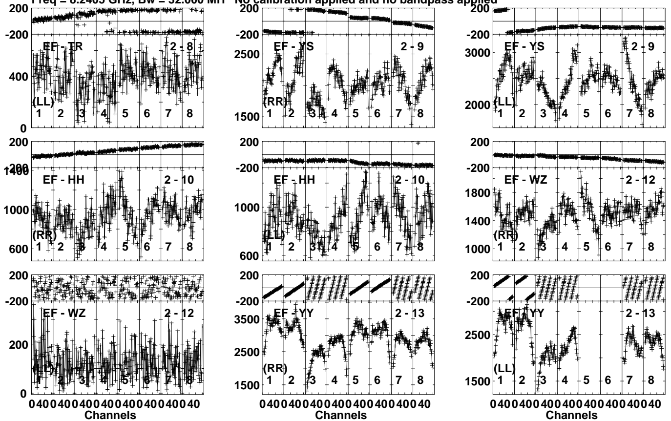
Lower frame: Micro Ampl Jy Top frame: Phas deg Vector averaged cross-power spectrum Several baselines displayed Timerange: 01/06:31:12 to 01/06:32:41
