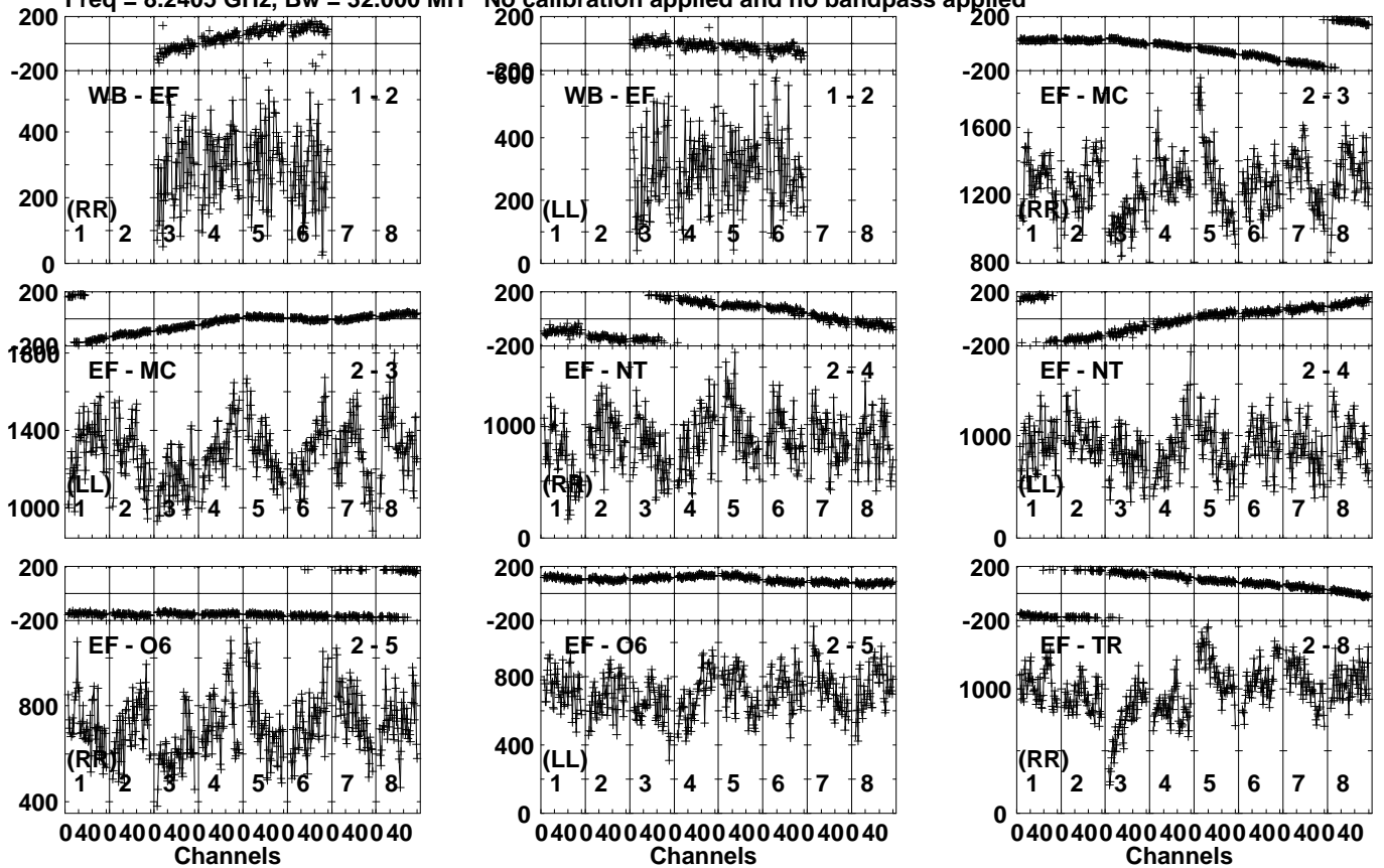
Lower frame: Micro Ampl Jy Top frame: Phas deg Vector averaged cross-power spectrum Several baselines displayed Timerange: 01/09:19:56 to 01/09:21:24
