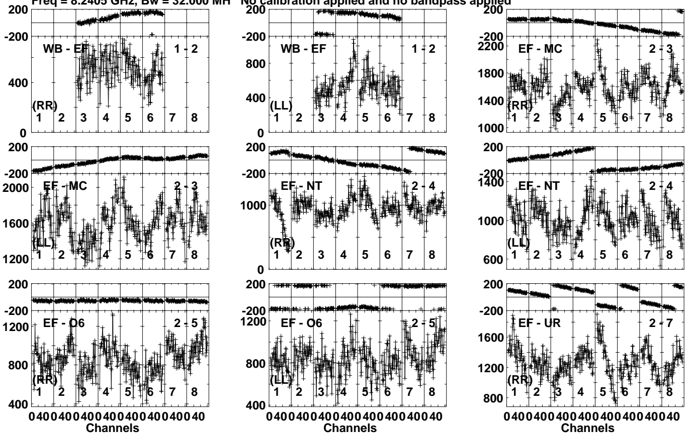
Lower frame: Micro Ampl Jy Top frame: Phas deg Vector averaged cross-power spectrum Several baselines displayed Timerange: 01/04:02:13 to 01/04:03:11
