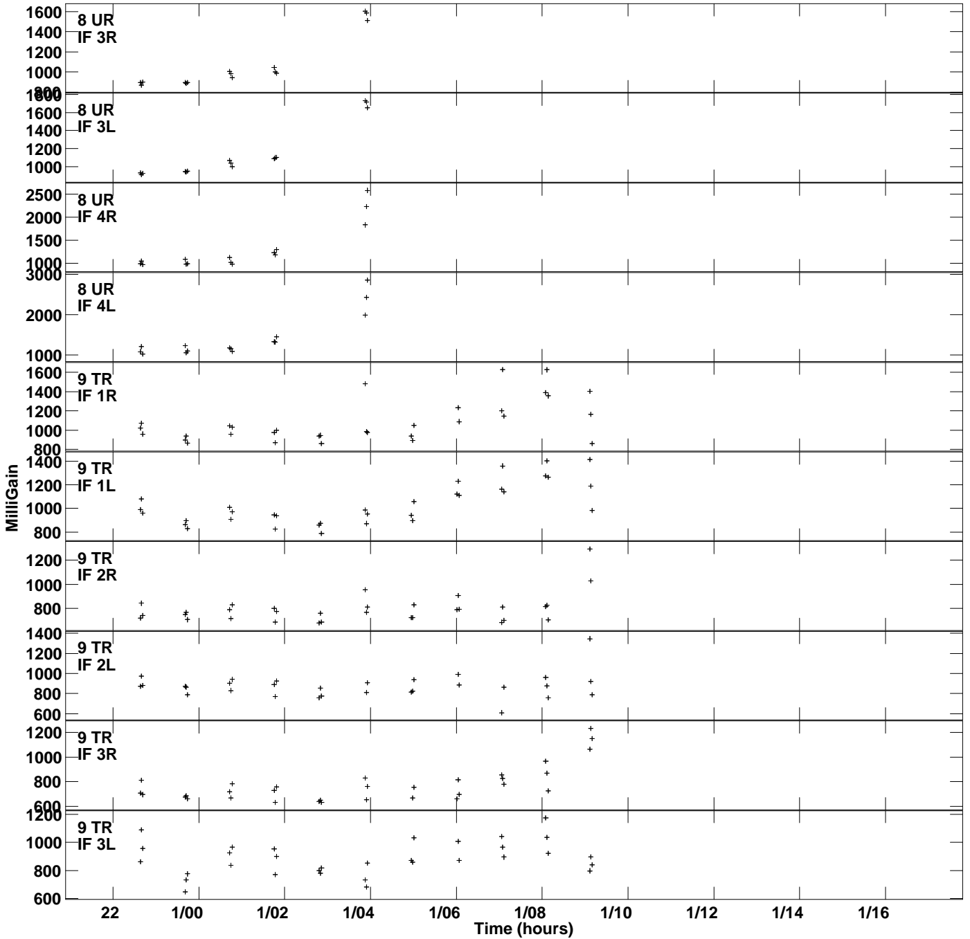
Plot file version 7 created 26-MAY-2023 12:38:33 Gain amp vs UTC time for OQ208.MULTI.1 SN 2 Rpol & Lpol IF 1 - 4
