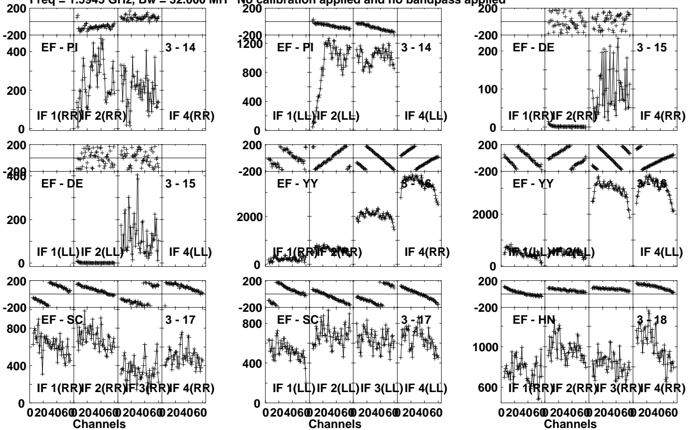
Lower frame: Micro Ampl Jy Top frame: Phas deg Vector averaged cross-power spectrum Several baselines displayed Timerange: 01/07:48:02 to 01/07:49:31
