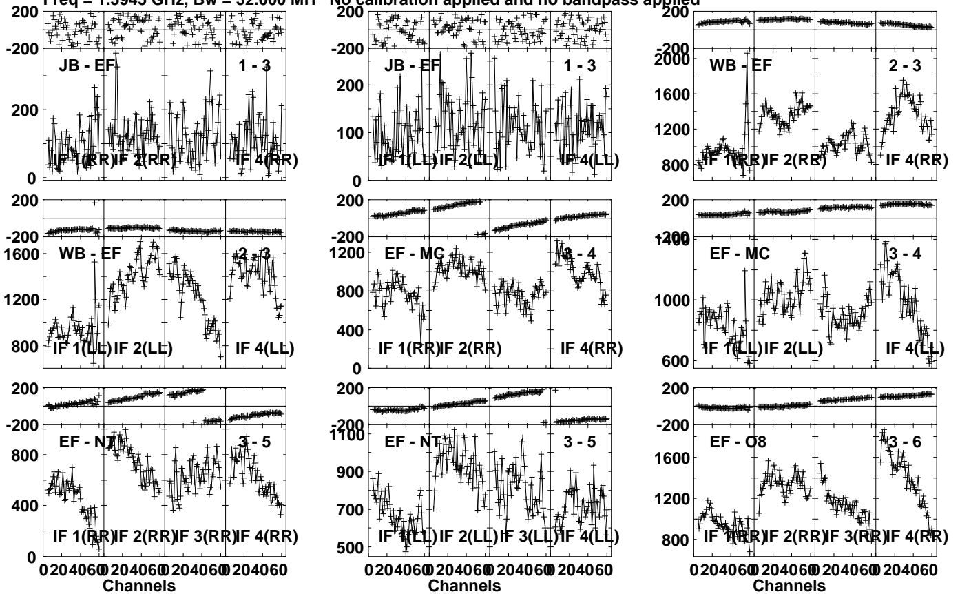
Lower frame: Micro Ampl Jy Top frame: Phas deg Vector averaged cross-power spectrum Several baselines displayed Timerange: 01/08:00:58 to 01/08:02:28
