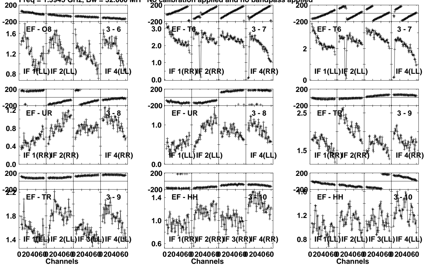
Lower frame: Milli Ampl Jy Top frame: Phas deg Vector averaged cross-power spectrum Several baselines displayed Timerange: 01/01:02:16 to 01/01:03:45
