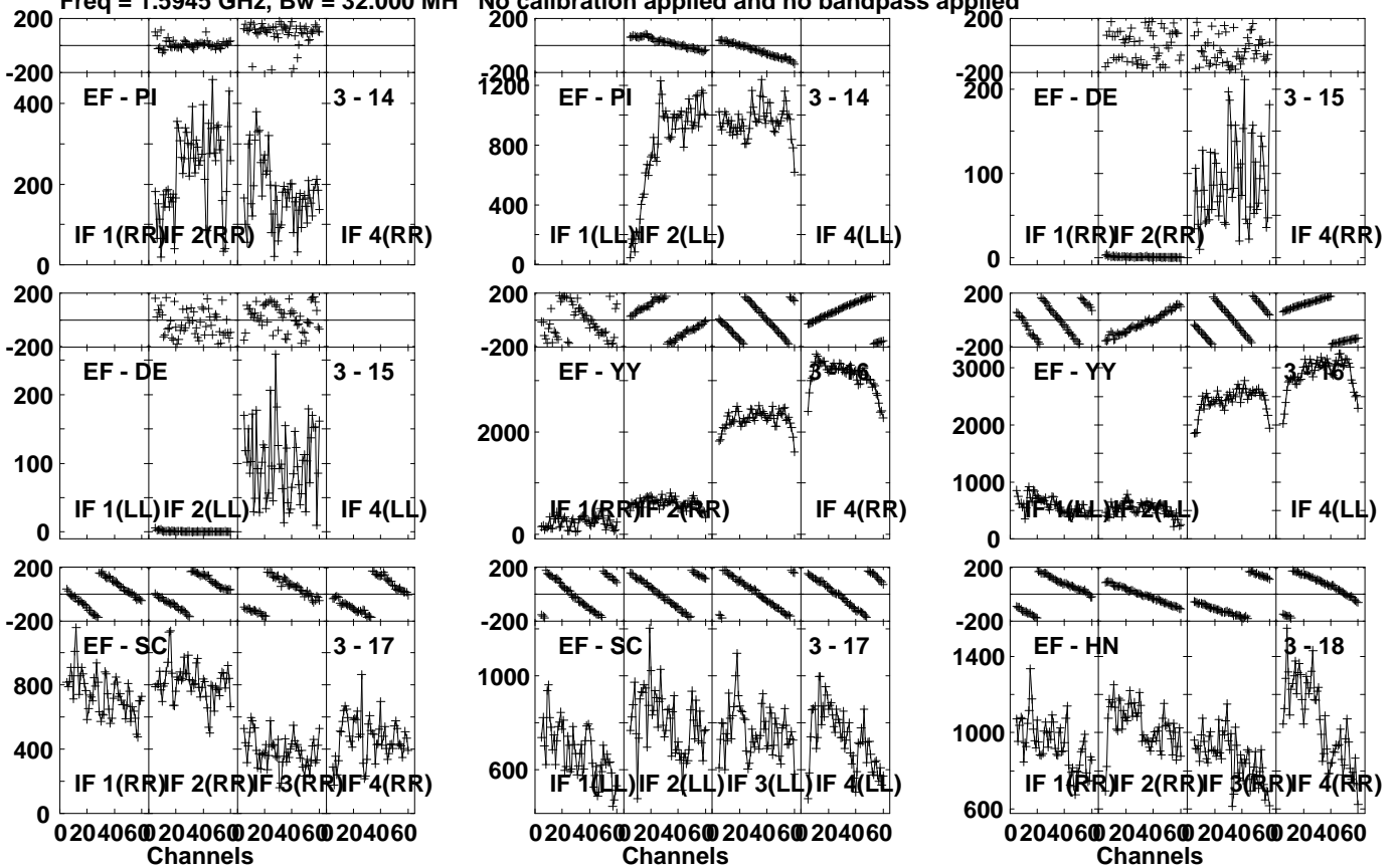
Lower frame: Micro Ampl Jy Top frame: Phas deg Vector averaged cross-power spectrum Several baselines displayed Timerange: 01/09:12:06 to 01/09:13:35
