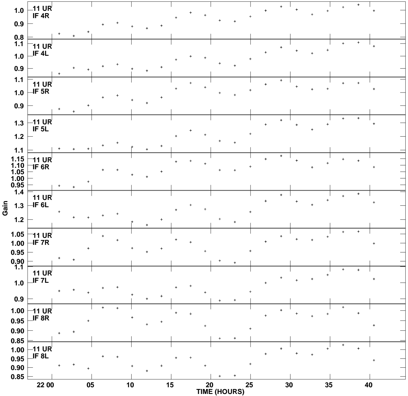
Plot file version 14 created 28-MAY-2010 15:38:40 Gain amp vs UTC time for OQ208.MULTI.1 SN 2 Rpol & Lpol IF 1 - 8
