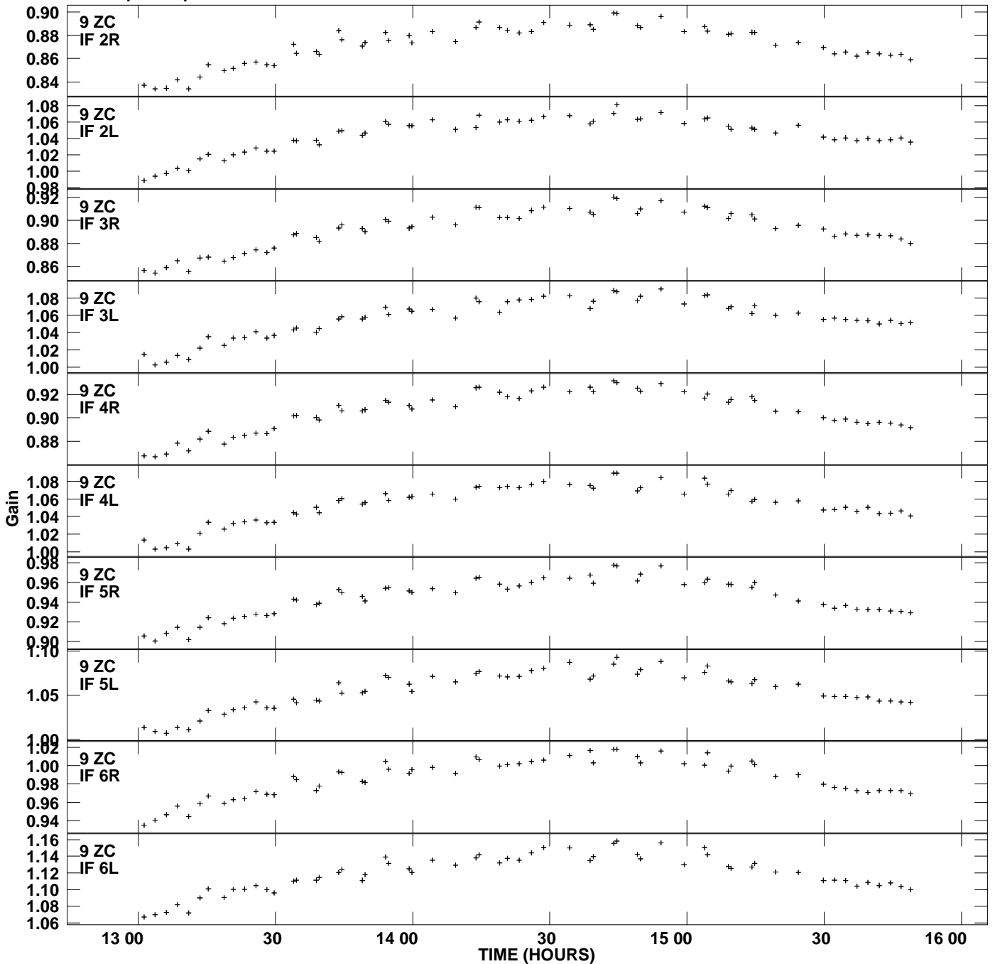
Plot file version 14 created 17-MAY-2012 02:12:17 Gain amp vs UTC time for 0528+134.MULTI.1 SN 2 Rpol & Lpol IF 1 - 8
