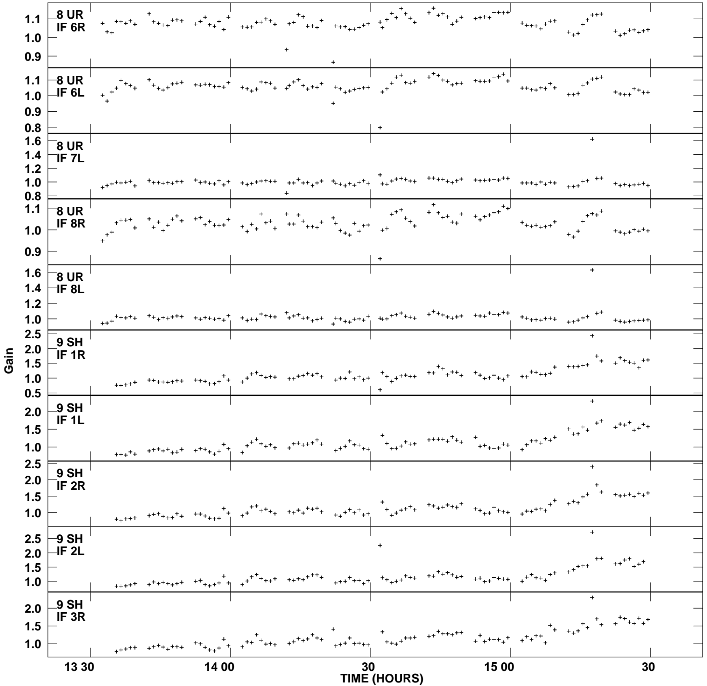
Plot file version 10 created 21-MAY-2012 22:35:51 Gain amp vs UTC time for 0528+134.MULTI.1 SN 2 Rpol & Lpol IF 1 - 8
