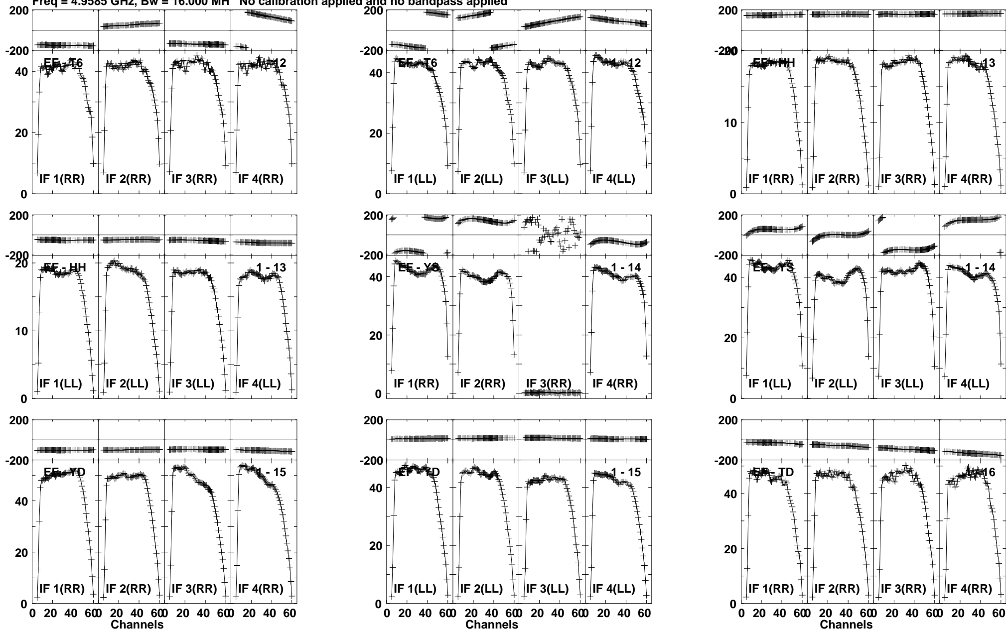
Lower frame: Milli Ampl Jy Top frame: Phas deg Vector averaged cross-power spectrum Baseline: EF (01) - T6 (12) Timerange: 00/18:15:01 to 00/18:15:59
