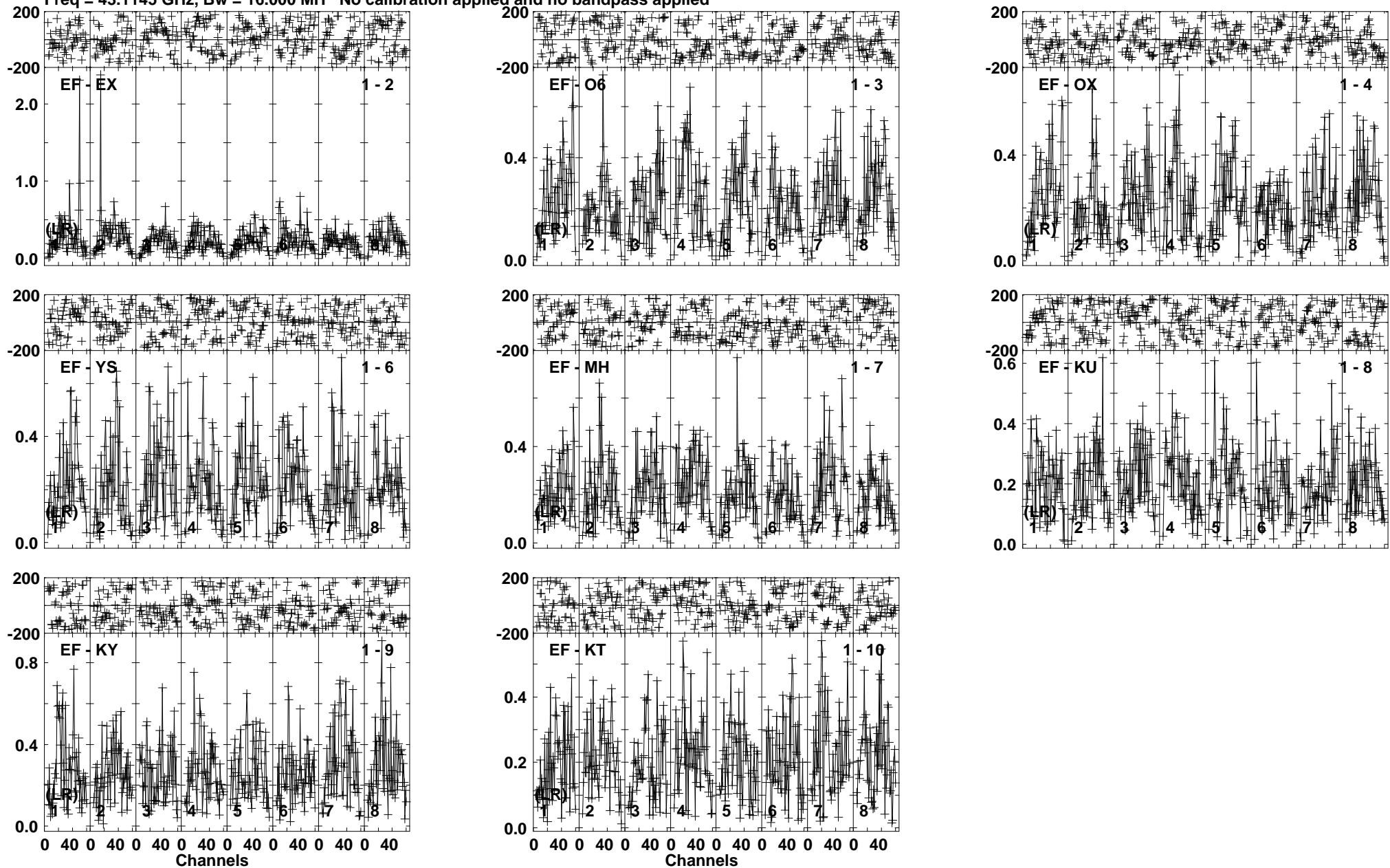
Lower frame: Milli Ampl Jy Top frame: Phas deg Vector averaged cross-power spectrum Baseline: EF (01) - EX (02) Timerange: 00/15:28:33 to 00/15:29:29
