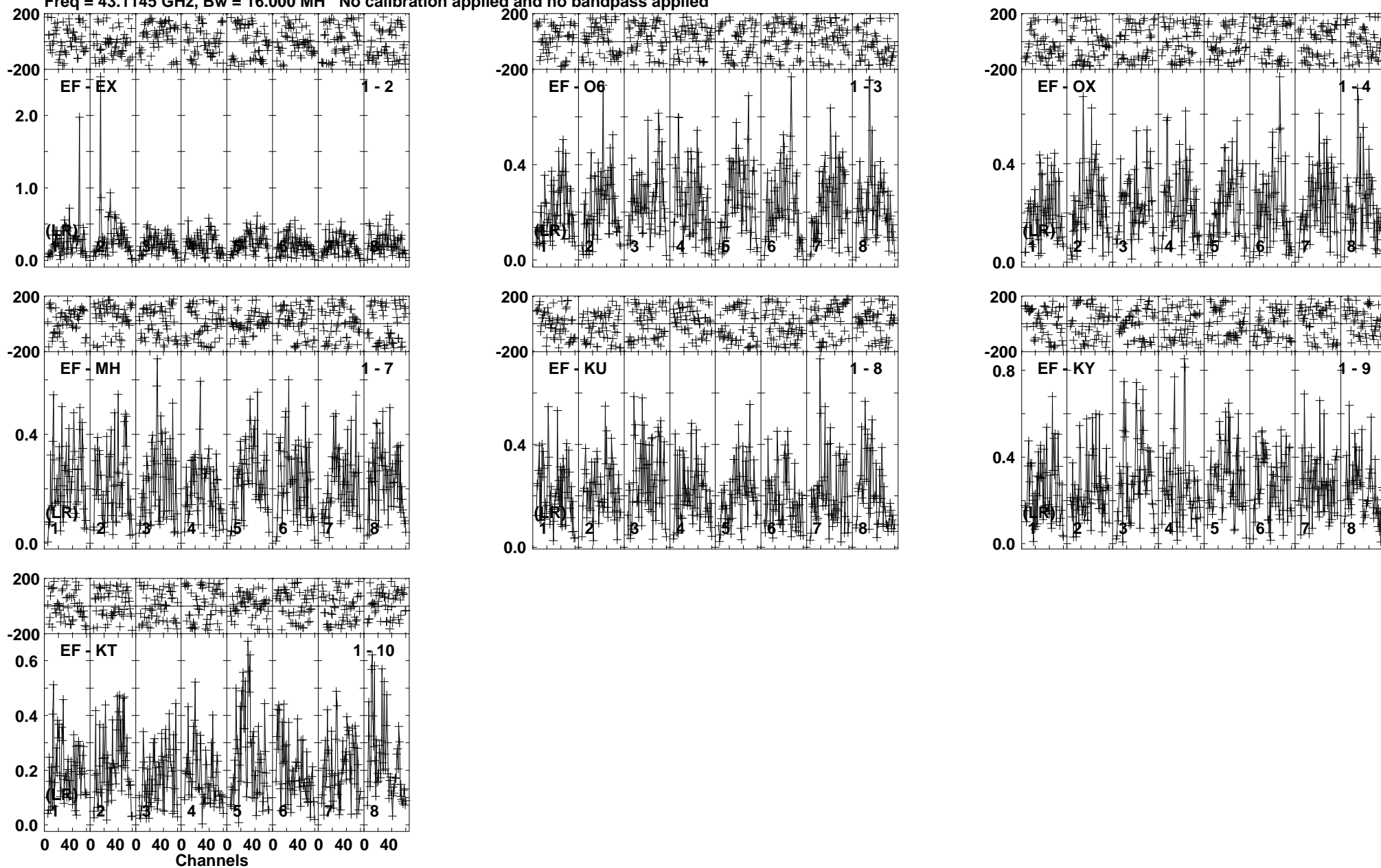
Lower frame: Milli Ampl Jy Top frame: Phas deg Vector averaged cross-power spectrum Baseline: EF (01) - EX (02) Timerange: 00/15:34:33 to 00/15:35:29
