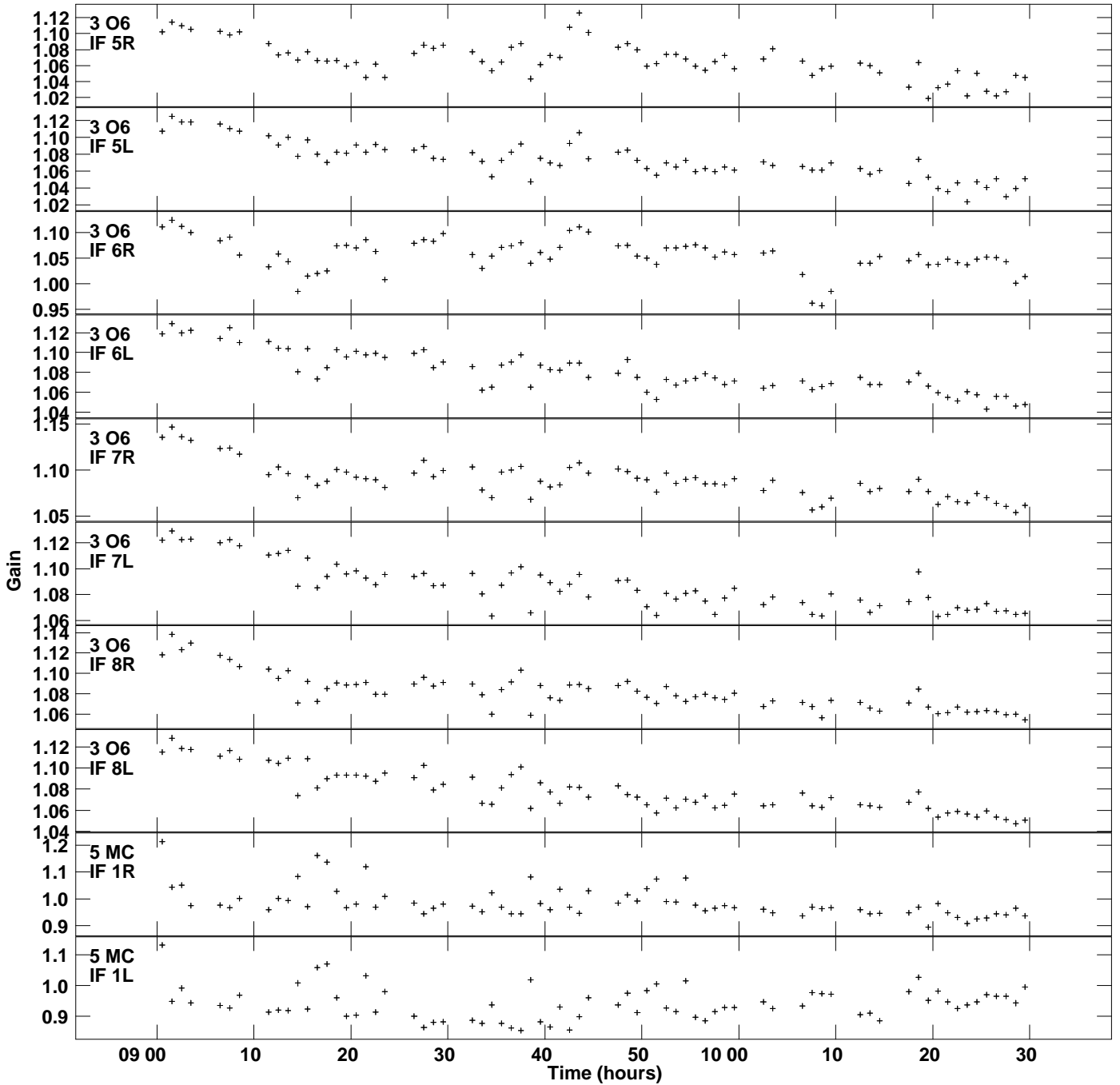
Plot file version 5 created 03-FEB-2016 18:05:07 Gain amp vs UTC time for J1642+3948.MULTI.1 SN 2 Rpol & Lpol IF 1 - 8
