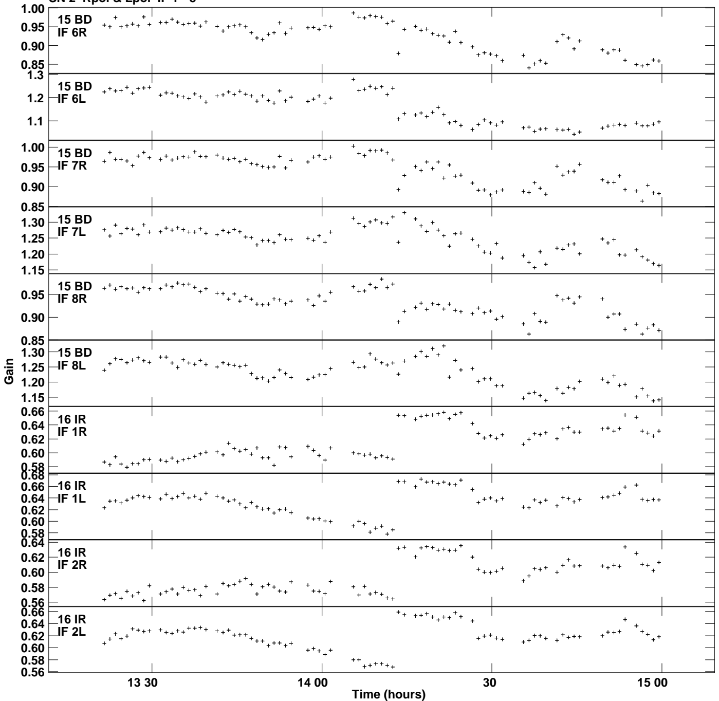
Plot file version 21 created 16-AUG-2016 15:52:30 Gain amp vs UTC time for J0418+3801.MULTI.1 SN 2 Rpol & Lpol IF 1 - 8
