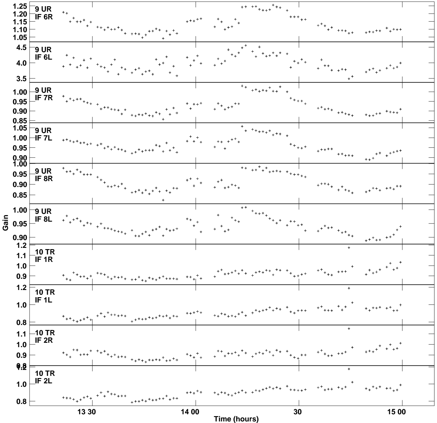
Plot file version 13 created 16-AUG-2016 15:52:30 Gain amp vs UTC time for J0418+3801.MULTI.1 SN 2 Rpol & Lpol IF 1 - 8
