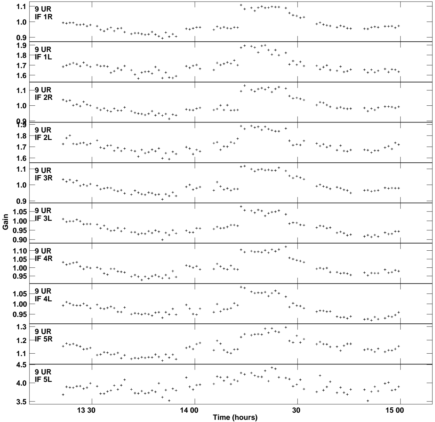
Plot file version 12 created 16-AUG-2016 15:52:30 Gain amp vs UTC time for J0418+3801.MULTI.1 SN 2 Rpol & Lpol IF 1 - 8
