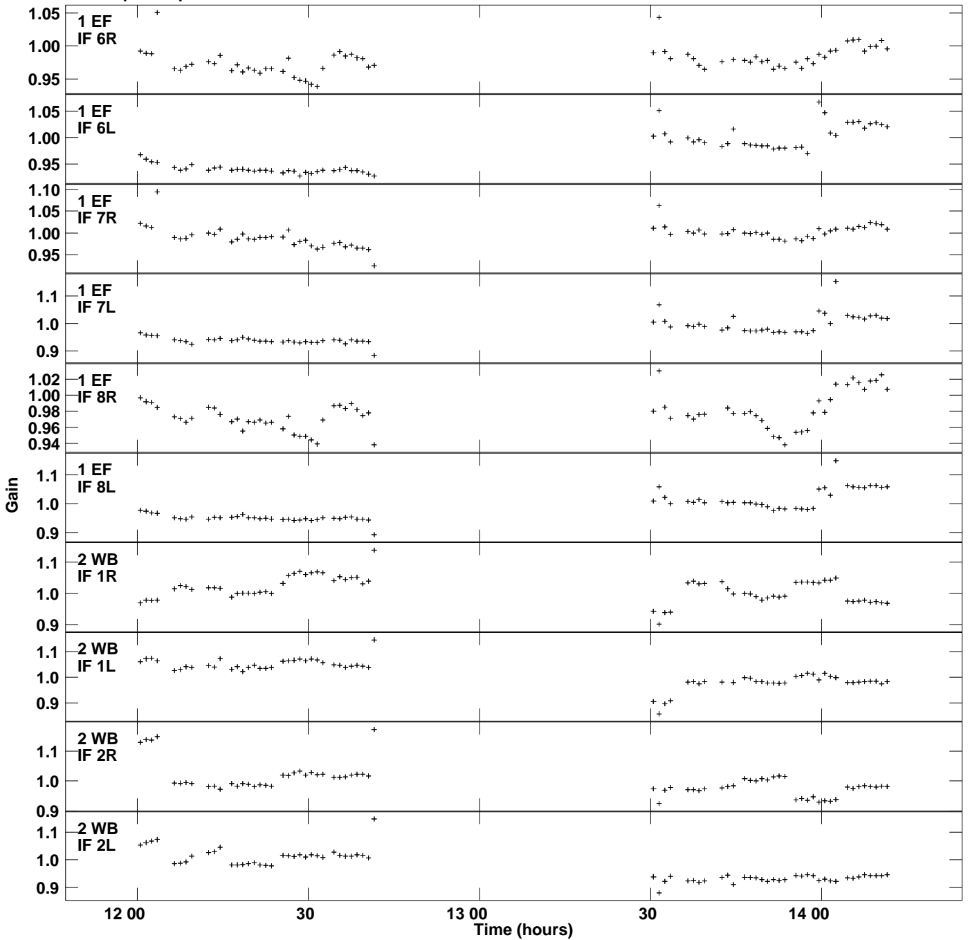
Plot file version 2 created 08-AUG-2016 10:16:48 Gain amp vs UTC time for 0234+285.MULTI.1 SN 2 Rpol & Lpol IF 1 - 8
