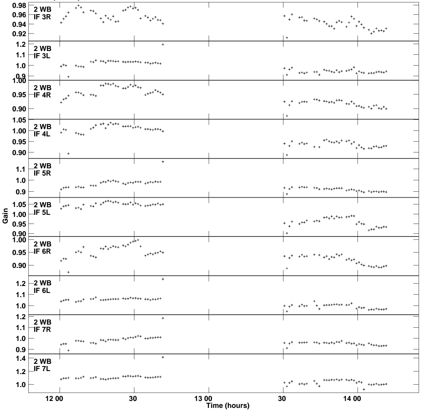
Plot file version 3 created 08-AUG-2016 10:16:48 Gain amp vs UTC time for 0234+285.MULTI.1 SN 2 Rpol & Lpol IF 1 - 8
