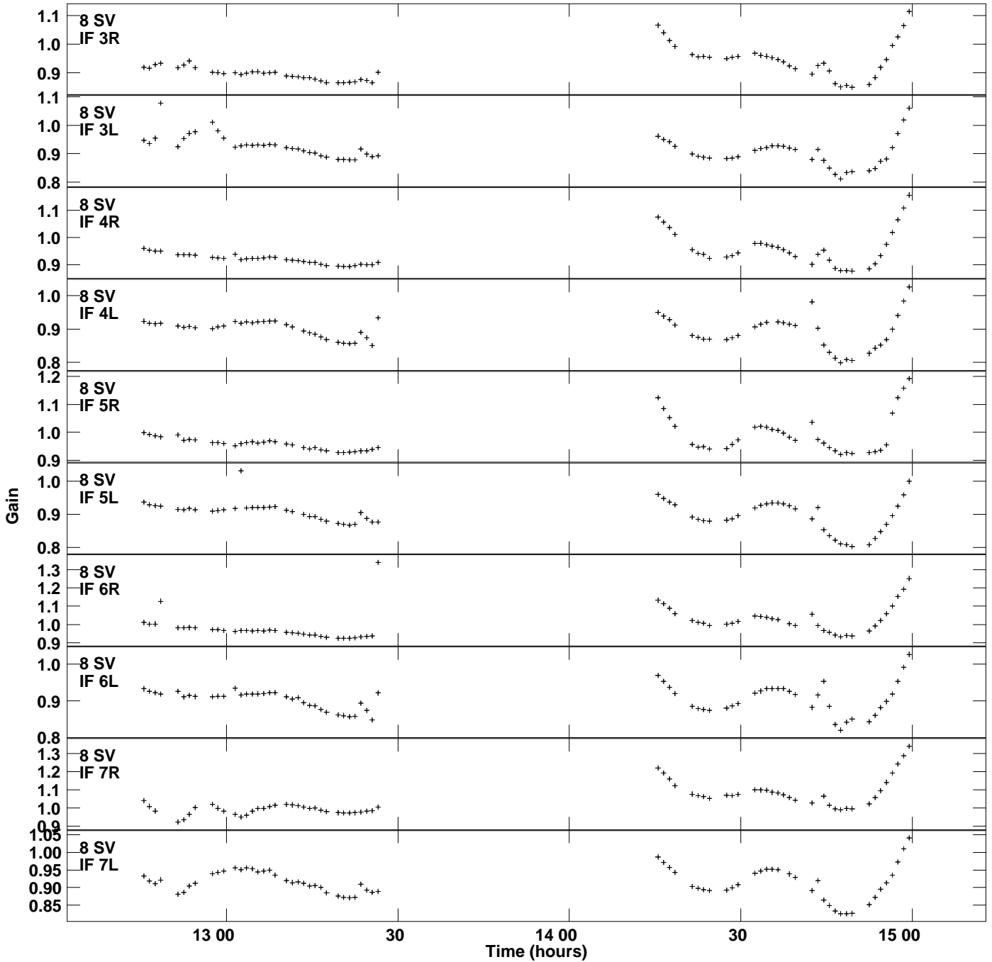
Plot file version 11 created 08-AUG-2016 10:17:14 Gain amp vs UTC time for 3C84.MULTI.1 SN 2 Rpol & Lpol IF 1 - 8
