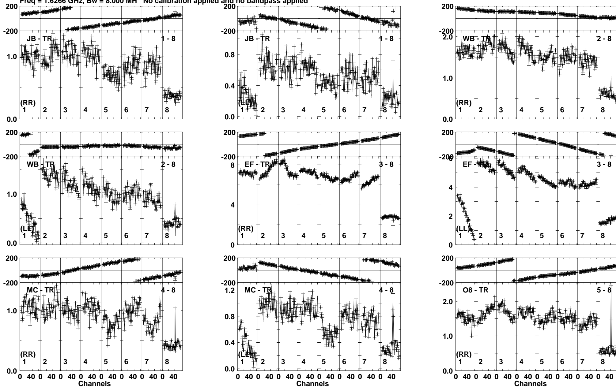
Lower frame: Milli Ampl Jy Top frame: Phas deg Vector averaged cross-power spectrum Baseline: JB (01) - TR (08) Timerange: 00/11:00:01 to 00/11:04:59
