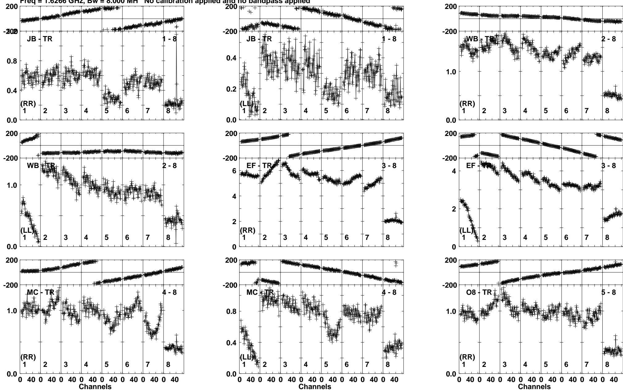
Lower frame: Milli Ampl Jy Top frame: Phas deg Vector averaged cross-power spectrum Baseline: JB (01) - TR (08) Timerange: 00/11:36:01 to 00/11:44:59
