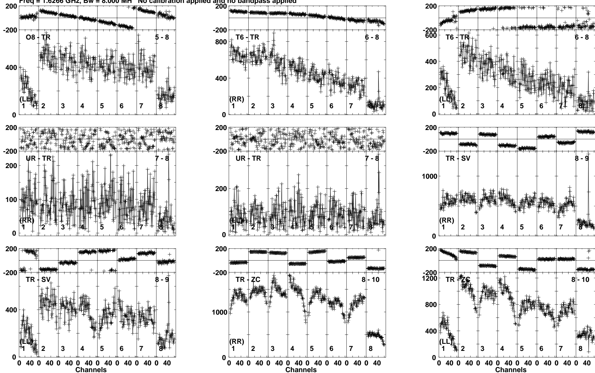
Lower frame: Micro Ampl Jy Top frame: Phas deg Vector averaged cross-power spectrum Baseline: O8 (05) - TR (08) Timerange: 00/11:15:01 to 00/11:24:59
