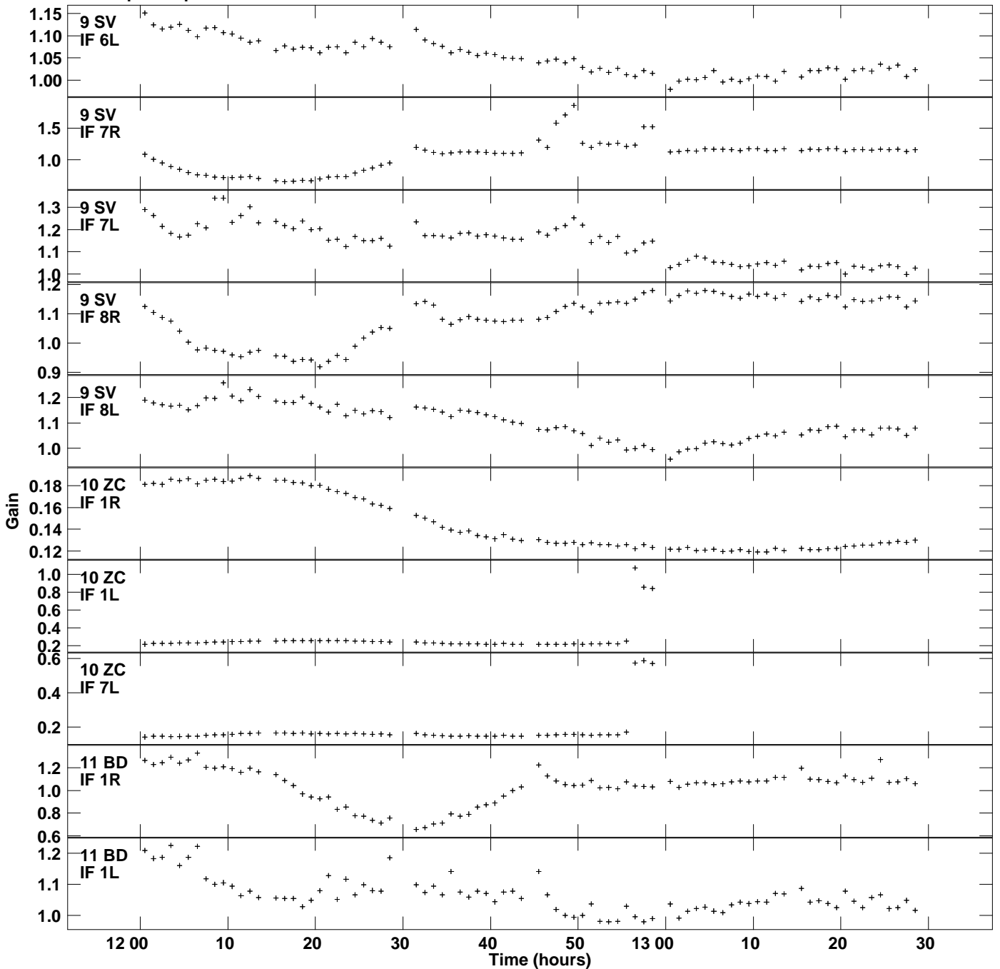
Plot file version 13 created 13-MAR-2018 11:23:40 Gain amp vs UTC time for J0854+2006.MULTI.1 SN 2 Rpol & Lpol IF 1 - 8
