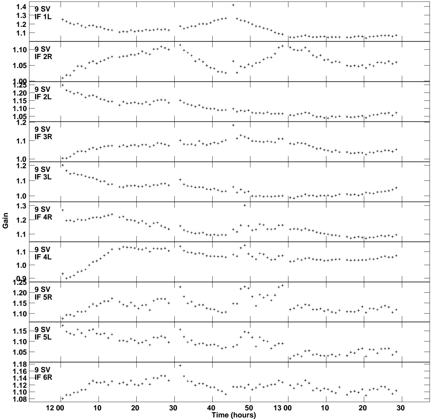
Plot file version 12 created 13-MAR-2018 11:23:40 Gain amp vs UTC time for J0854+2006.MULTI.1 SN 2 Rpol & Lpol IF 1 - 8
