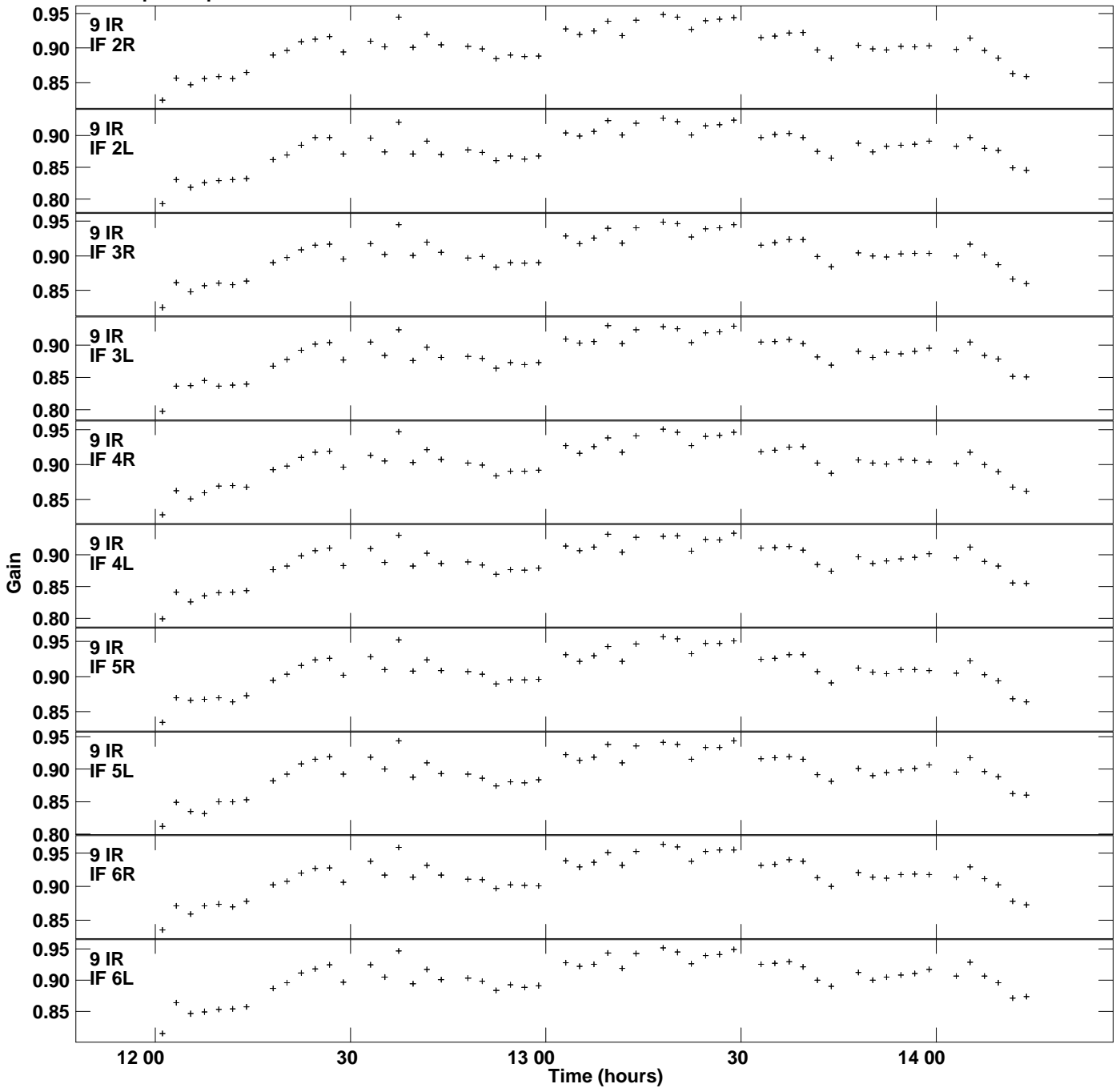
Plot file version 14 created 10-JAN-2018 12:57:34 Gain amp vs UTC time for J0319+4130.MULTI.1 SN 2 Rpol & Lpol IF 1 - 8
