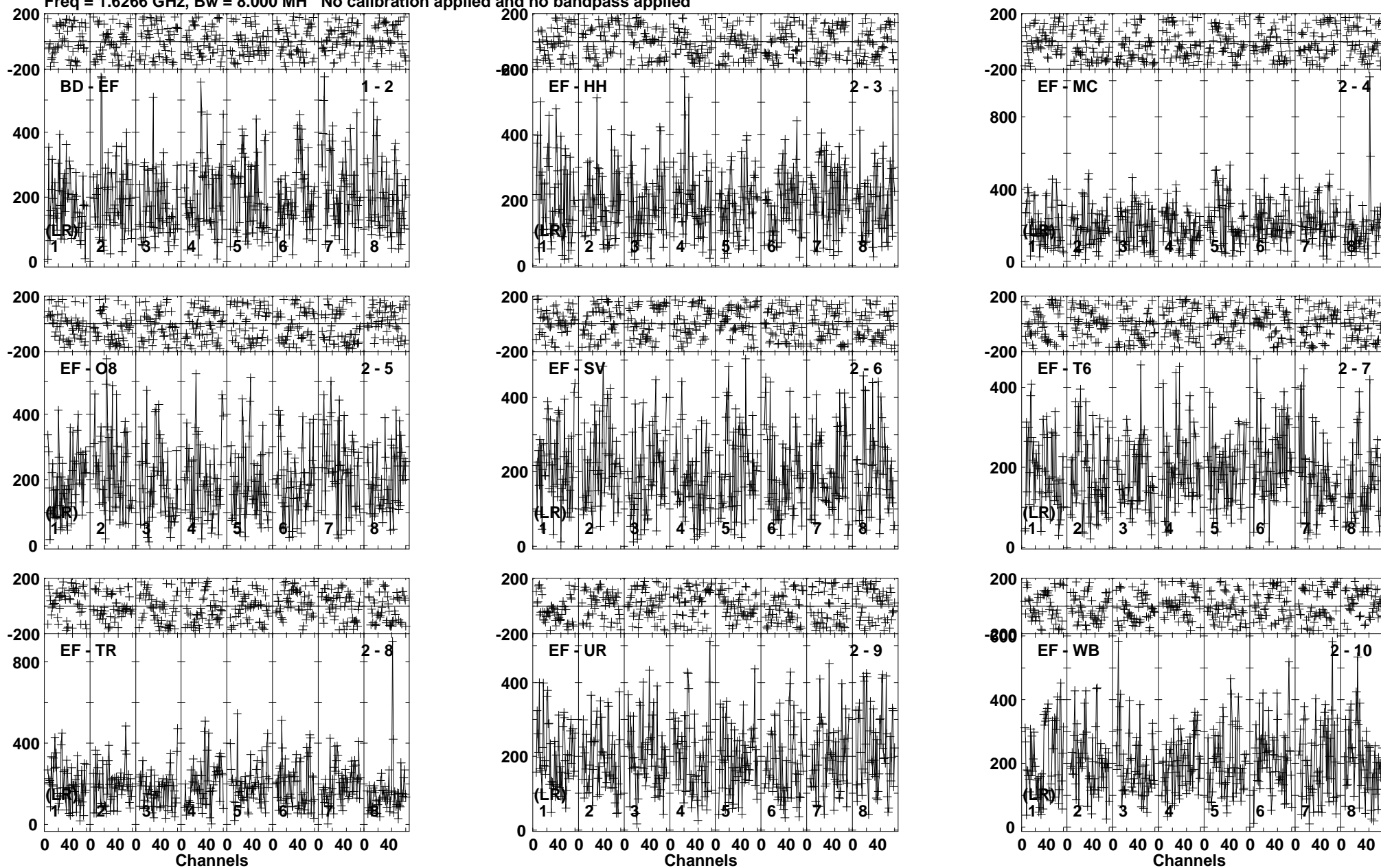
Lower frame: Micro Ampl Jy Top frame: Phas deg Vector averaged cross-power spectrum Baseline: BD (01) - EF (02) Timerange: 00/16:52:33 to 00/16:54:59
