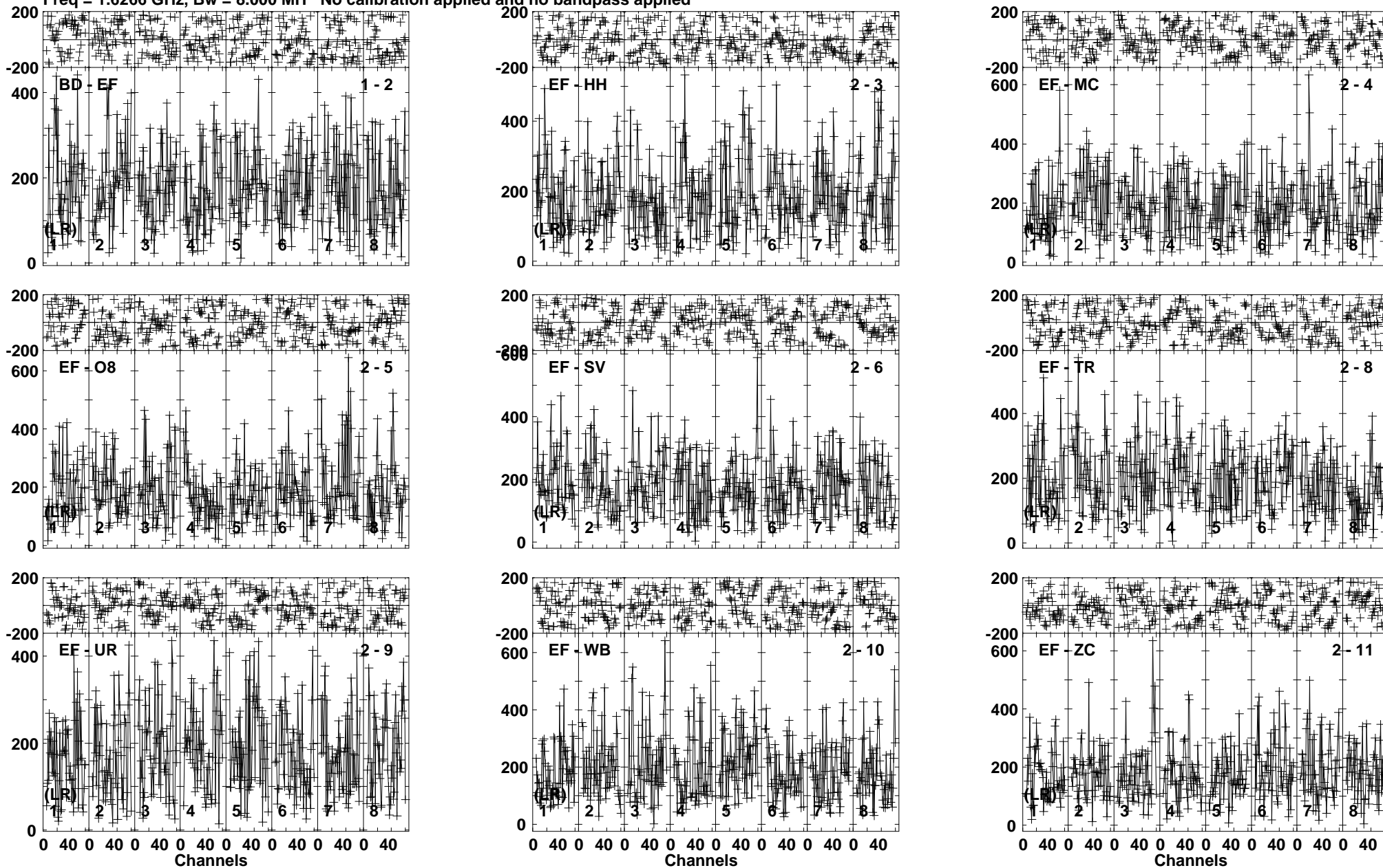
Lower frame: Micro Ampl Jy Top frame: Phas deg Vector averaged cross-power spectrum Baseline: BD (01) - EF (02) Timerange: 00/18:26:03 to 00/18:28:29
