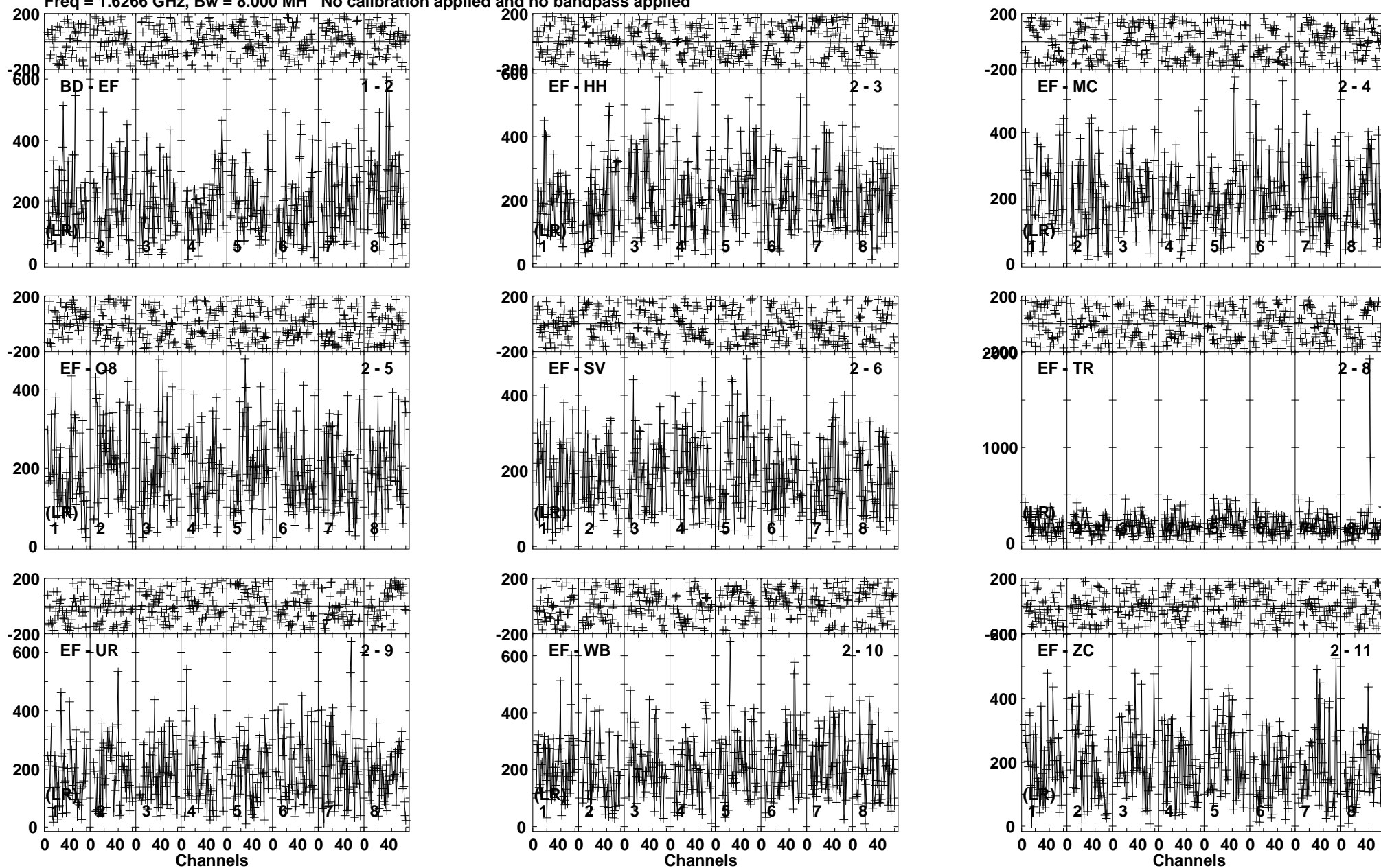
Lower frame: Micro Ampl Jy Top frame: Phas deg Vector averaged cross-power spectrum Baseline: BD (01) - EF (02) Timerange: 00/17:21:05 to 00/17:23:29
