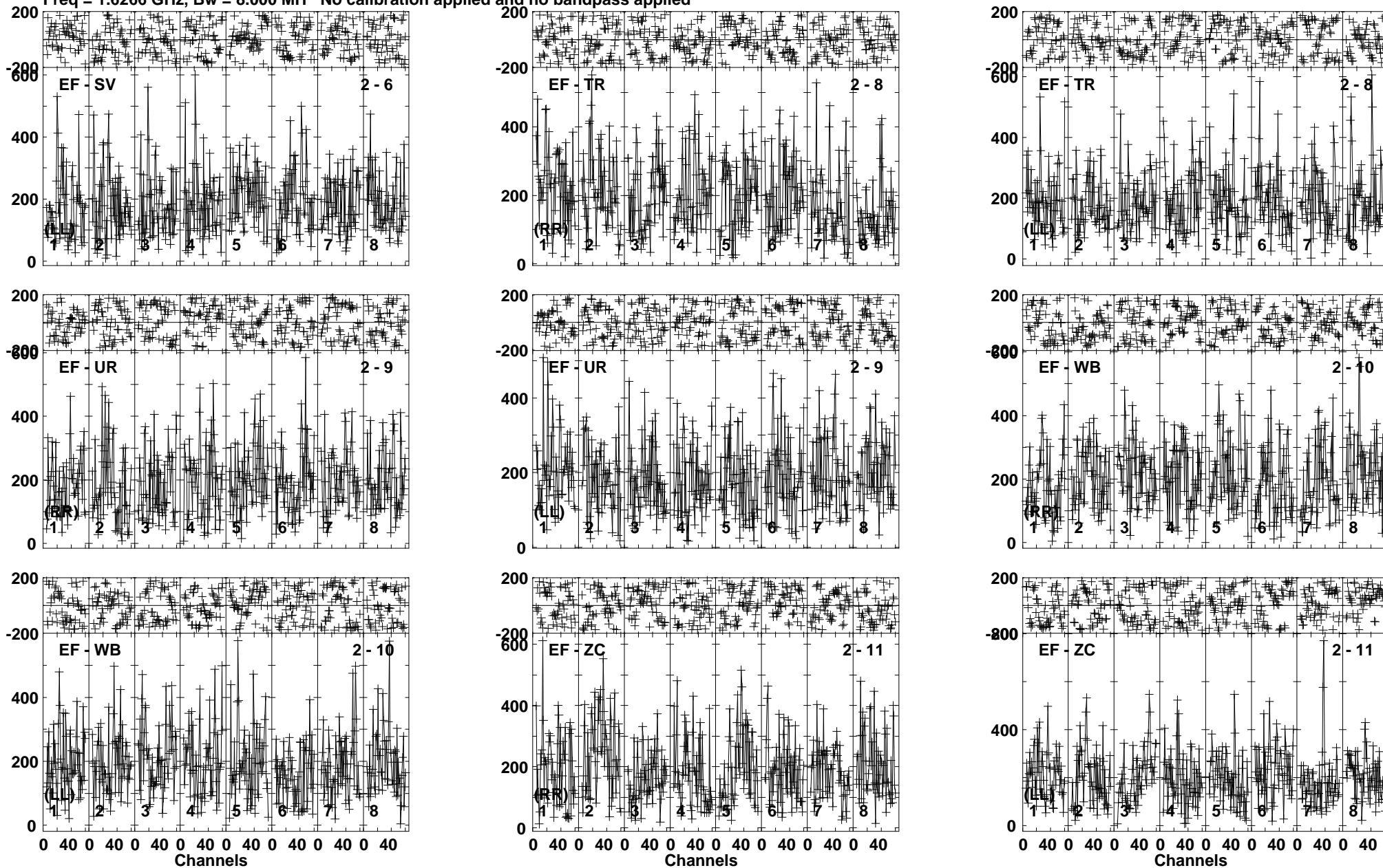
Lower frame: Micro Ampl Jy Top frame: Phas deg Vector averaged cross-power spectrum Baseline: EF (02) - SV (06) Timerange: 00/18:38:03 to 00/18:40:29
