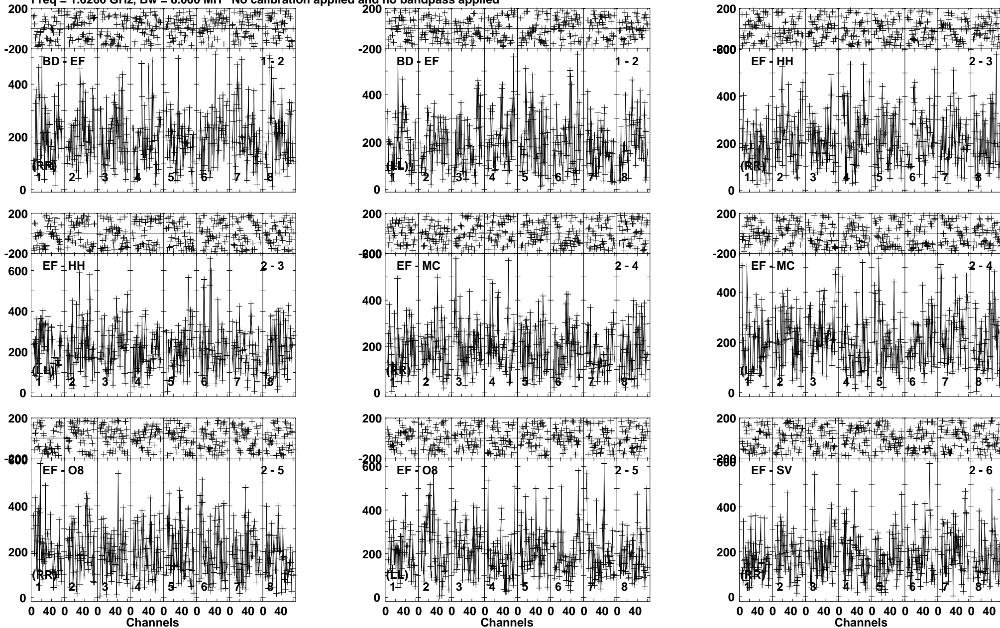
Lower frame: Micro Ampl Jy Top frame: Phas deg Vector averaged cross-power spectrum Baseline: BD (01) - EF (02) Timerange: 00/16:23:33 to 00/16:25:59
