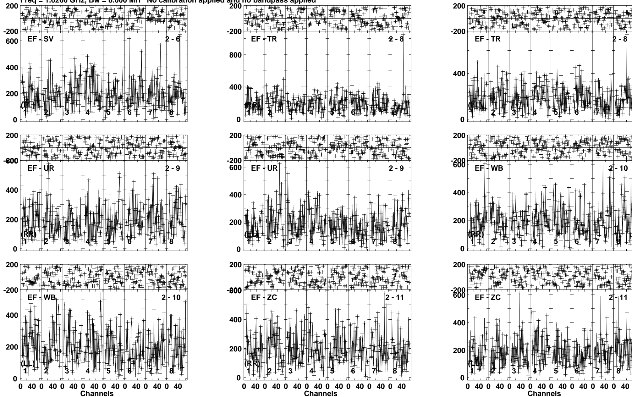
Lower frame: Micro Ampl Jy Top frame: Phas deg Vector averaged cross-power spectrum Baseline: EF (02) - SV (06) Timerange: 00/18:23:33 to 00/18:25:59
