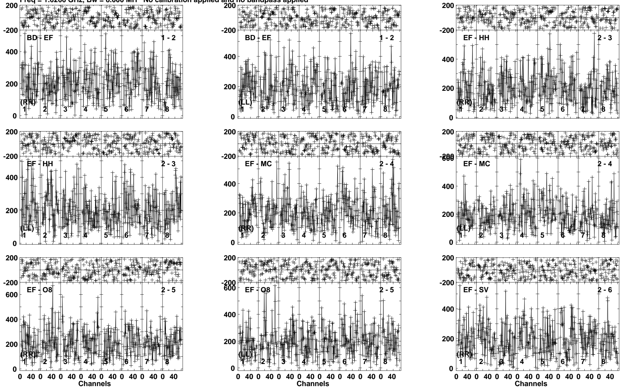
Lower frame: Micro Ampl Jy Top frame: Phas deg Vector averaged cross-power spectrum Baseline: BD (01) - EF (02) Timerange: 00/16:09:05 to 00/16:11:29
