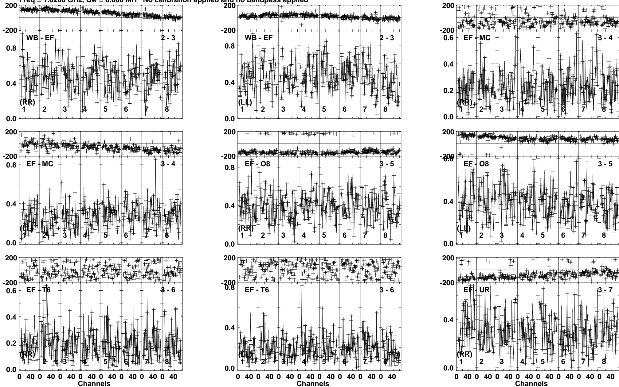
Lower frame: Milli Ampl Jy Top frame: Phas deg Vector averaged cross-power spectrum Baseline: WB (02) - EF (03) Timerange: 00/14:26:21 to 00/14:28:40
