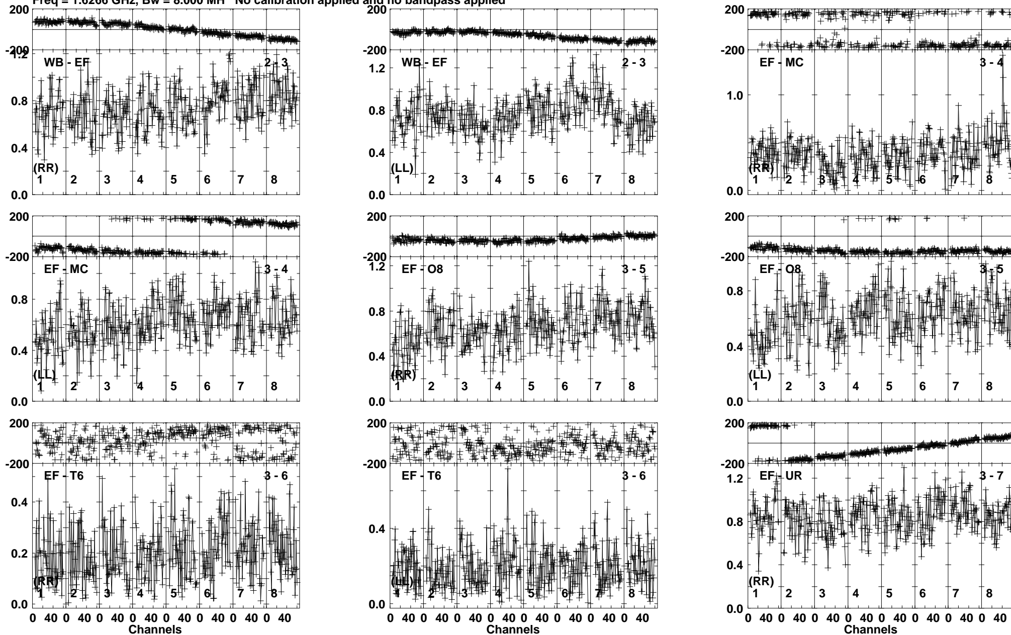
Lower frame: Milli Ampl Jy Top frame: Phas deg Vector averaged cross-power spectrum Baseline: WB (02) - EF (03) Timerange: 00/15:59:20 to 00/16:01:40
