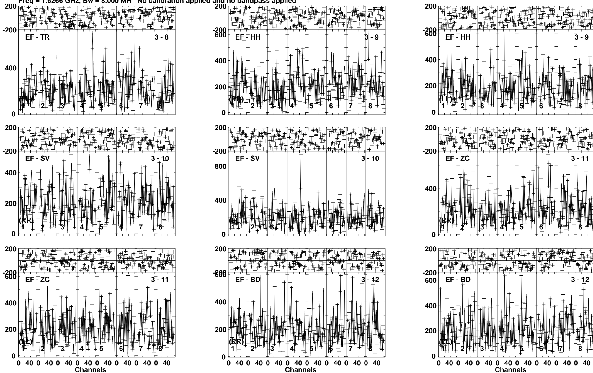
Lower frame: Micro Ampl Jy Top frame: Phas deg Vector averaged cross-power spectrum Baseline: EF (03) - TR (08) Timerange: 00/17:23:01 to 00/17:25:20
