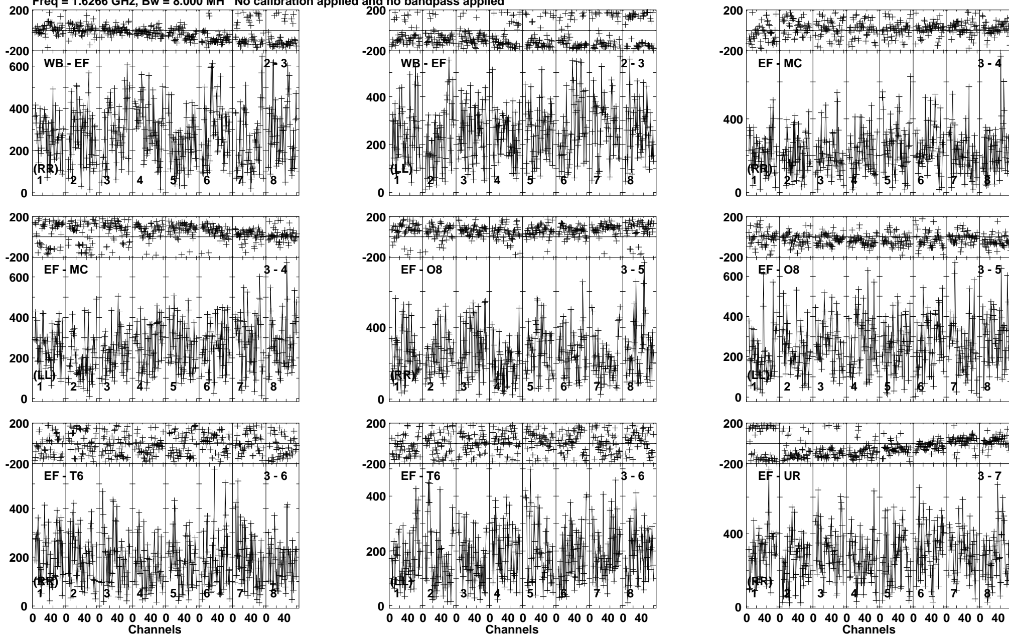
Lower frame: Micro Ampl Jy Top frame: Phas deg Vector averaged cross-power spectrum Baseline: WB (02) - EF (03) Timerange: 00/15:34:20 to 00/15:36:40
