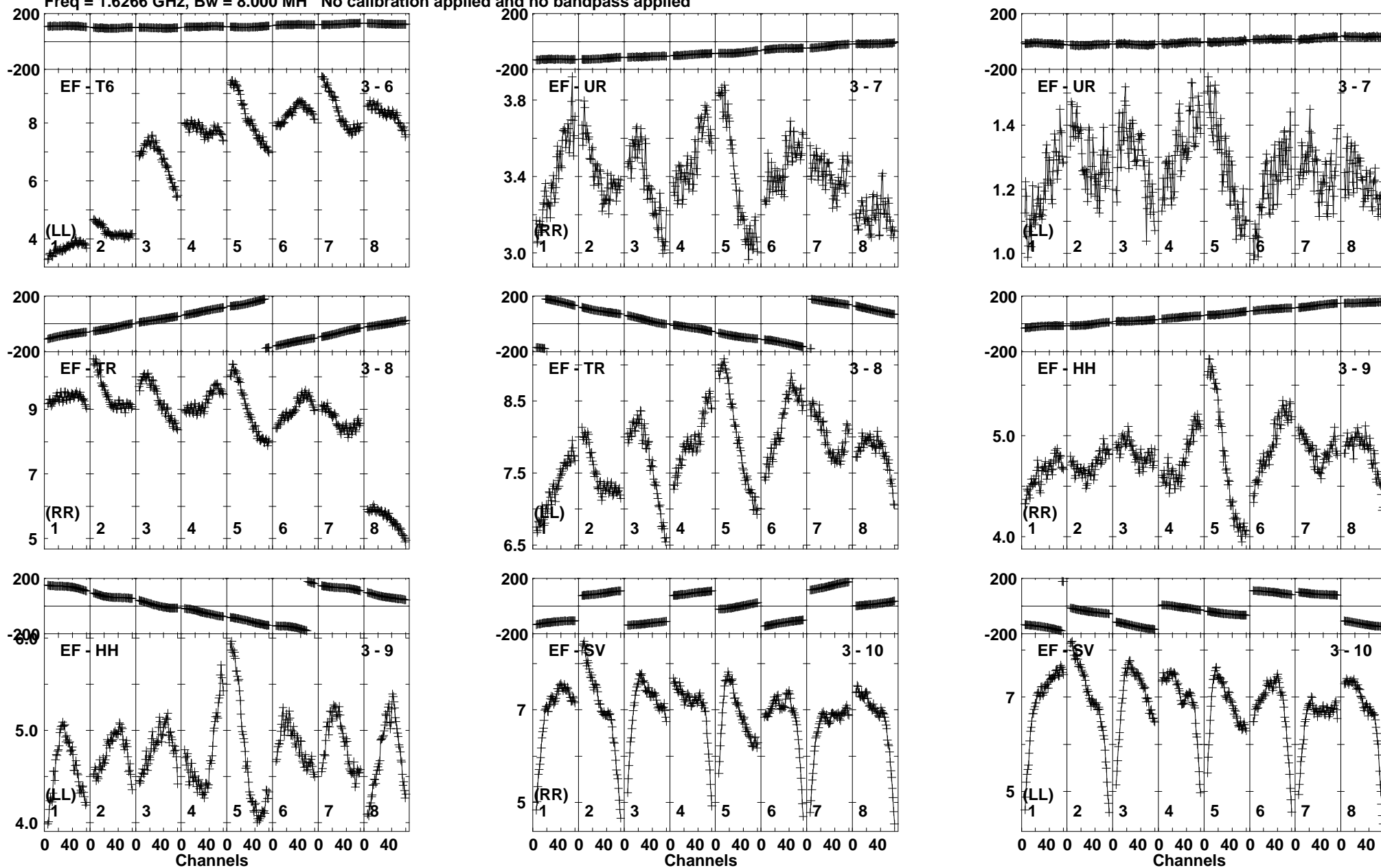
Lower frame: Milli Ampl Jy Top frame: Phas deg Vector averaged cross-power spectrum Baseline: EF (03) - T6 (06) Timerange: 00/13:28:00 to 00/13:39:59
