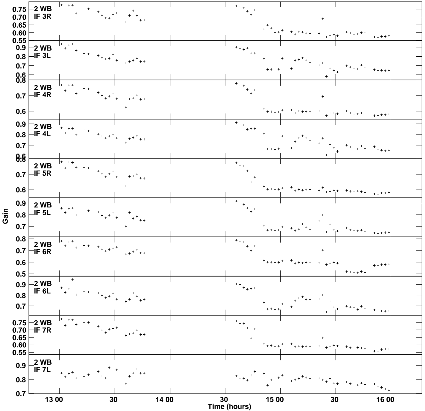
Plot file version 3 created 02-AUG-2018 14:55:03 Gain amp vs UTC time for J0319+4130.MULTI.1 SN 2 Rpol & Lpol IF 1 - 8
