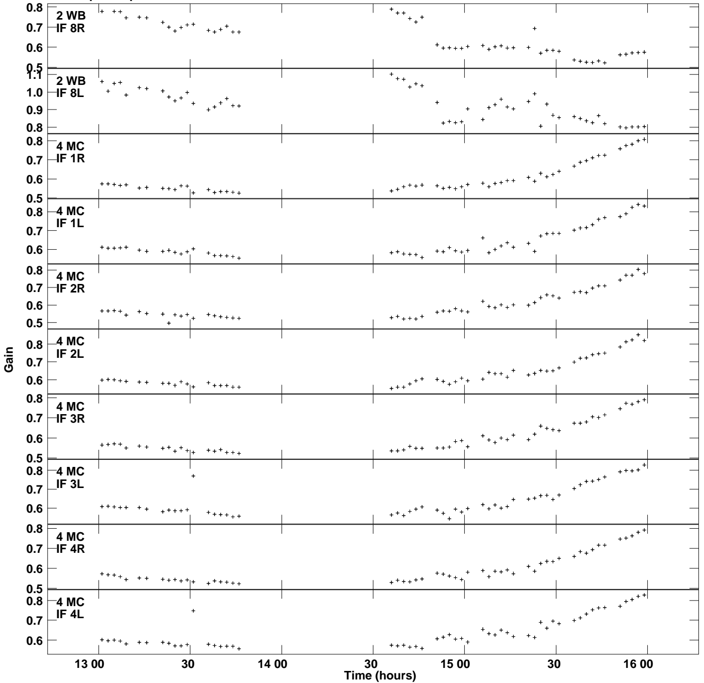
Plot file version 4 created 02-AUG-2018 14:55:03 Gain amp vs UTC time for J0319+4130.MULTI.1 SN 2 Rpol & Lpol IF 1 - 8
