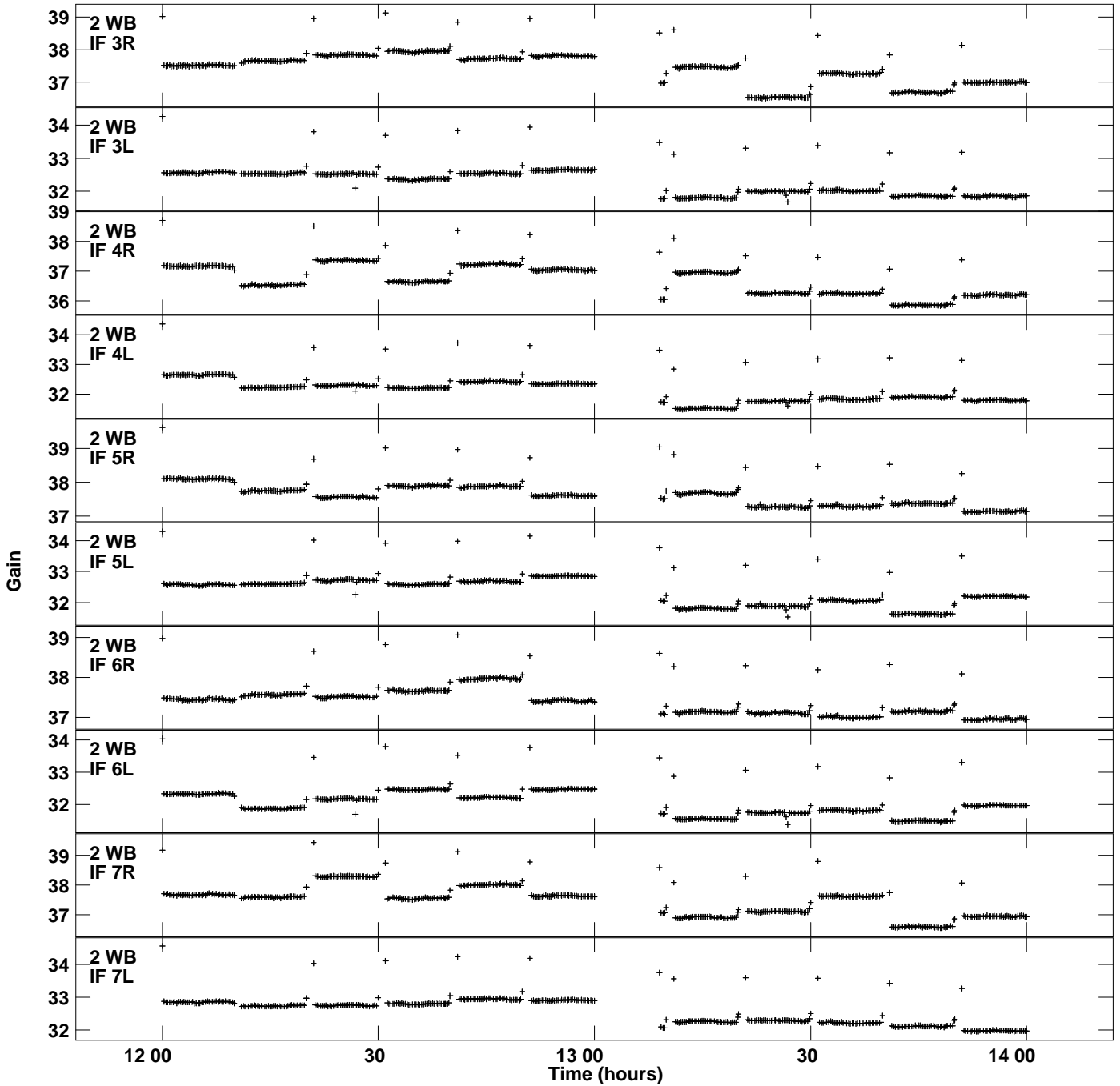
Plot file version 3 created 10-DEC-2019 18:34:00 Gain amp vs UTC time for N19M3_1.UVDATA.1 CL 2 Rpol & Lpol IF 1 - 8
