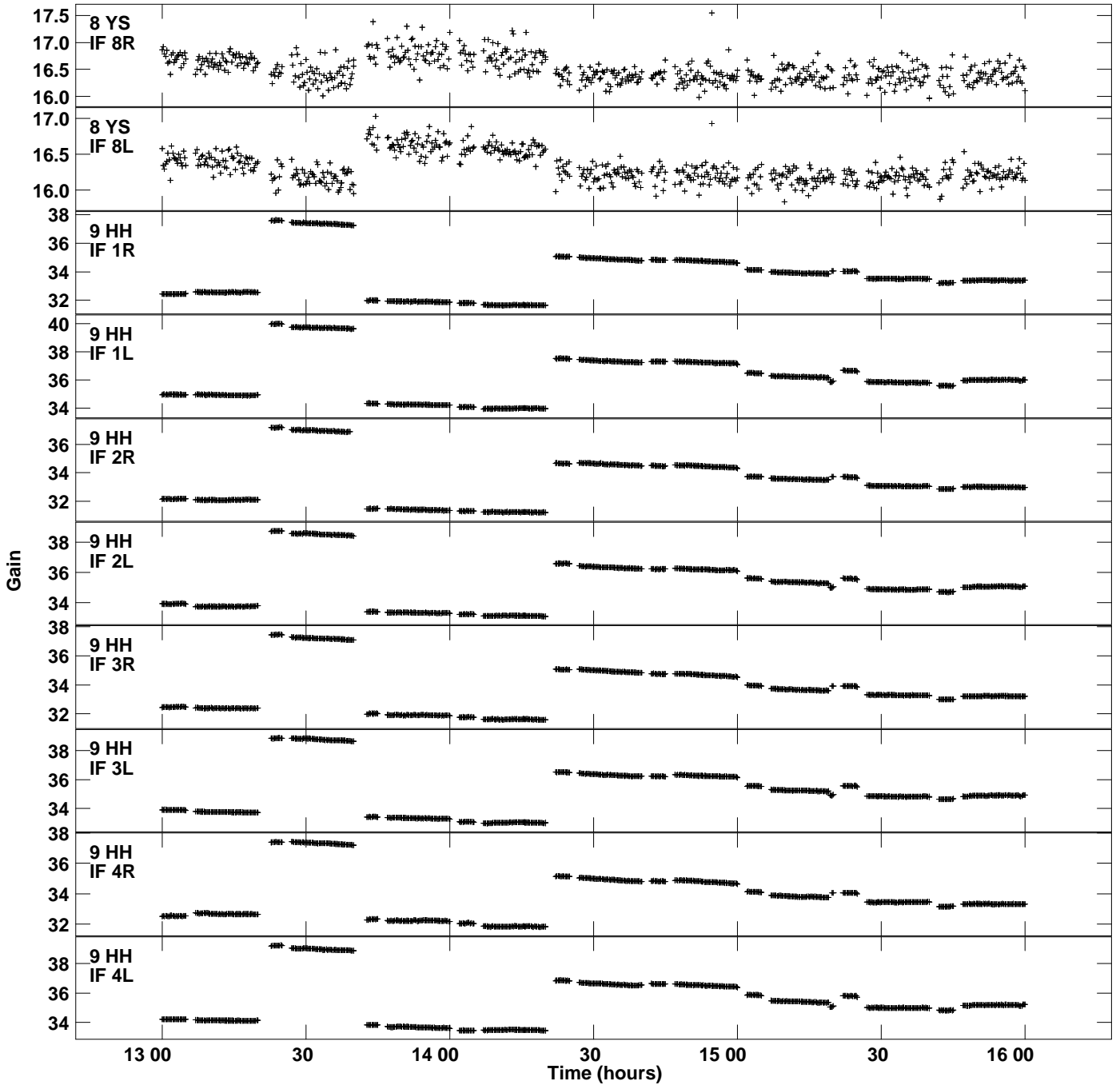
Plot file version 12 created 16-AUG-2019 17:27:31 Gain amp vs UTC time for N19X1.UVDATA.1 CL 2 Rpol & Lpol IF 1 - 8
