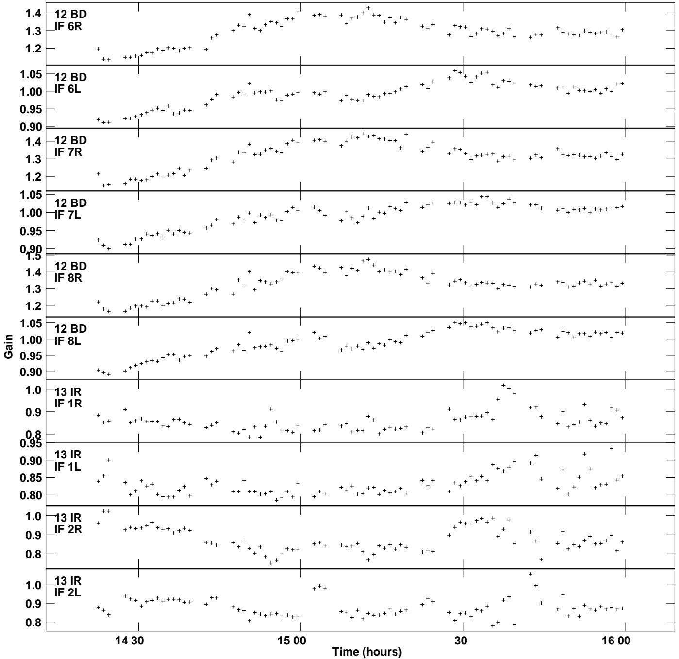
Plot file version 18 created 16-AUG-2019 17:49:37 Gain amp vs UTC time for J1159+2914.MULTI.1 SN 2 Rpol & Lpol IF 1 - 8
