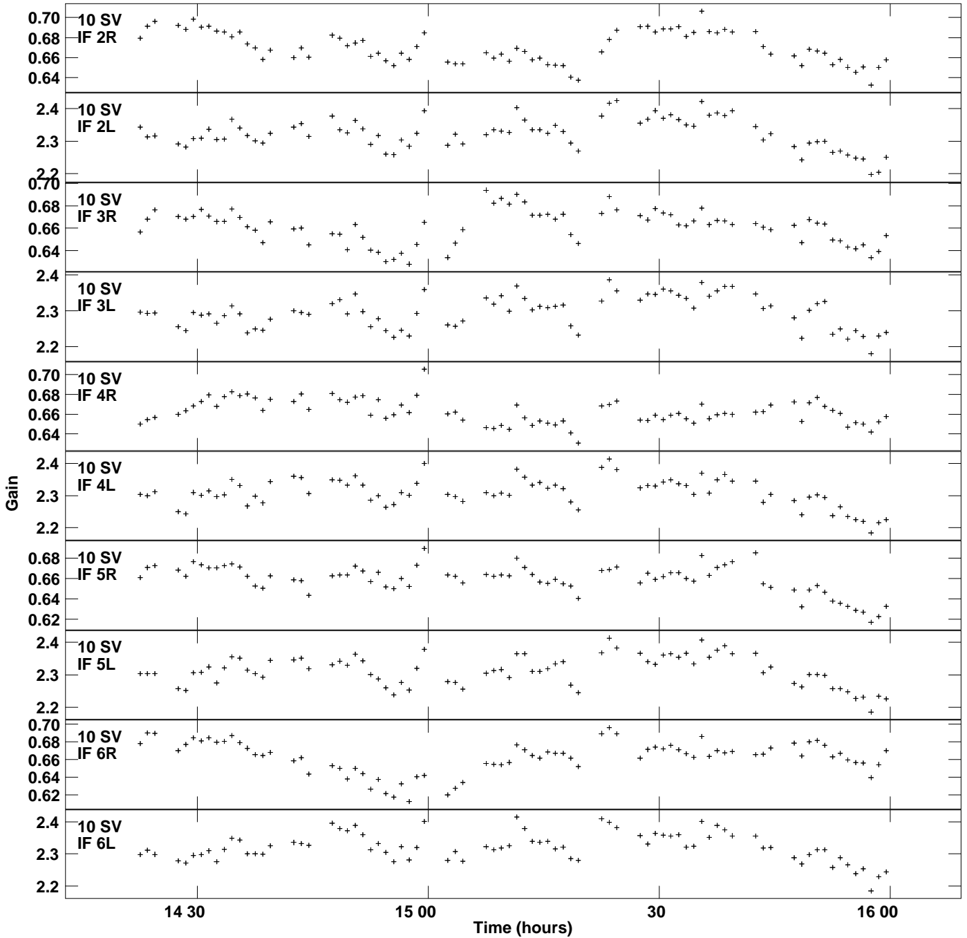
Plot file version 14 created 16-AUG-2019 17:49:37 Gain amp vs UTC time for J1159+2914.MULTI.1 SN 2 Rpol & Lpol IF 1 - 8
