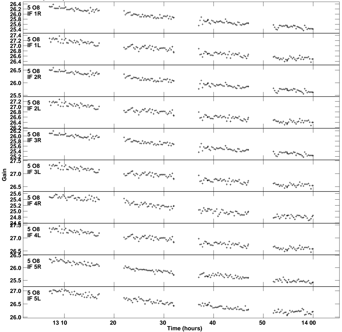
Plot file version 5 created 02-DEC-2020 10:45:47 Gain amp vs UTC time for N20C3_2.TMP.1 CL 4 Rpol & Lpol IF 1 - 16
