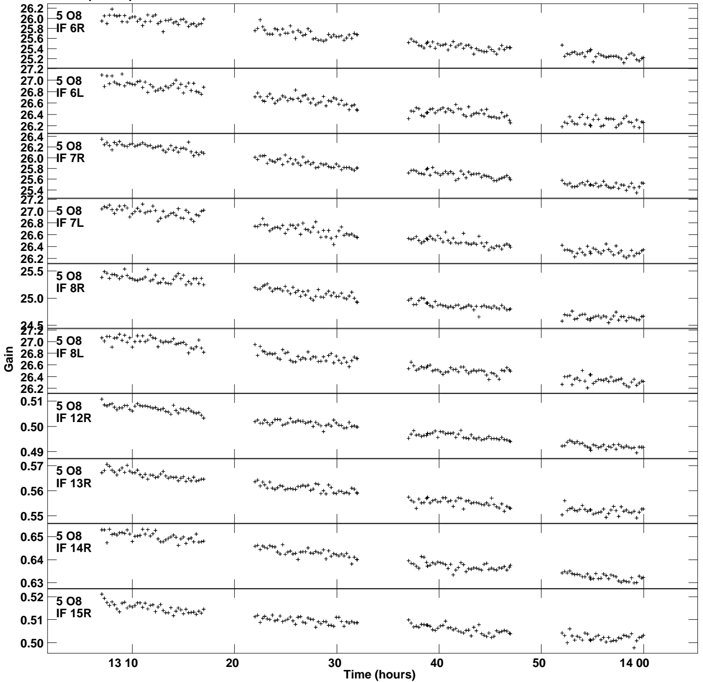
Plot file version 6 created 02-DEC-2020 10:45:47 Gain amp vs UTC time for N20C3_2.TMP.1 CL 4 Rpol & Lpol IF 1 - 16
