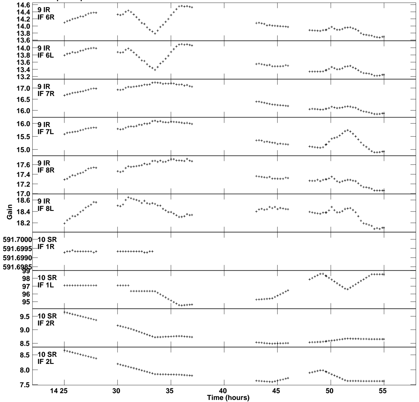
Plot file version 10 created 06-APR-2020 12:49:47 Gain amp vs UTC time for N20M1_2.TMP.1 CL 4 Rpol & Lpol IF 1 - 8
