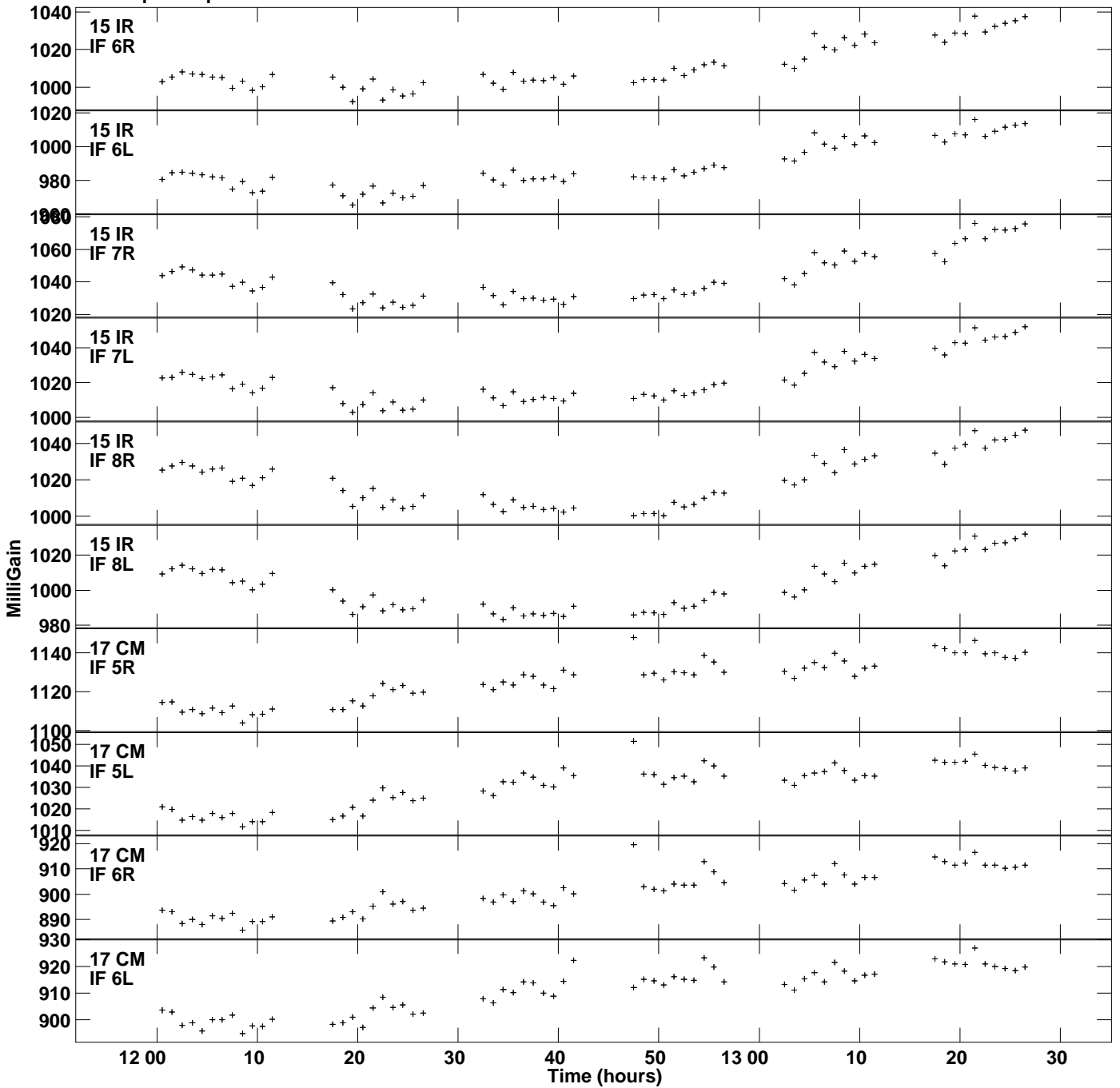
Plot file version 22 created 02-AUG-2021 22:41:25 Gain amp vs UTC time for J0854+2006.MULTI.1 SN 2 Rpol & Lpol IF 1 - 8
