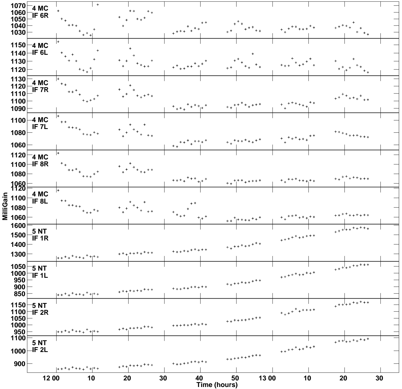
Plot file version 6 created 02-AUG-2021 22:41:25 Gain amp vs UTC time for J0854+2006.MULTI.1 SN 2 Rpol & Lpol IF 1 - 8
