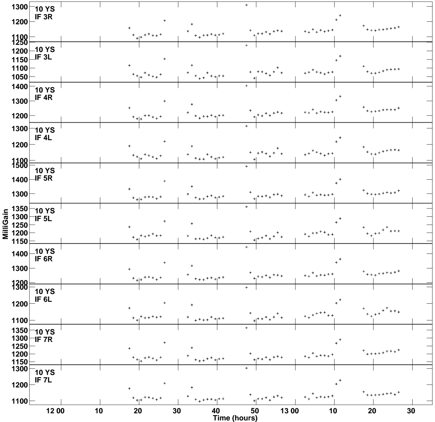
Plot file version 15 created 02-AUG-2021 22:41:25 Gain amp vs UTC time for J0854+2006.MULTI.1 SN 2 Rpol & Lpol IF 1 - 8
