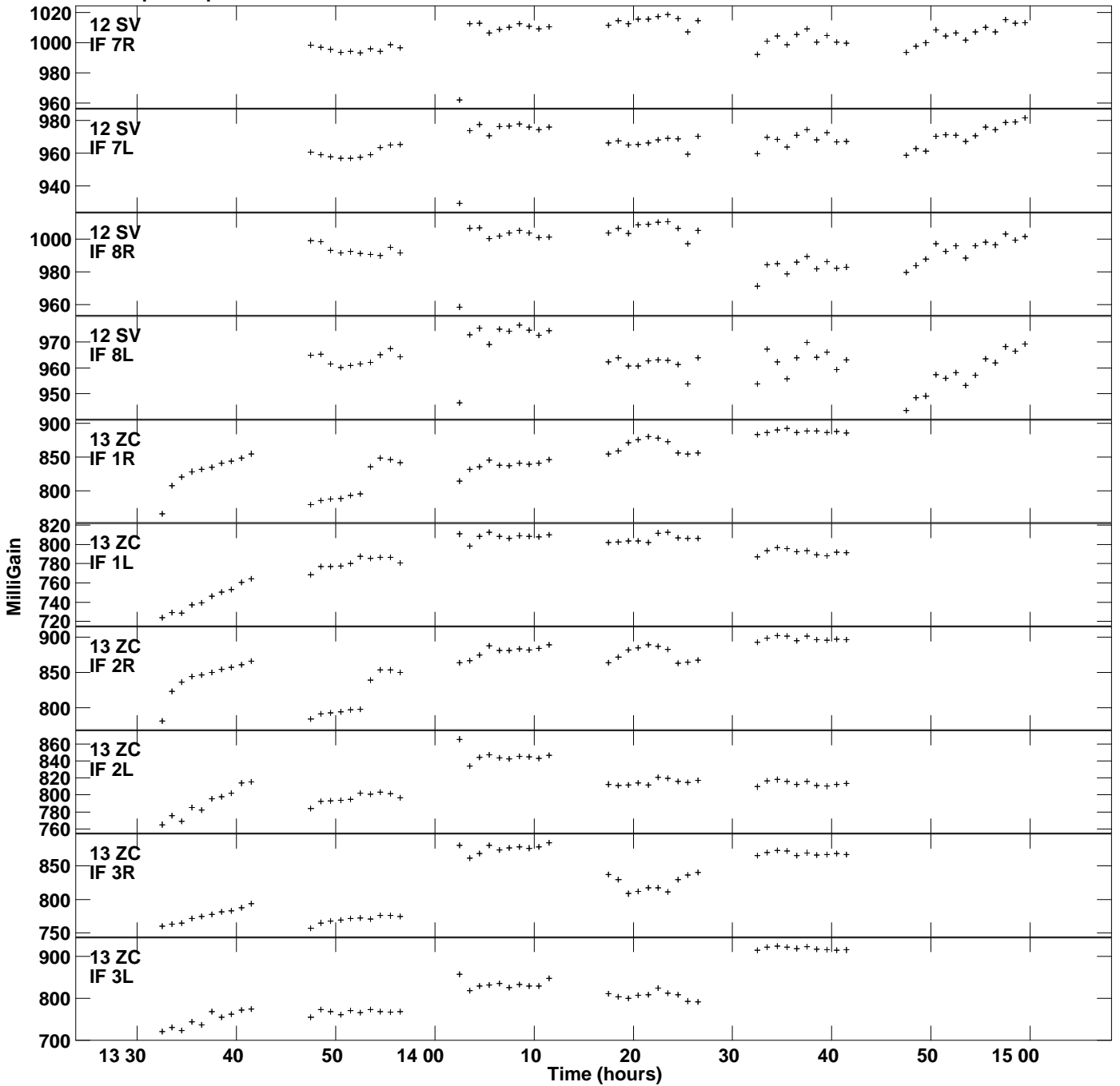
Plot file version 19 created 02-AUG-2021 22:40:31 Gain amp vs UTC time for J1058+0133.MULTI.1 SN 2 Rpol & Lpol IF 1 - 8
