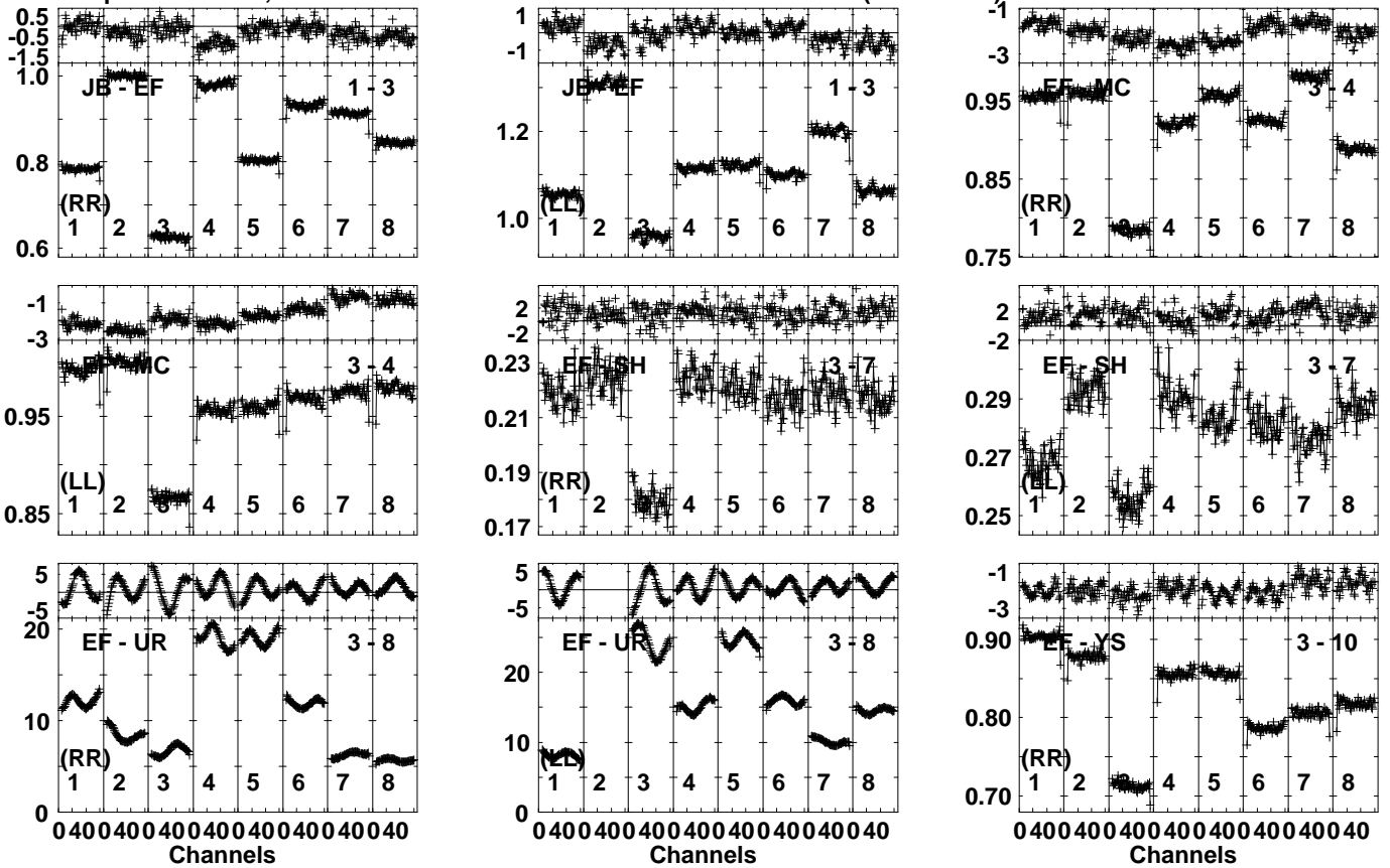
Lower frame: Ampl Jy Top frame: Phas deg Vector averaged cross-power spectrum Several baselines displayed Timerange: 00/13:37:01 to 00/13:46:59
