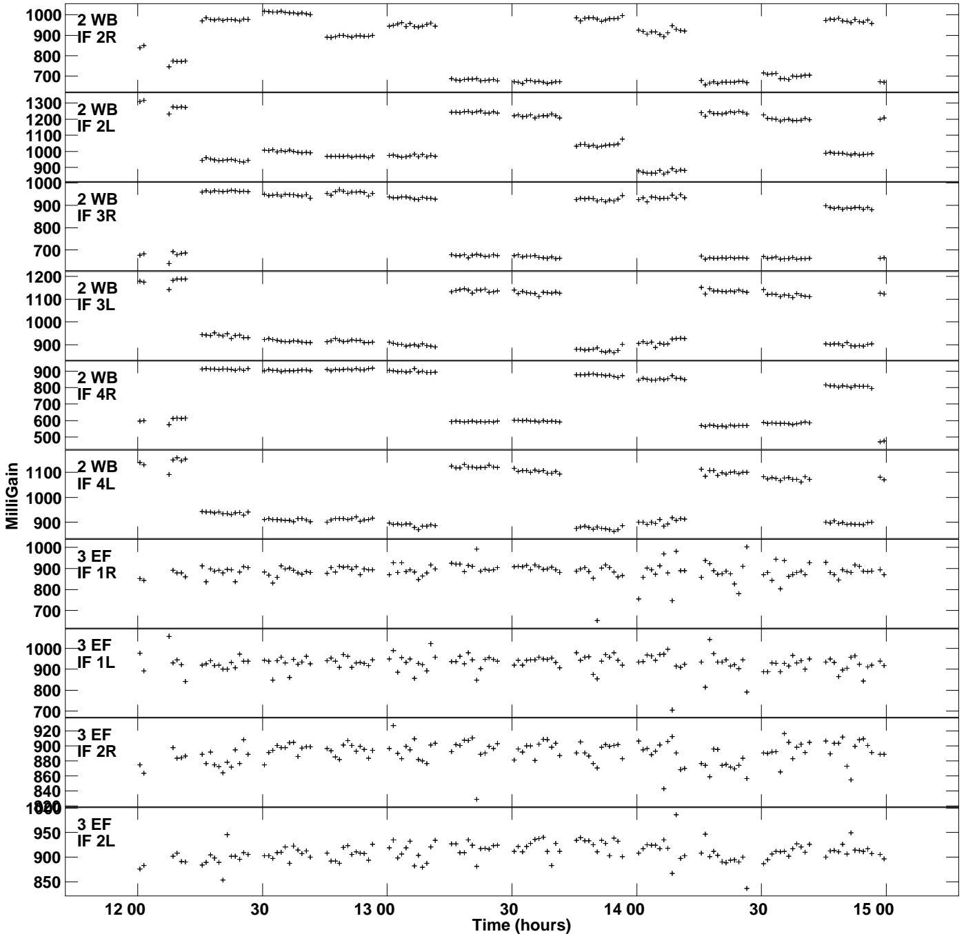
Plot file version 2 created 27-JUL-2021 18:08:31 Gain amp vs UTC time for J0956+2515.MULTI.1 SN 2 Rpol & Lpol IF 1 - 4
