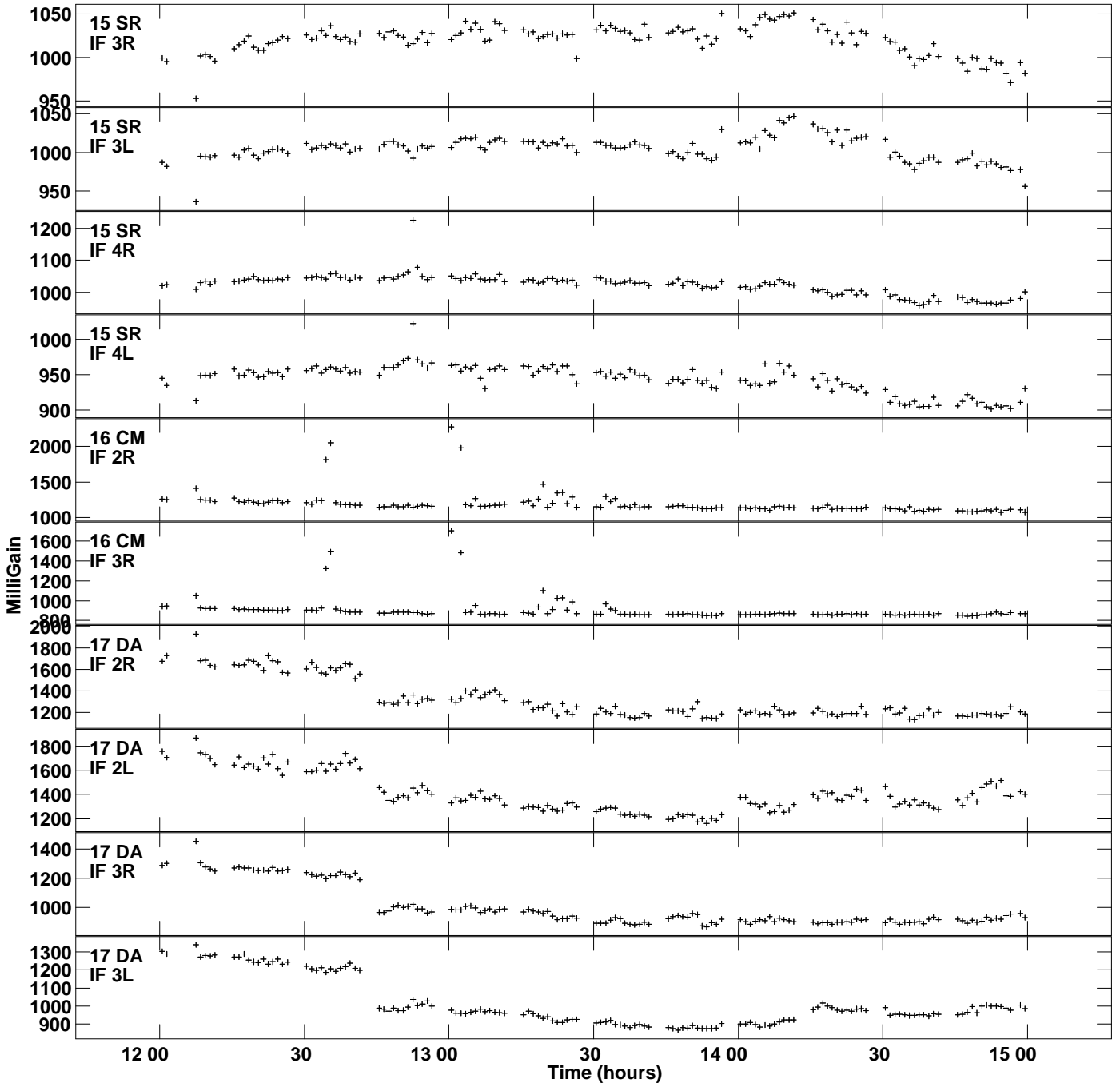
Plot file version 11 created 27-JUL-2021 18:08:31 Gain amp vs UTC time for J0956+2515.MULTI.1 SN 2 Rpol & Lpol IF 1 - 4
