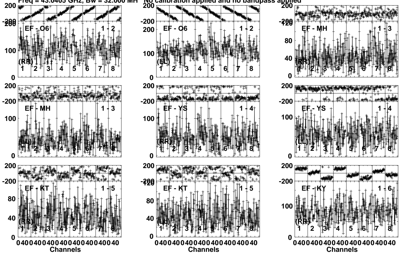
Lower frame: Micro Ampl Jy Top frame: Phas deg Vector averaged cross-power spectrum Several baselines displayed Timerange: 00/12:37:00 to 00/12:50:00
