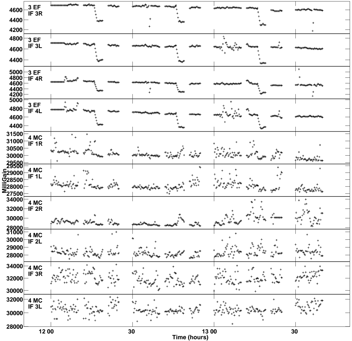
Plot file version 3 created 14-JUN-2023 13:57:11 Gain amp vs UTC time for N22L3_1.UVDATA.1 CL 2 Rpol & Lpol IF 1 - 4
