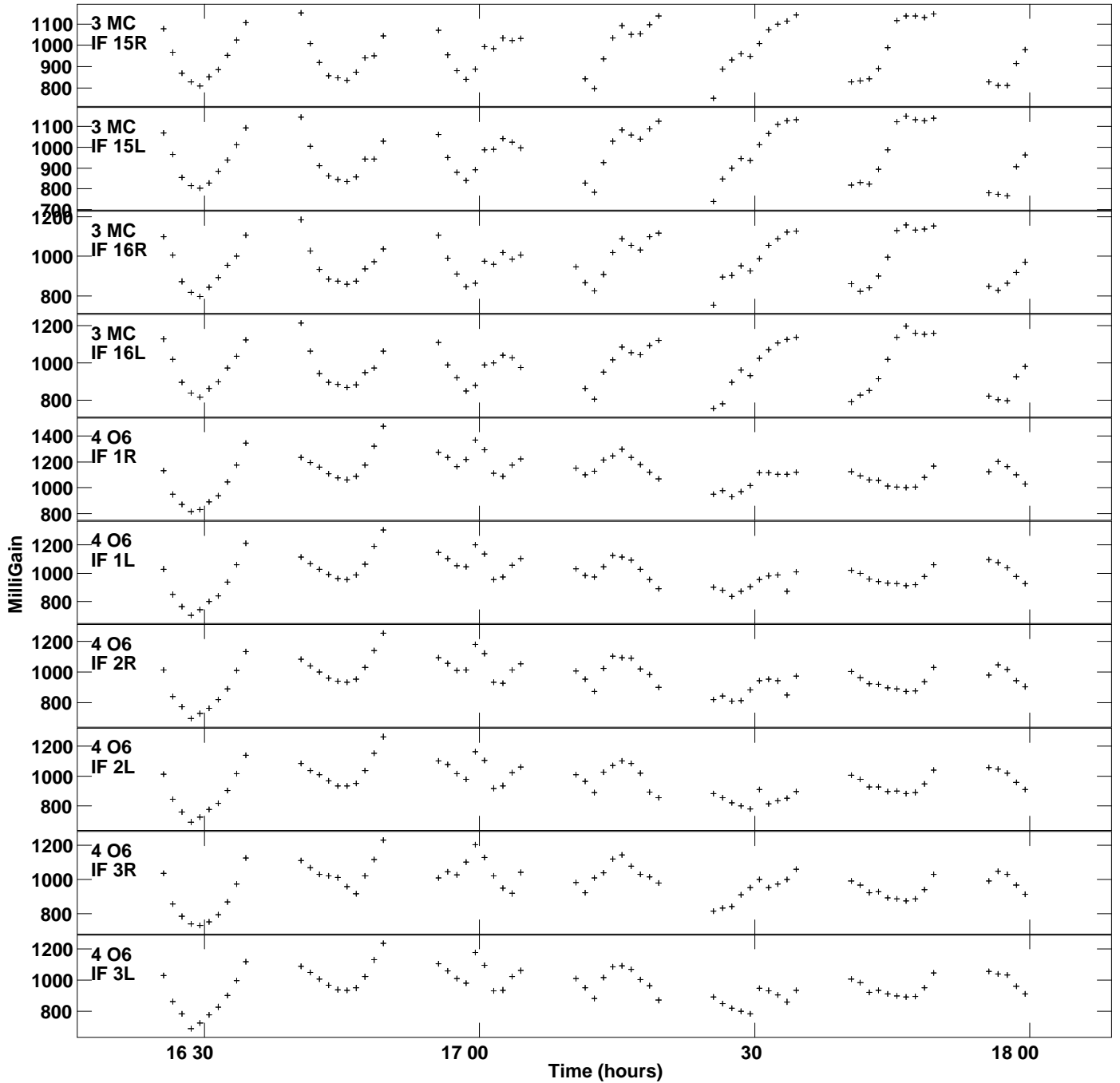
Plot file version 10 created 13-DEC-2023 15:24:05 Gain amp vs UTC time for 0133+476.MULTI.1 SN 2 Rpol & Lpol IF 1 - 16
