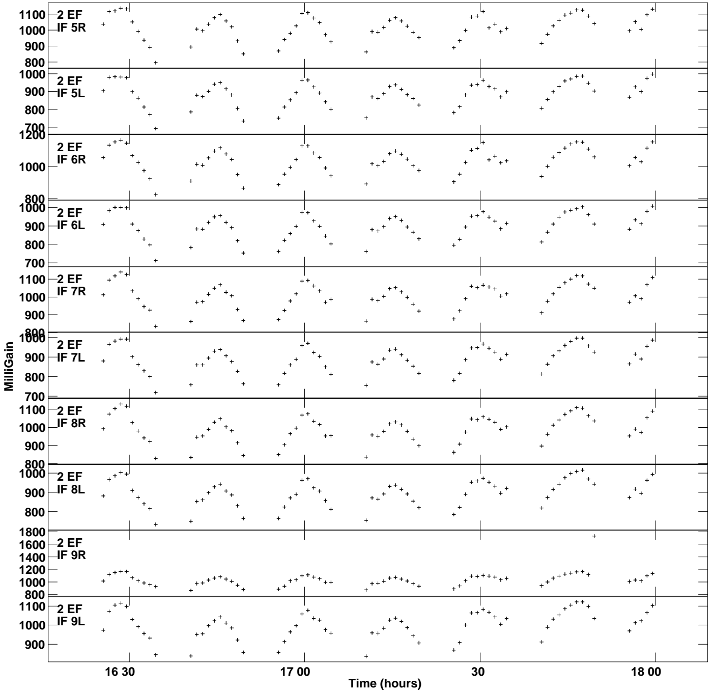
Plot file version 5 created 13-DEC-2023 15:24:05 Gain amp vs UTC time for 0133+476.MULTI.1 SN 2 Rpol & Lpol IF 1 - 16
