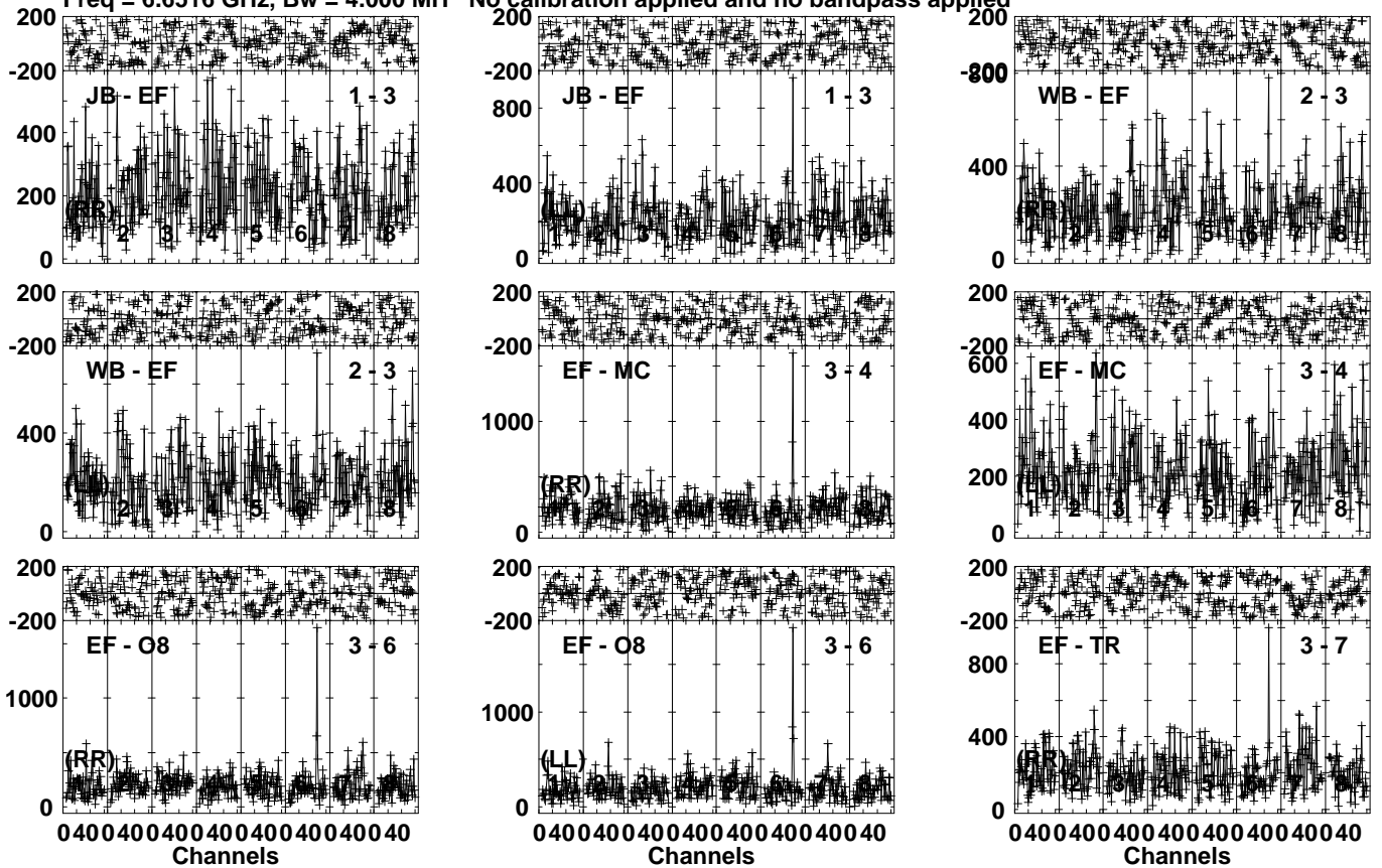
Lower frame: Micro Ampl Jy Top frame: Phas deg Vector averaged cross-power spectrum Several baselines displayed Timerange: 00/15:08:01 to 00/15:10:59
