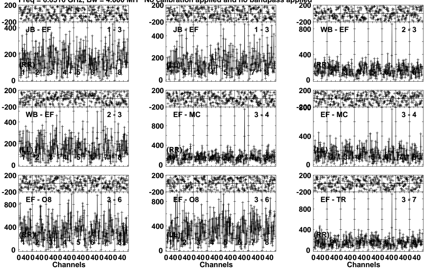
Lower frame: Micro Ampl Jy Top frame: Phas deg Vector averaged cross-power spectrum Several baselines displayed Timerange: 00/15:34:01 to 00/15:37:59
