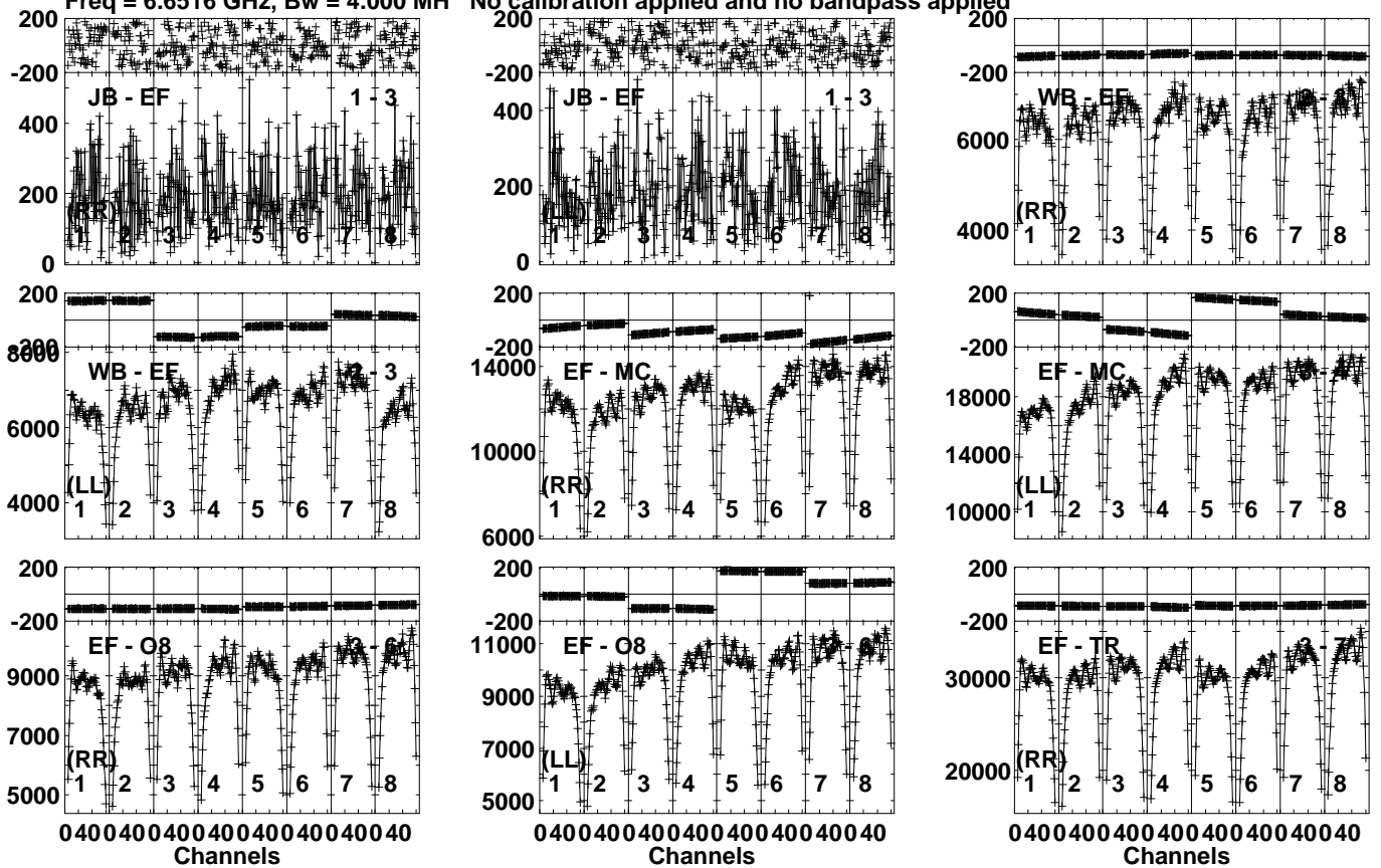
Lower frame: Micro Ampl Jy Top frame: Phas deg Vector averaged cross-power spectrum Several baselines displayed Timerange: 00/16:13:01 to 00/16:16:59
