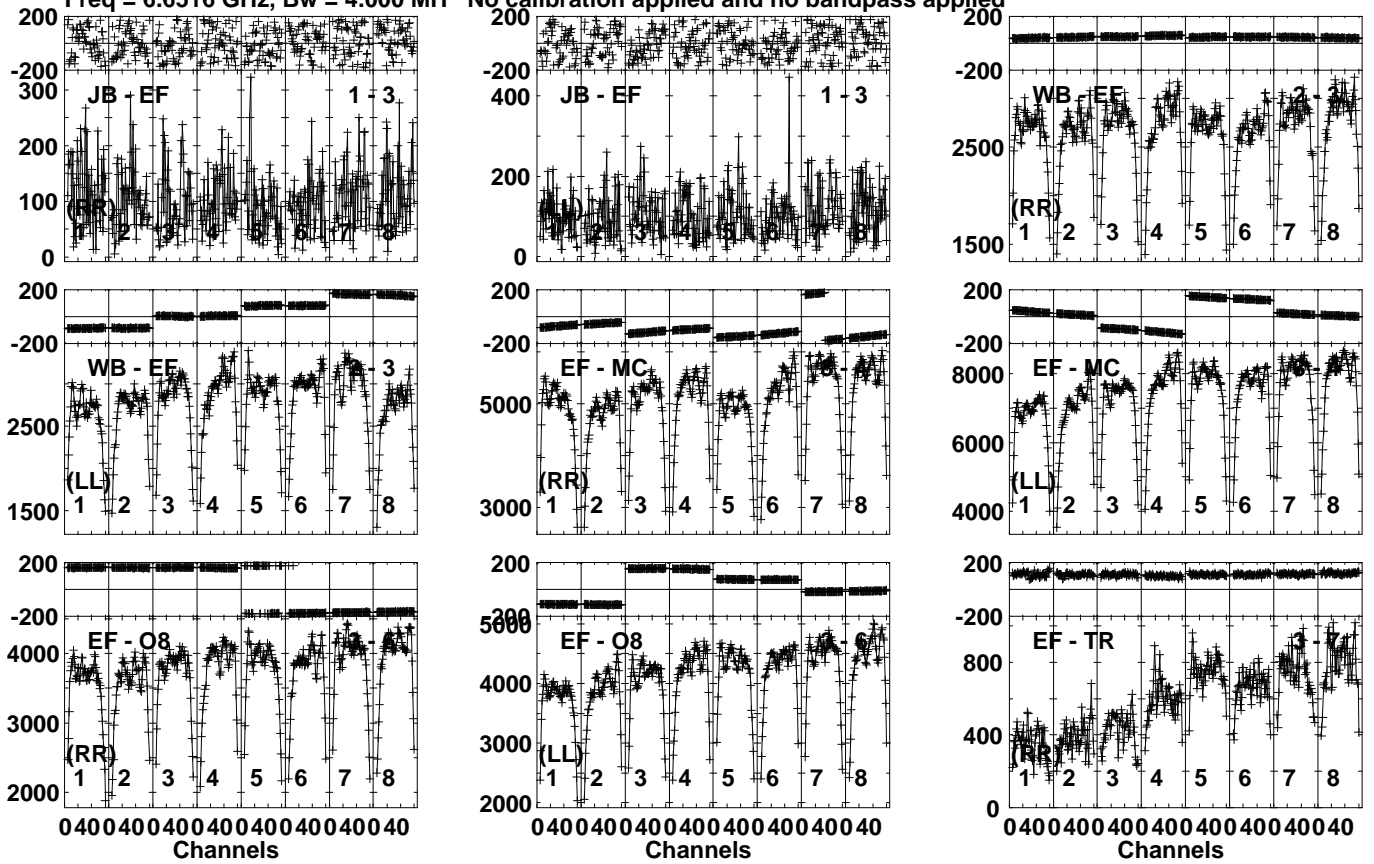
Lower frame: Micro Ampl Jy Top frame: Phas deg Vector averaged cross-power spectrum Several baselines displayed Timerange: 00/15:52:01 to 00/16:01:59
