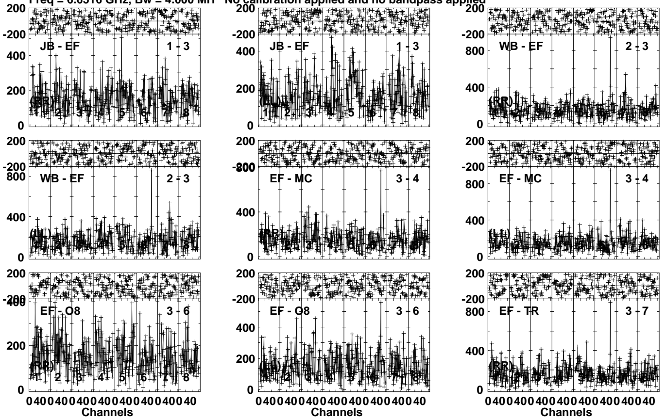
Lower frame: Micro Ampl Jy Top frame: Phas deg Vector averaged cross-power spectrum Several baselines displayed Timerange: 00/15:43:01 to 00/15:46:59
