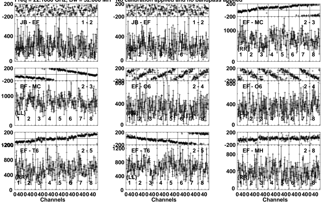
Lower frame: Micro Ampl Jy Top frame: Phas deg Vector averaged cross-power spectrum Several baselines displayed Timerange: 00/10:14:31 to 00/10:15:29
