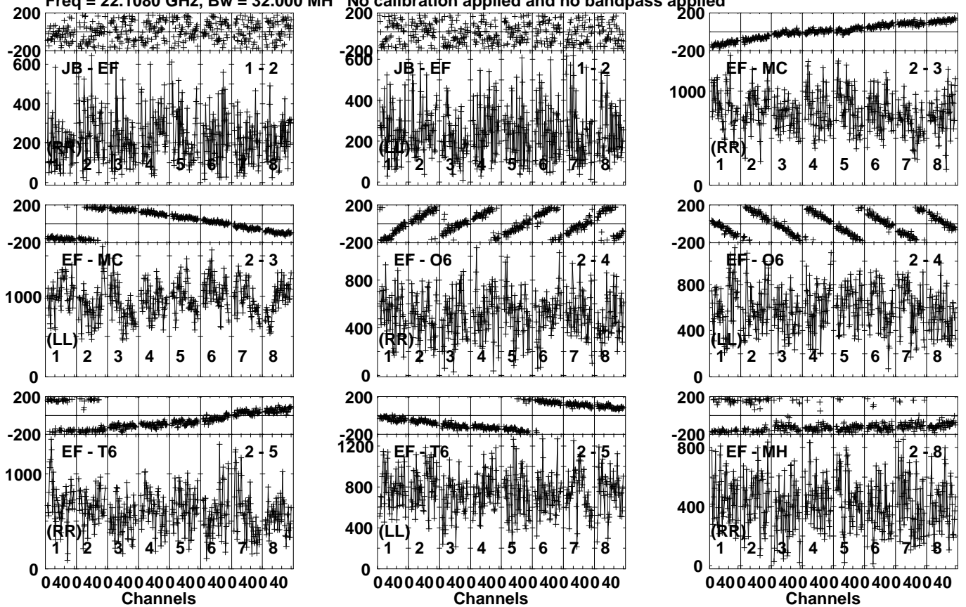
Lower frame: Micro Ampl Jy Top frame: Phas deg Vector averaged cross-power spectrum Several baselines displayed Timerange: 00/13:23:31 to 00/13:24:29
