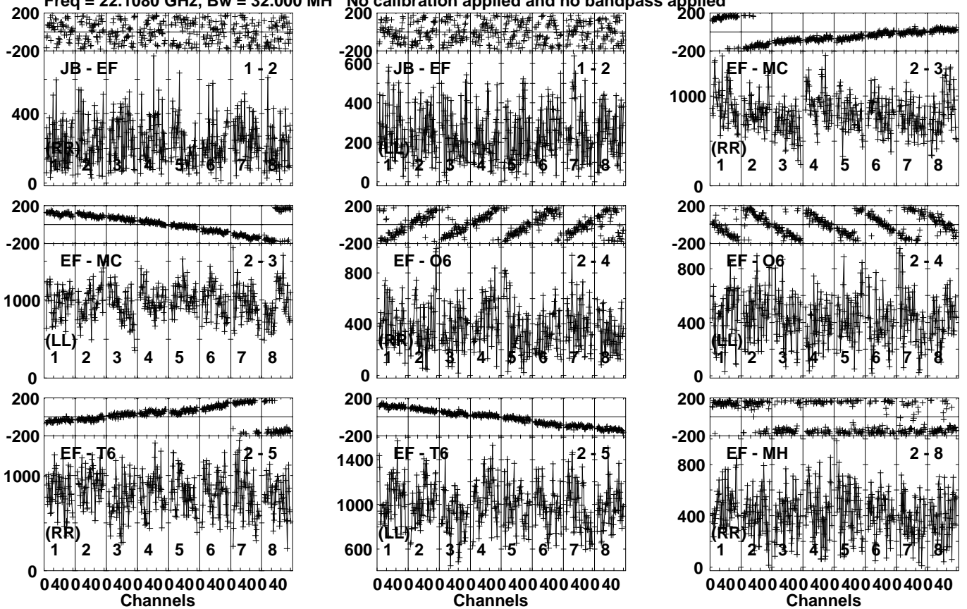
Lower frame: Micro Ampl Jy Top frame: Phas deg Vector averaged cross-power spectrum Several baselines displayed Timerange: 00/12:25:31 to 00/12:26:29
