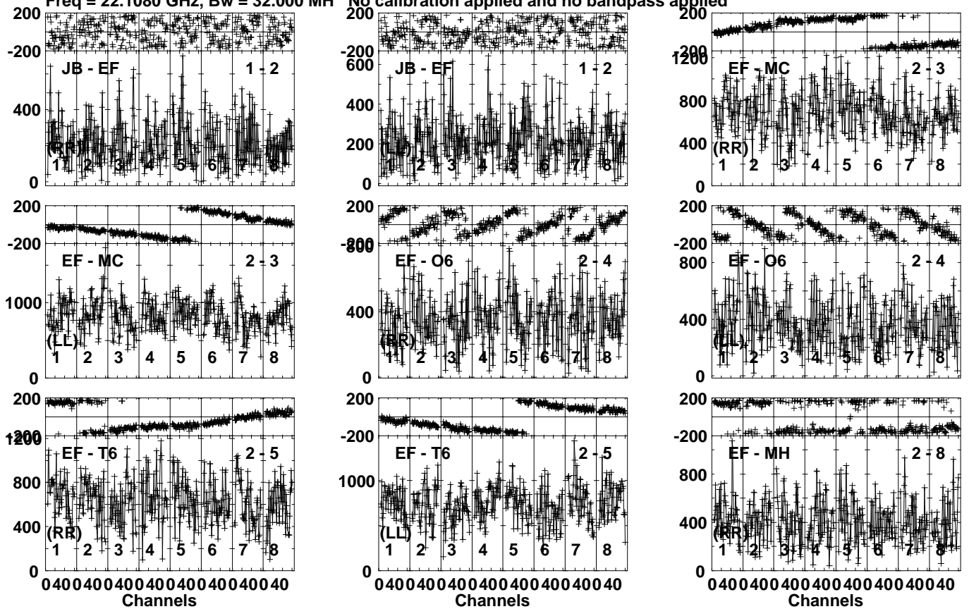
Lower frame: Micro Ampl Jy Top frame: Phas deg Vector averaged cross-power spectrum Several baselines displayed Timerange: 00/11:38:33 to 00/11:39:29
