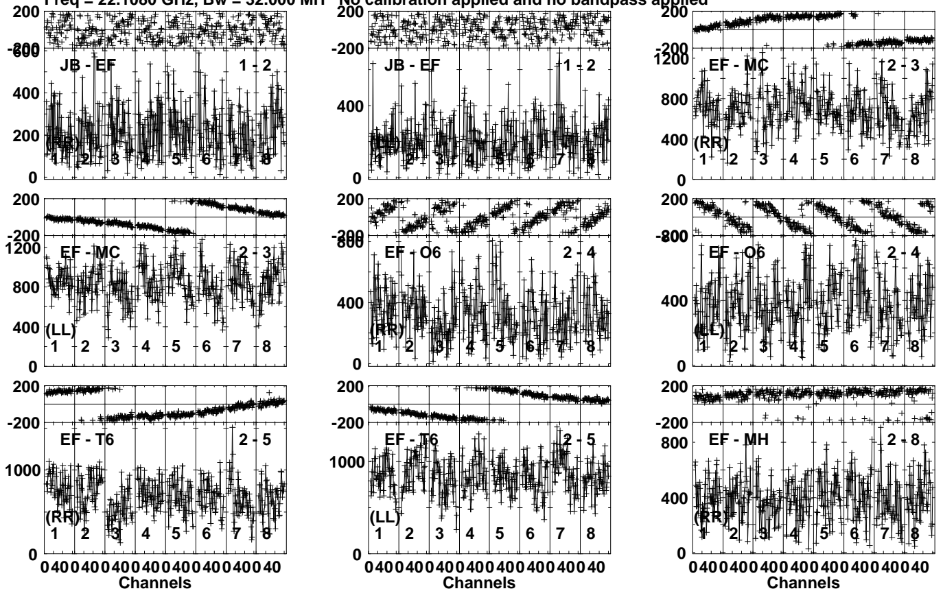
Lower frame: Micro Ampl Jy Top frame: Phas deg Vector averaged cross-power spectrum Several baselines displayed Timerange: 00/11:45:31 to 00/11:46:29
