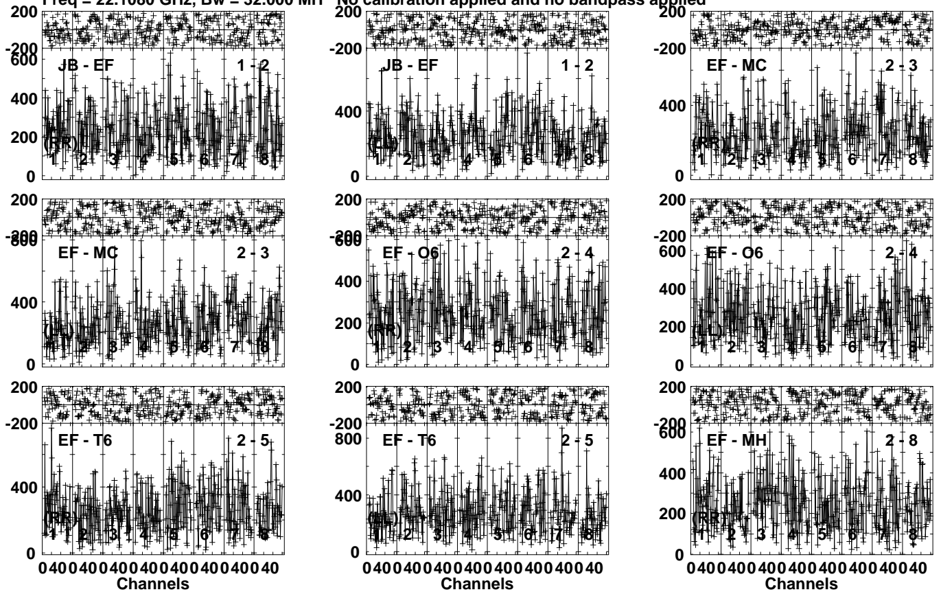
Lower frame: Micro Ampl Jy Top frame: Phas deg Vector averaged cross-power spectrum Several baselines displayed Timerange: 00/13:13:31 to 00/13:14:29
