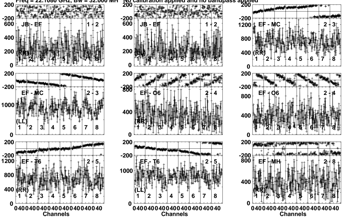
Lower frame: Micro Ampl Jy Top frame: Phas deg Vector averaged cross-power spectrum Several baselines displayed Timerange: 00/11:10:33 to 00/11:11:29
