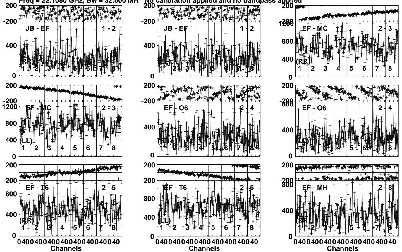
Lower frame: Micro Ampl Jy Top frame: Phas deg Vector averaged cross-power spectrum Several baselines displayed Timerange: 00/10:27:33 to 00/10:28:29
