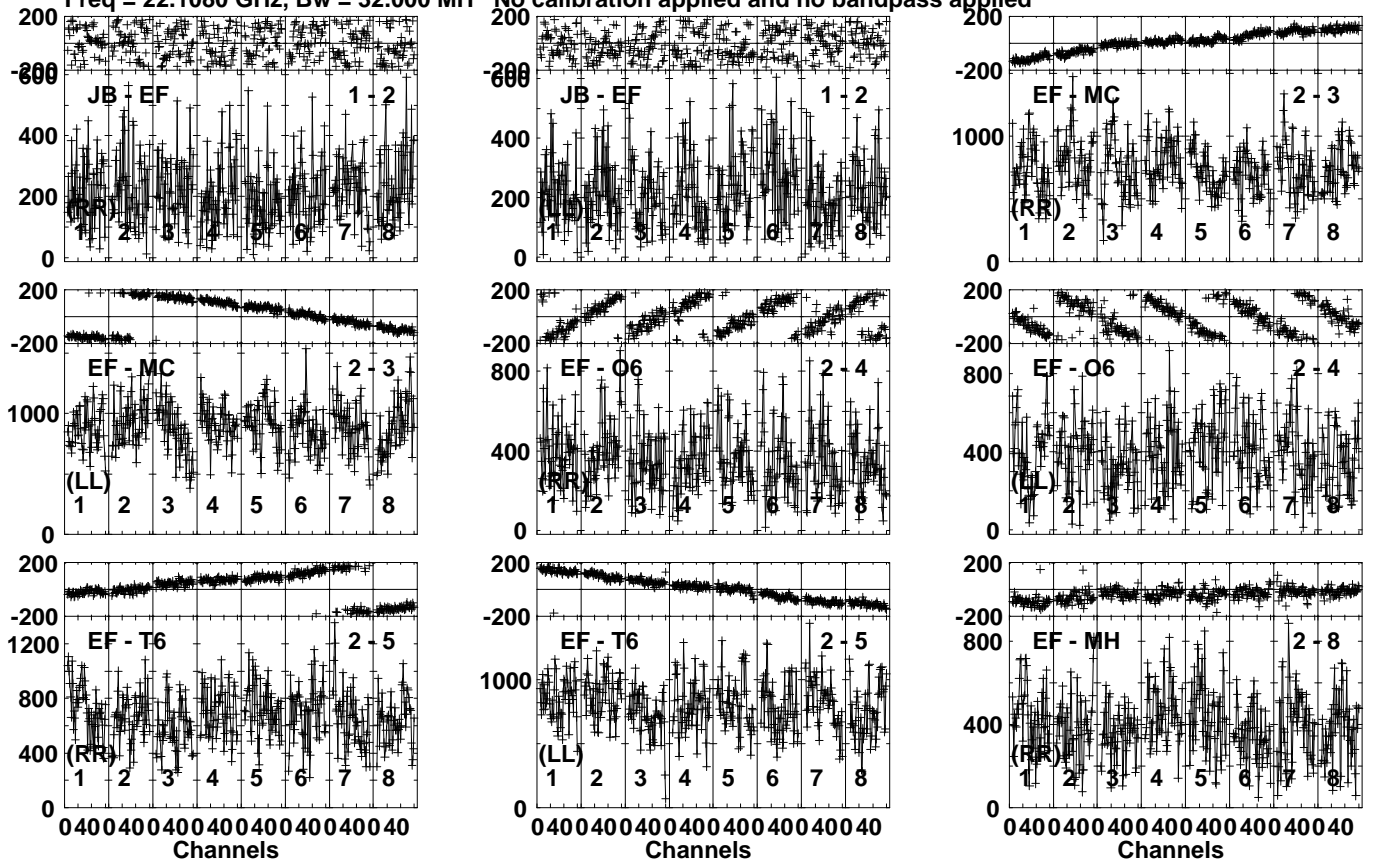
Lower frame: Micro Ampl Jy Top frame: Phas deg Vector averaged cross-power spectrum Several baselines displayed Timerange: 00/11:32:31 to 00/11:33:29
