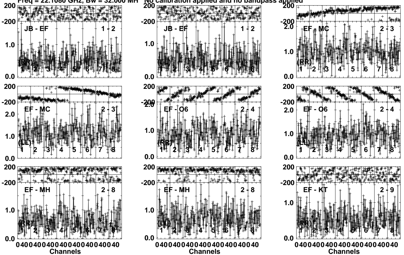
Lower frame: Milli Ampl Jy Top frame: Phas deg Vector averaged cross-power spectrum Several baselines displayed Timerange: 00/14:33:33 to 00/14:34:29
