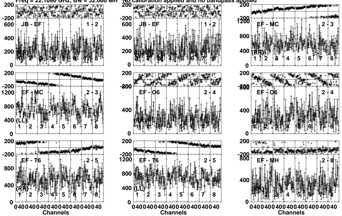
Lower frame: Micro Ampl Jy Top frame: Phas deg Vector averaged cross-power spectrum Several baselines displayed Timerange: 00/10:42:33 to 00/10:43:29
