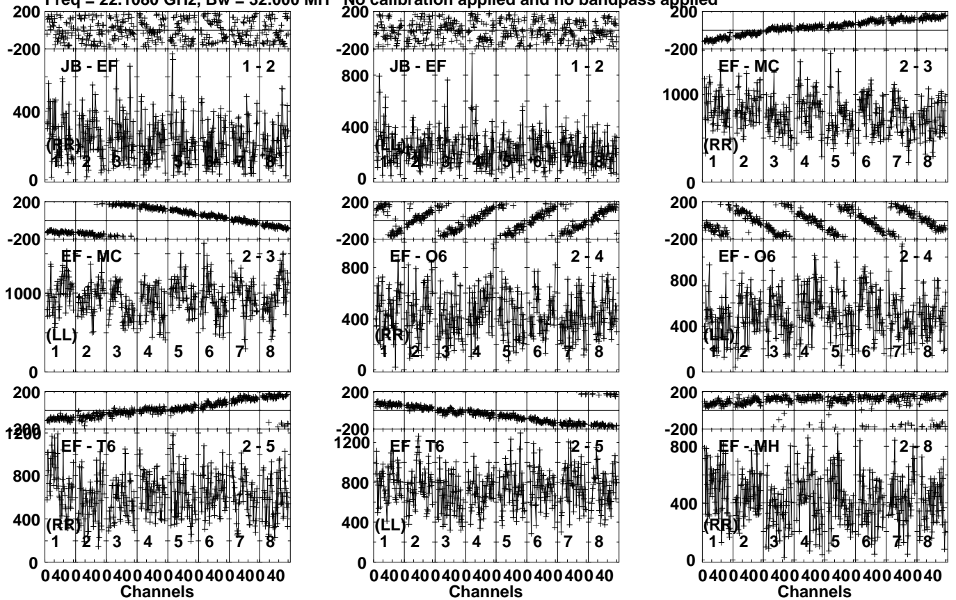
Lower frame: Micro Ampl Jy Top frame: Phas deg Vector averaged cross-power spectrum Several baselines displayed Timerange: 00/13:12:31 to 00/13:13:29
