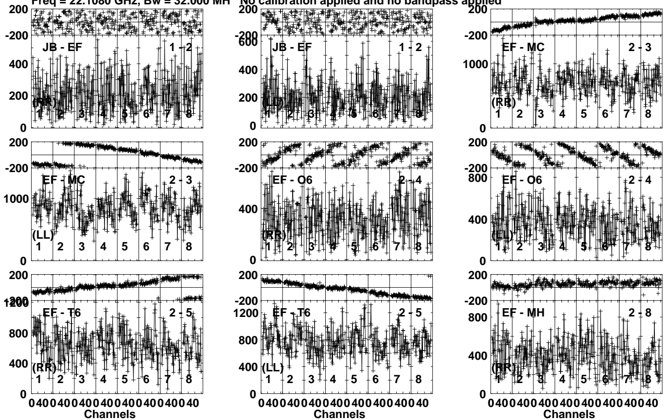
Lower frame: Micro Ampl Jy Top frame: Phas deg Vector averaged cross-power spectrum Several baselines displayed Timerange: 00/11:27:33 to 00/11:28:29
