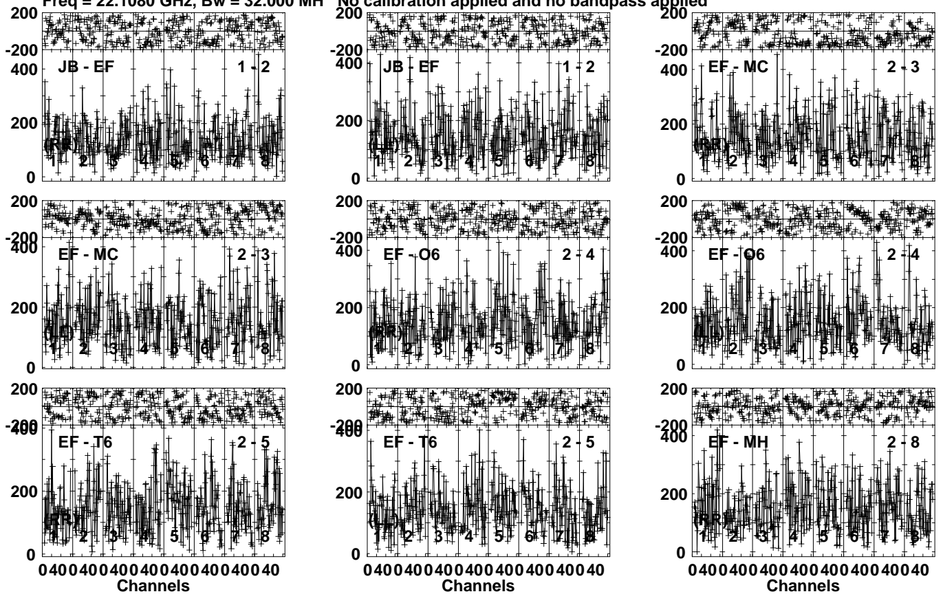
Lower frame: Micro Ampl Jy Top frame: Phas deg Vector averaged cross-power spectrum Several baselines displayed Timerange: 00/14:50:31 to 00/14:51:29
