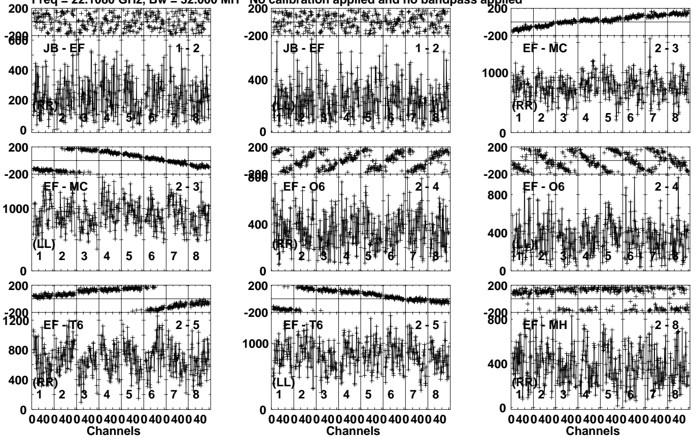
Lower frame: Micro Ampl Jy Top frame: Phas deg Vector averaged cross-power spectrum Several baselines displayed Timerange: 00/11:04:31 to 00/11:05:29
