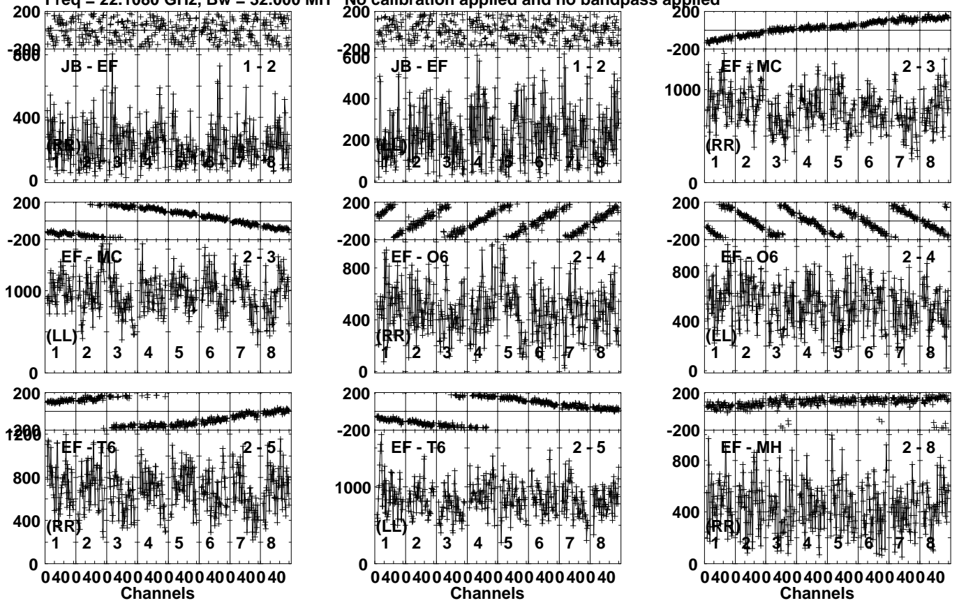
Lower frame: Micro Ampl Jy Top frame: Phas deg Vector averaged cross-power spectrum Several baselines displayed Timerange: 00/13:10:33 to 00/13:11:29
