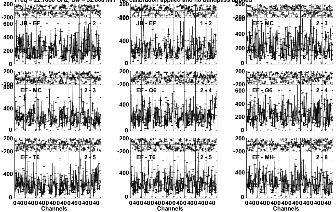
Lower frame: Micro Ampl Jy Top frame: Phas deg Vector averaged cross-power spectrum Several baselines displayed Timerange: 00/10:32:31 to 00/10:33:29
