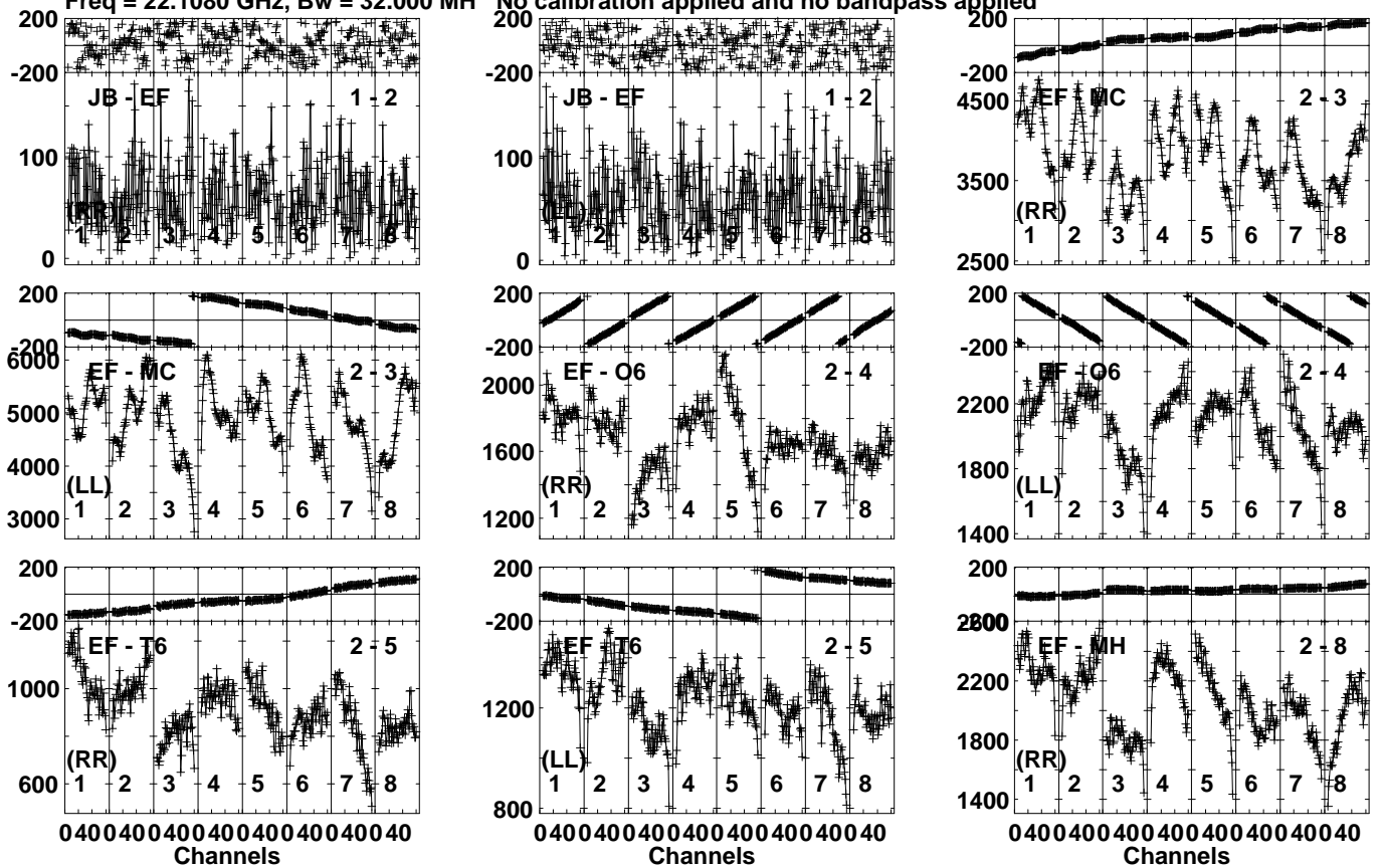
Lower frame: Micro Ampl Jy Top frame: Phas deg Vector averaged cross-power spectrum Several baselines displayed Timerange: 00/11:48:31 to 00/11:53:29
