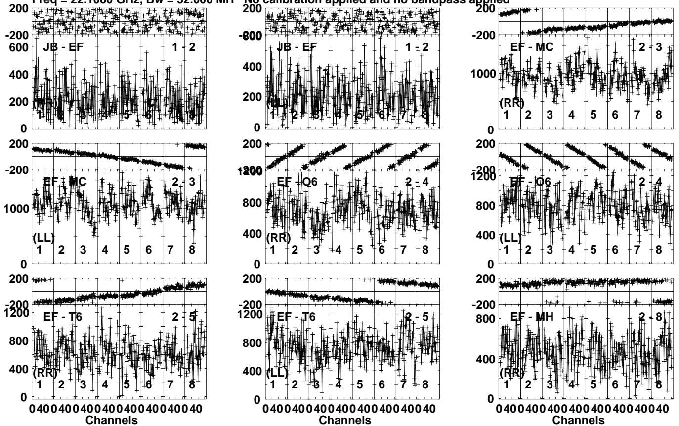
Lower frame: Micro Ampl Jy Top frame: Phas deg Vector averaged cross-power spectrum Several baselines displayed Timerange: 00/14:03:31 to 00/14:04:29
