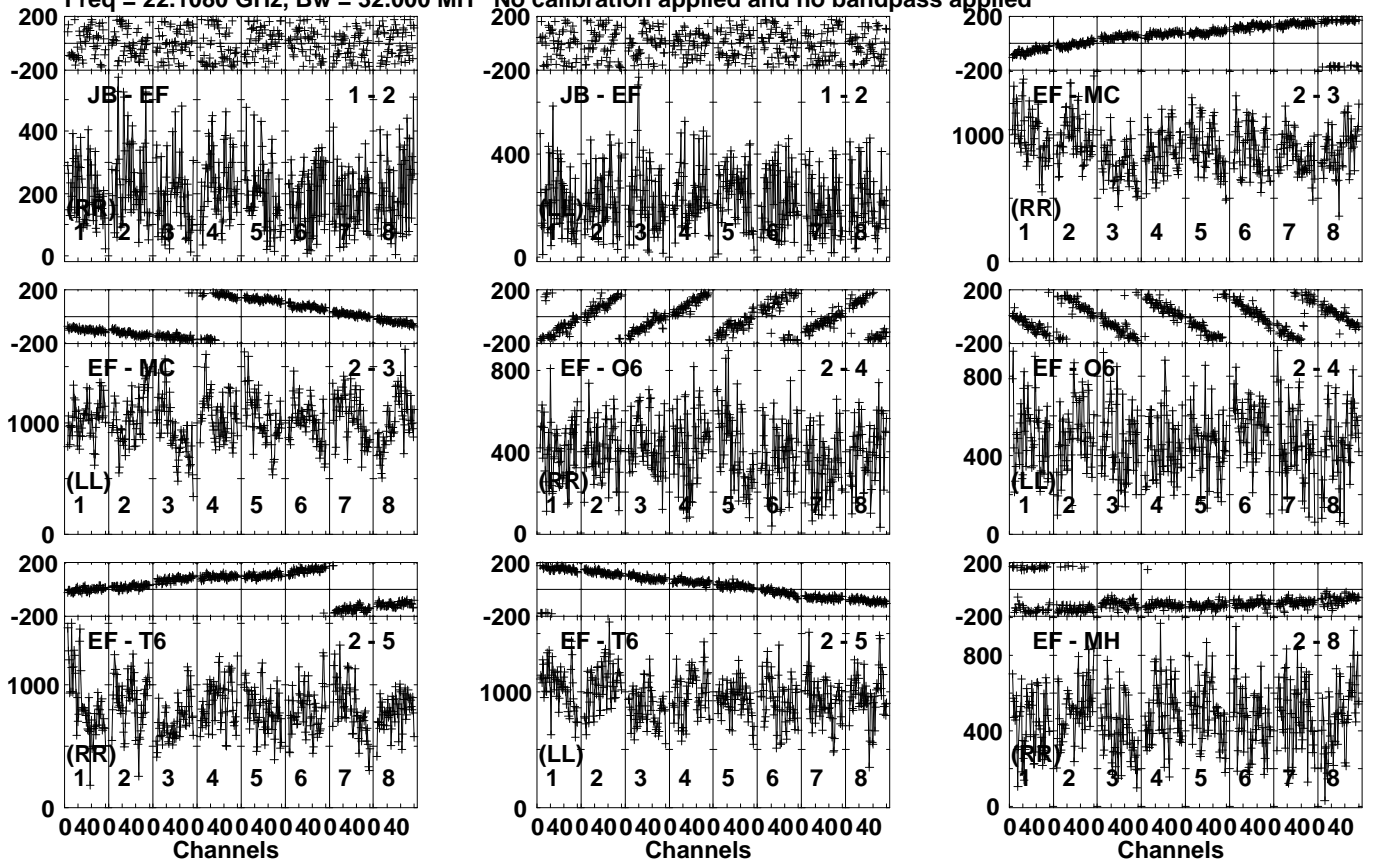
Lower frame: Micro Ampl Jy Top frame: Phas deg Vector averaged cross-power spectrum Several baselines displayed Timerange: 00/12:40:31 to 00/12:41:29
