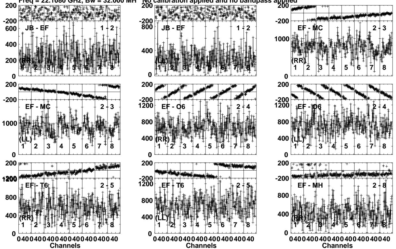
Lower frame: Micro Ampl Jy Top frame: Phas deg Vector averaged cross-power spectrum Several baselines displayed Timerange: 00/14:59:03 to 00/14:59:59
