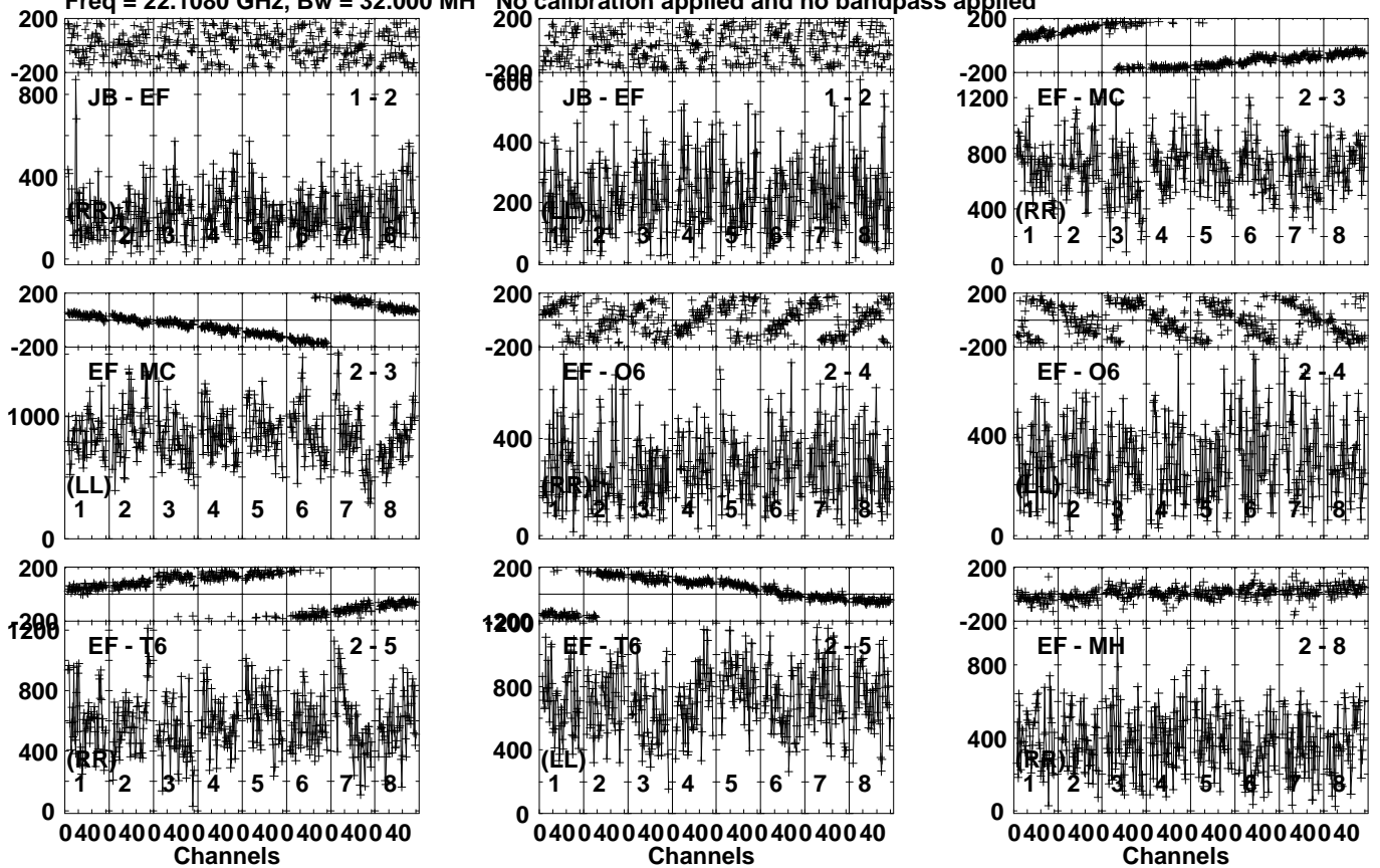
Lower frame: Micro Ampl Jy Top frame: Phas deg Vector averaged cross-power spectrum Several baselines displayed Timerange: 00/10:31:33 to 00/10:32:29
