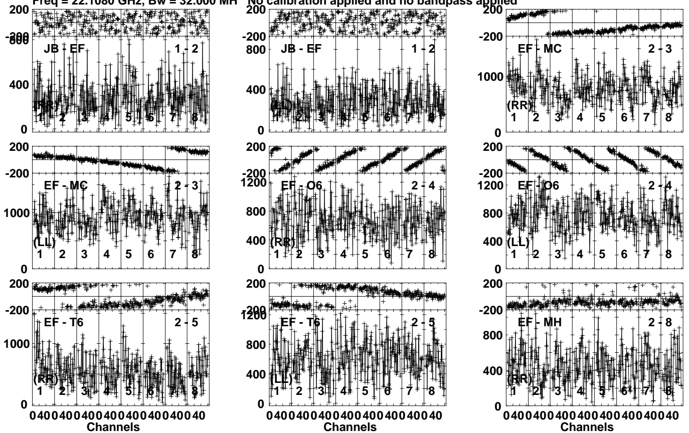
Lower frame: Micro Ampl Jy Top frame: Phas deg Vector averaged cross-power spectrum Several baselines displayed Timerange: 00/14:55:31 to 00/14:56:29
