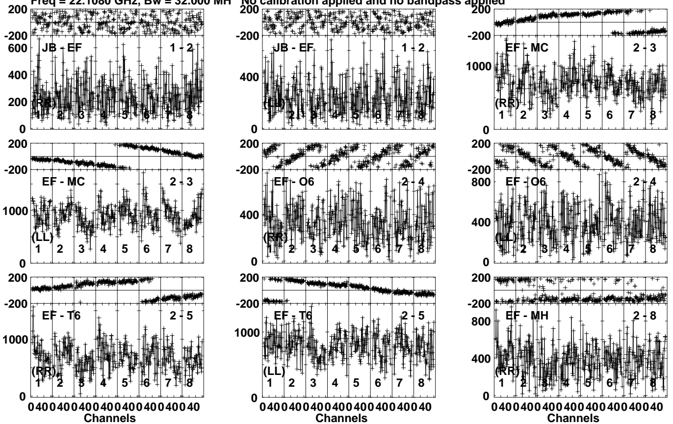
Lower frame: Micro Ampl Jy Top frame: Phas deg Vector averaged cross-power spectrum Several baselines displayed Timerange: 00/11:08:31 to 00/11:09:29
