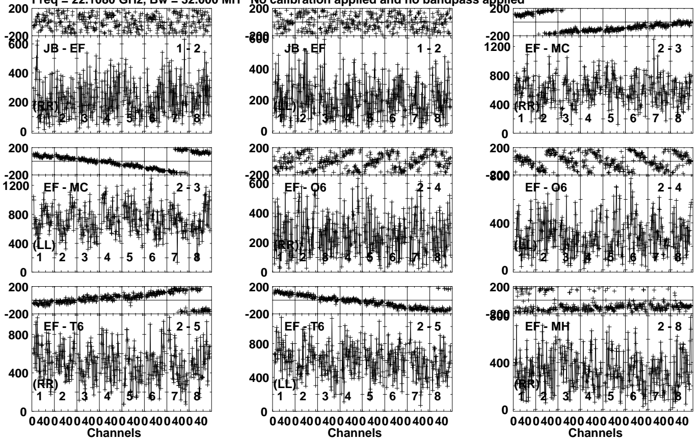
Lower frame: Micro Ampl Jy Top frame: Phas deg Vector averaged cross-power spectrum Several baselines displayed Timerange: 00/10:51:31 to 00/10:52:29
