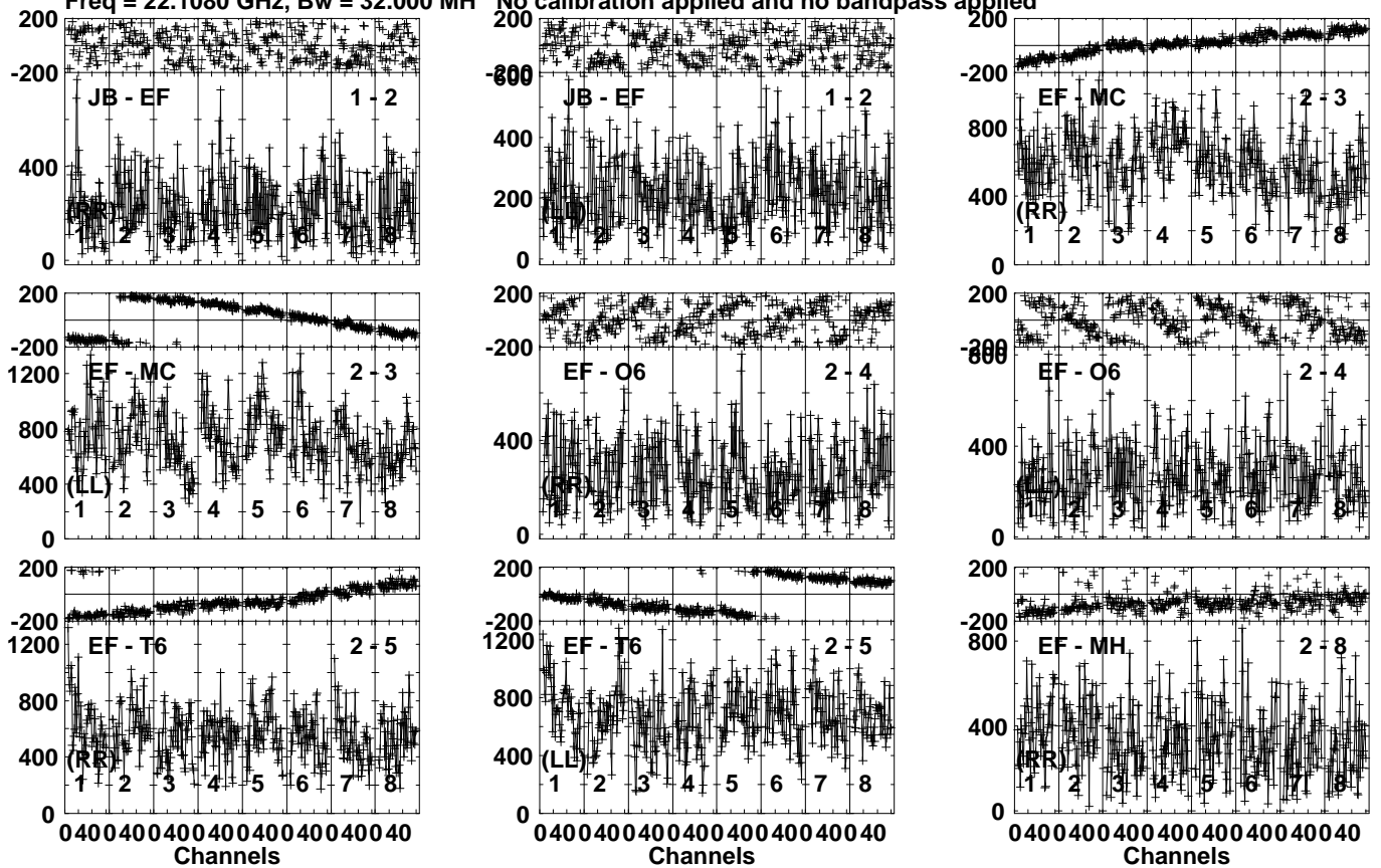
Lower frame: Micro Ampl Jy Top frame: Phas deg Vector averaged cross-power spectrum Several baselines displayed Timerange: 00/10:38:31 to 00/10:39:29
