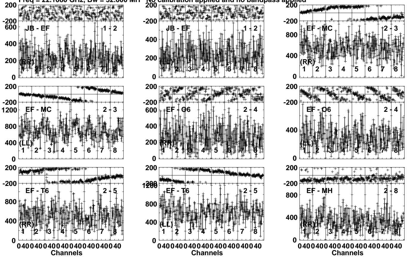
Lower frame: Micro Ampl Jy Top frame: Phas deg Vector averaged cross-power spectrum Several baselines displayed Timerange: 00/10:46:33 to 00/10:47:29
