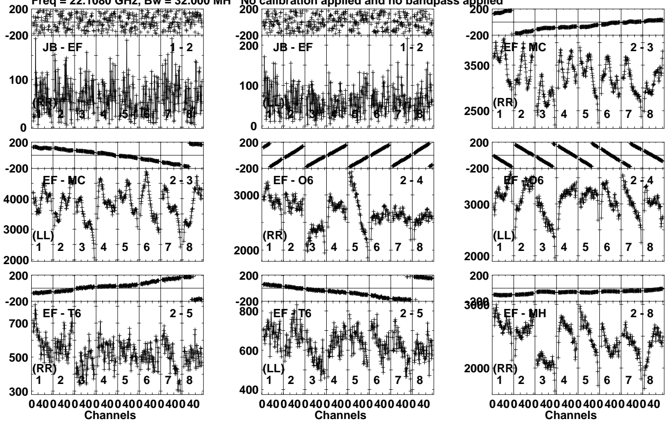
Lower frame: Micro Ampl Jy Top frame: Phas deg Vector averaged cross-power spectrum Several baselines displayed Timerange: 00/13:37:31 to 00/13:42:29
