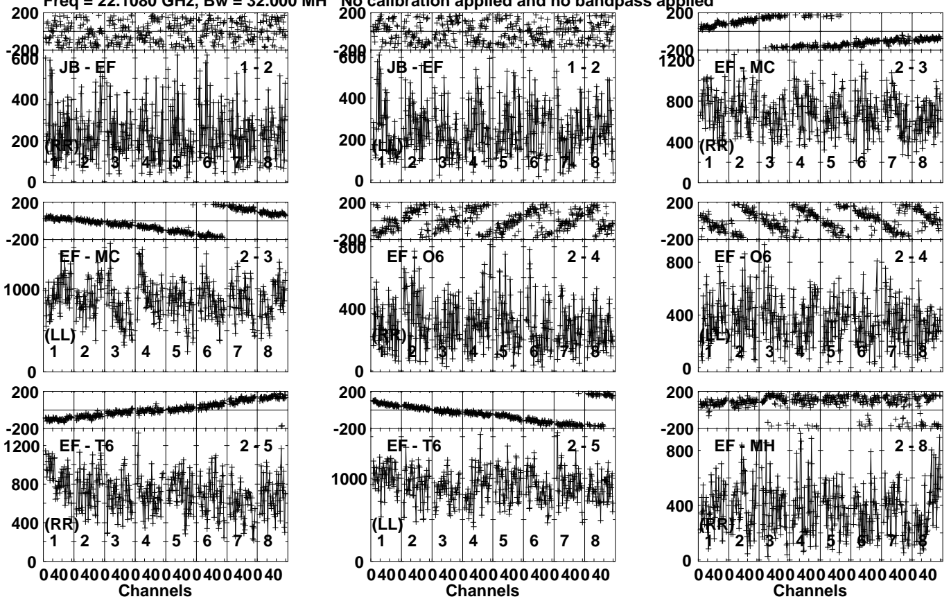
Lower frame: Micro Ampl Jy Top frame: Phas deg Vector averaged cross-power spectrum Several baselines displayed Timerange: 00/12:05:31 to 00/12:06:29
