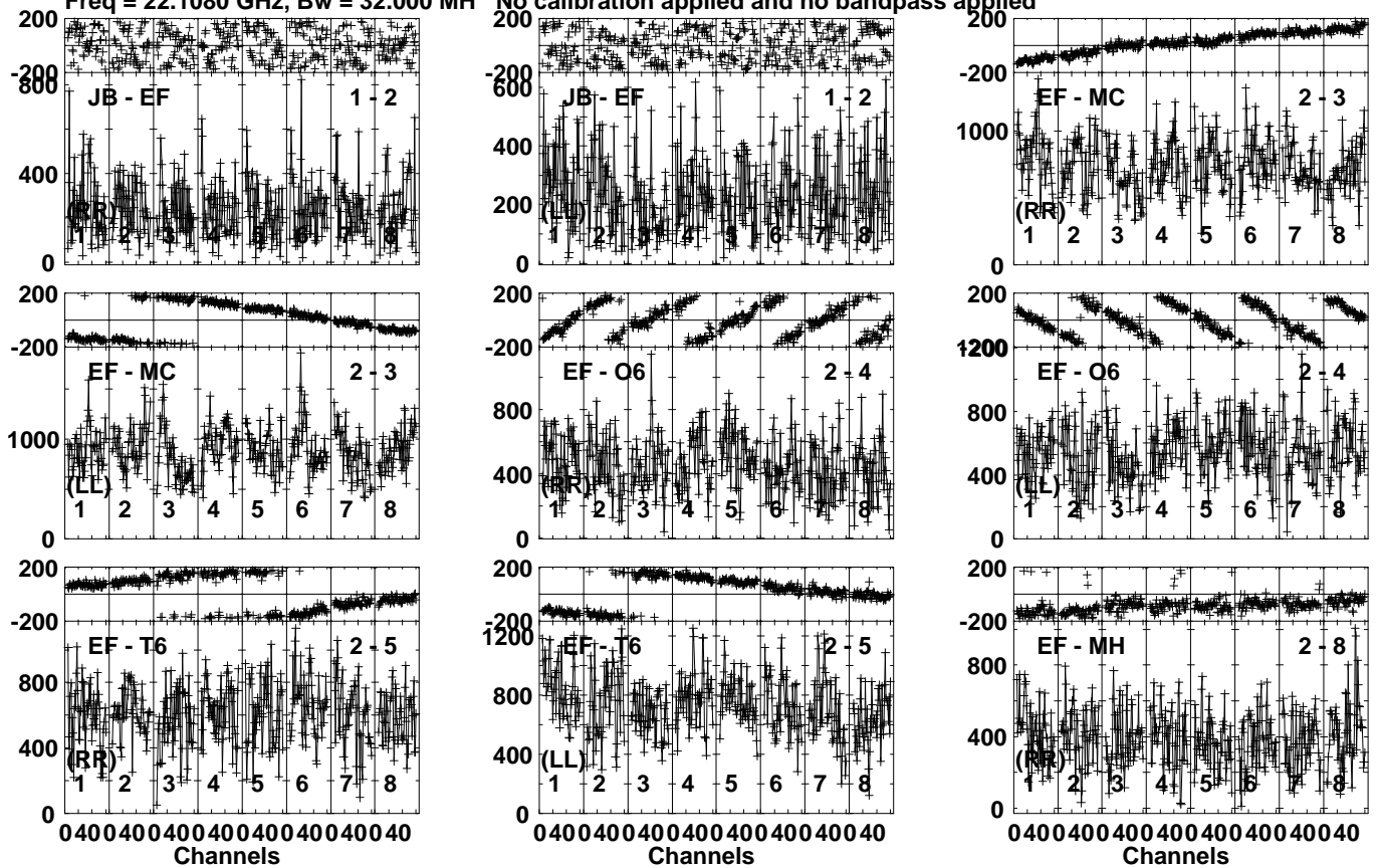
Lower frame: Micro Ampl Jy Top frame: Phas deg Vector averaged cross-power spectrum Several baselines displayed Timerange: 00/13:21:31 to 00/13:22:29
