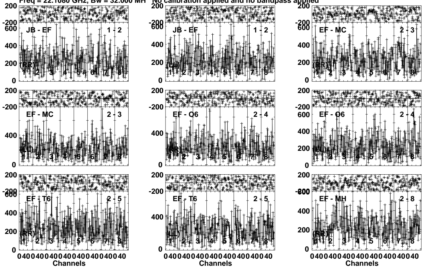
Lower frame: Micro Ampl Jy Top frame: Phas deg Vector averaged cross-power spectrum Several baselines displayed Timerange: 00/10:15:33 to 00/10:16:29
