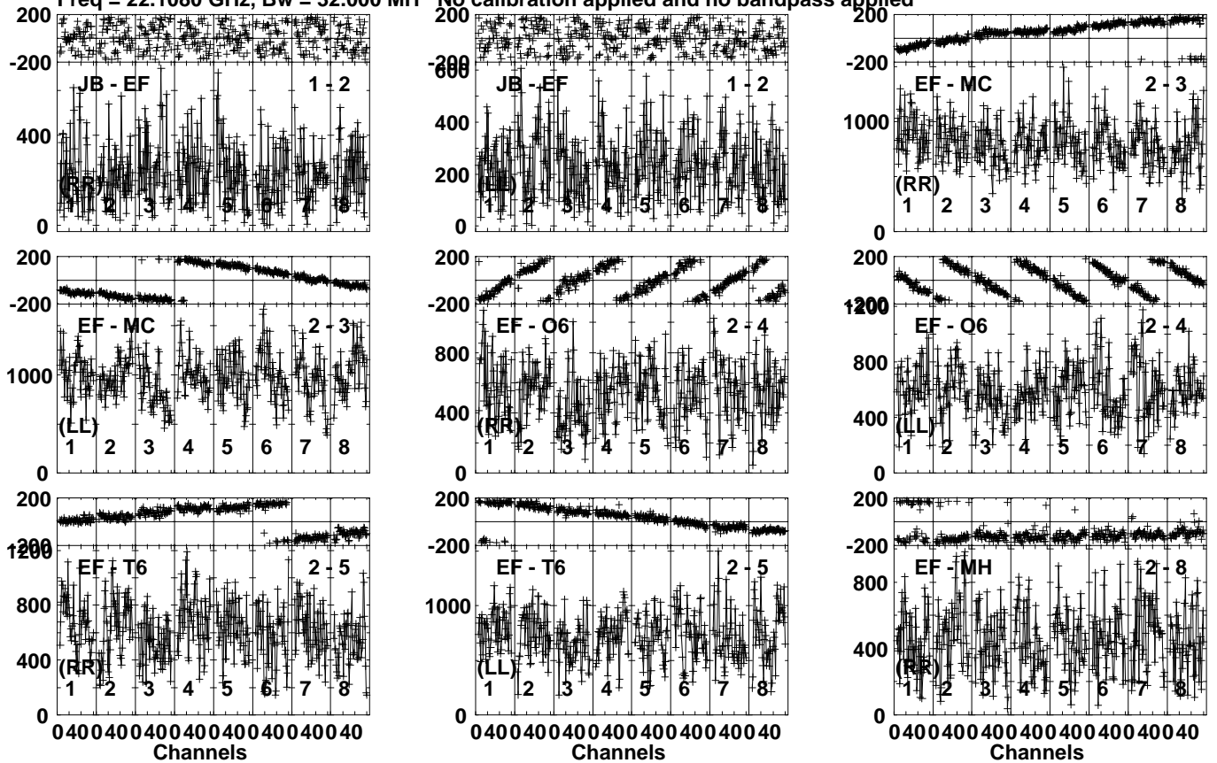
Lower frame: Micro Ampl Jy Top frame: Phas deg Vector averaged cross-power spectrum Several baselines displayed Timerange: 00/13:25:33 to 00/13:26:29
