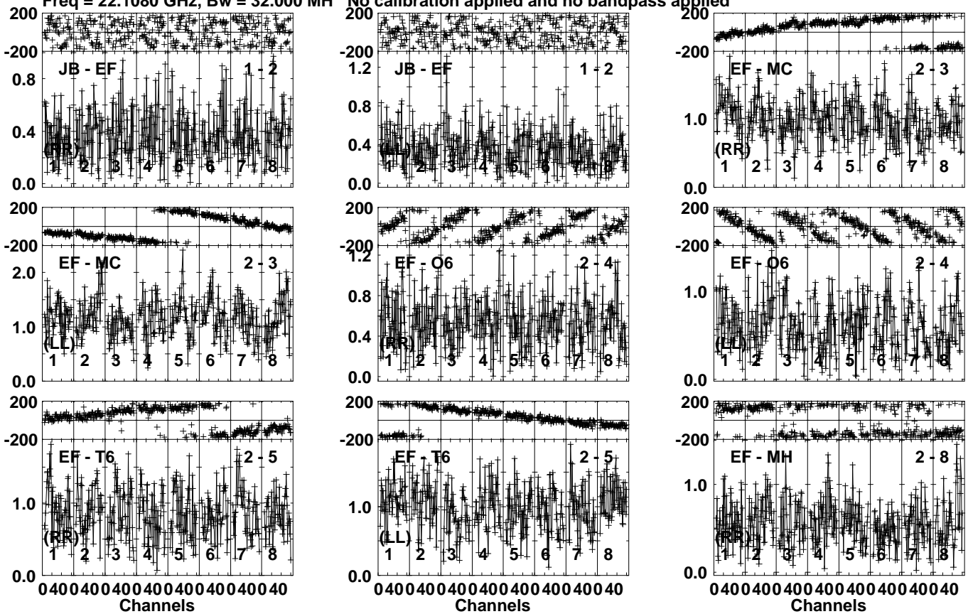
Lower frame: Milli Ampl Jy Top frame: Phas deg Vector averaged cross-power spectrum Several baselines displayed Timerange: 00/12:51:31 to 00/12:52:29
