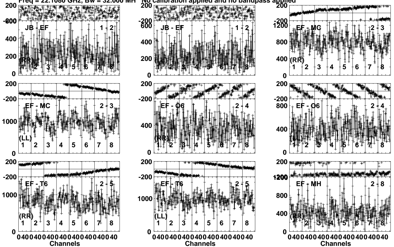
Lower frame: Micro Ampl Jy Top frame: Phas deg Vector averaged cross-power spectrum Several baselines displayed Timerange: 00/12:12:31 to 00/12:13:29
