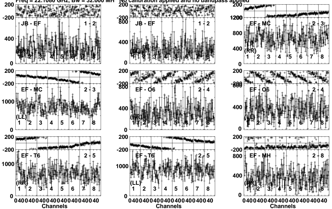
Lower frame: Micro Ampl Jy Top frame: Phas deg Vector averaged cross-power spectrum Several baselines displayed Timerange: 00/11:59:31 to 00/12:00:29
