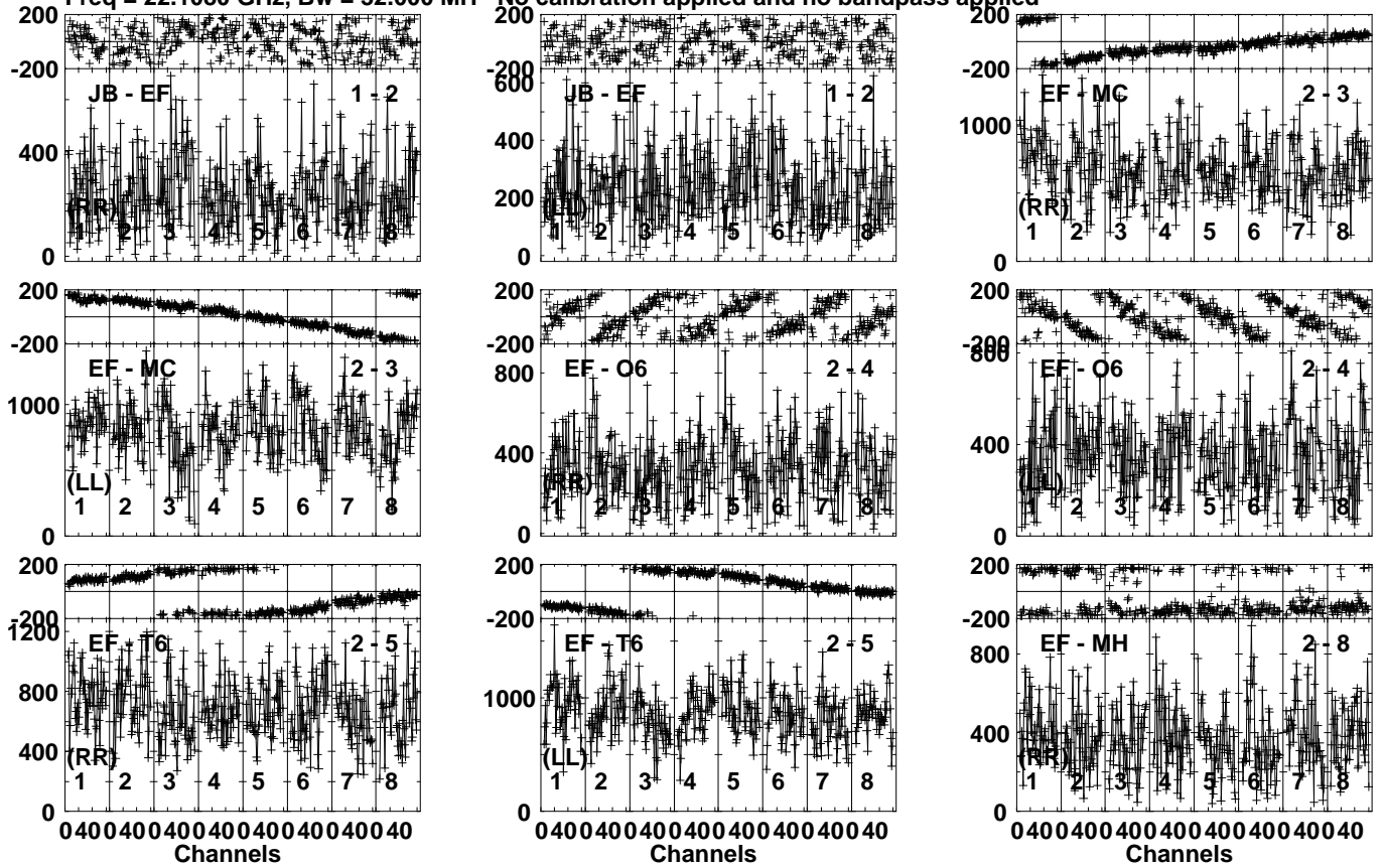
Lower frame: Micro Ampl Jy Top frame: Phas deg Vector averaged cross-power spectrum Several baselines displayed Timerange: 00/12:03:31 to 00/12:04:29
