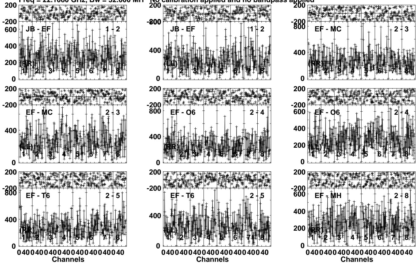
Lower frame: Micro Ampl Jy Top frame: Phas deg Vector averaged cross-power spectrum Several baselines displayed Timerange: 00/12:06:33 to 00/12:07:29
