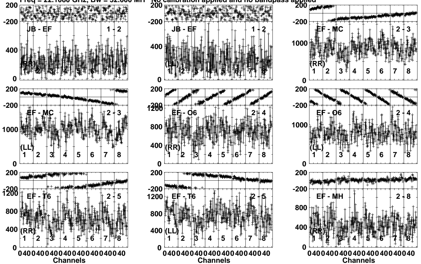
Lower frame: Micro Ampl Jy Top frame: Phas deg Vector averaged cross-power spectrum Several baselines displayed Timerange: 00/14:08:31 to 00/14:09:29
