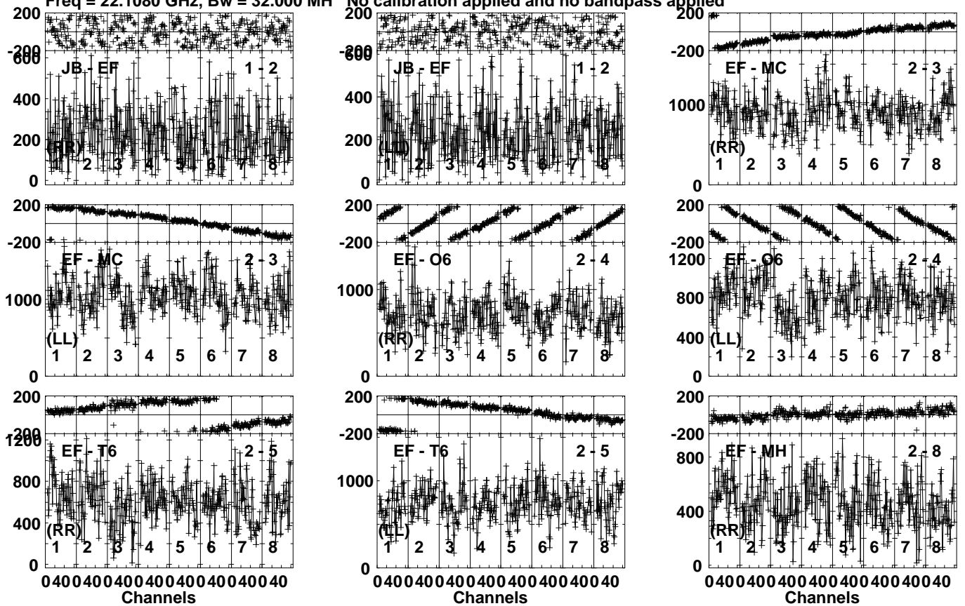
Lower frame: Micro Ampl Jy Top frame: Phas deg Vector averaged cross-power spectrum Several baselines displayed Timerange: 00/14:10:31 to 00/14:11:29
