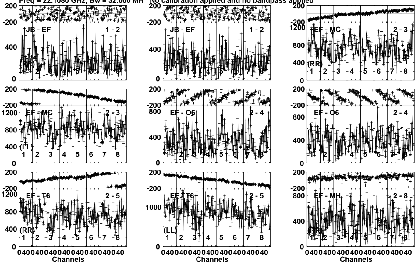
Lower frame: Micro Ampl Jy Top frame: Phas deg Vector averaged cross-power spectrum Several baselines displayed Timerange: 00/11:25:33 to 00/11:26:29
