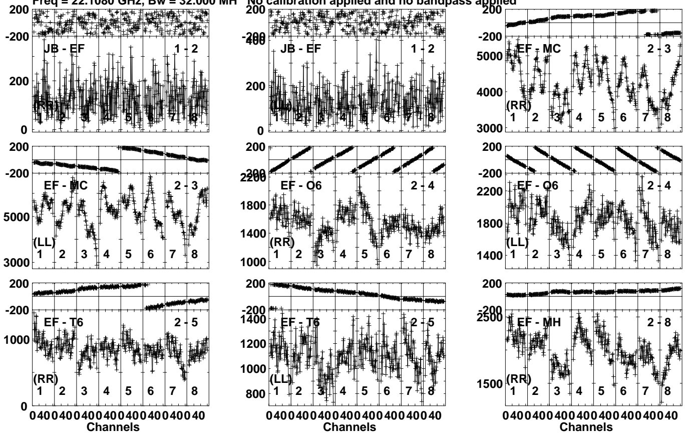
Lower frame: Micro Ampl Jy Top frame: Phas deg Vector averaged cross-power spectrum Several baselines displayed Timerange: 00/10:00:01 to 00/10:04:59
