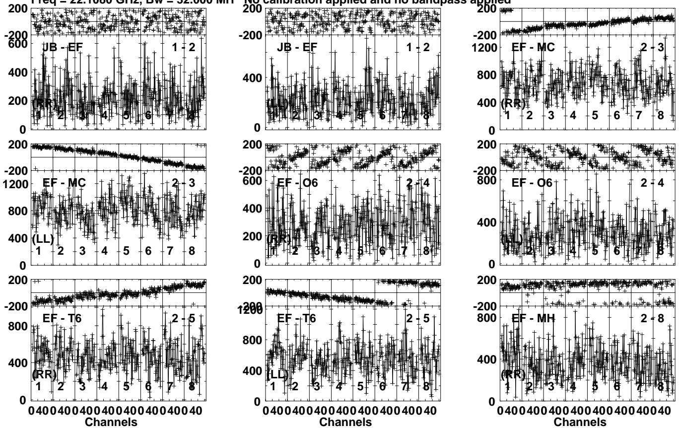
Lower frame: Micro Ampl Jy Top frame: Phas deg Vector averaged cross-power spectrum Several baselines displayed Timerange: 00/10:23:31 to 00/10:24:29
