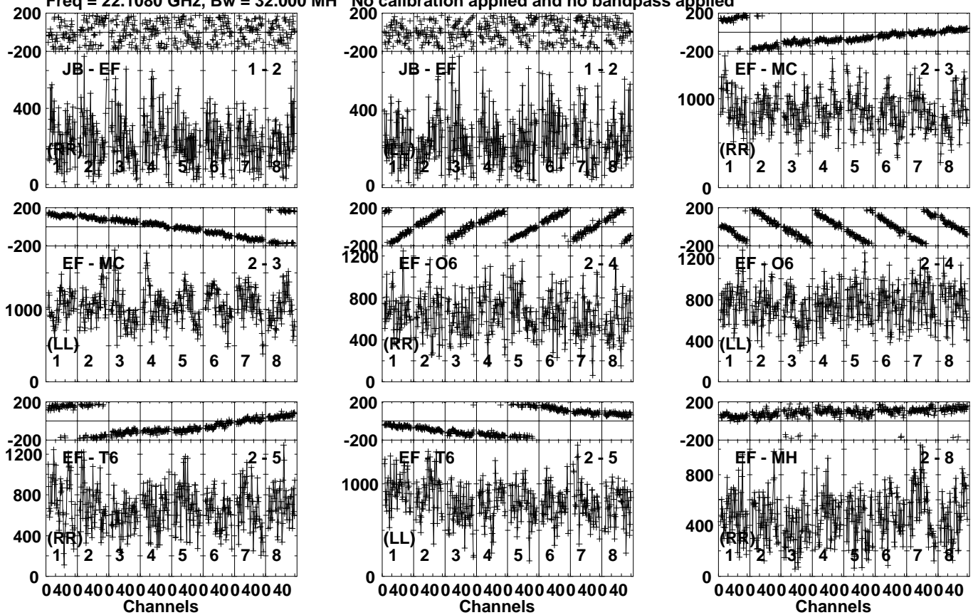
Lower frame: Micro Ampl Jy Top frame: Phas deg Vector averaged cross-power spectrum Several baselines displayed Timerange: 00/13:55:31 to 00/13:56:29
