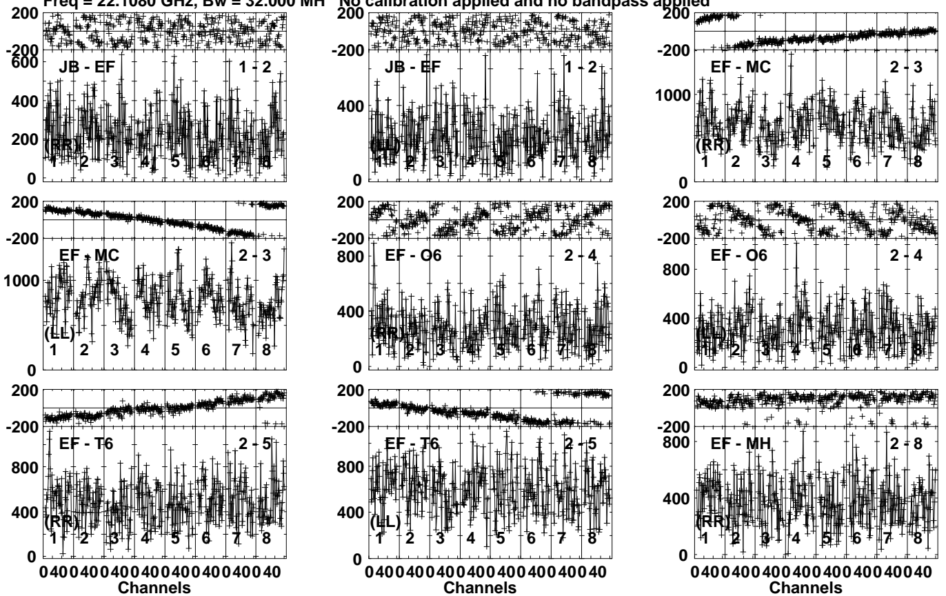
Lower frame: Micro Ampl Jy Top frame: Phas deg Vector averaged cross-power spectrum Several baselines displayed Timerange: 00/10:25:31 to 00/10:26:29
