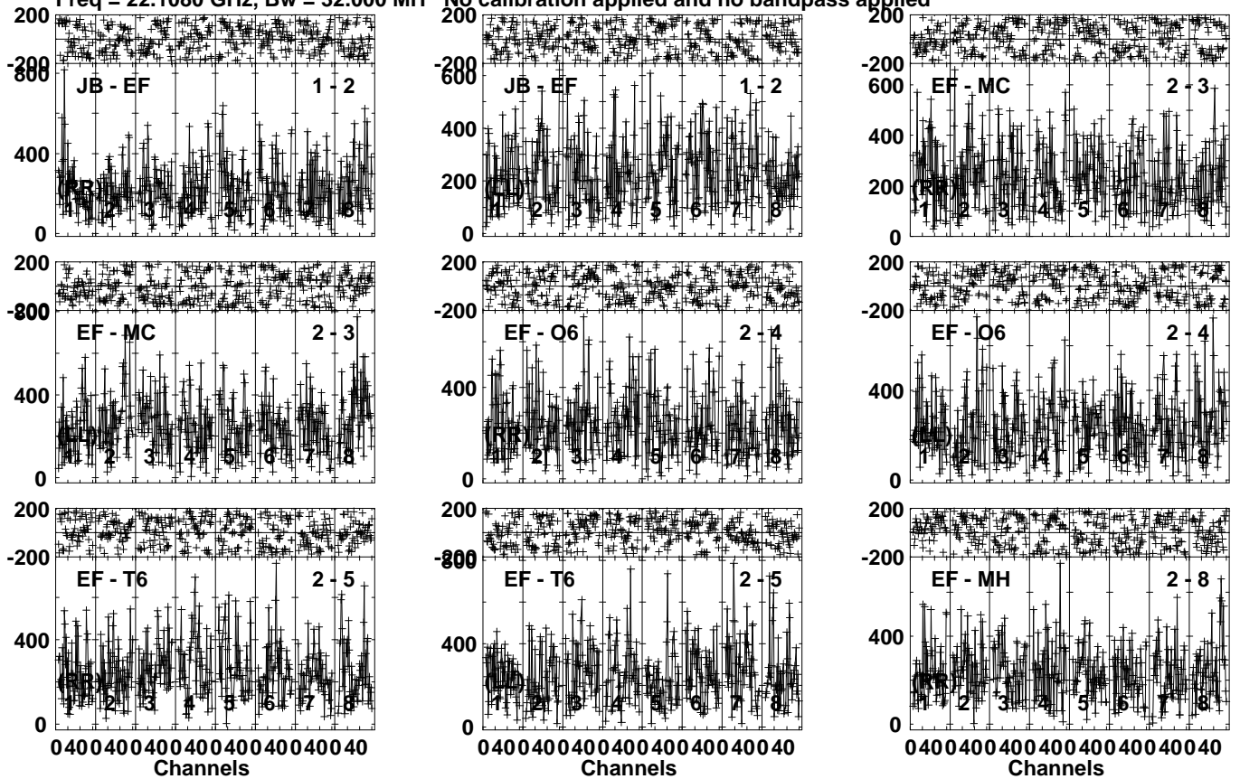
Lower frame: Micro Ampl Jy Top frame: Phas deg Vector averaged cross-power spectrum Several baselines displayed Timerange: 00/11:22:31 to 00/11:23:29
