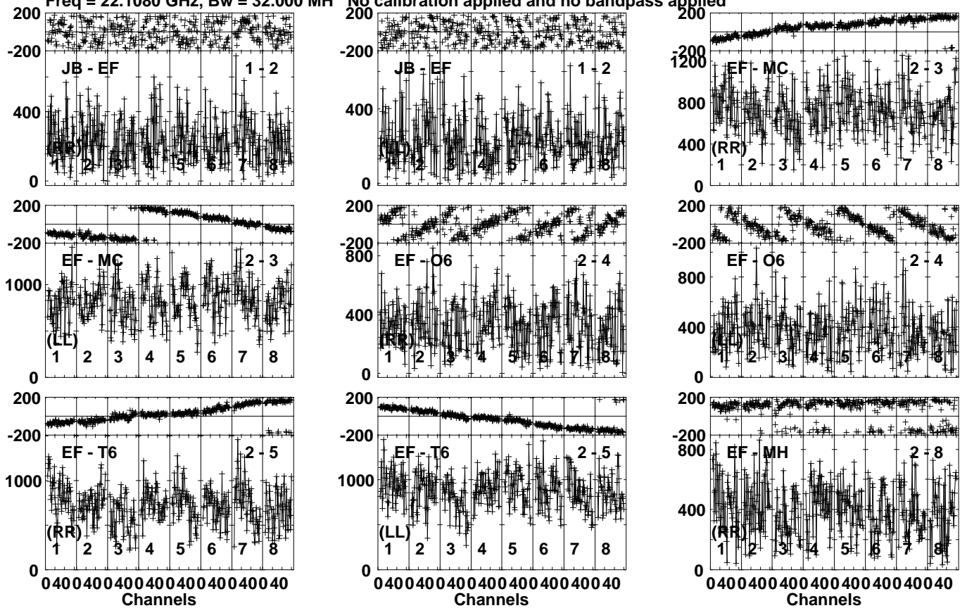
Lower frame: Micro Ampl Jy Top frame: Phas deg Vector averaged cross-power spectrum Several baselines displayed Timerange: 00/11:40:33 to 00/11:41:29
