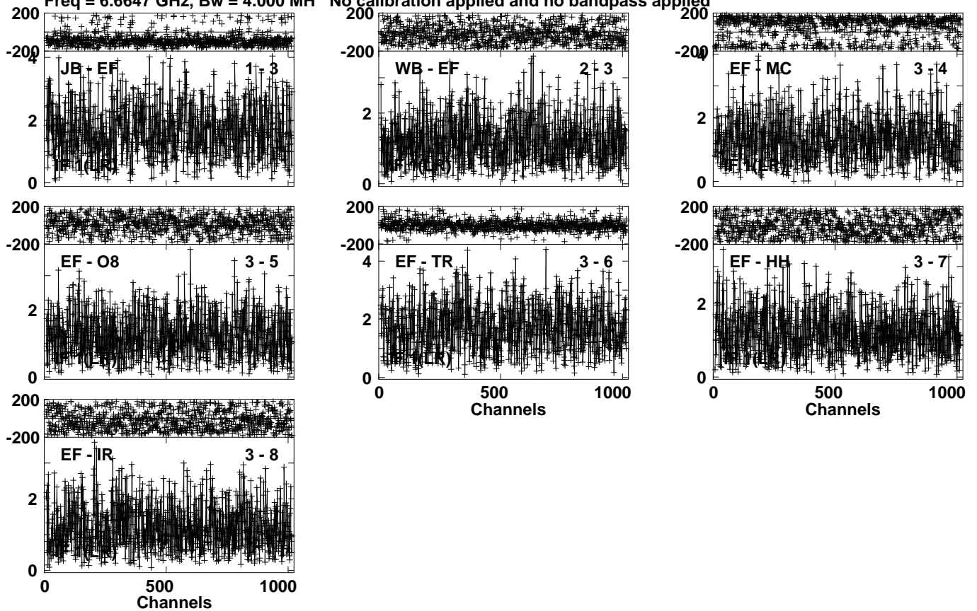
Lower frame: Milli Amp Jy Top frame: Phas deg Vector averaged cross-power spectrum Several baselines displayed Timerange: 00/14:22:40 to 00/14:24:40
