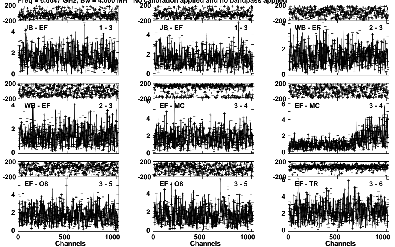
Lower frame: Milli Ampl Jy Top frame: Phas deg Vector averaged cross-power spectrum Several baselines displayed Timerange: 00/17:21:04 to 00/17:22:59
