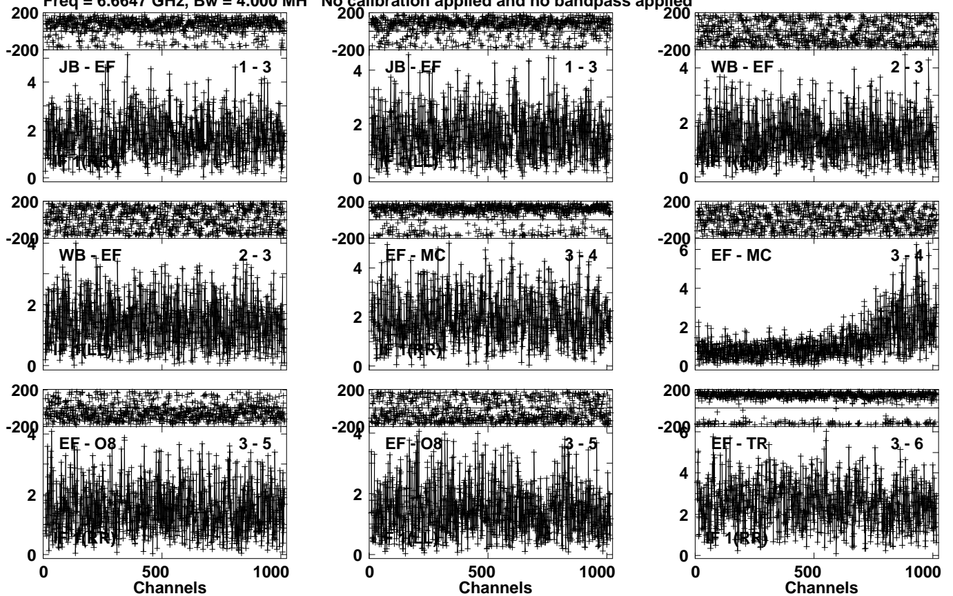
Lower frame: Milli Ampl Jy Top frame: Phas deg Vector averaged cross-power spectrum Several baselines displayed Timerange: 00/14:46:22 to 00/14:48:19
