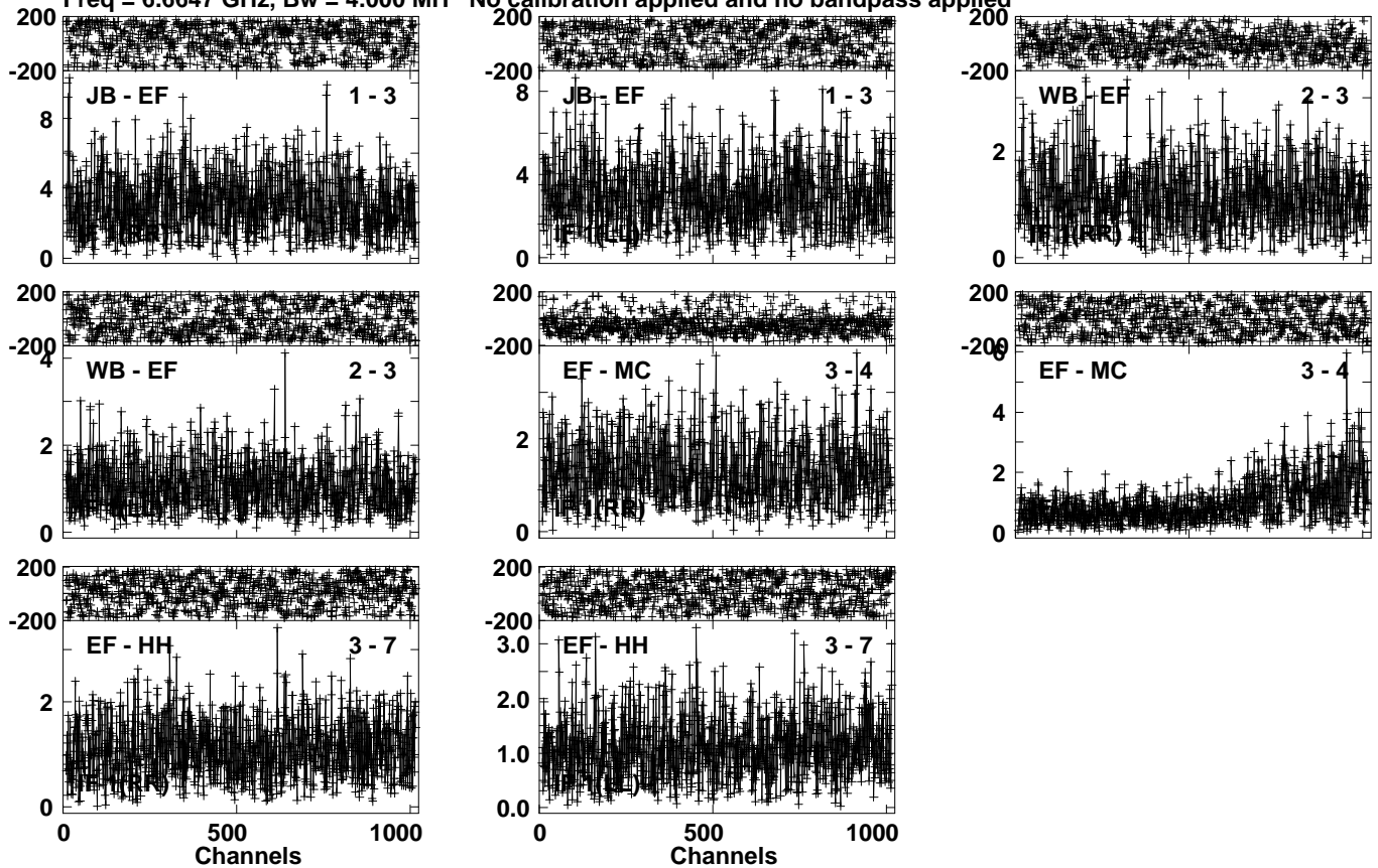
Lower frame: Milli Ampl Jy Top frame: Phas deg Vector averaged cross-power spectrum Several baselines displayed Timerange: 00/18:17:21 to 00/18:19:20
