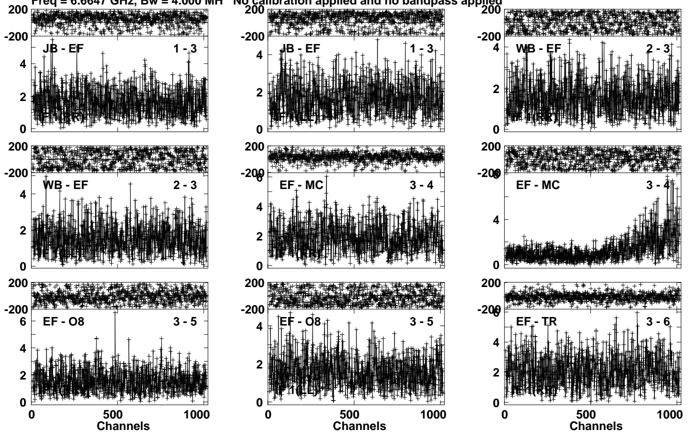
Lower frame: Milli Ampl Jy Top frame: Phas deg Vector averaged cross-power spectrum Several baselines displayed Timerange: 00/14:17:04 to 00/14:18:59
