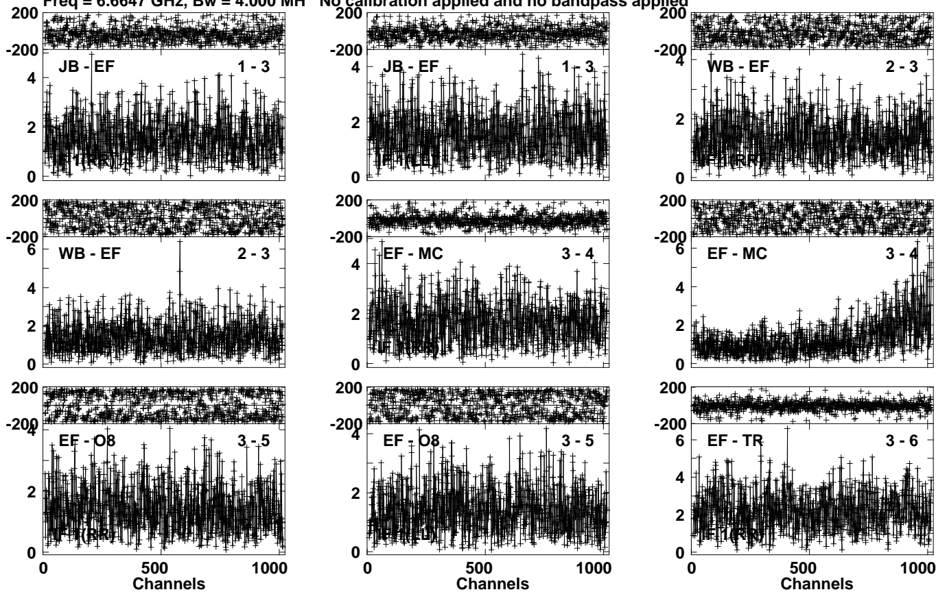
Lower frame: Milli Ampl Jy Top frame: Phas deg Vector averaged cross-power spectrum Several baselines displayed Timerange: 00/17:10:24 to 00/17:12:20
