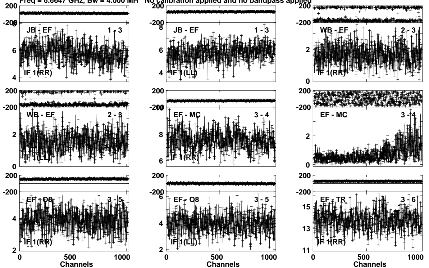
Lower frame: Milli Ampl Jy Top frame: Phas deg Vector averaged cross-power spectrum Several baselines displayed Timerange: 00/11:32:21 to 00/11:36:20
