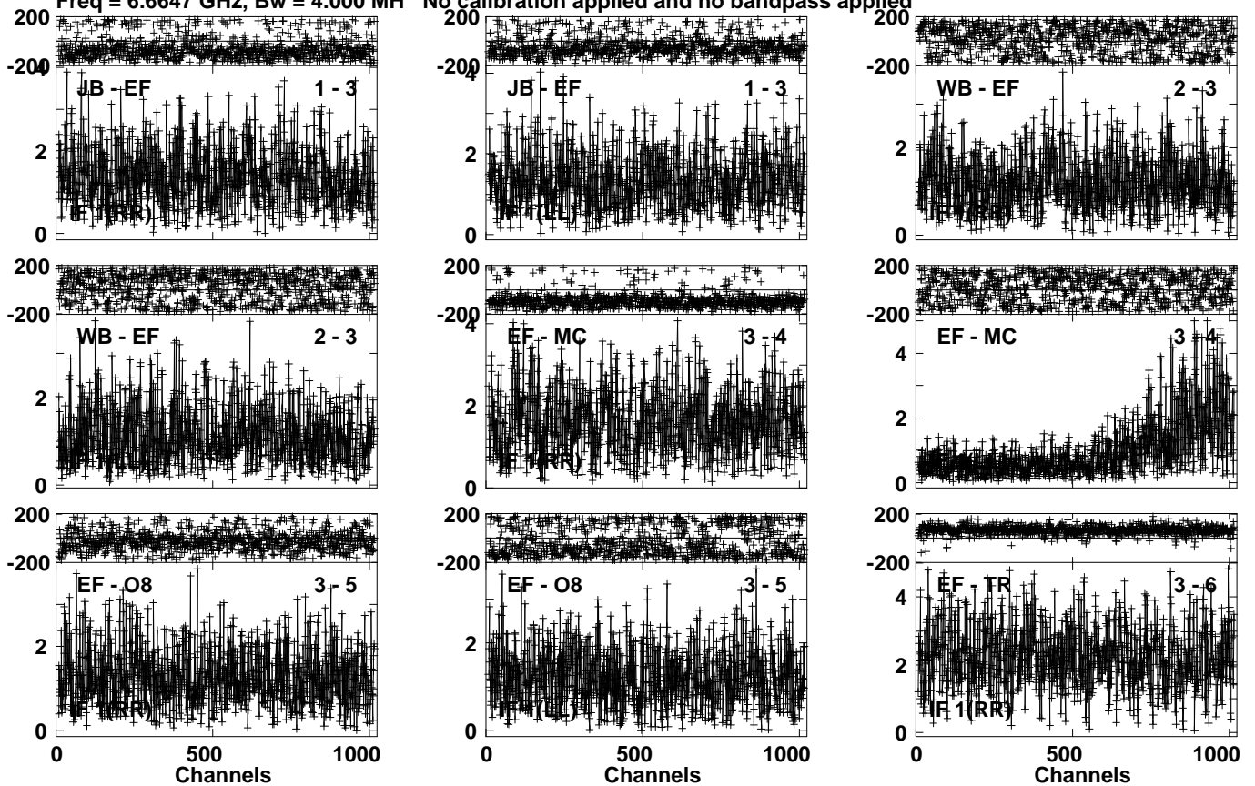
Lower frame: Milli Ampl Jy Top frame: Phas deg Vector averaged cross-power spectrum Several baselines displayed Timerange: 00/11:58:40 to 00/12:00:39
