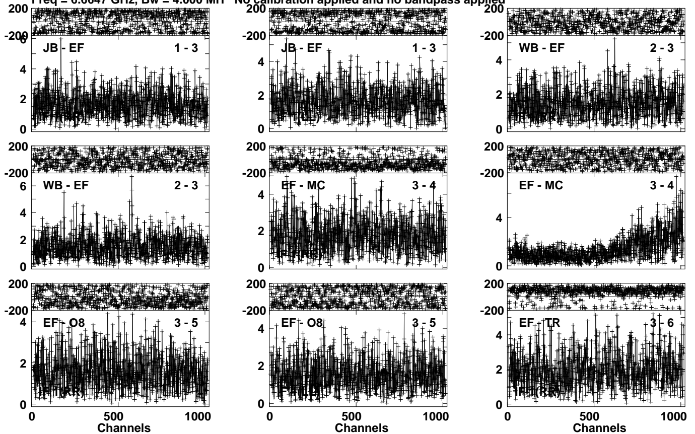
Lower frame: Milli Ampl Jy Top frame: Phas deg Vector averaged cross-power spectrum Several baselines displayed Timerange: 00/13:55:44 to 00/13:57:39
