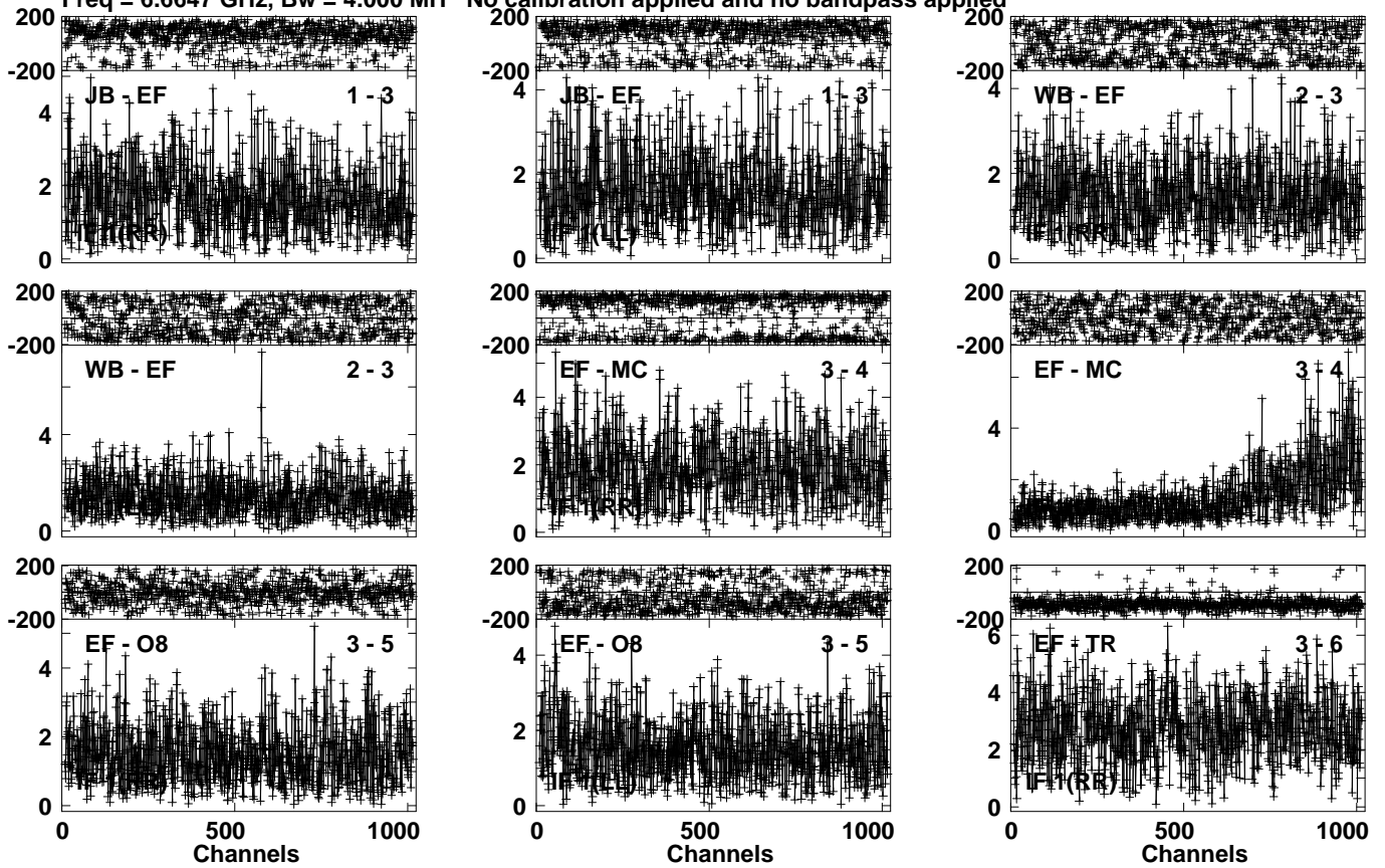
Lower frame: Milli Ampl Jy Top frame: Phas deg Vector averaged cross-power spectrum Several baselines displayed Timerange: 00/12:14:22 to 00/12:16:19
