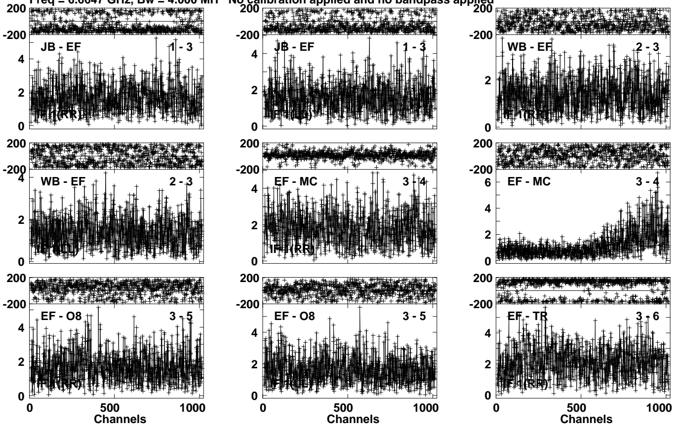
Lower frame: Milli Ampl Jy Top frame: Phas deg Vector averaged cross-power spectrum Several baselines displayed Timerange: 00/15:47:42 to 00/15:49:40
