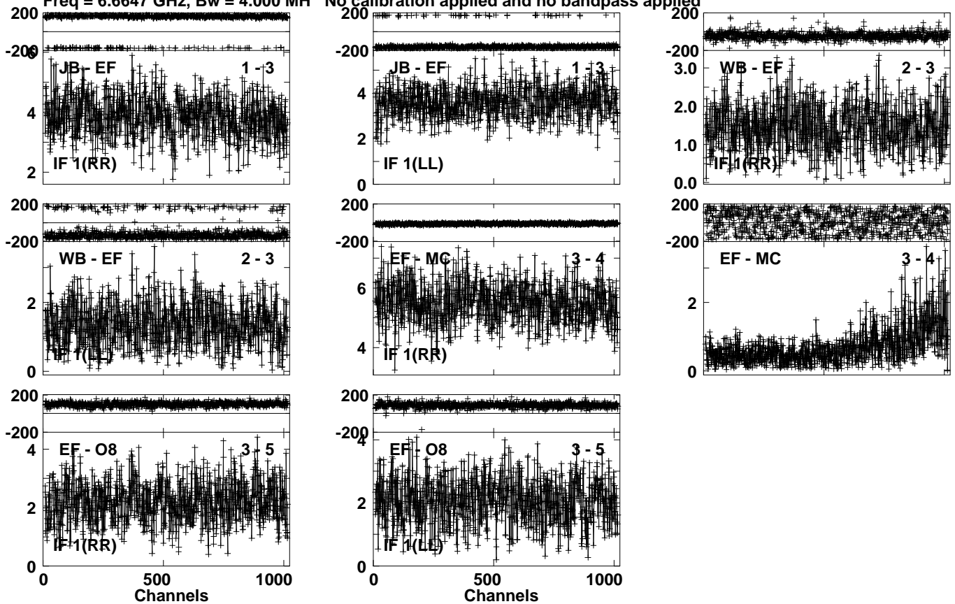
Lower frame: Milli Ampl Jy Top frame: Phas deg Vector averaged cross-power spectrum Several baselines displayed Timerange: 00/17:40:21 to 00/17:44:19
