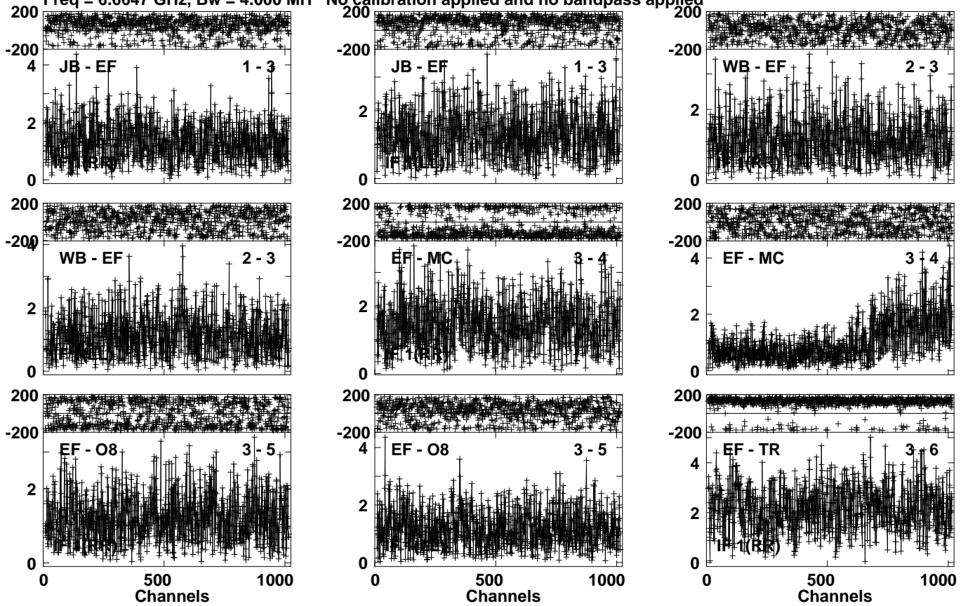
Lower frame: Milli Ampl Jy Top frame: Phas deg Vector averaged cross-power spectrum Several baselines displayed Timerange: 00/11:29:20 to 00/11:31:19
