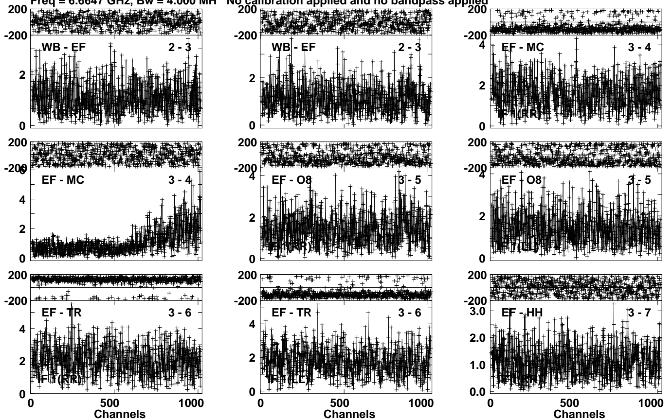
Lower frame: Milli Ampl Jy Top frame: Phas deg Vector averaged cross-power spectrum Several baselines displayed Timerange: 00/16:36:01 to 00/16:37:59
