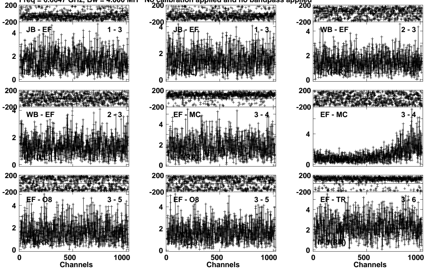
Lower frame: Milli Ampl Jy Top frame: Phas deg Vector averaged cross-power spectrum Several baselines displayed Timerange: 00/16:19:42 to 00/16:21:40
