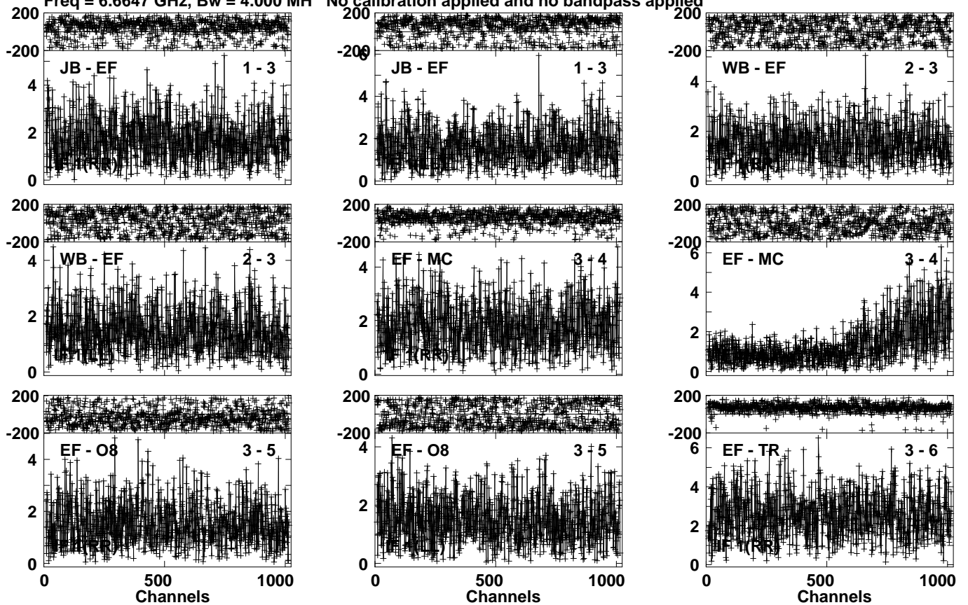
Lower frame: Milli Ampl Jy Top frame: Phas deg Vector averaged cross-power spectrum Several baselines displayed Timerange: 00/13:05:04 to 00/13:06:59
