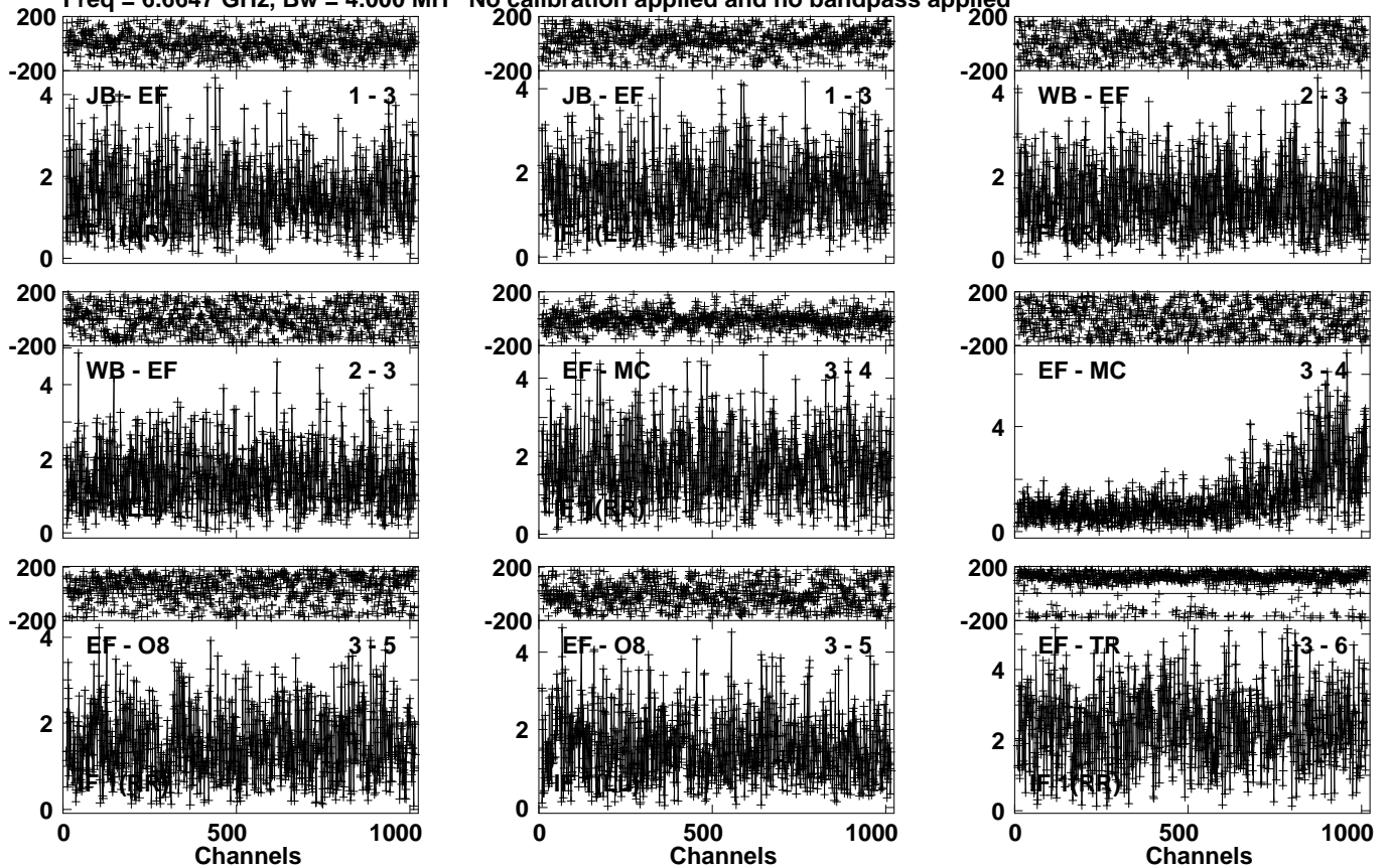
Lower frame: Milli Ampl Jy Top frame: Phas deg Vector averaged cross-power spectrum Several baselines displayed Timerange: 00/11:02:22 to 00/11:04:19
