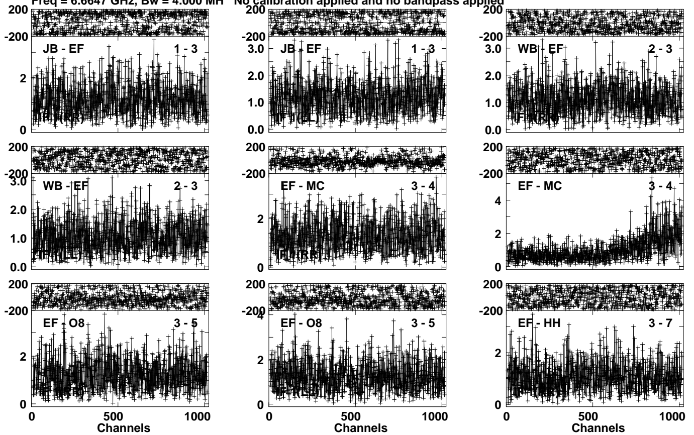
Lower frame: Milli Ampl Jy Top frame: Phas deg Vector averaged cross-power spectrum Several baselines displayed Timerange: 00/18:06:40 to 00/18:08:40
