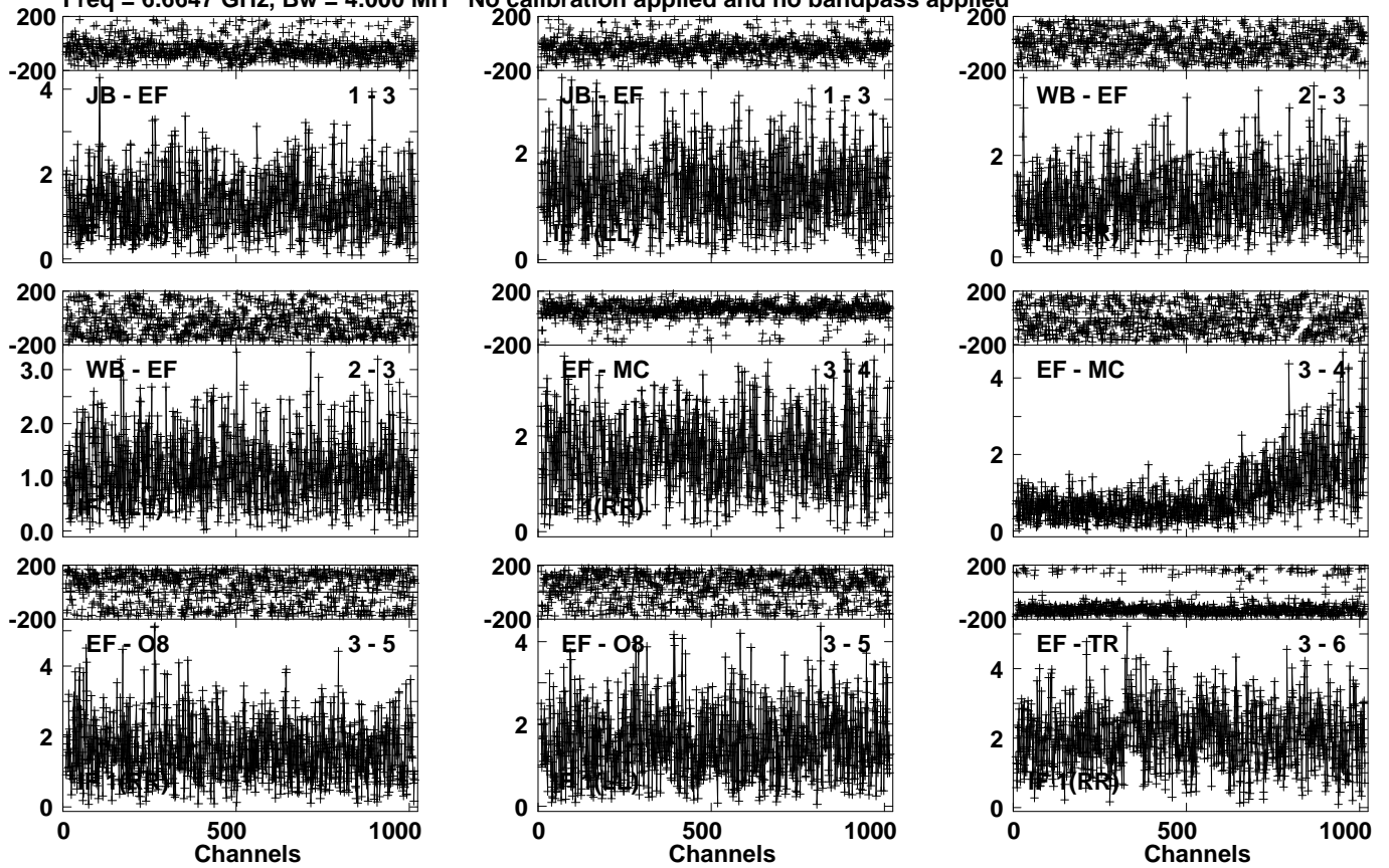
Lower frame: Milli Ampl Jy Top frame: Phas deg Vector averaged cross-power spectrum Several baselines displayed Timerange: 00/17:16:01 to 00/17:18:00
