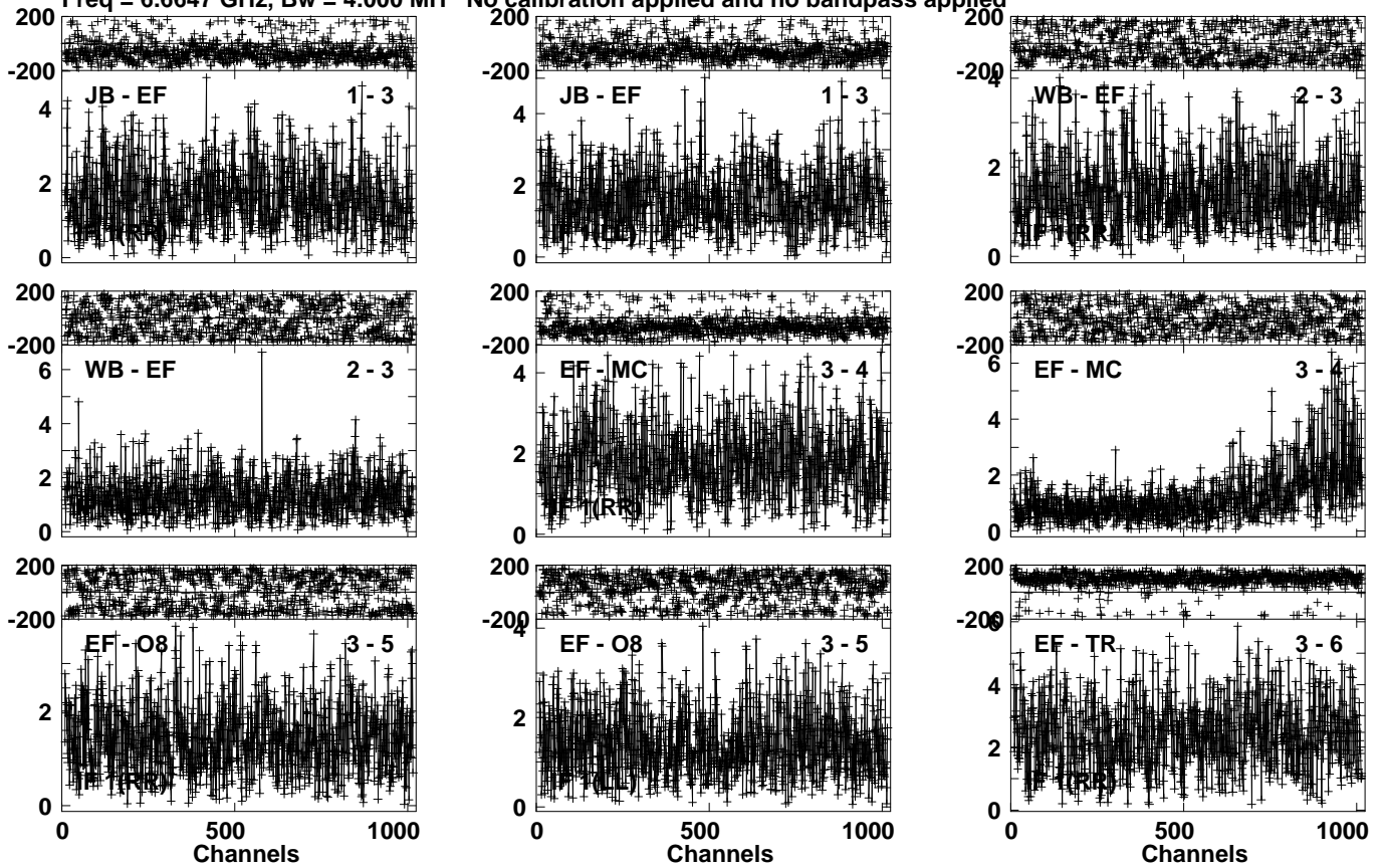
Lower frame: Milli Ampl Jy Top frame: Phas deg Vector averaged cross-power spectrum Several baselines displayed Timerange: 00/15:18:22 to 00/15:20:20
