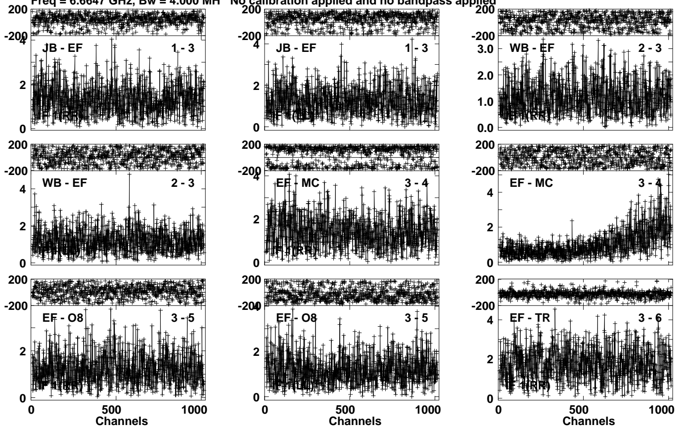
Lower frame: Milli Ampl Jy Top frame: Phas deg Vector averaged cross-power spectrum Several baselines displayed Timerange: 00/13:10:40 to 00/13:12:39
