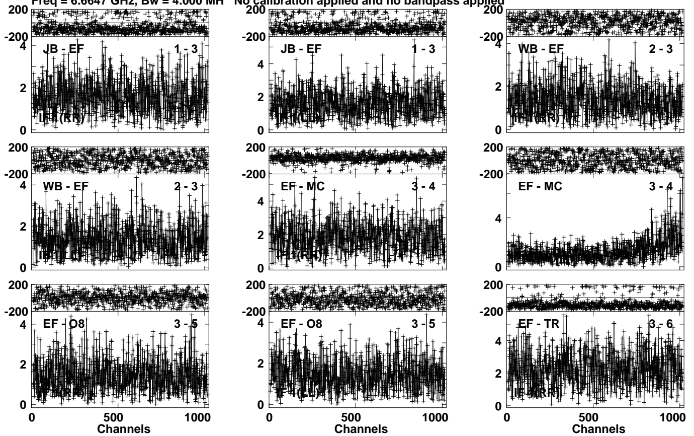
Lower frame: Milli Ampl Jy Top frame: Phas deg Vector averaged cross-power spectrum Several baselines displayed Timerange: 00/15:07:44 to 00/15:09:40
