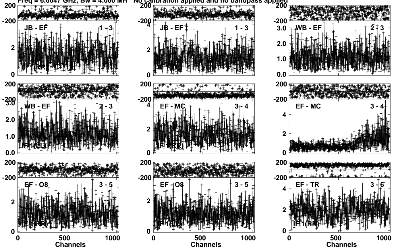
Lower frame: Milli Ampl Jy Top frame: Phas deg Vector averaged cross-power spectrum Several baselines displayed Timerange: 00/15:34:41 to 00/15:36:40
