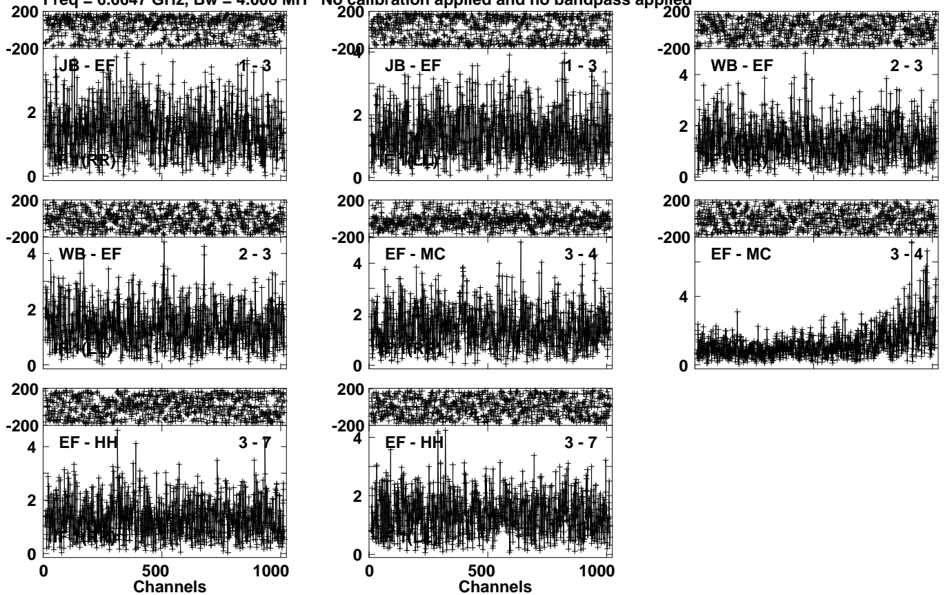
Lower frame: Milli Ampl Jy Top frame: Phas deg Vector averaged cross-power spectrum Several baselines displayed Timerange: 00/18:22:26 to 00/18:24:20
