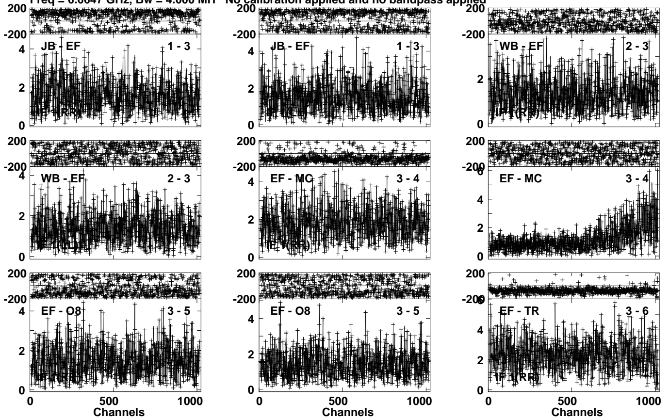
Lower frame: Milli Ampl Jy Top frame: Phas deg Vector averaged cross-power spectrum Several baselines displayed Timerange: 00/16:49:02 to 00/16:51:00
