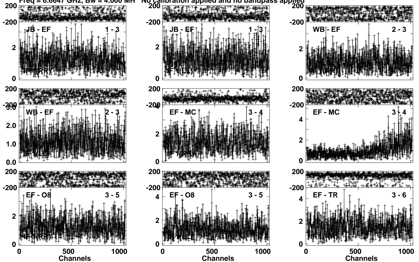
Lower frame: Milli Ampl Jy Top frame: Phas deg Vector averaged cross-power spectrum Several baselines displayed Timerange: 00/17:56:00 to 00/17:58:00
