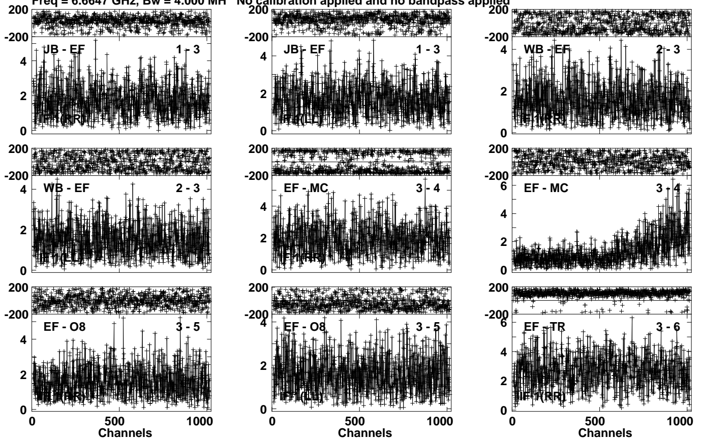
Lower frame: Milli Ampl Jy Top frame: Phas deg Vector averaged cross-power spectrum Several baselines displayed Timerange: 00/13:26:24 to 00/13:28:19
