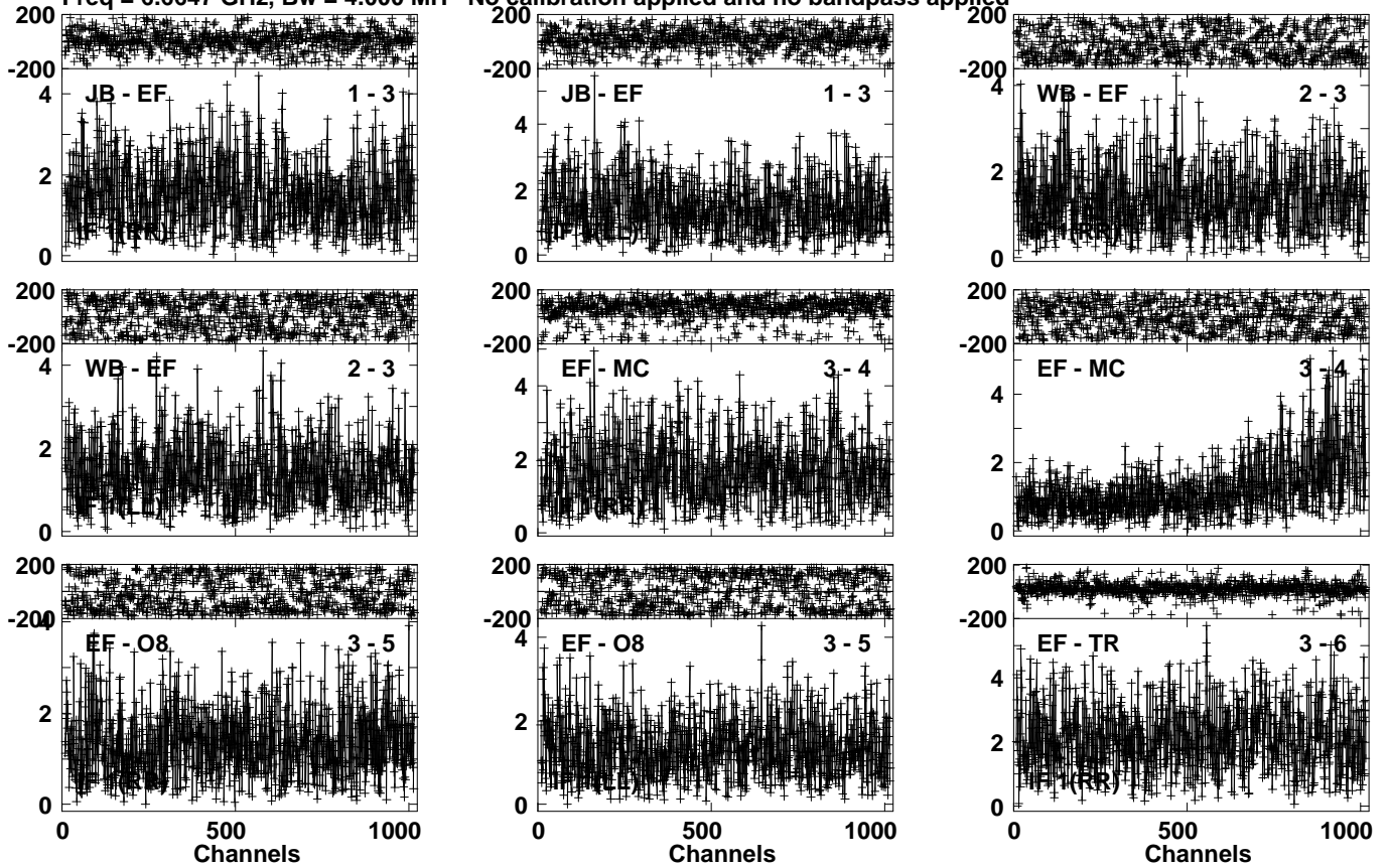
Lower frame: Milli Ampl Jy Top frame: Phas deg Vector averaged cross-power spectrum Several baselines displayed Timerange: 00/16:59:42 to 00/17:01:39
