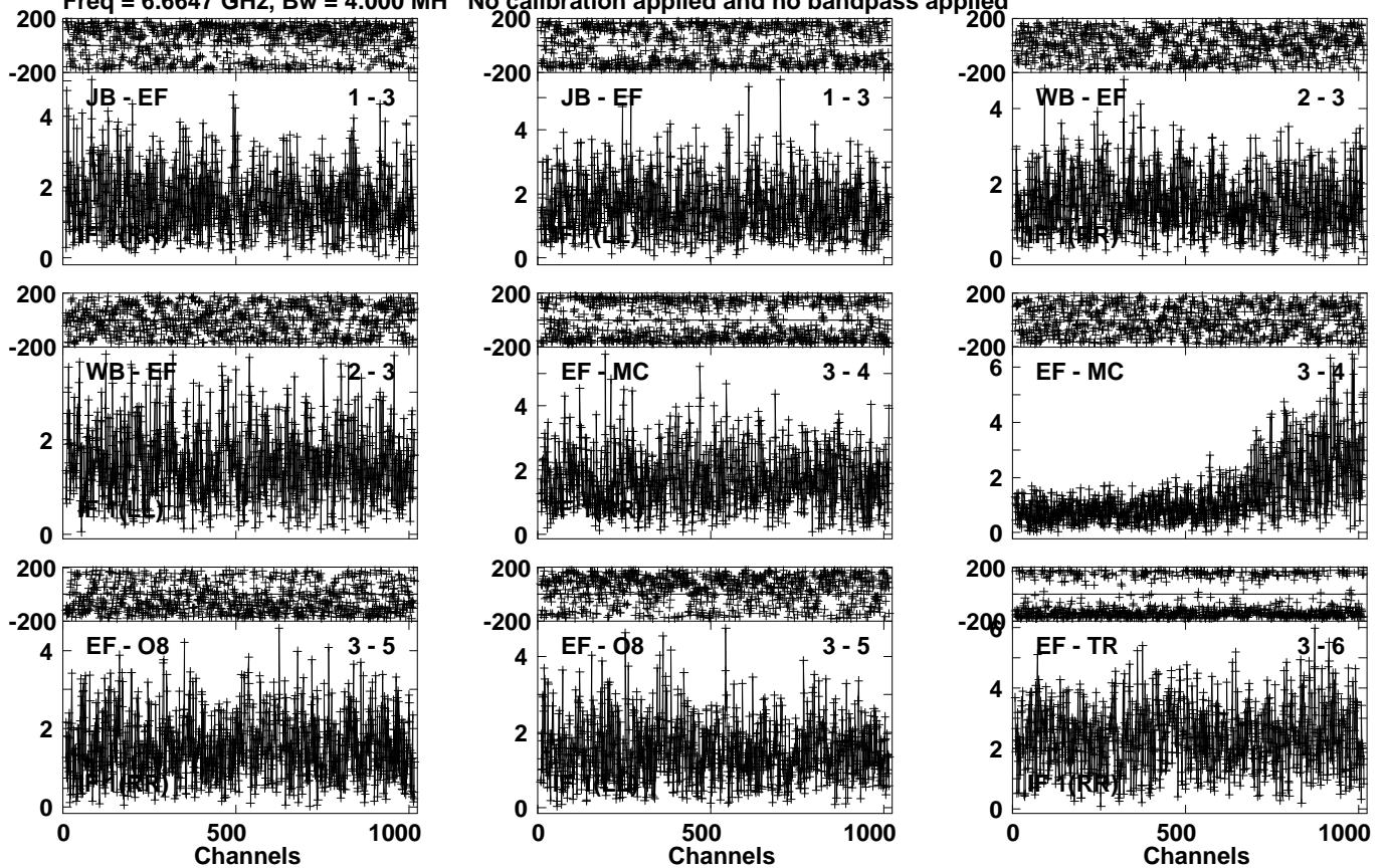
Lower frame: Milli Ampl Jy Top frame: Phas deg Vector averaged cross-power spectrum Several baselines displayed Timerange: 00/11:13:03 to 00/11:14:59
