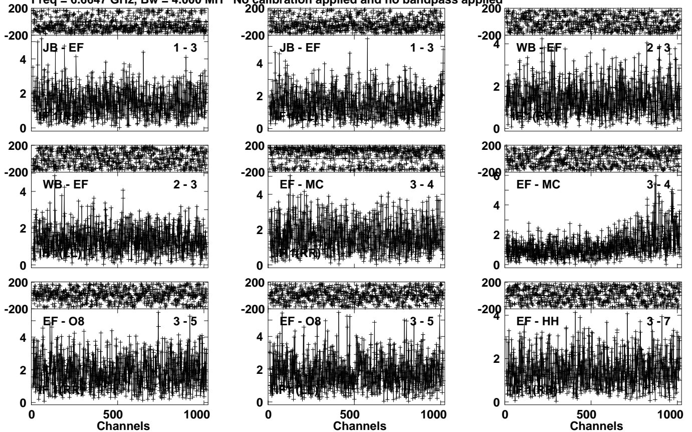
Lower frame: Milli Ampl Jy Top frame: Phas deg Vector averaged cross-power spectrum Several baselines displayed Timerange: 00/18:01:07 to 00/18:02:59
