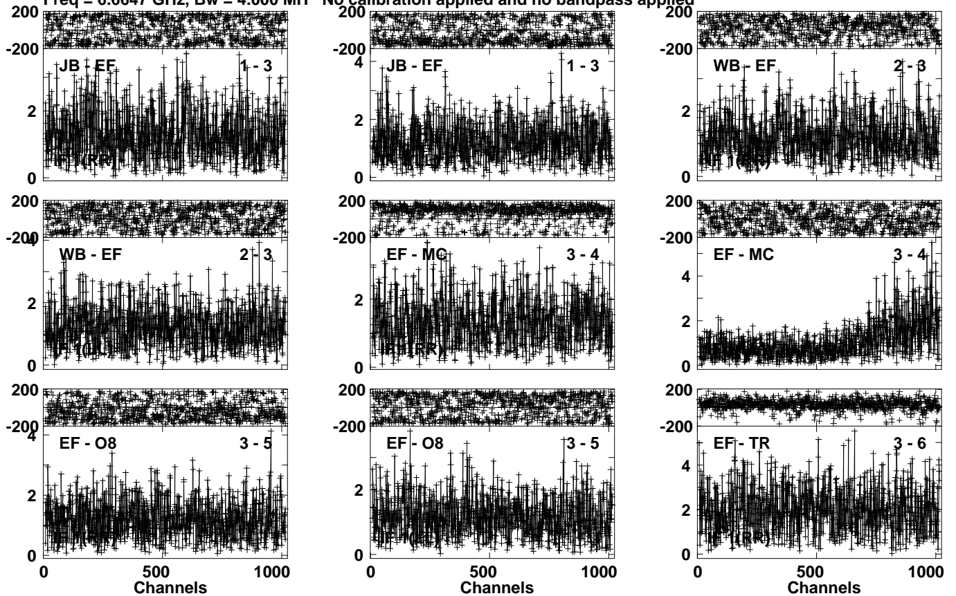
Lower frame: Milli Ampl Jy Top frame: Phas deg Vector averaged cross-power spectrum Several baselines displayed Timerange: 00/10:41:00 to 00/10:43:00
