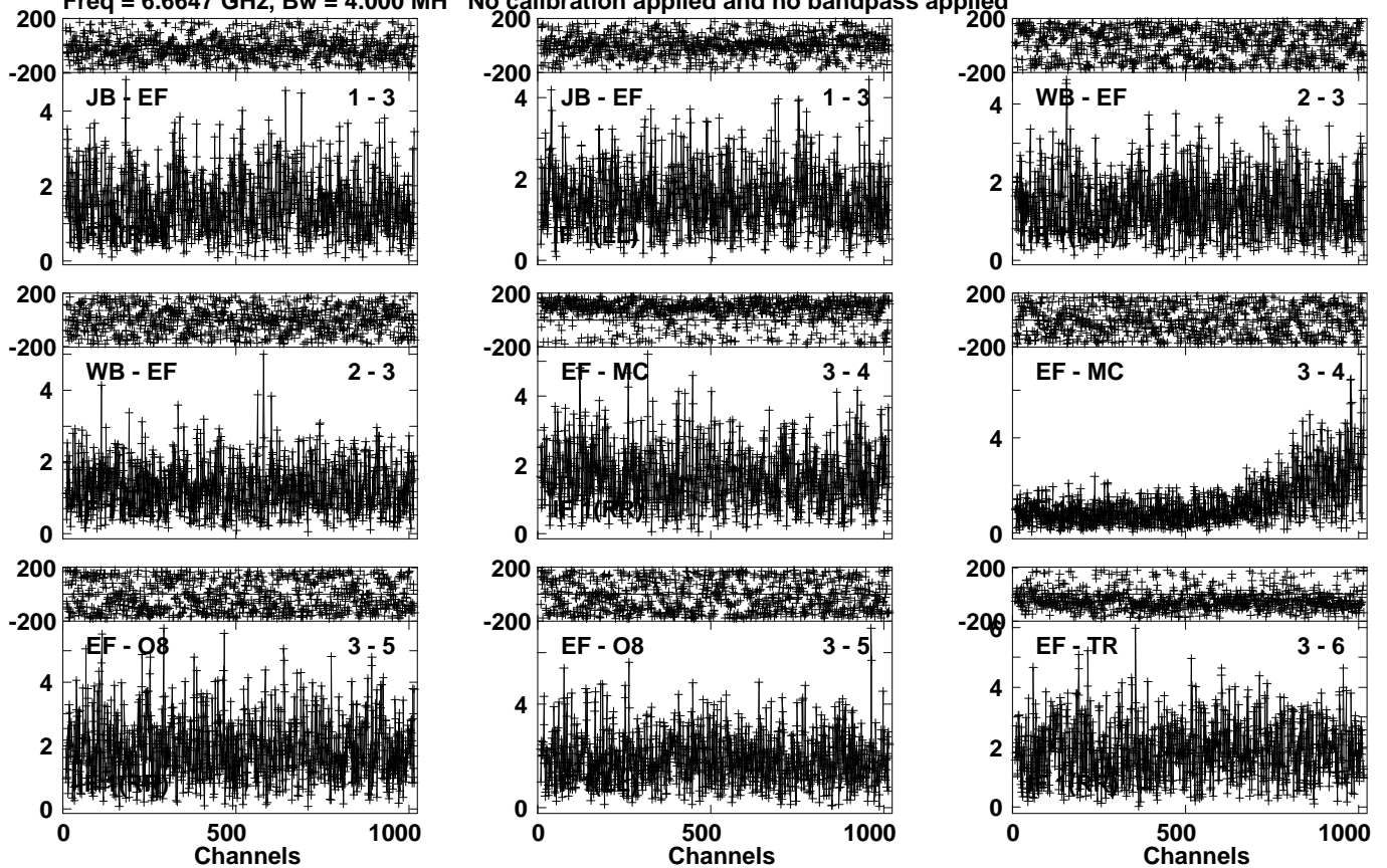
Lower frame: Milli Ampl Jy Top frame: Phas deg Vector averaged cross-power spectrum Several baselines displayed Timerange: 00/17:50:26 to 00/17:52:20
