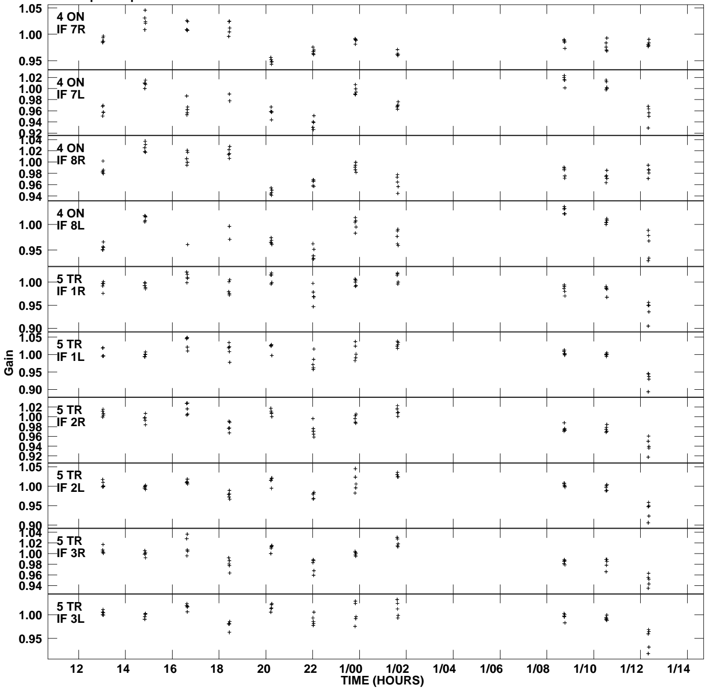
Plot file version 7 created 01-MAY-2014 01:15:08 Gain amp vs UTC time for J0749+7420.MULTI.1 SN 4 Rpol & Lpol IF 1 - 8
