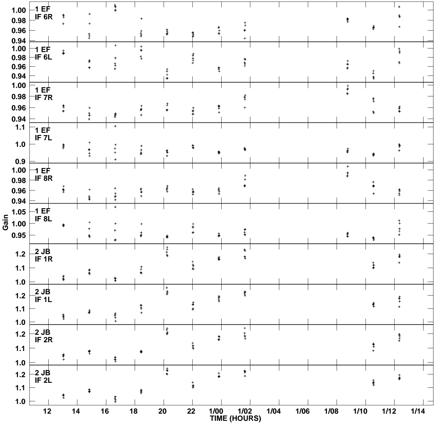
Plot file version 2 created 01-MAY-2014 01:15:08 Gain amp vs UTC time for J0749+7420.MULTI.1 SN 4 Rpol & Lpol IF 1 - 8
