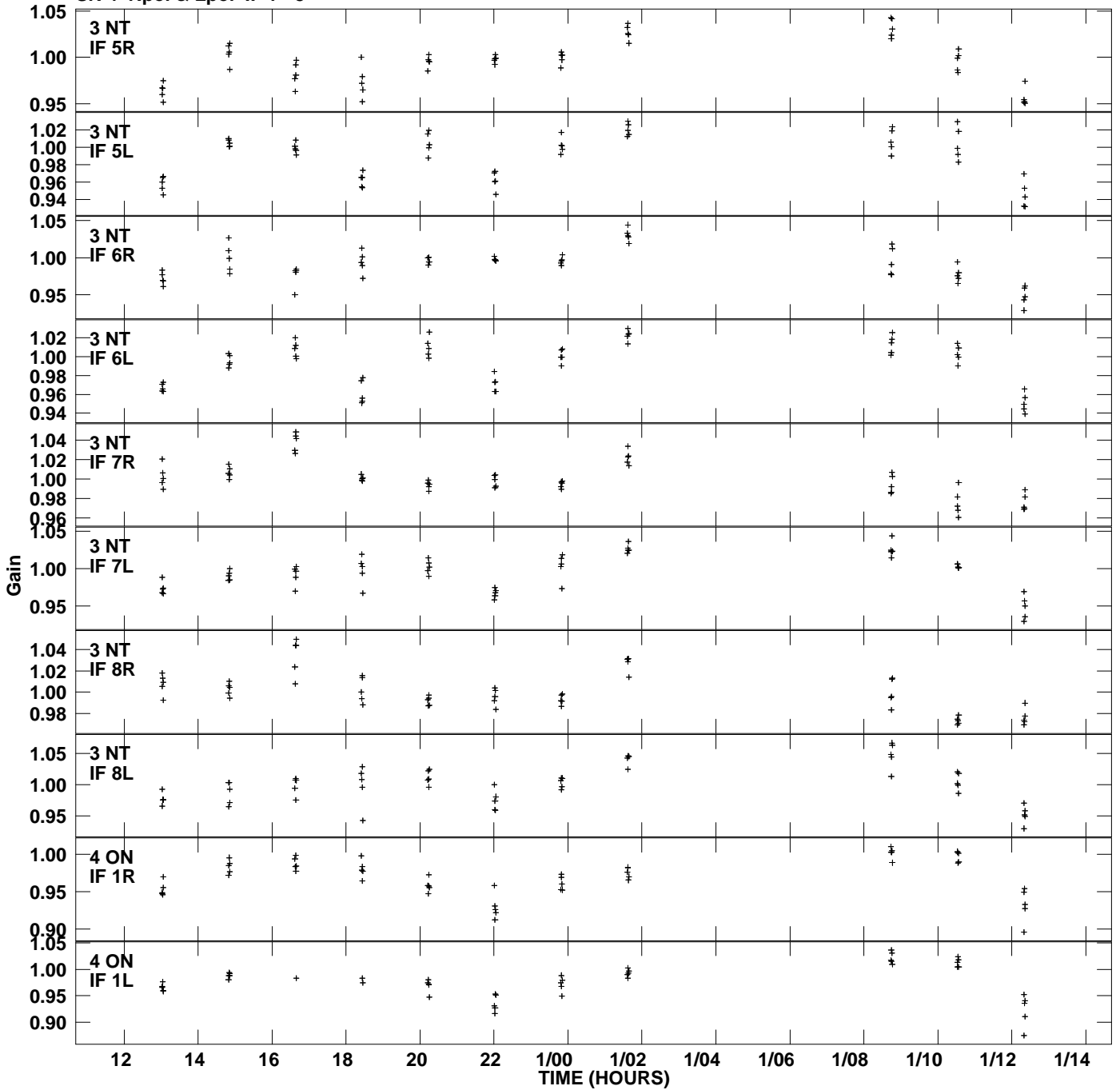
Plot file version 5 created 01-MAY-2014 01:15:08 Gain amp vs UTC time for J0749+7420.MULTI.1 SN 4 Rpol & Lpol IF 1 - 8
