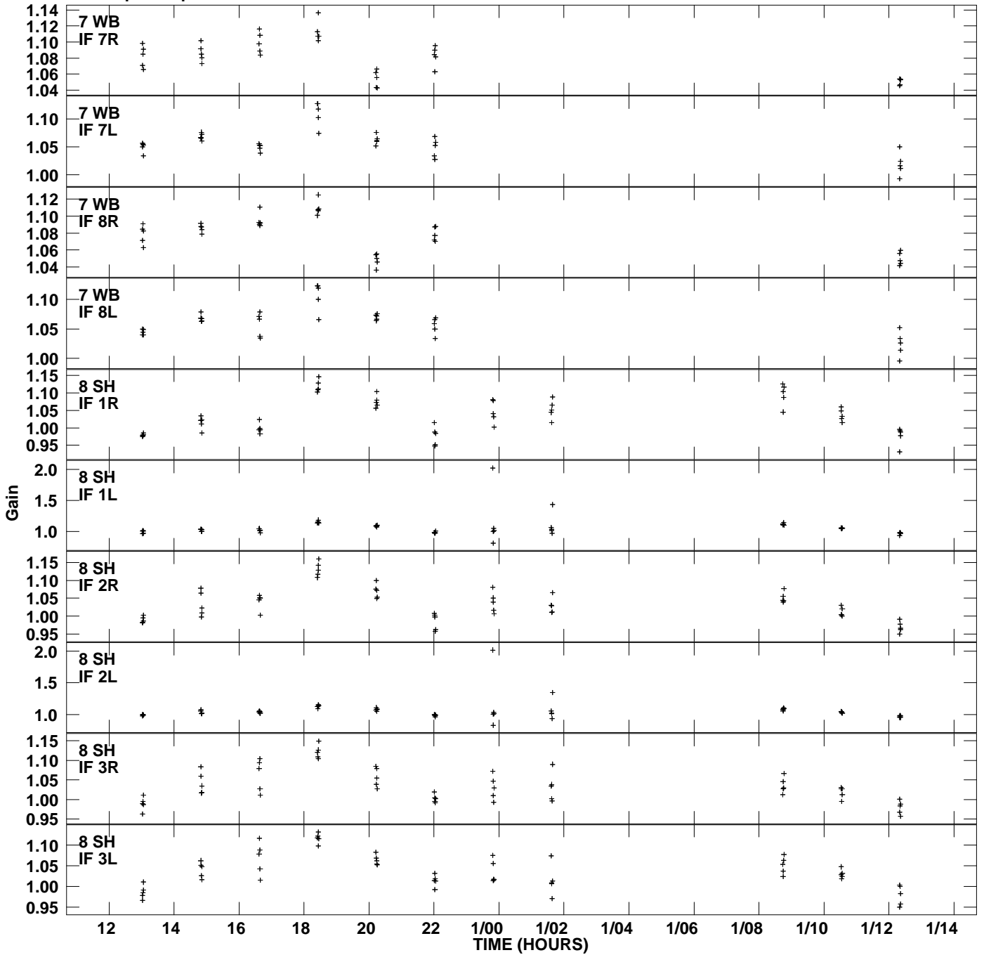
Plot file version 10 created 01-MAY-2014 01:15:08 Gain amp vs UTC time for J0749+7420.MULTI.1 SN 4 Rpol & Lpol IF 1 - 8
