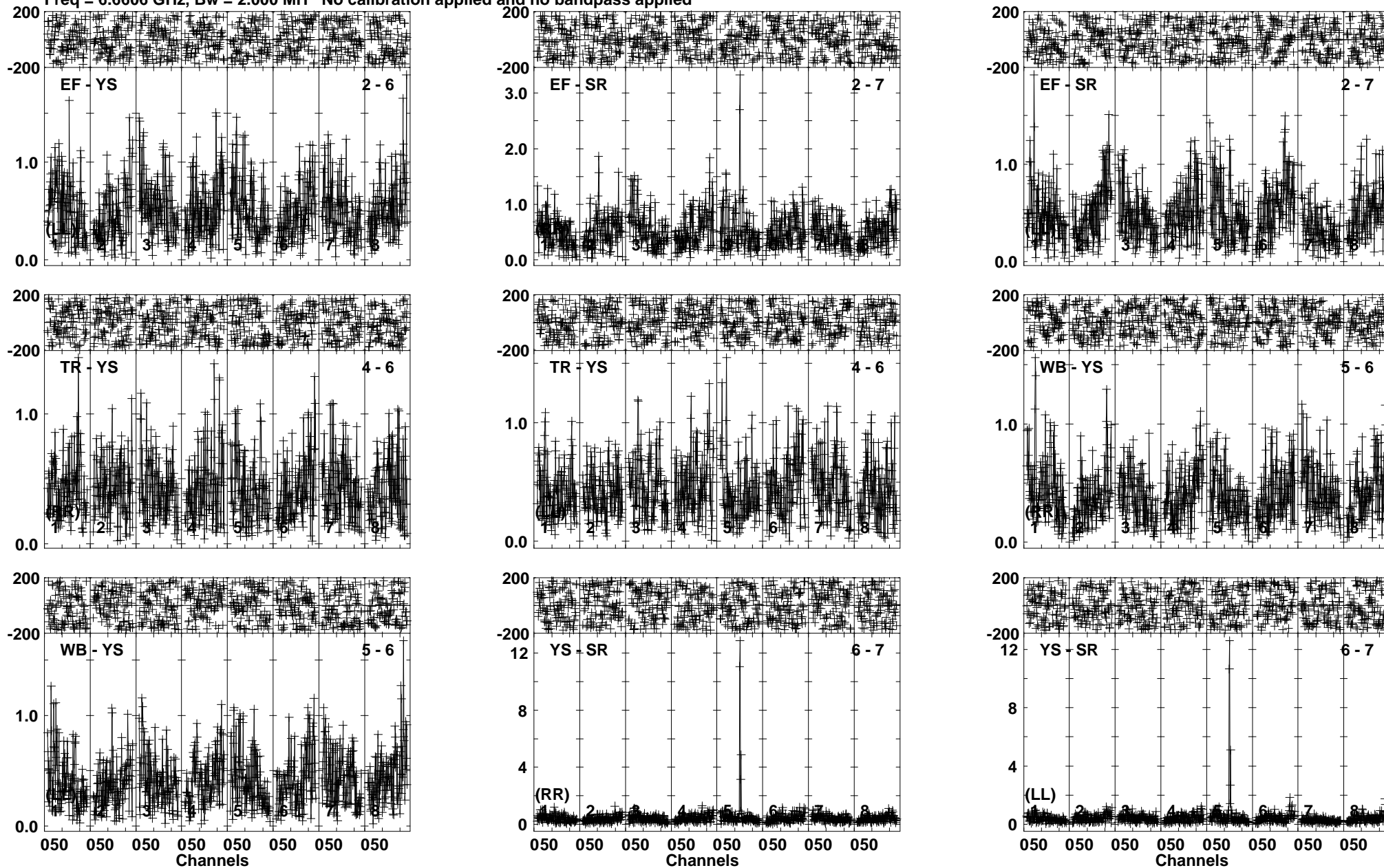
Lower frame: Milli Ampl Jy Top frame: Phas deg Vector averaged cross-power spectrum Baseline: EF (02) - YS (06) Timerange: 00/15:14:30 to 00/15:17:45
