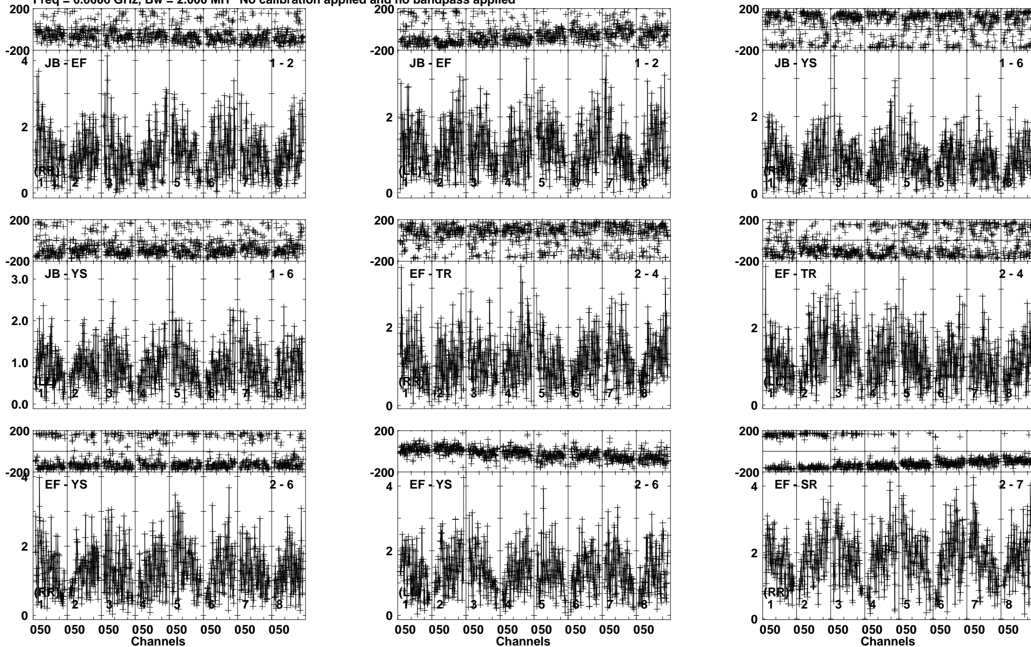
Lower frame: Milli Ampl Jy Top frame: Phas deg Vector averaged cross-power spectrum Baseline: JB (01) - EF (02) Timerange: 00/17:35:15 to 00/17:36:59
