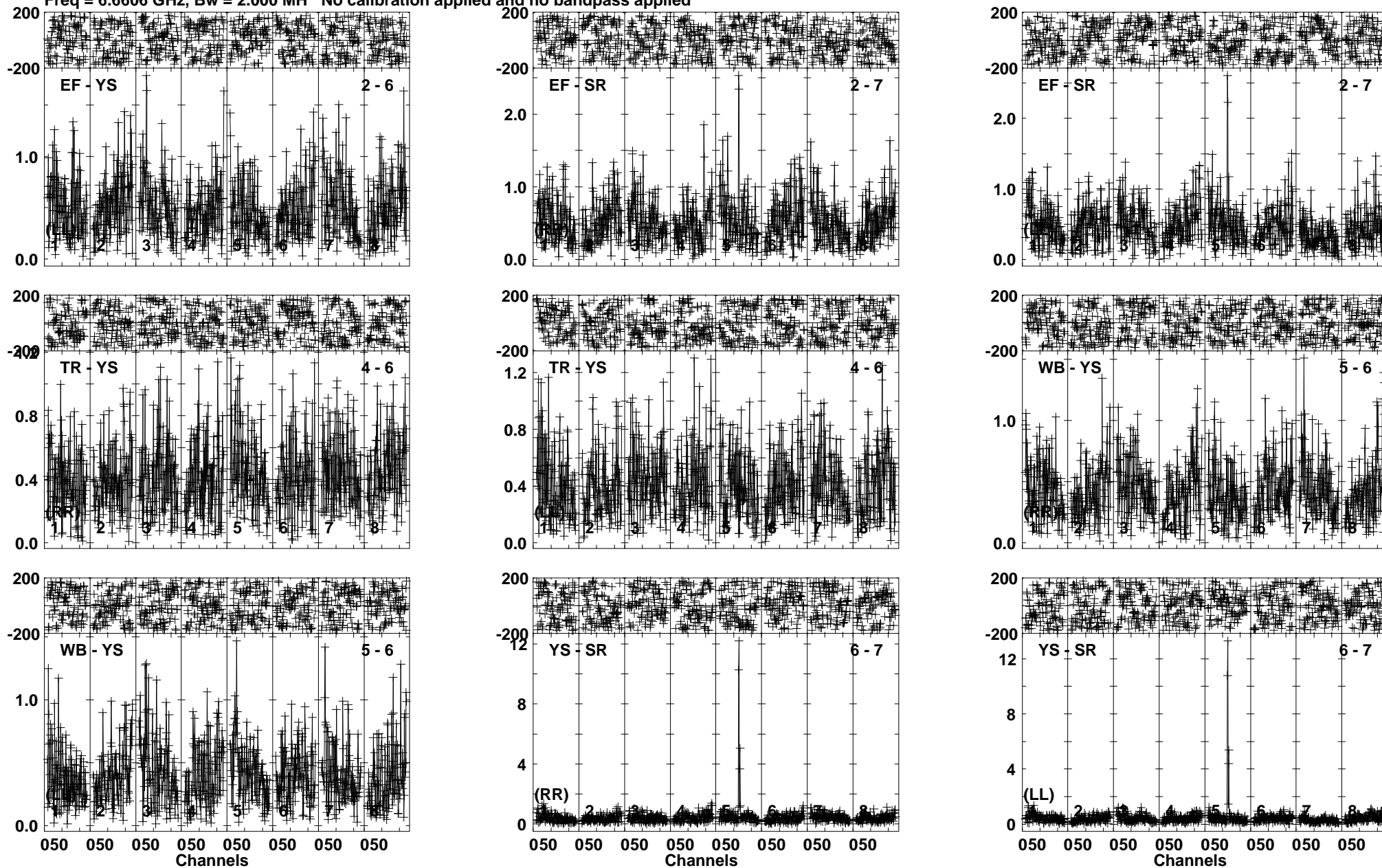
Lower frame: Milli Ampl Jy Top frame: Phas deg Vector averaged cross-power spectrum Baseline: EF (02) - YS (06) Timerange: 00/15:20:01 to 00/15:23:15
