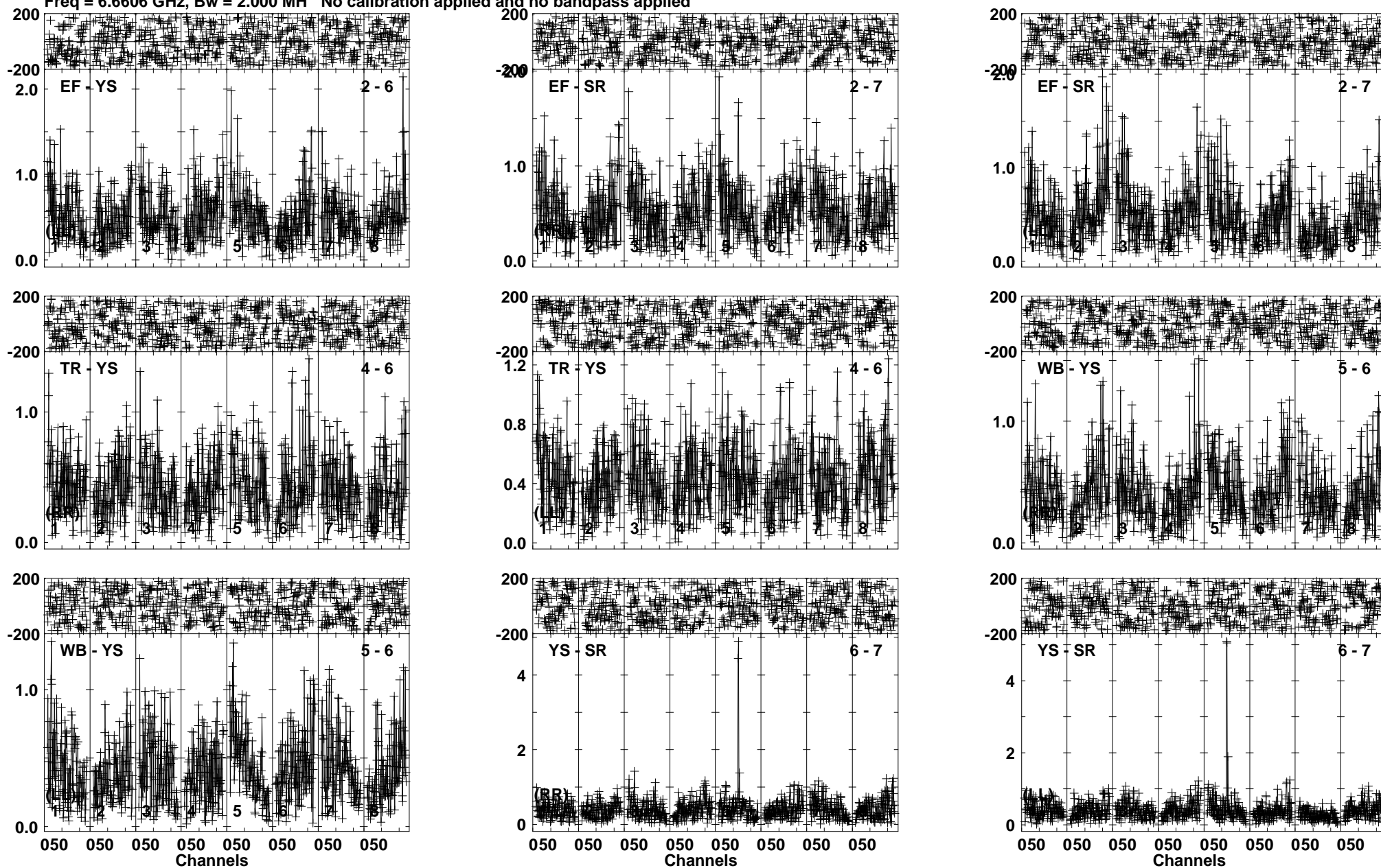
Lower frame: Milli Ampl Jy Top frame: Phas deg Vector averaged cross-power spectrum Baseline: EF (02) - YS (06) Timerange: 00/14:06:46 to 00/14:10:00
