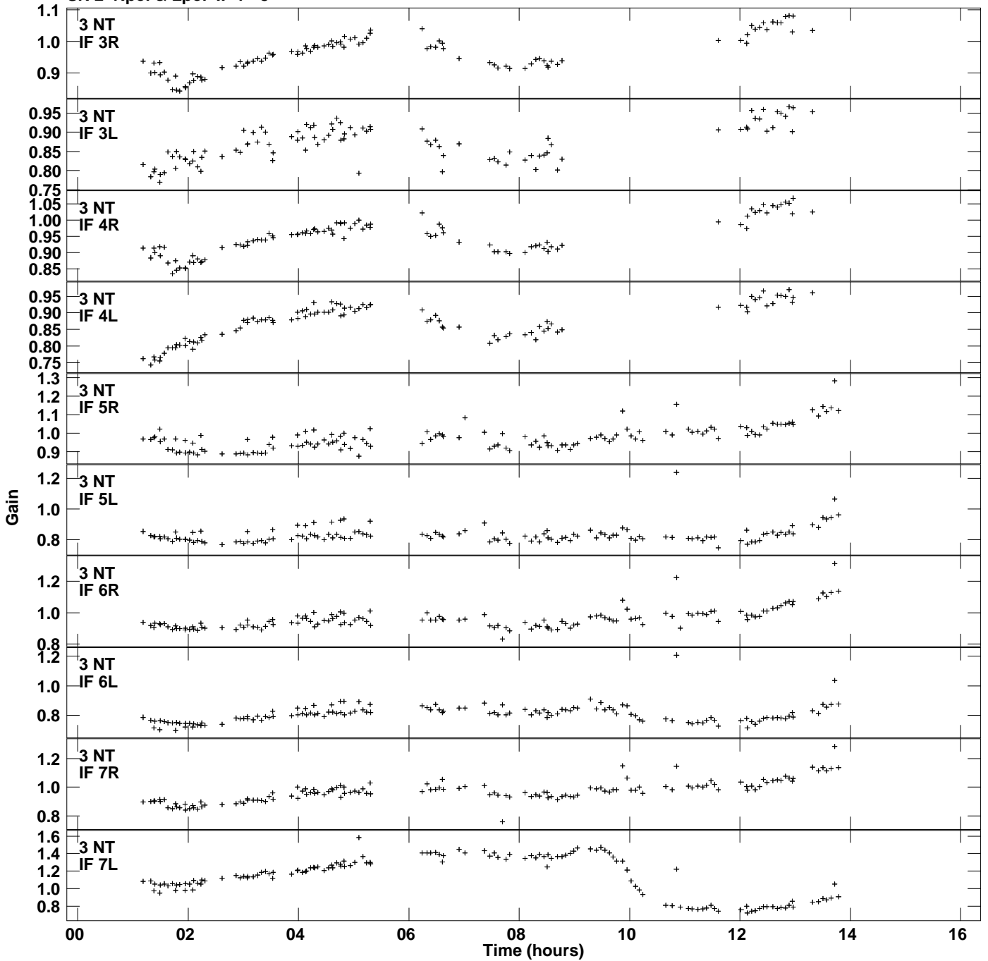
Plot file version 3 created 20-APR-2017 11:10:58 Gain amp vs UTC time for J2007+4029.MULTI.1 SN 2 Rpol & Lpol IF 1 - 8
