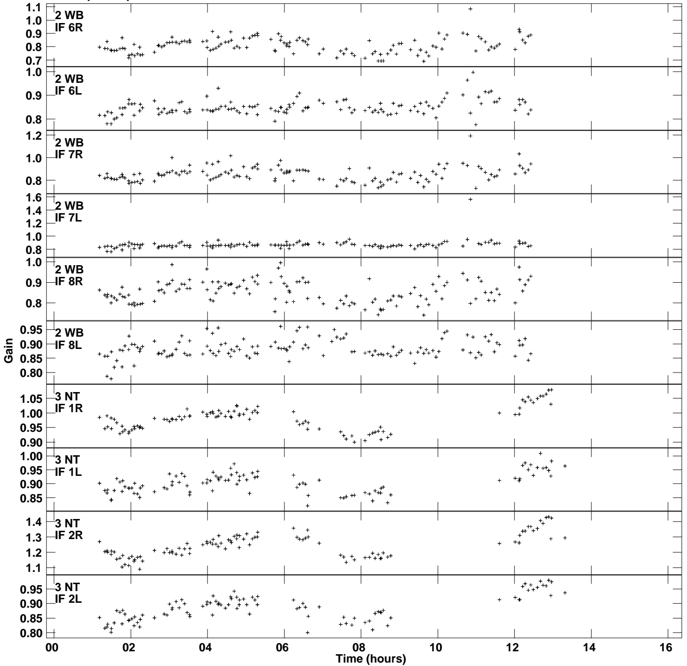
Plot file version 2 created 20-APR-2017 11:10:58 Gain amp vs UTC time for J2007+4029.MULTI.1 SN 2 Rpol & Lpol IF 1 - 8
