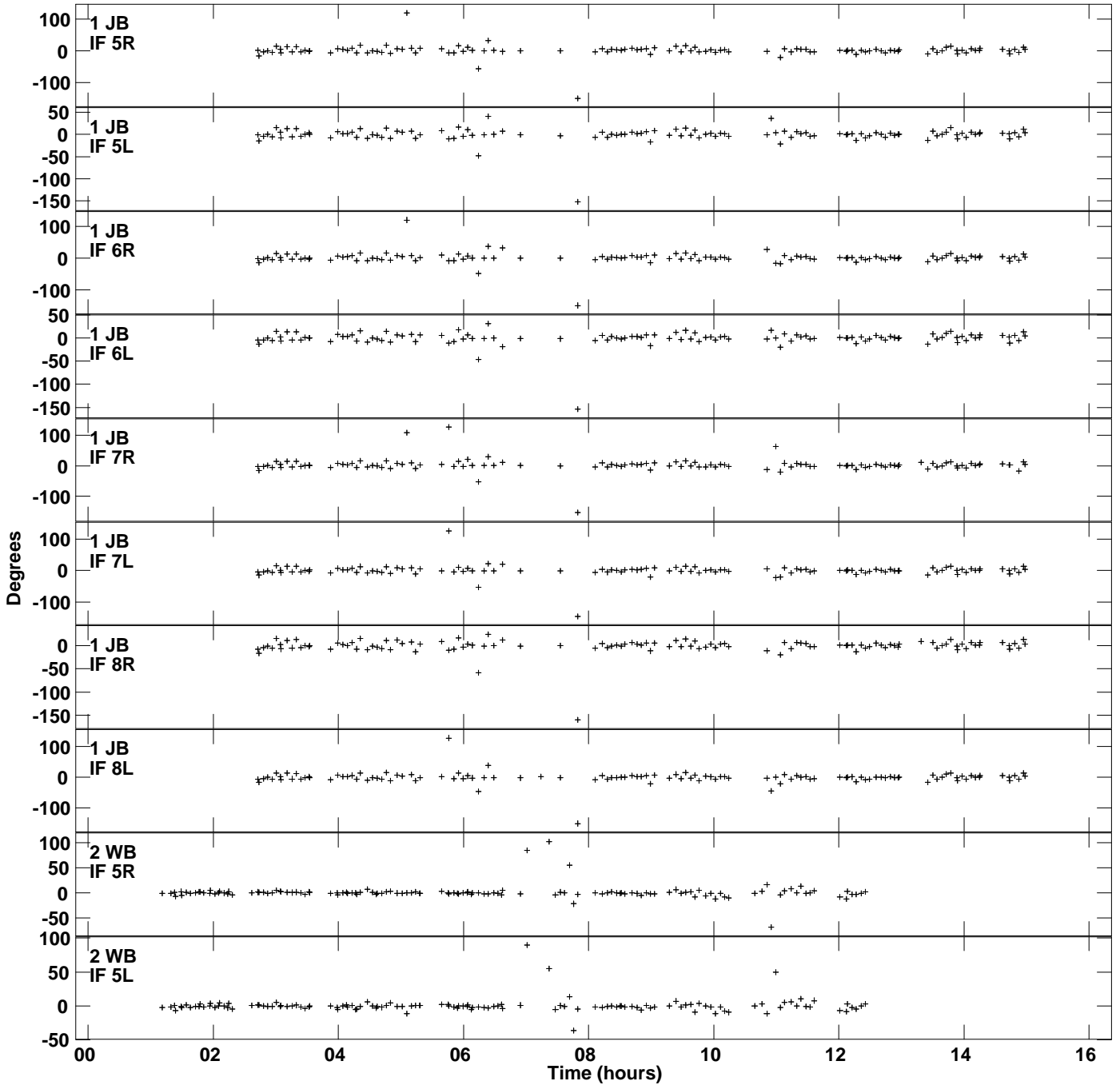
Plot file version 1 created 20-APR-2017 11:10:42 Gain phs vs UTC time for J2007+4029.MULTI.1 SN 1 Rpol & Lpol IF 1 - 8
