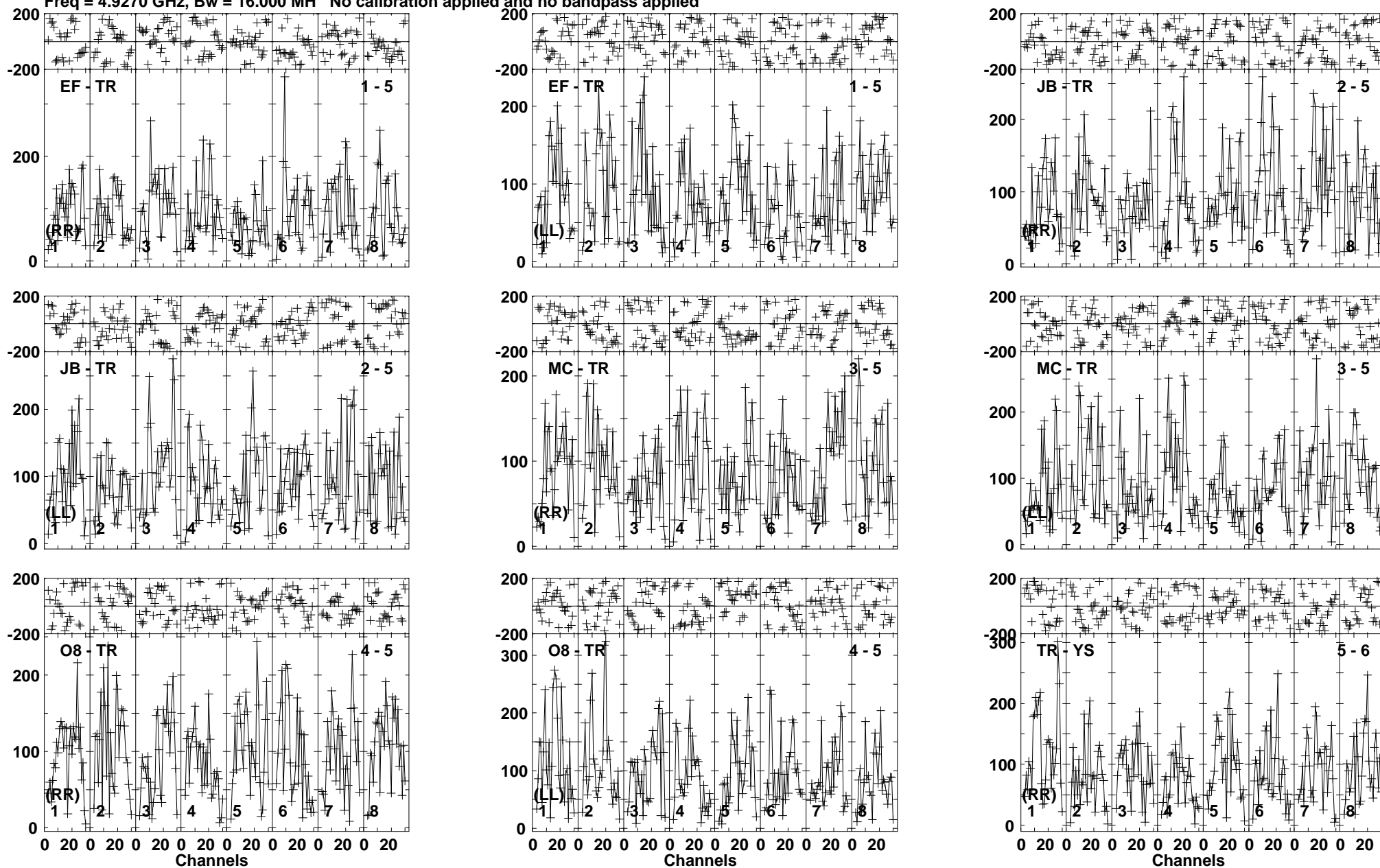
Lower frame: Micro Ampl Jy Top frame: Phas deg Vector averaged cross-power spectrum Baseline: EF (01) - TR (05) Timerange: 00/06:17:21 to 00/06:20:49
