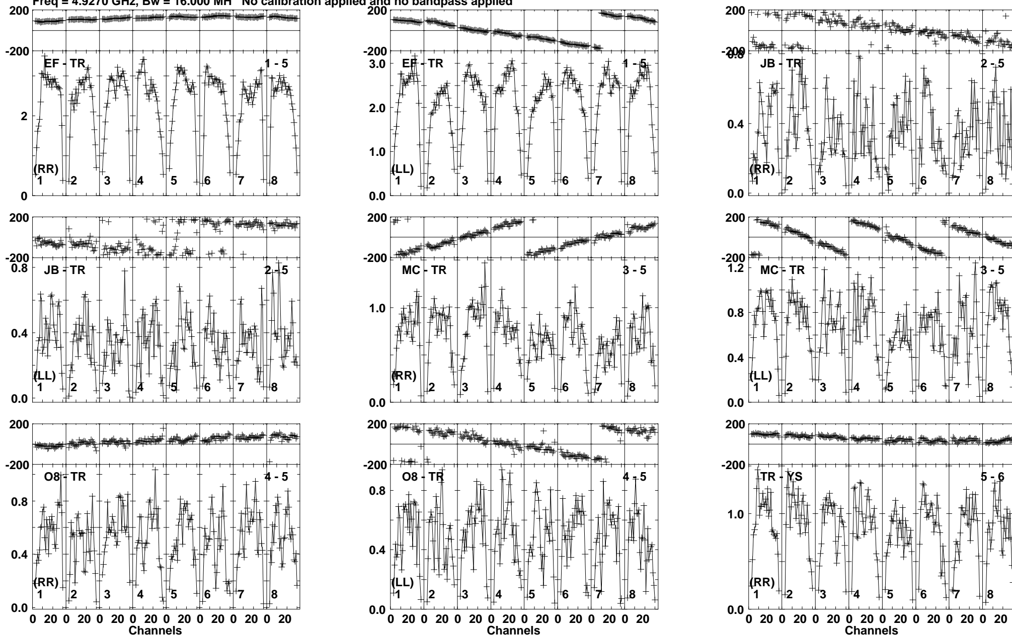
Lower frame: Milli Ampl Jy Top frame: Phas deg Vector averaged cross-power spectrum Baseline: EF (01) - TR (05) Timerange: 00/09:16:51 to 00/09:18:19
