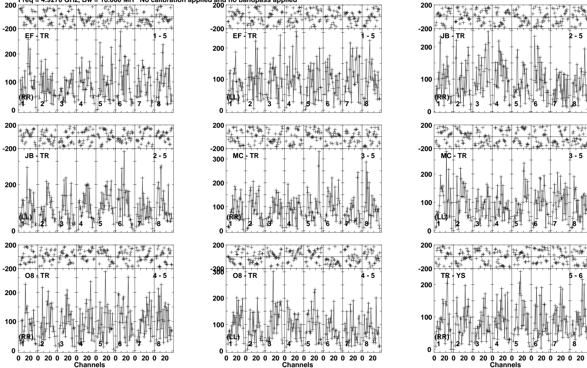
Lower frame: Micro Ampl Jy Top frame: Phas deg Vector averaged cross-power spectrum Baseline: EF (01) - TR (05) Timerange: 00/09:58:21 to 00/10:01:49
