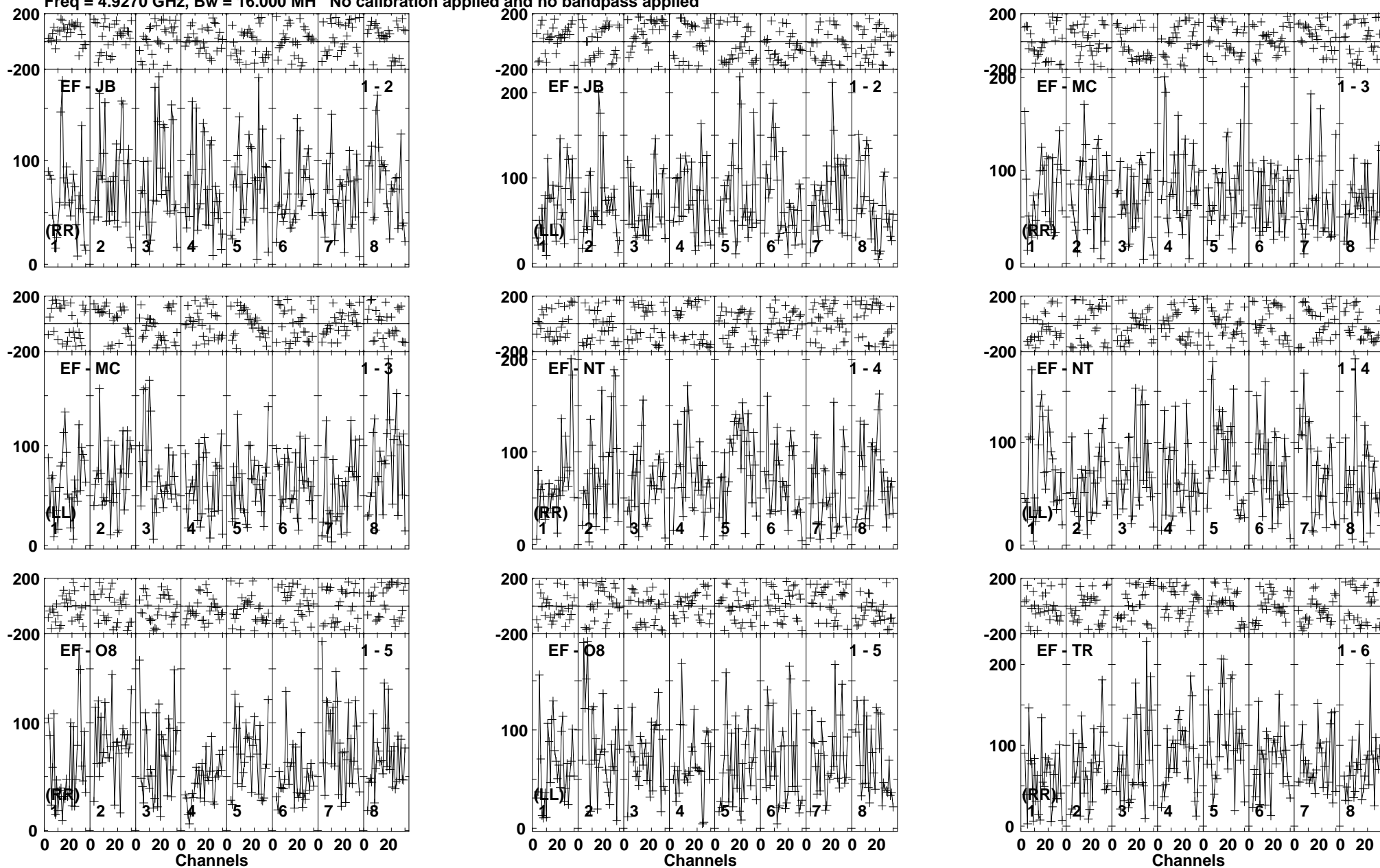
Lower frame: Micro Ampl Jy Top frame: Phas deg Vector averaged cross-power spectrum Baseline: EF (01) - JB (02) Timerange: 01/03:35:30 to 01/03:39:20
