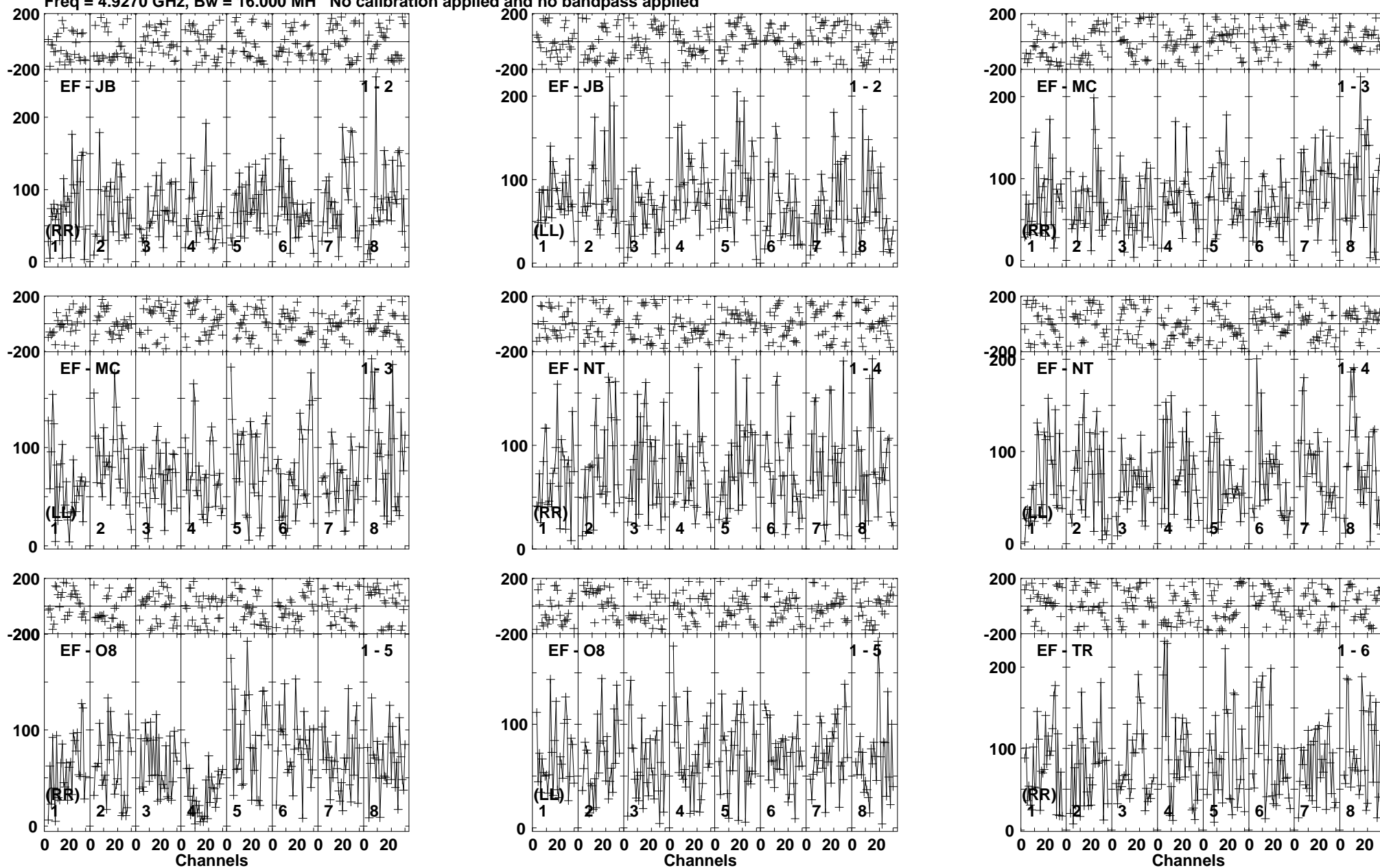
Lower frame: Micro Ampl Jy Top frame: Phas deg Vector averaged cross-power spectrum Baseline: EF (01) - JB (02) Timerange: 01/00:24:30 to 01/00:28:09
