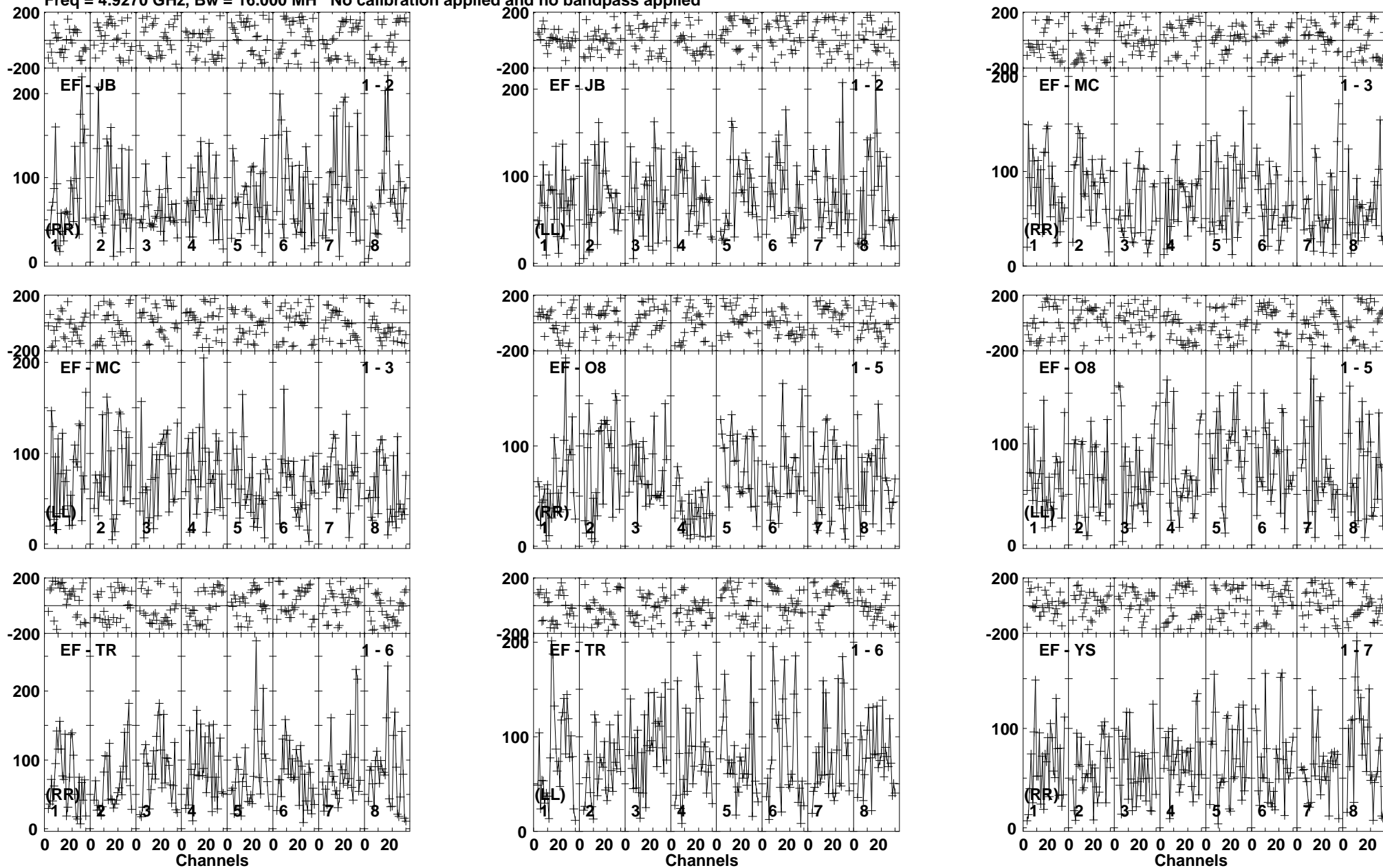
Lower frame: Micro Ampl Jy Top frame: Phas deg Vector averaged cross-power spectrum Baseline: EF (01) - JB (02) Timerange: 00/22:03:30 to 00/22:07:20
