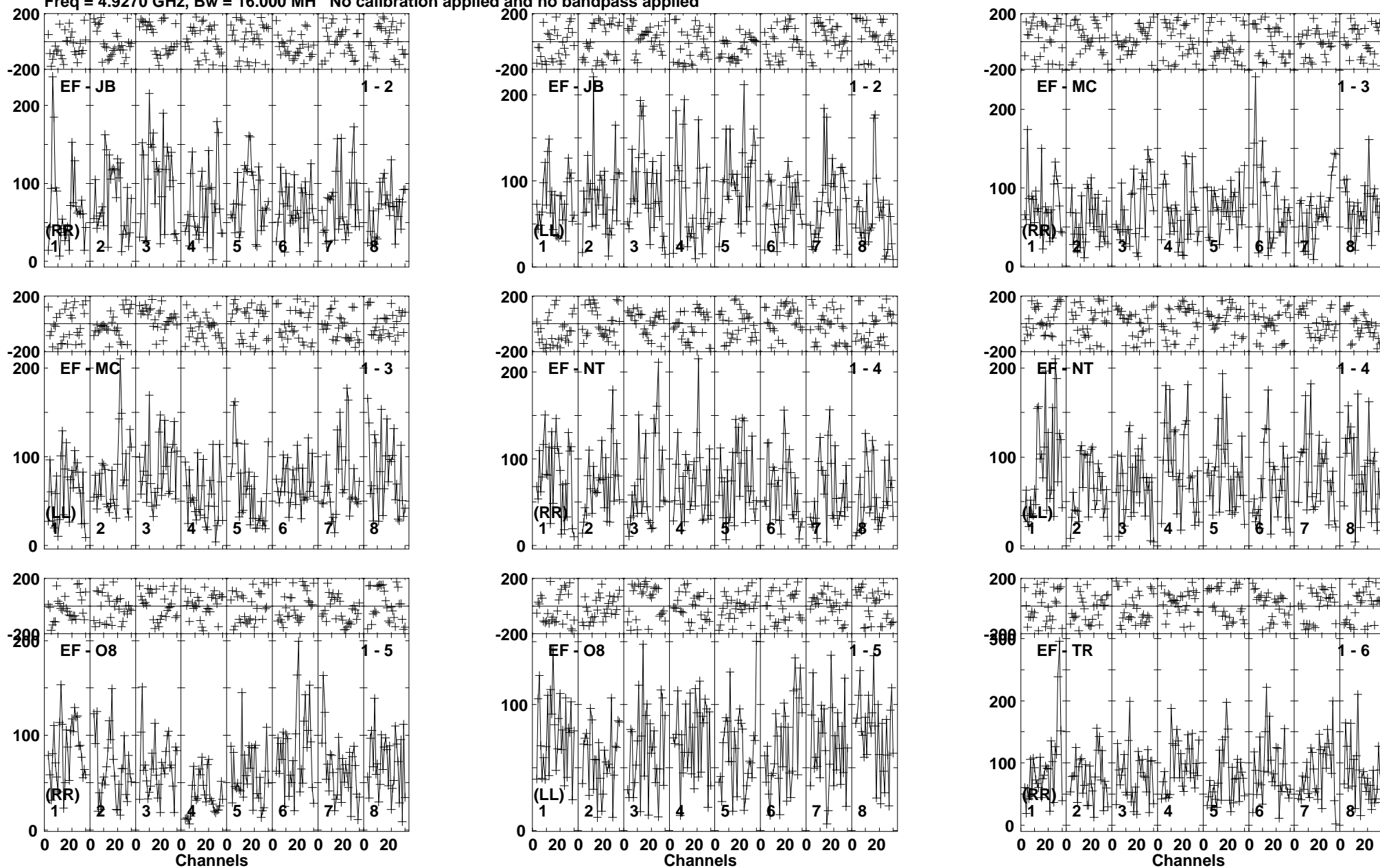
Lower frame: Micro Ampl Jy Top frame: Phas deg Vector averaged cross-power spectrum Baseline: EF (01) - JB (02) Timerange: 01/05:00:31 to 01/05:04:20
