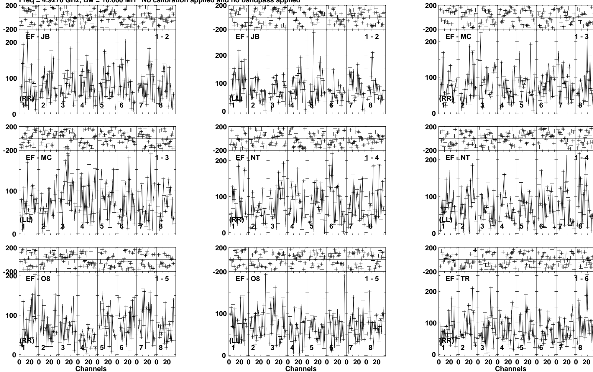
Lower frame: Micro Ampl Jy Top frame: Phas deg Vector averaged cross-power spectrum Baseline: EF (01) - JB (02) Timerange: 00/20:08:31 to 00/20:12:09
