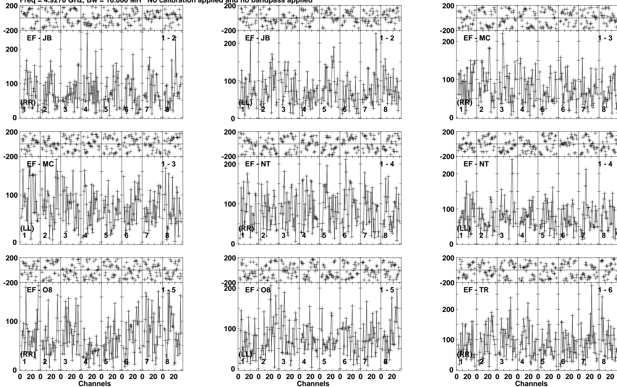
Lower frame: Micro Ampl Jy Top frame: Phas deg Vector averaged cross-power spectrum Baseline: EF (01) - JB (02) Timerange: 00/19:48:30 to 00/19:52:09
