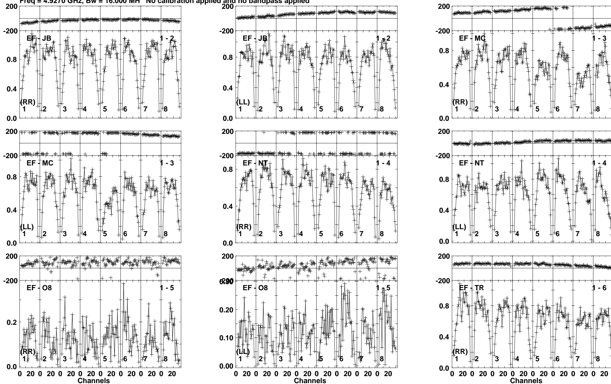
Lower frame: Milli Ampl Jy Top frame: Phas deg Vector averaged cross-power spectrum Baseline: EF (01) - JB (02) Timerange: 00/15:41:11 to 00/15:44:10
