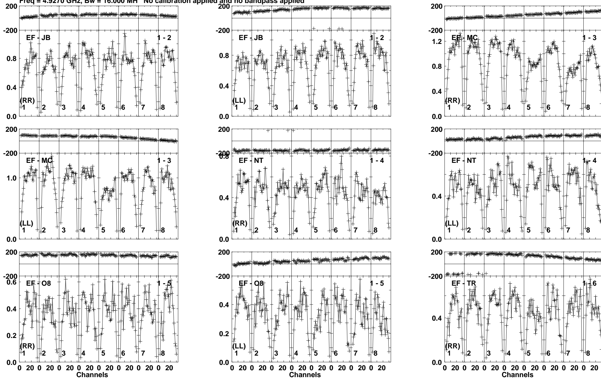
Lower frame: Milli Ampl Jy Top frame: Phas deg Vector averaged cross-power spectrum Baseline: EF (01) - JB (02) Timerange: 00:12:46:21 to 00:12:49:20
