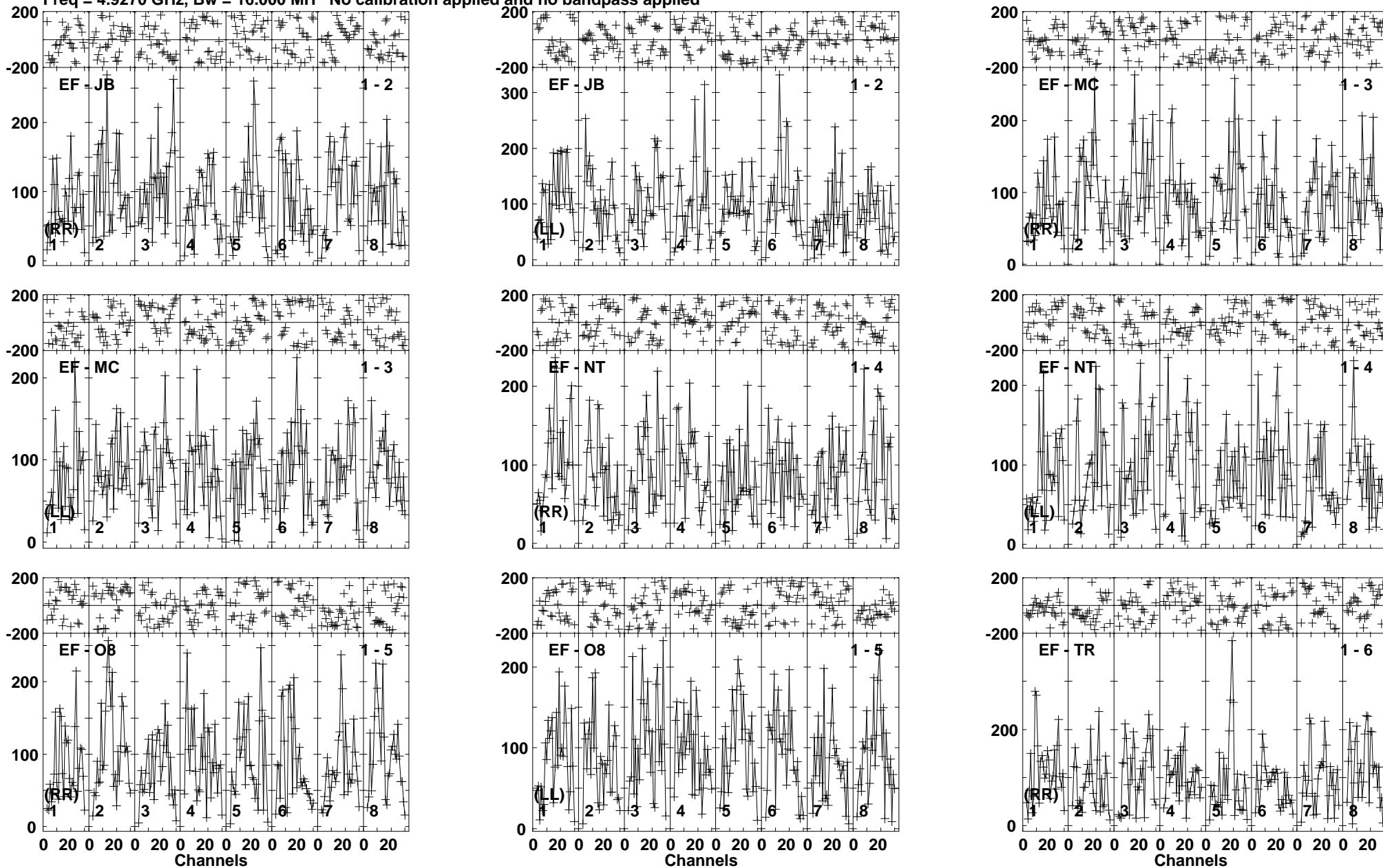
Lower frame: Micro Ampl Jy Top frame: Phas deg Vector averaged cross-power spectrum Baseline: EF (01) - JB (02) Timerange: 00/12:59:51 to 00/13:02:49
