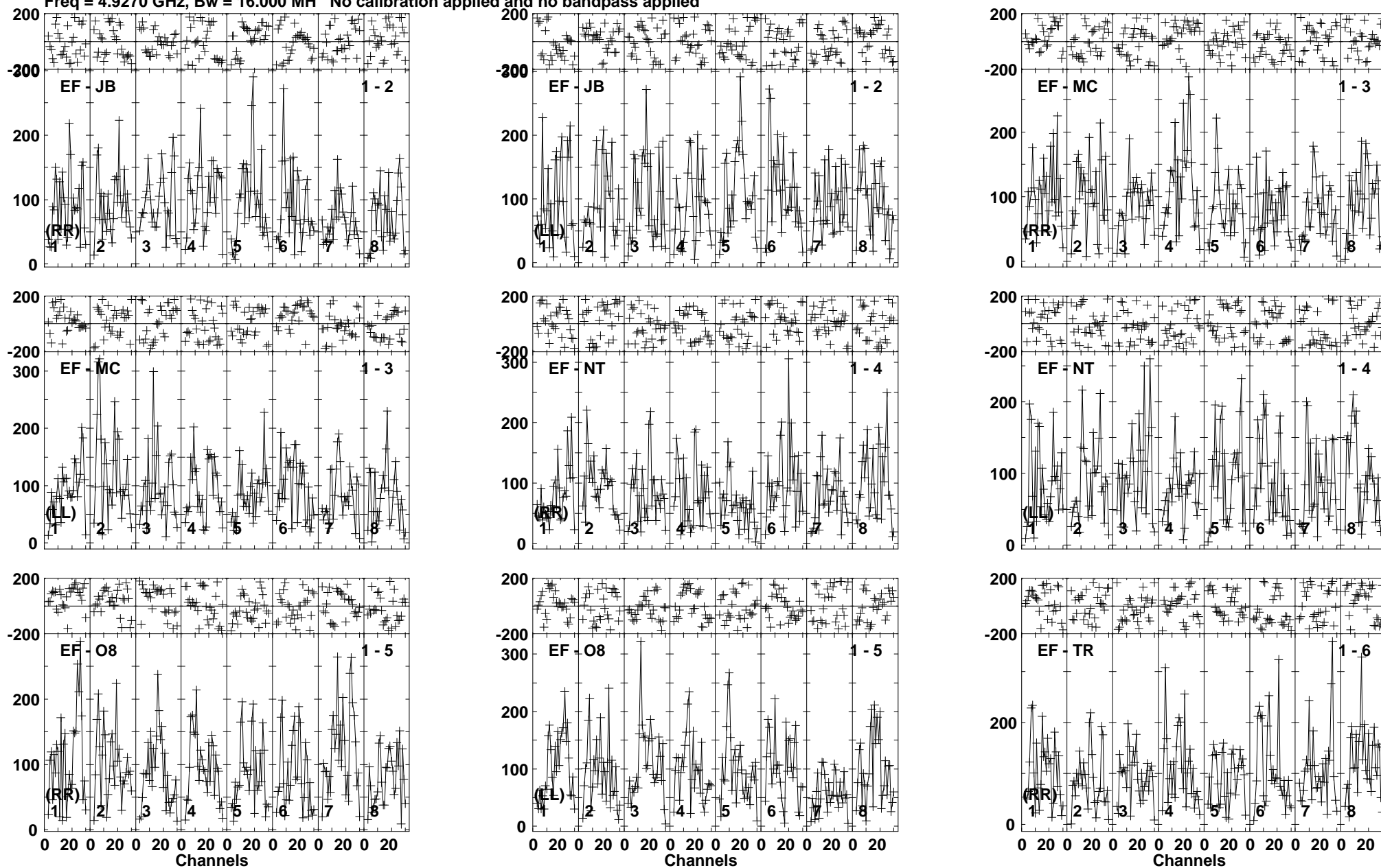
Lower frame: Micro Ampl Jy Top frame: Phas deg Vector averaged cross-power spectrum Baseline: EF (01) - JB (02) Timerange: 00/15:45:40 to 00/15:48:40
