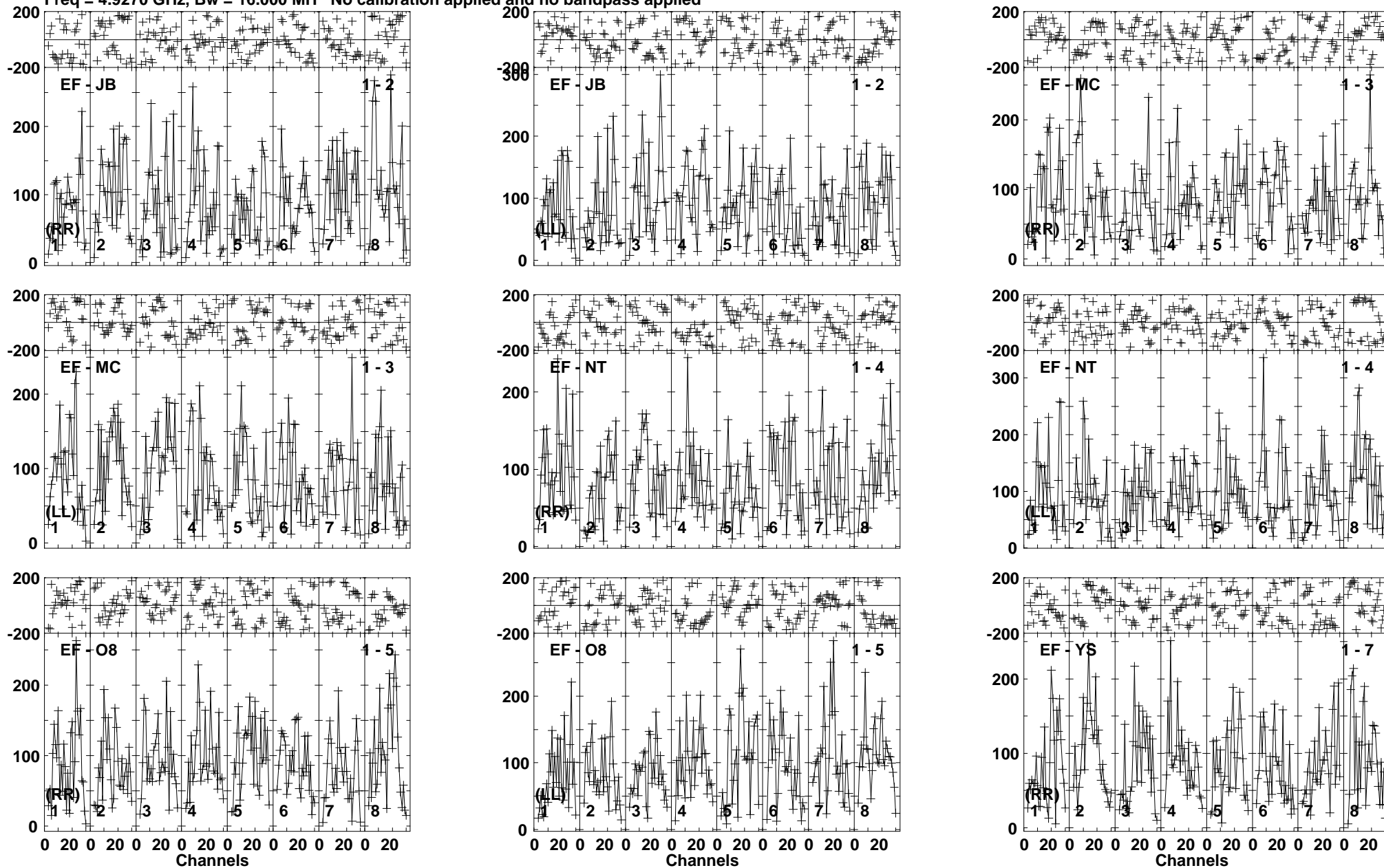
Lower frame: Micro Ampl Jy Top frame: Phas deg Vector averaged cross-power spectrum Baseline: EF (01) - JB (02) Timerange: 00/12:19:20 to 00/12:22:20
