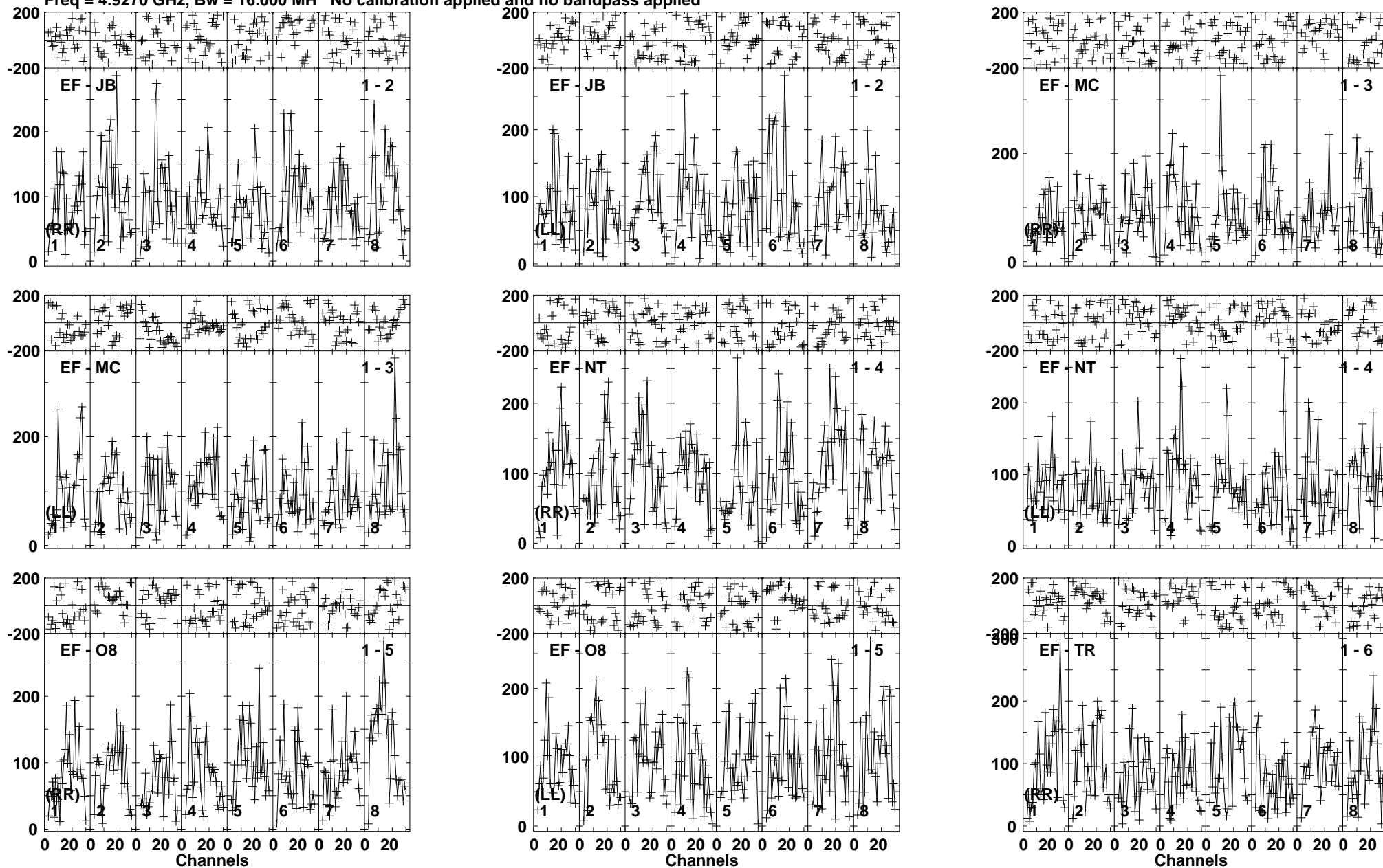
Lower frame: Micro Ampl Jy Top frame: Phas deg Vector averaged cross-power spectrum Baseline: EF (01) - JB (02) Timerange: 00/15:36:40 to 00/15:39:40
