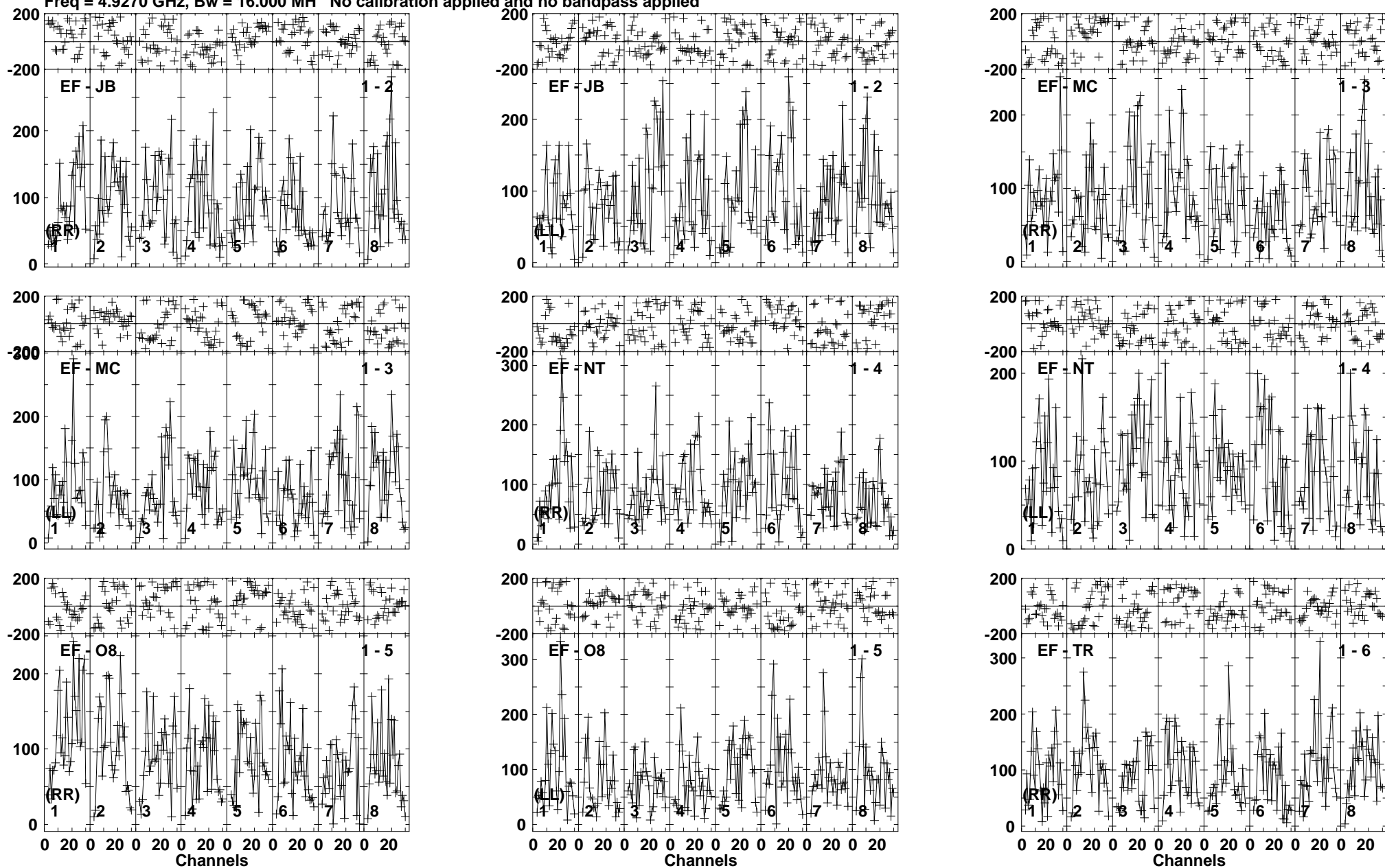
Lower frame: Micro Ampl Jy Top frame: Phas deg Vector averaged cross-power spectrum Baseline: EF (01) - JB (02) Timerange: 00/15:14:10 to 00/15:17:10
