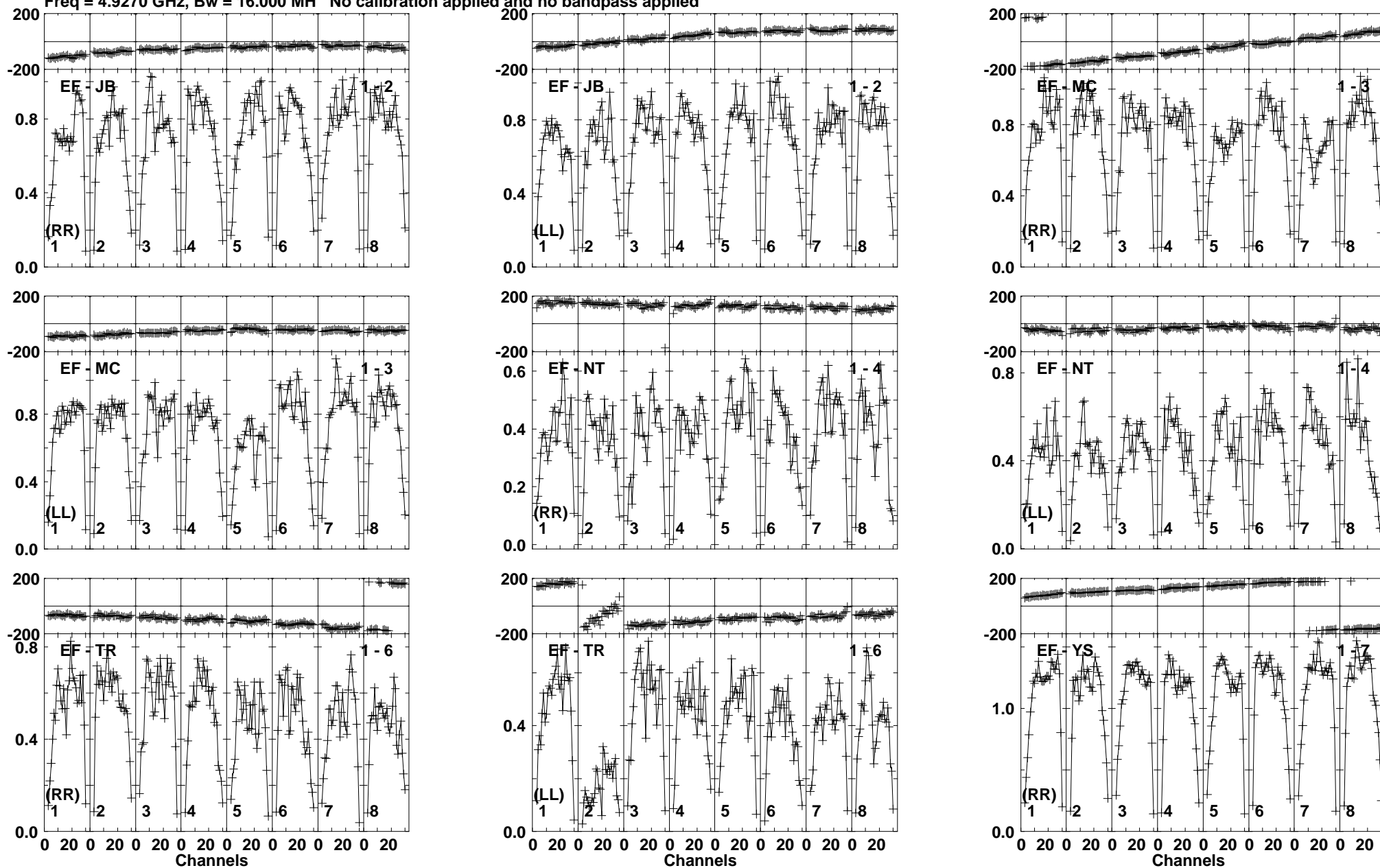
Lower frame: Milli Ampl Jy Top frame: Phas deg Vector averaged cross-power spectrum Baseline: EF (01) - JB (02) Timerange: 00/14:28:21 to 00/14:31:19
