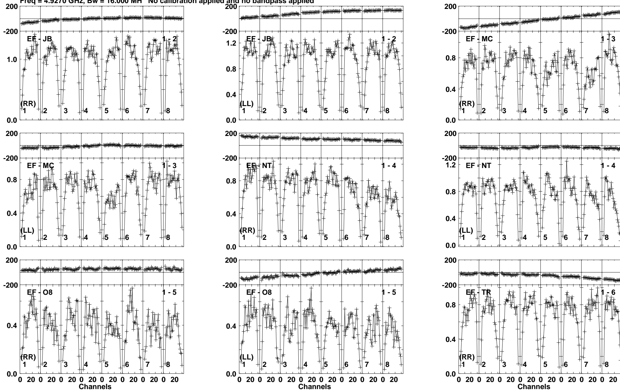
Lower frame: Milli Ampl Jy Top frame: Phas deg Vector averaged cross-power spectrum Baseline: EF (01) - JB (02) Timerange: 00/12:58:30 to 00/13:01:30
