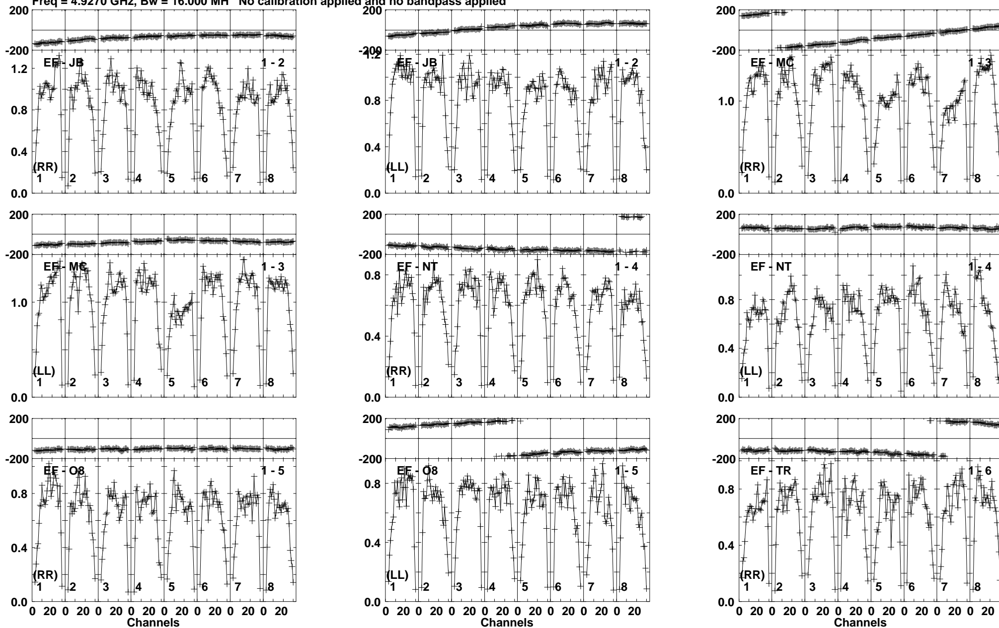
Lower frame: Milli Ampl Jy Top frame: Phas deg Vector averaged cross-power spectrum Baseline: EF (01) - JB (02) Timerange: 00/13:16:30 to 00/13:19:30
