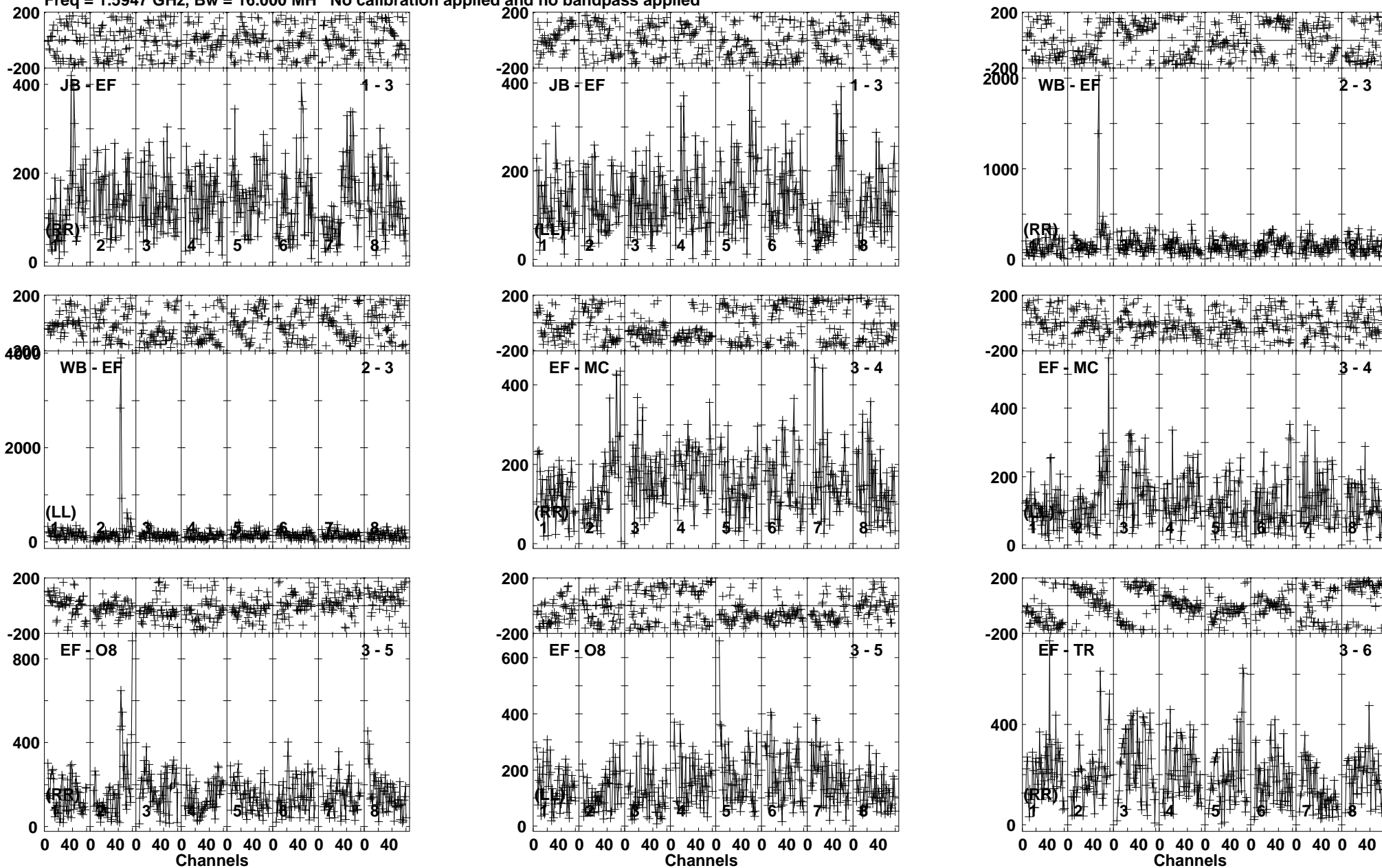
Lower frame: Micro Ampl Jy Top frame: Phas deg Vector averaged cross-power spectrum Baseline: JB (01) - EF (03) Timerange: 01/00:26:01 to 01/00:28:29
