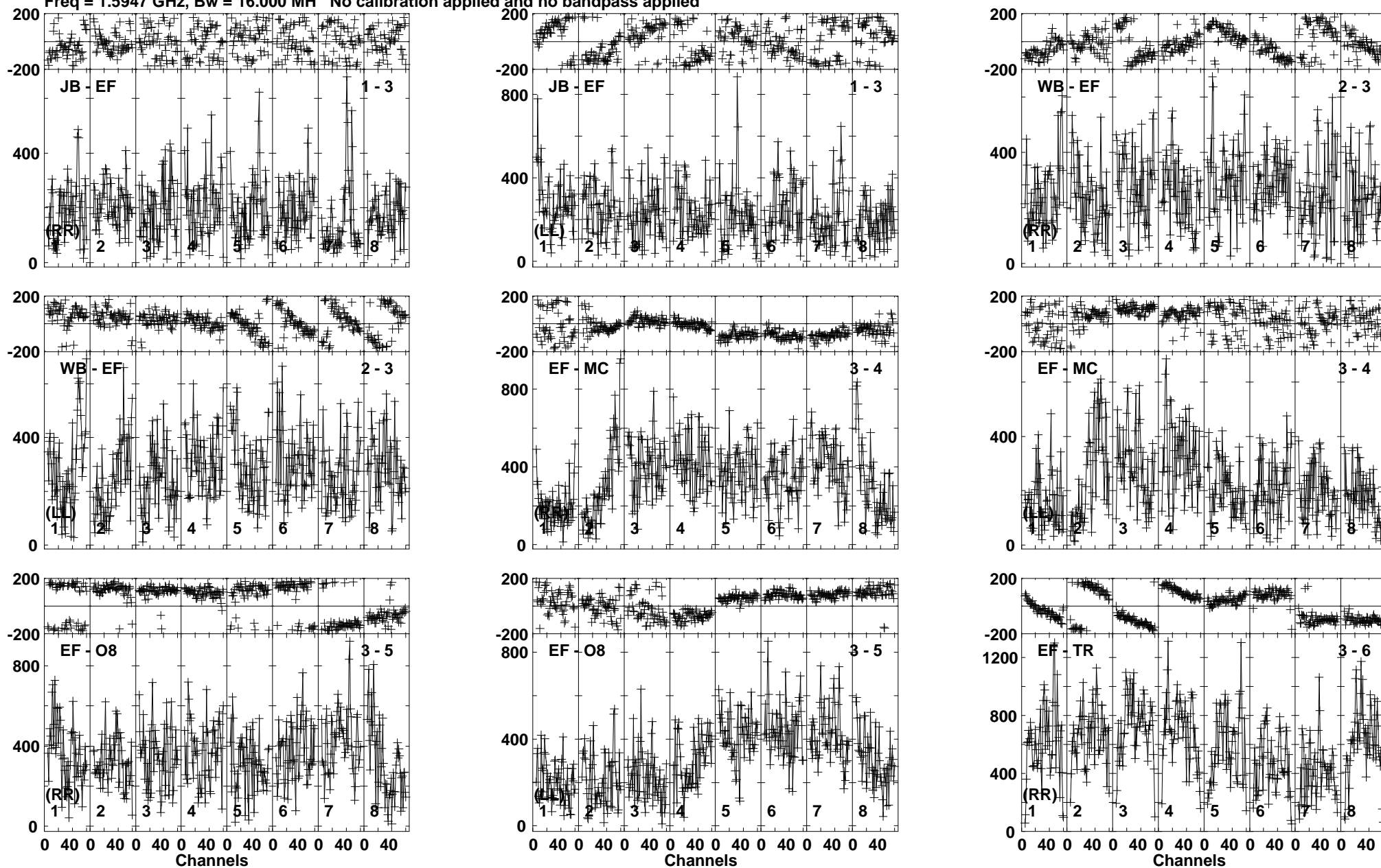
Lower frame: Micro Ampl Jy Top frame: Phas deg Vector averaged cross-power spectrum Baseline: JB (01) - EF (03) Timerange: 00/23:44:51 to 00/23:46:19
