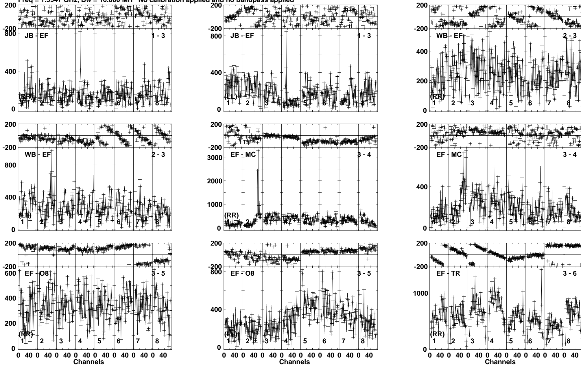
Lower frame: Micro Ampl Jy Top frame: Phas deg Vector averaged cross-power spectrum Baseline: JB (01) - EF (03) Timerange: 00/23:55:51 to 00/23:57:49
