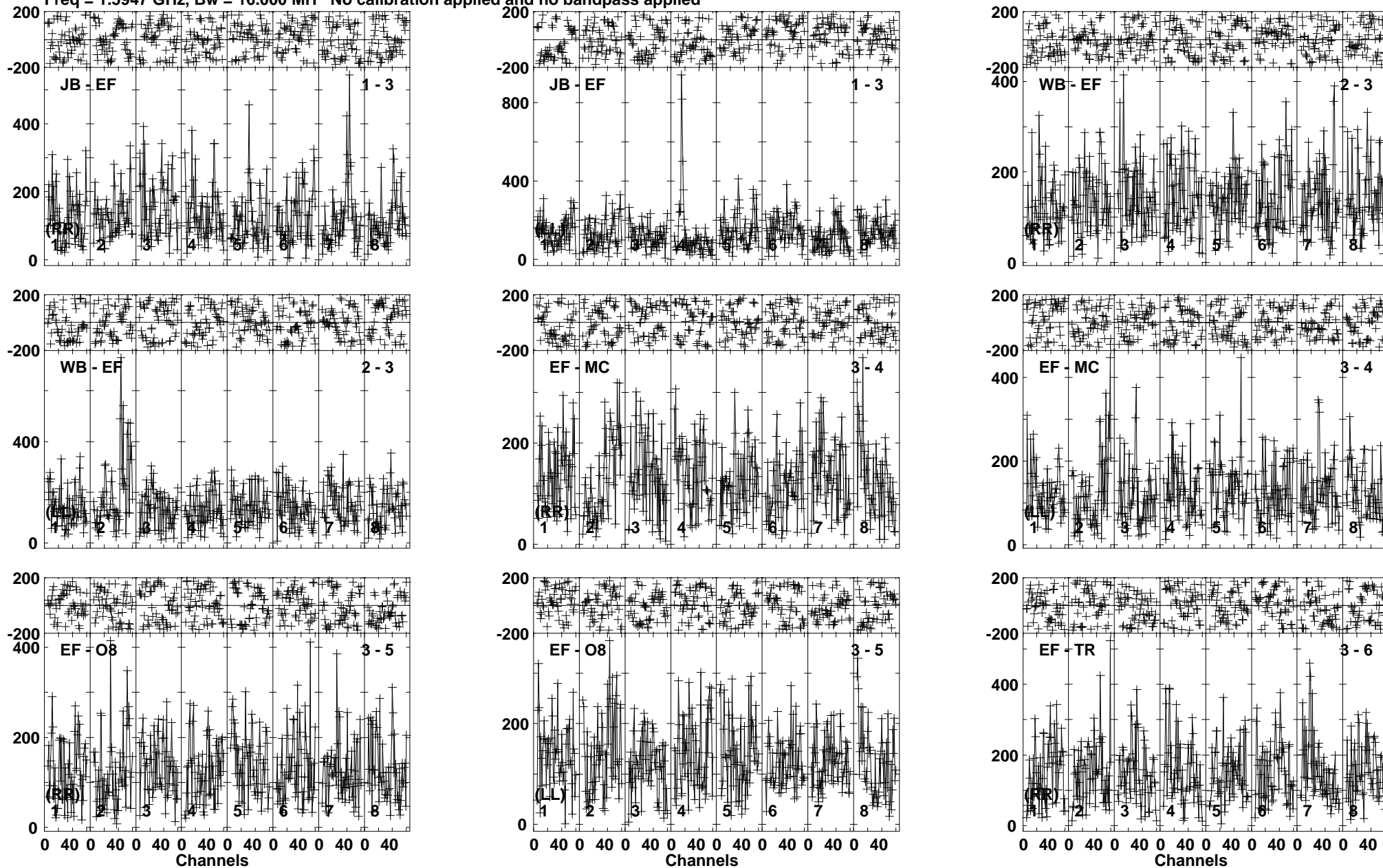
Lower frame: Micro Ampl Jy Top frame: Phas deg Vector averaged cross-power spectrum Baseline: JB (01) - EF (03) Timerange: 01/00:01:51 to 01/00:04:19
