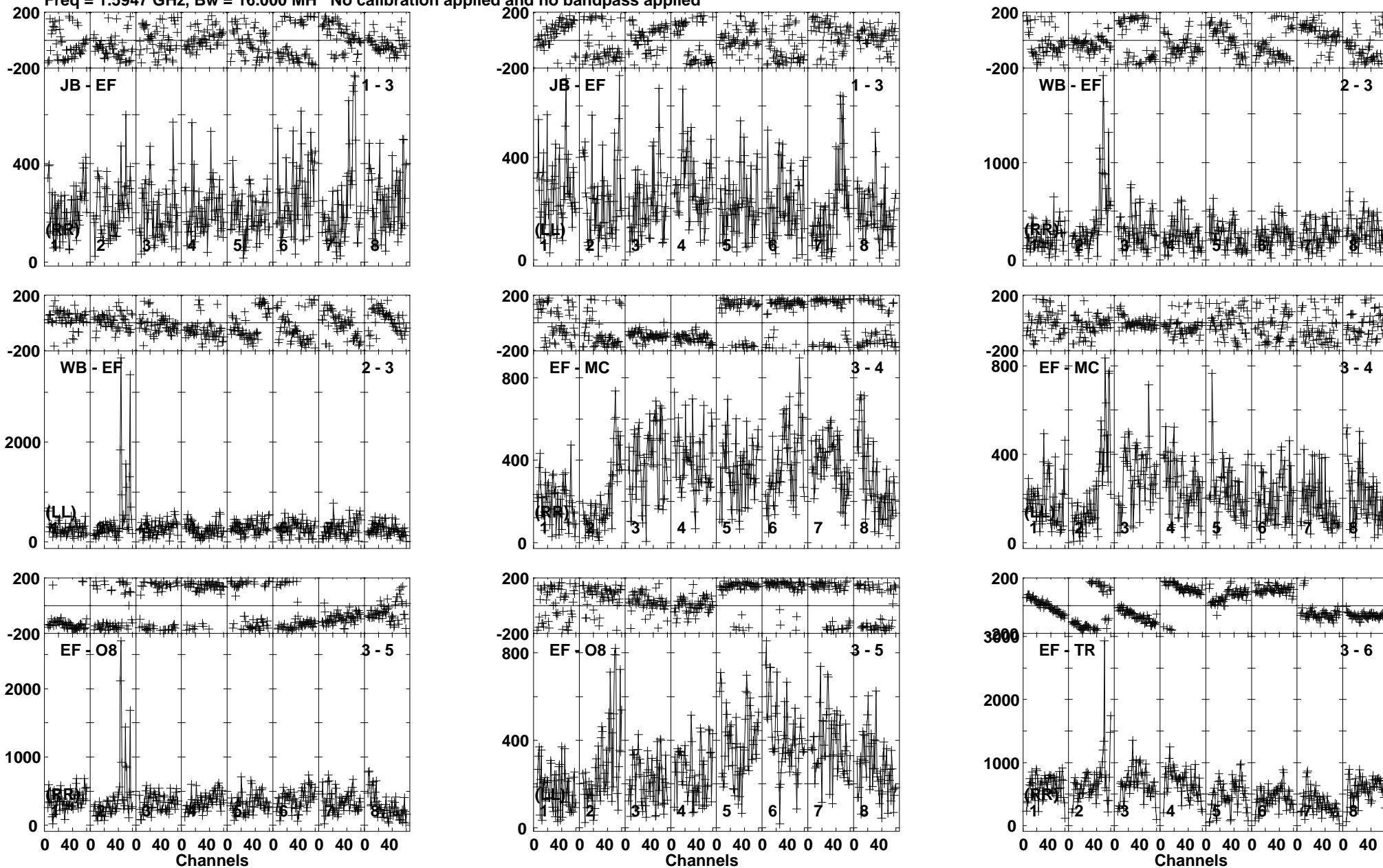
Lower frame: Micro Ampl Jy Top frame: Phas deg Vector averaged cross-power spectrum Baseline: JB (01) - EF (03) Timerange: 01/01:21:01 to 01/01:22:29
