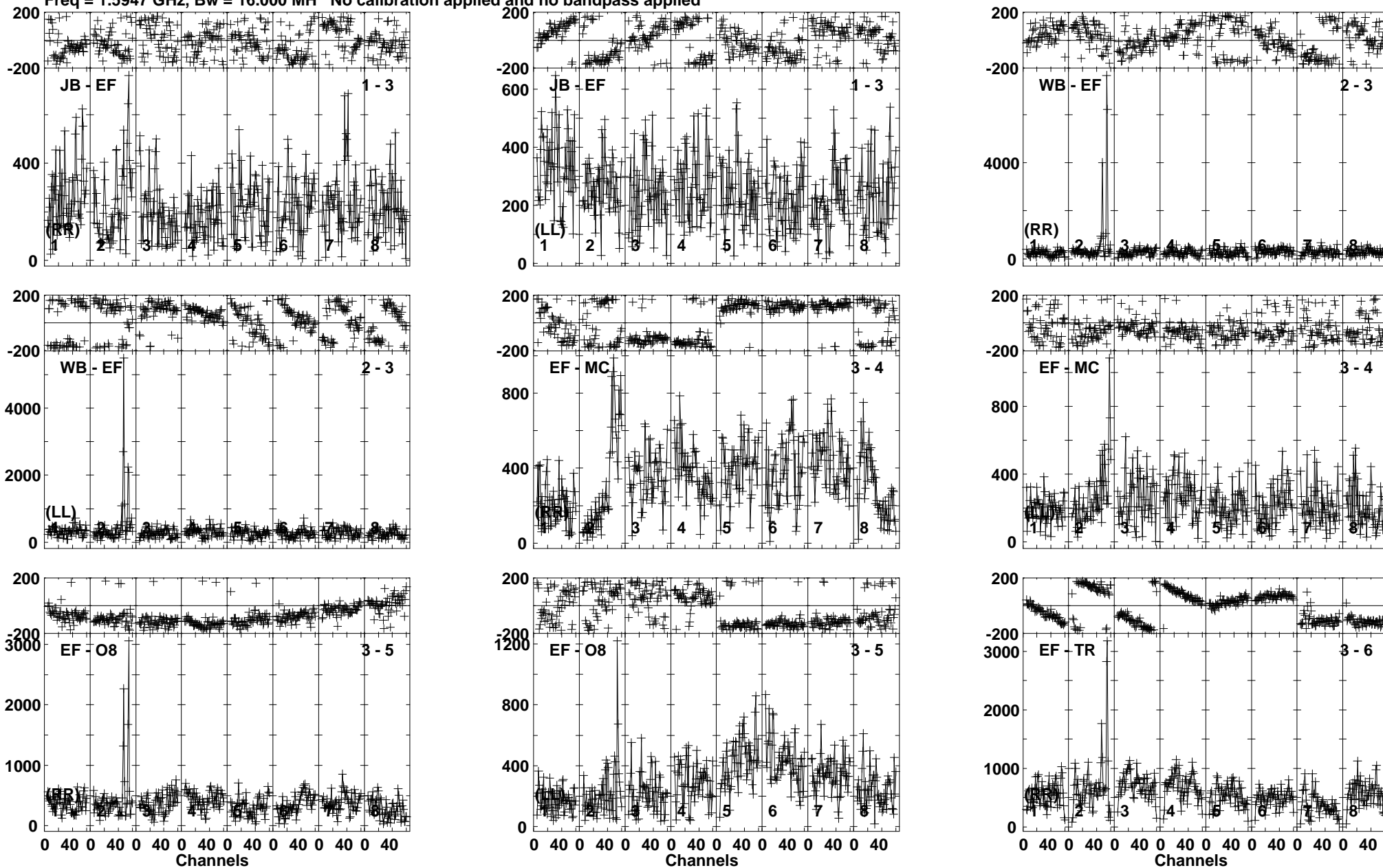
Lower frame: Micro Ampl Jy Top frame: Phas deg Vector averaged cross-power spectrum Baseline: JB (01) - EF (03) Timerange: 01/01:09:31 to 01/01:10:29
