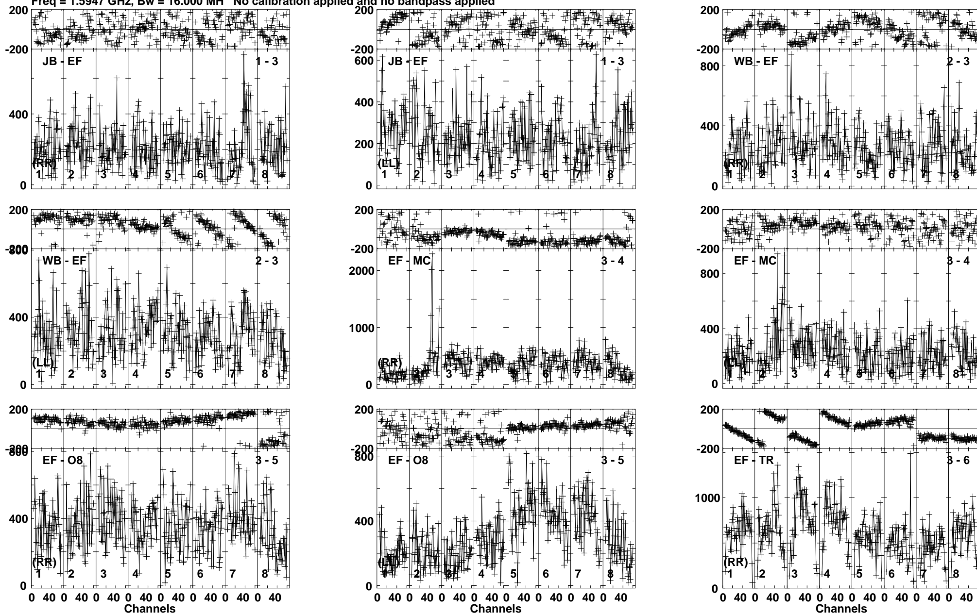
Lower frame: Micro Ampl Jy Top frame: Phas deg Vector averaged cross-power spectrum Baseline: JB (01) - EF (03) Timerange: 01/00:13:01 to 01/00:13:59
