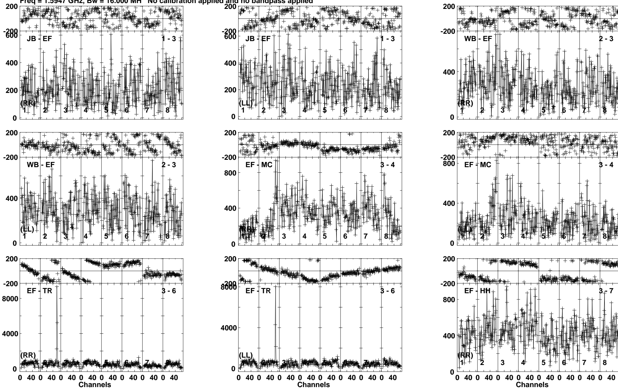
Lower frame: Micro Ampl Jy Top frame: Phas deg Vector averaged cross-power spectrum Baseline: JB (01) - EF (03) Timerange: 01/02:05:31 to 01/02:06:59
