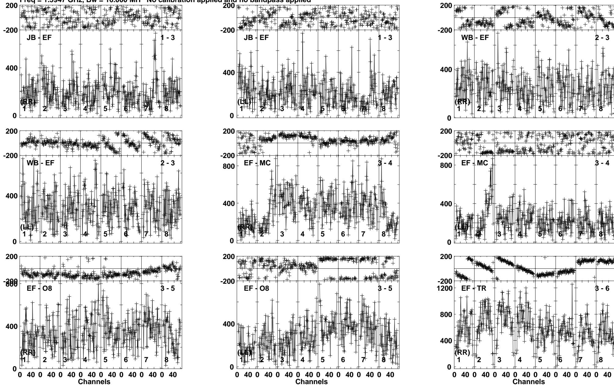
Lower frame: Micro Ampl Jy Top frame: Phas deg Vector averaged cross-power spectrum Baseline: JB (01) - EF (03) Timerange: 00:22:53:01 to 00:22:53:59
