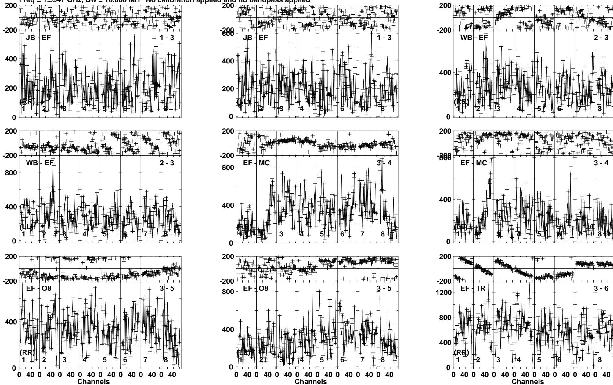
Lower frame: Micro Ampl Jy Top frame: Phas deg Vector averaged cross-power spectrum Baseline: JB (01) - EF (03) Timerange: 00:22:36:51 to 00:22:37:49
