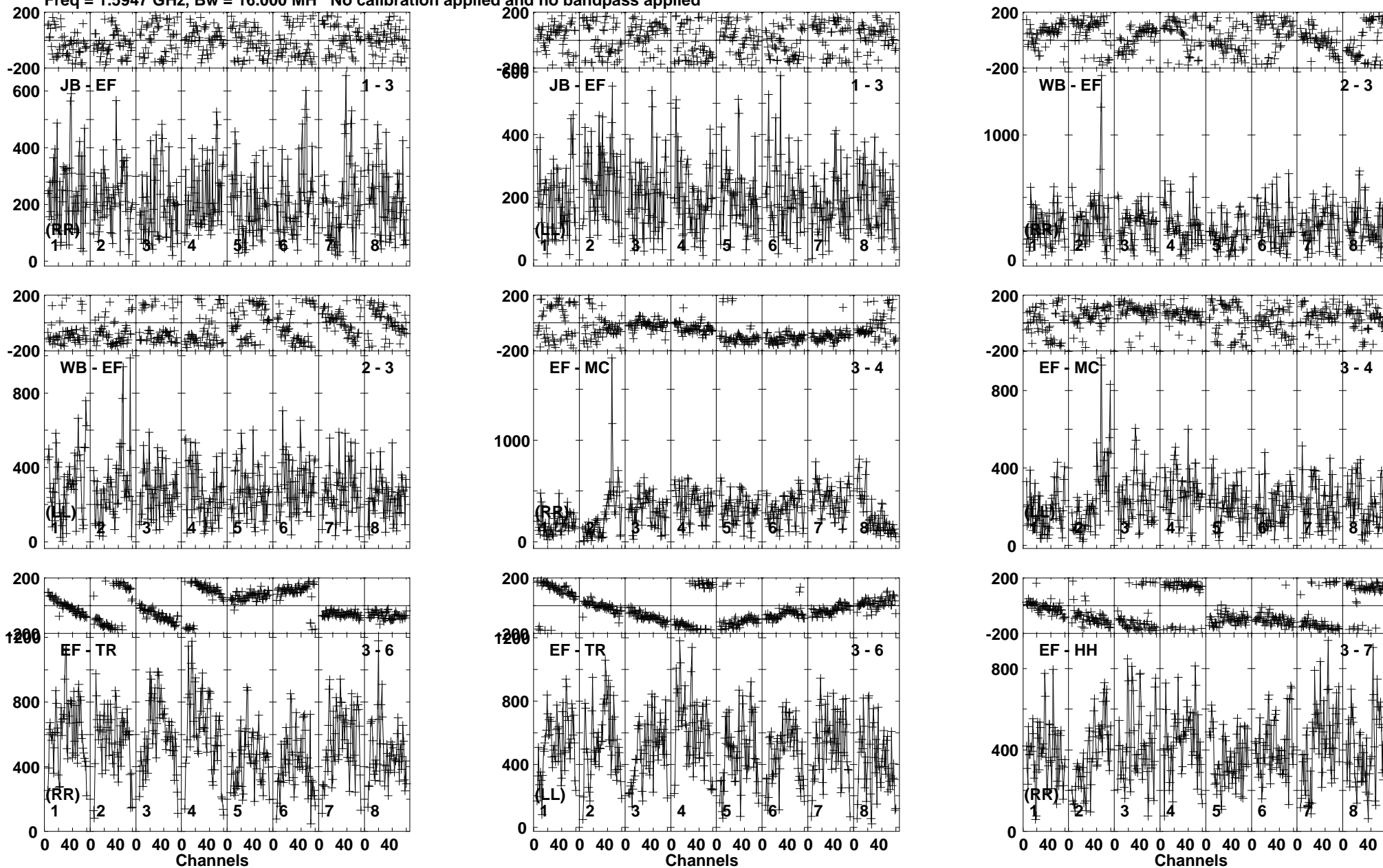
Lower frame: Micro Ampl Jy Top frame: Phas deg Vector averaged cross-power spectrum Baseline: JB (01) - EF (03) Timerange: 00:22:12:01 to 00:22:13:29
