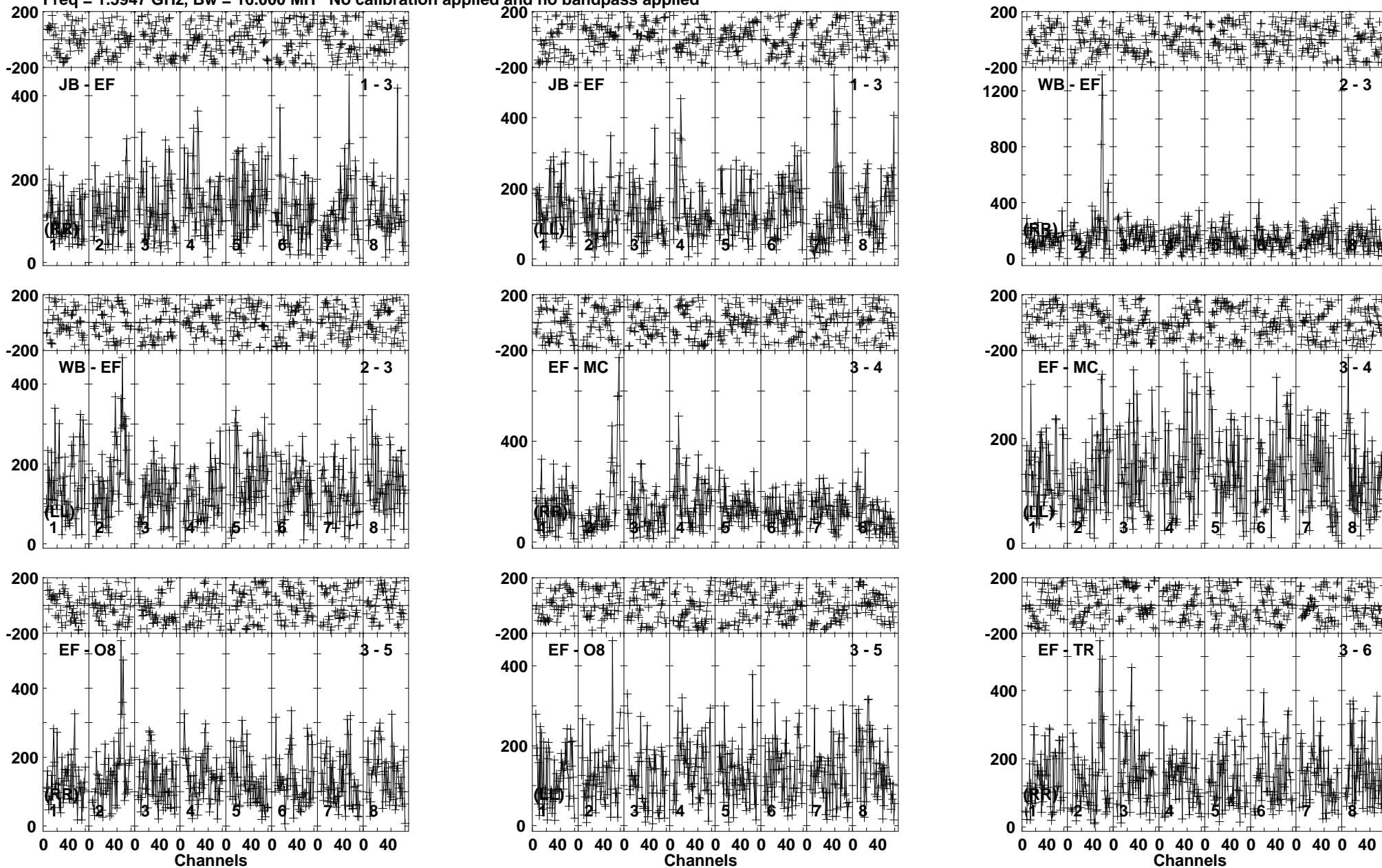
Lower frame: Micro Ampl Jy Top frame: Phas deg Vector averaged cross-power spectrum Baseline: JB (01) - EF (03) Timerange: 00/23:38:21 to 00/23:40:49
