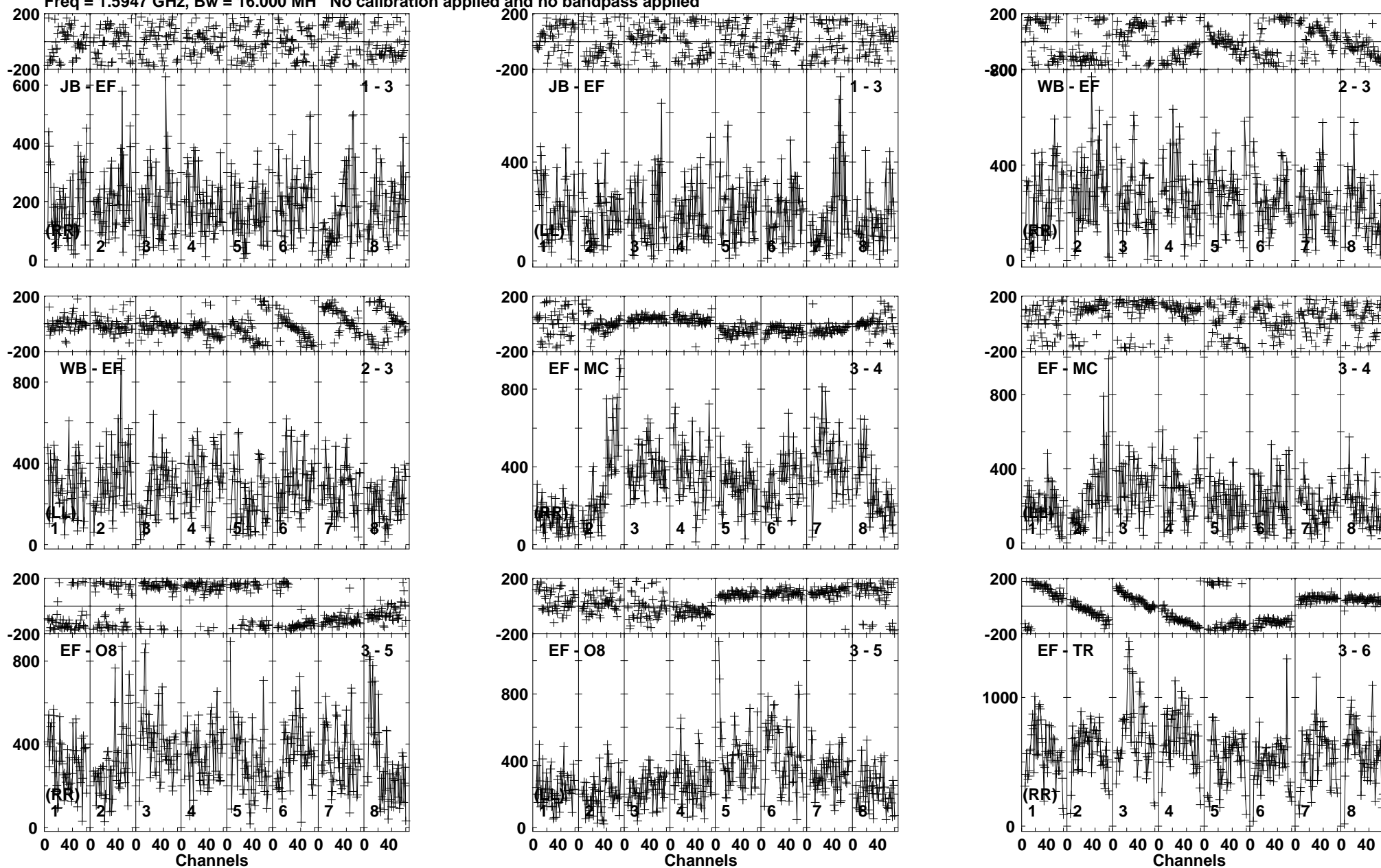
Lower frame: Micro Ampl Jy Top frame: Phas deg Vector averaged cross-power spectrum Baseline: JB (01) - EF (03) Timerange: 00:22:32:11 to 00:22:33:39
