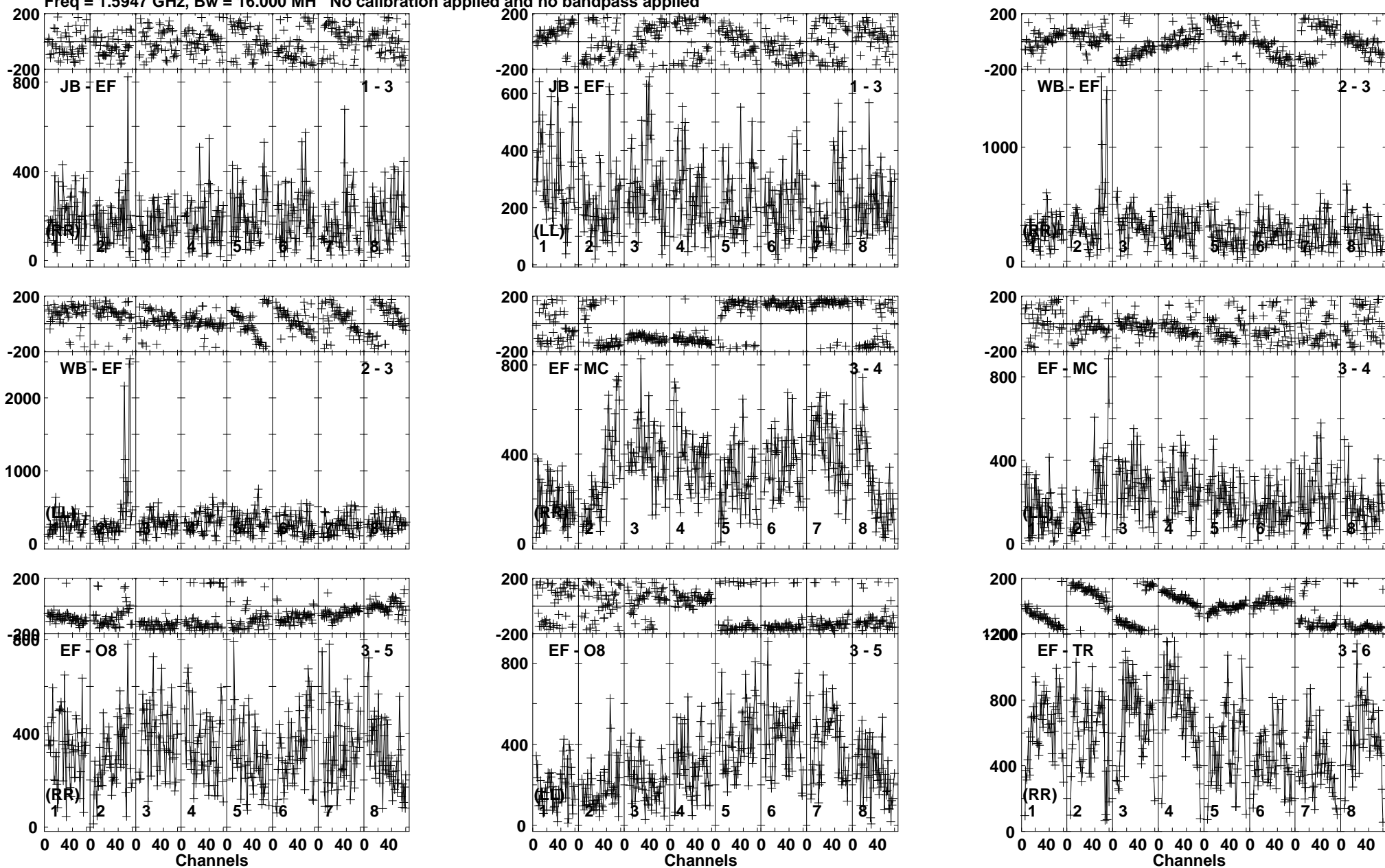
Lower frame: Micro Ampl Jy Top frame: Phas deg Vector averaged cross-power spectrum Baseline: JB (01) - EF (03) Timerange: 01/01:13:01 to 01/01:14:29
