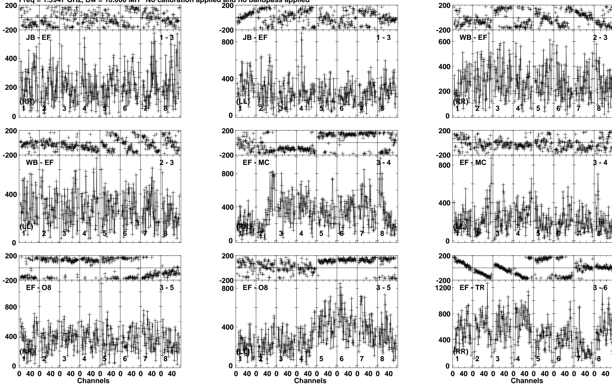
Lower frame: Micro Ampl Jy Top frame: Phas deg Vector averaged cross-power spectrum Baseline: JB (01) - EF (03) Timerange: 01/01:25:41 to 01/01:26:39
