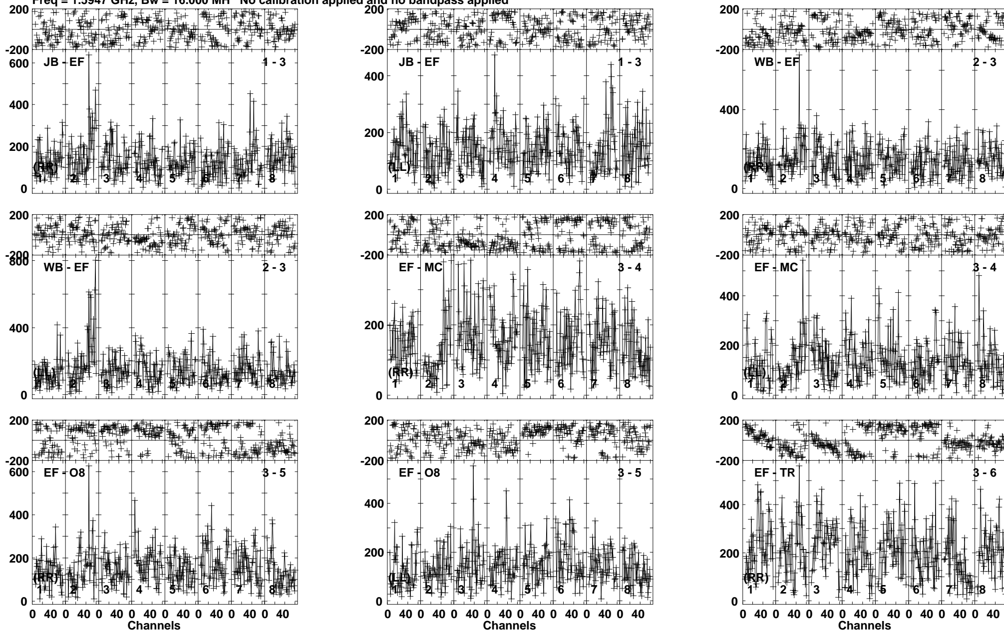
Lower frame: Micro Ampl Jy Top frame: Phas deg Vector averaged cross-power spectrum Baseline: JB (01) - EF (03) Timerange: 01/01:22:31 to 01/01:24:59
