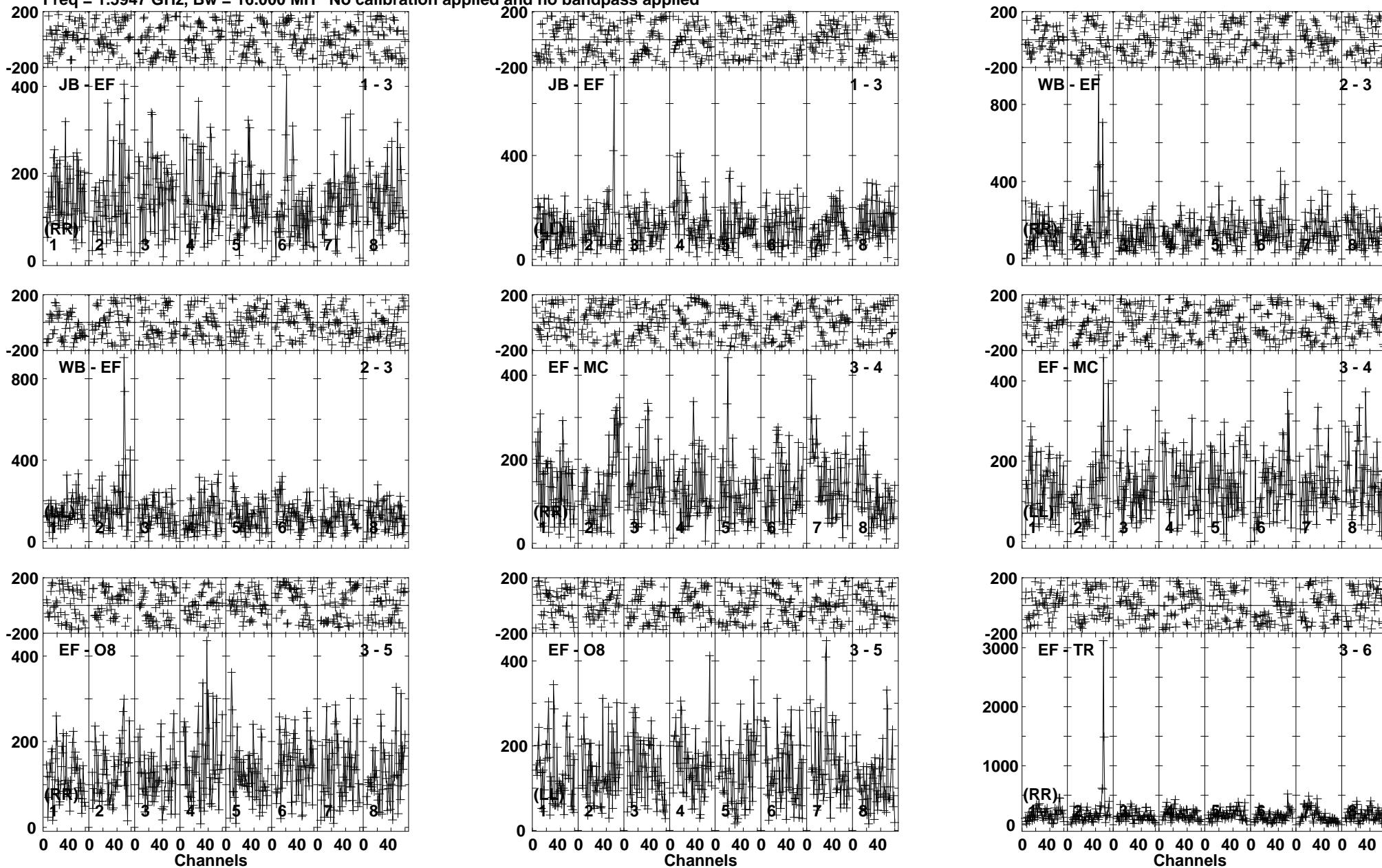
Lower frame: Micro Ampl Jy Top frame: Phas deg Vector averaged cross-power spectrum Baseline: JB (01) - EF (03) Timerange: 01/01:30:41 to 01/01:33:09
