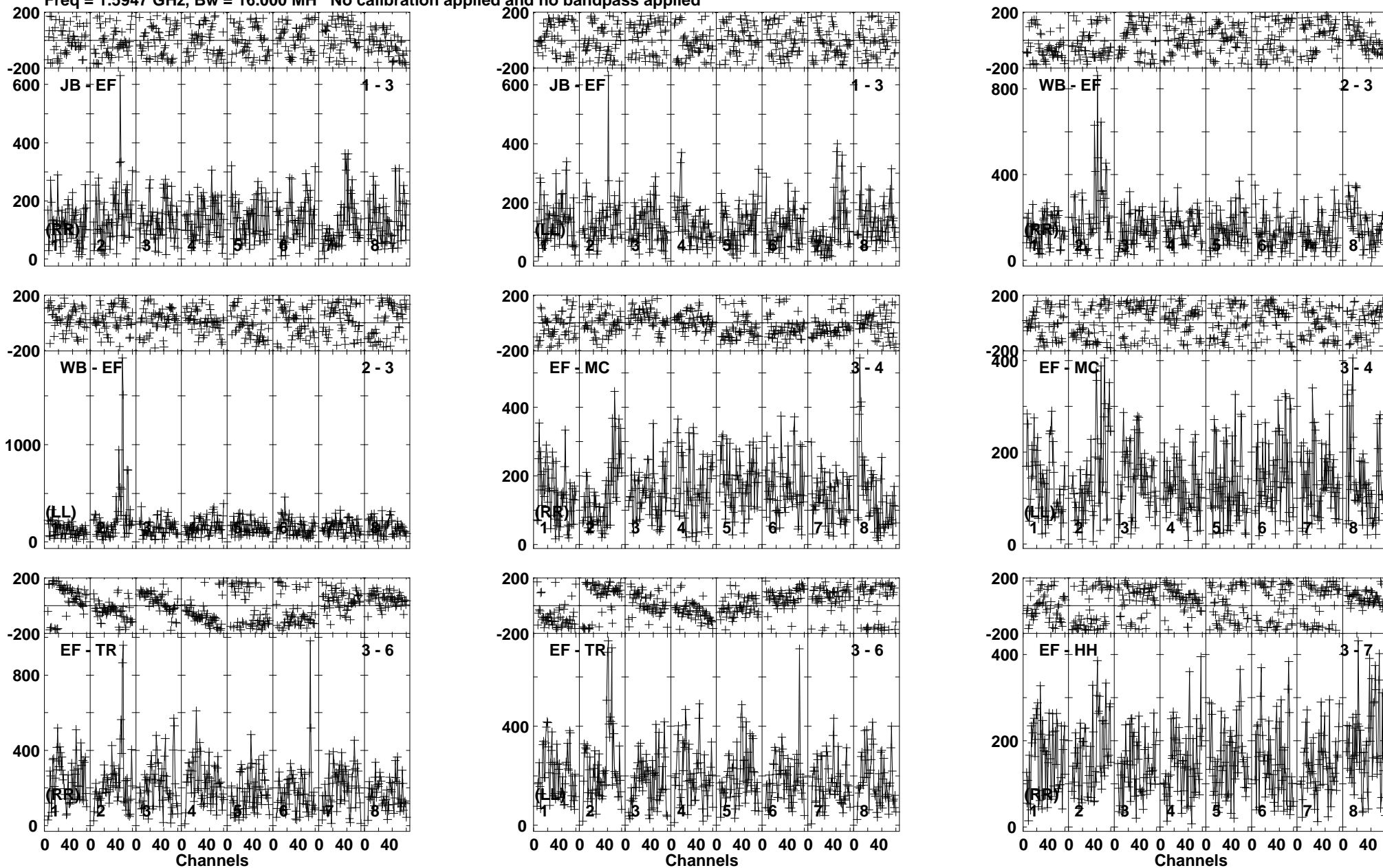
Lower frame: Micro Ampl Jy Top frame: Phas deg Vector averaged cross-power spectrum Baseline: JB (01) - EF (03) Timerange: 00/22:29:41 to 00/22:32:09
