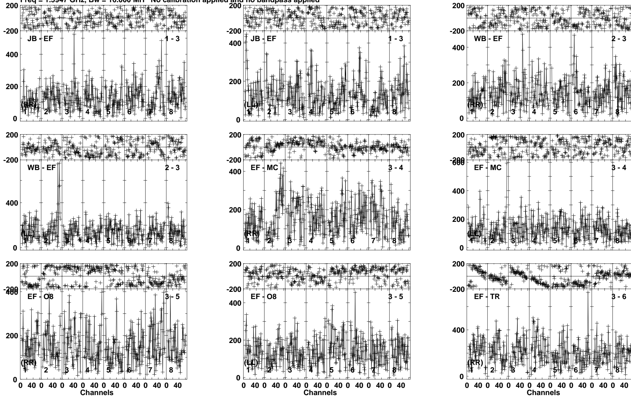
Lower frame: Micro Ampl Jy Top frame: Phas deg Vector averaged cross-power spectrum Baseline: JB (01) - EF (03) Timerange: 00/23:26:11 to 00/23:28:39
