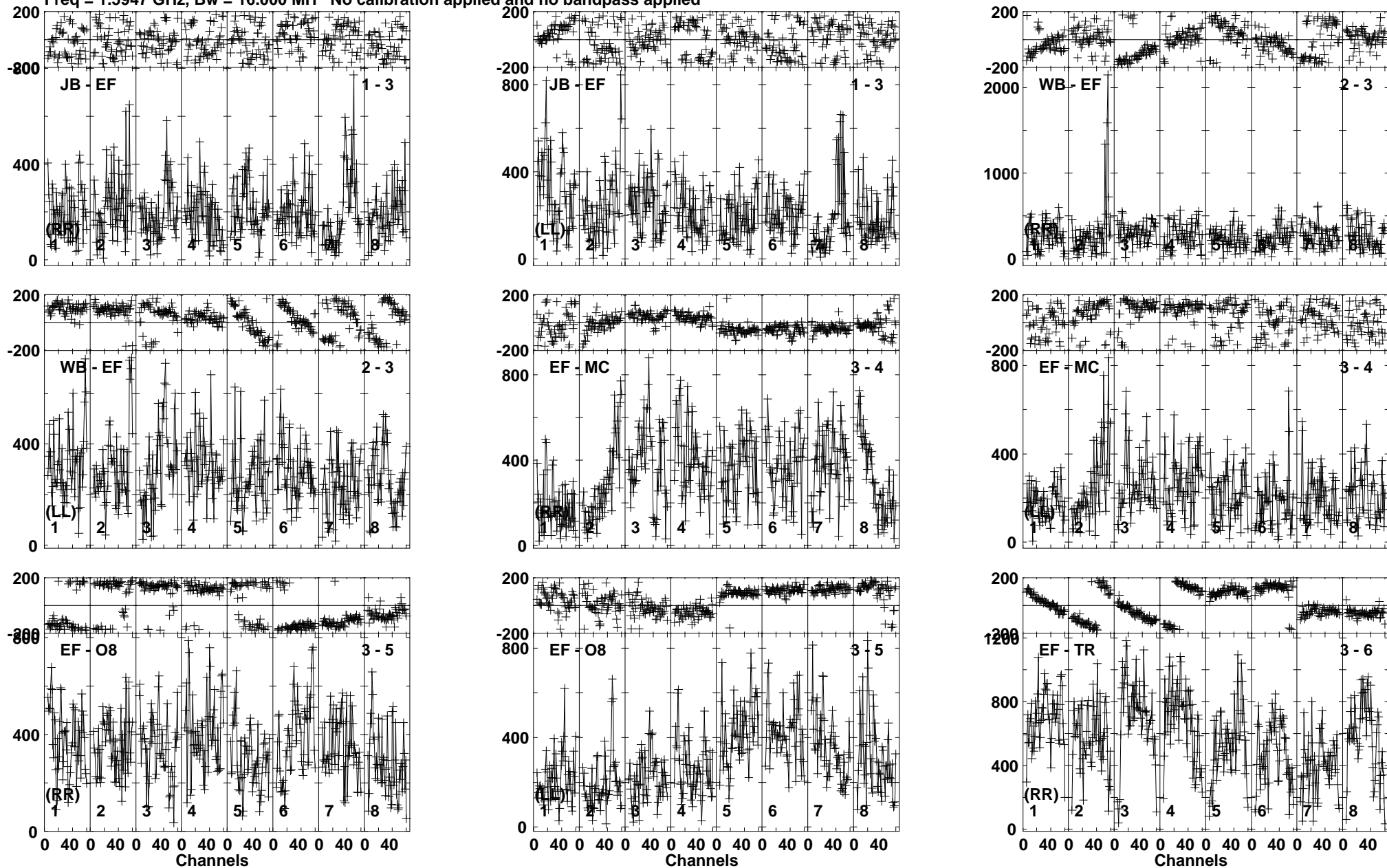
Lower frame: Micro Ampl Jy Top frame: Phas deg Vector averaged cross-power spectrum Baseline: JB (01) - EF (03) Timerange: 00/23:40:51 to 00/23:42:19
