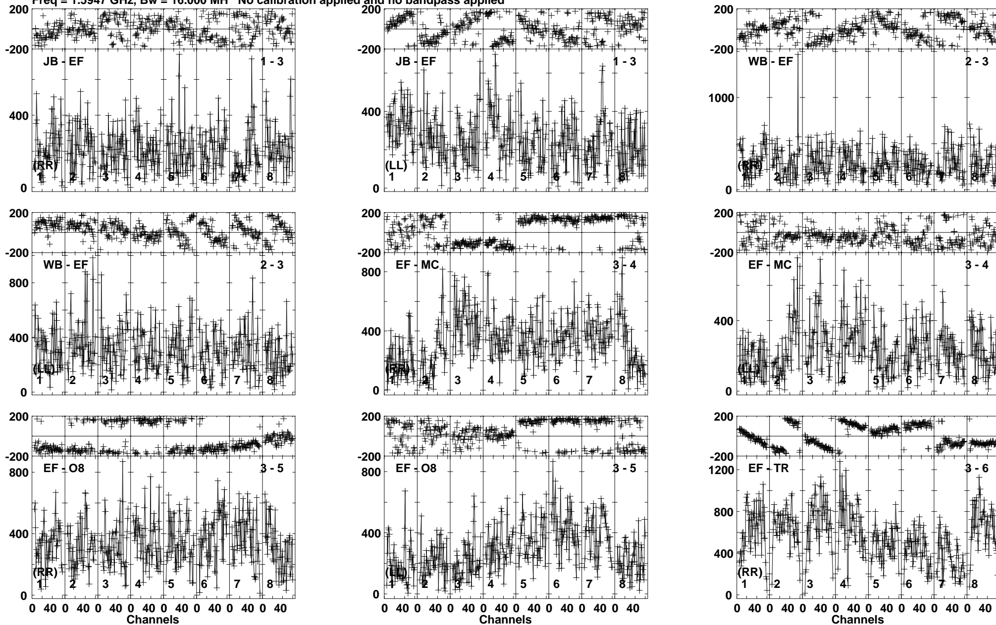
Lower frame: Micro Ampl Jy Top frame: Phas deg Vector averaged cross-power spectrum Baseline: JB (01) - EF (03) Timerange: 01/01:17:31 to 01/01:18:29
