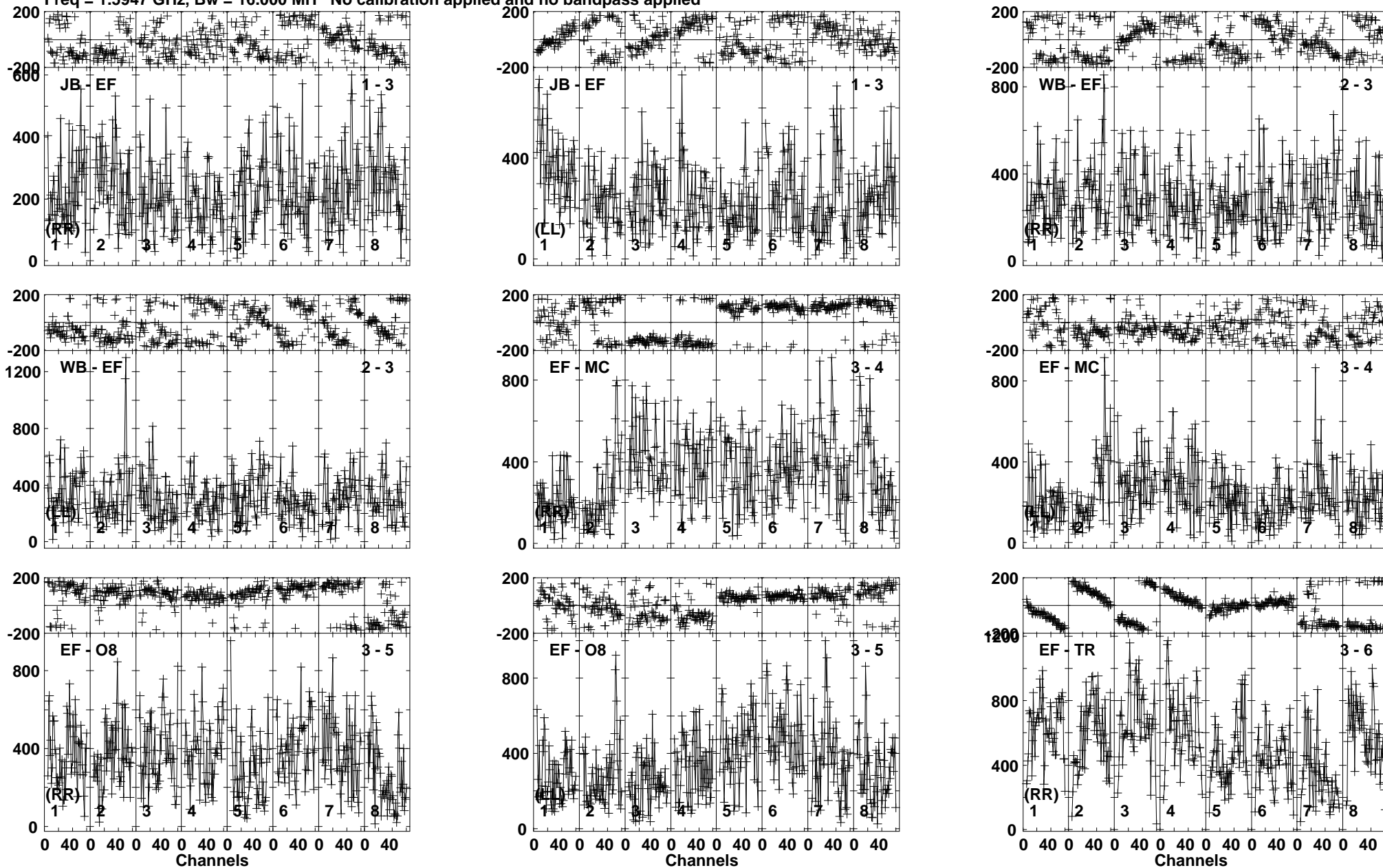
Lower frame: Micro Ampl Jy Top frame: Phas deg Vector averaged cross-power spectrum Baseline: JB (01) - EF (03) Timerange: 01/01:33:41 to 01/01:34:39
