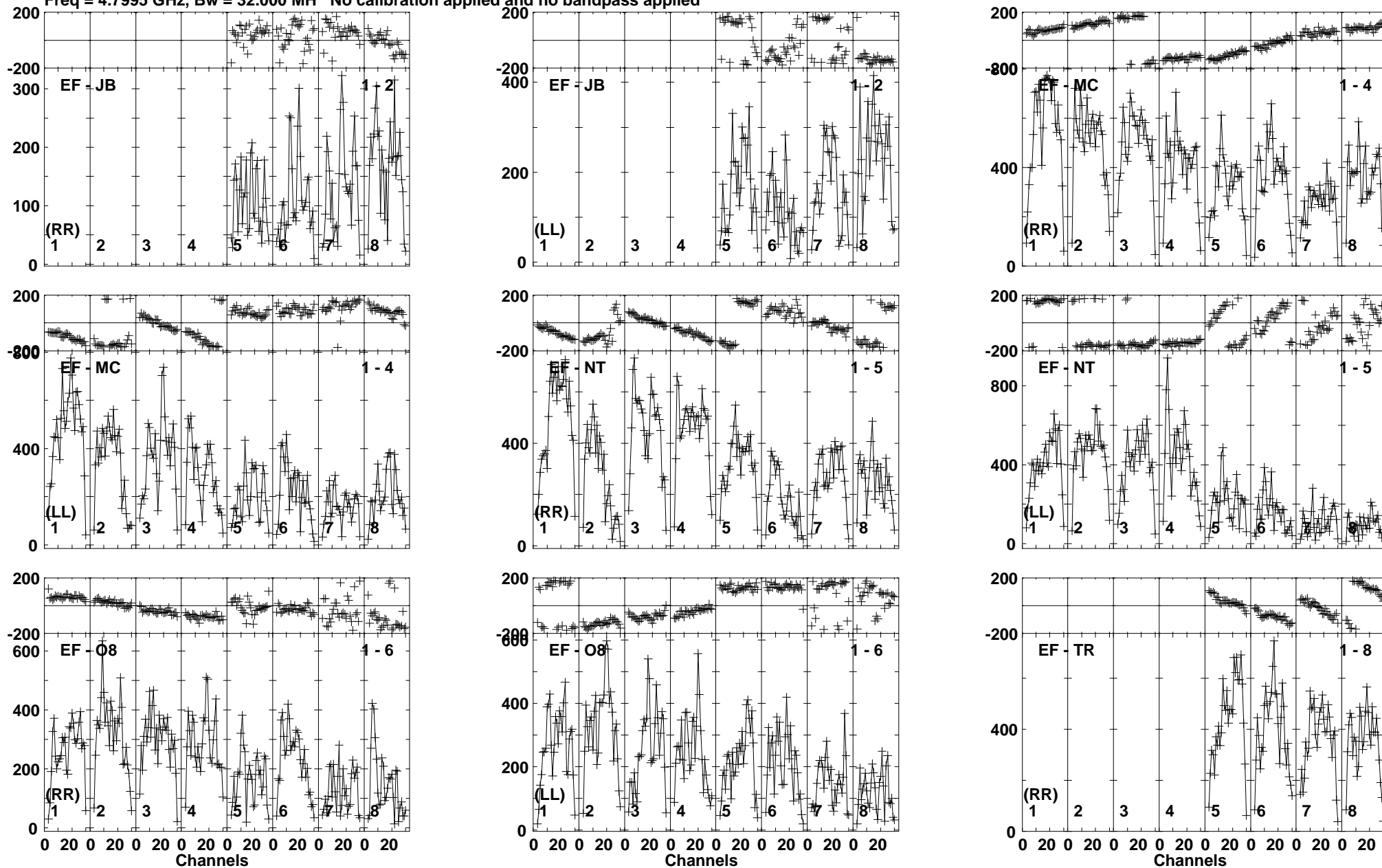
Lower frame: Micro Ampl Jy Top frame: Phas deg Vector averaged cross-power spectrum Baseline: EF (01) - JB (02) Timerange: 00/21:38:51 to 00/21:39:49
