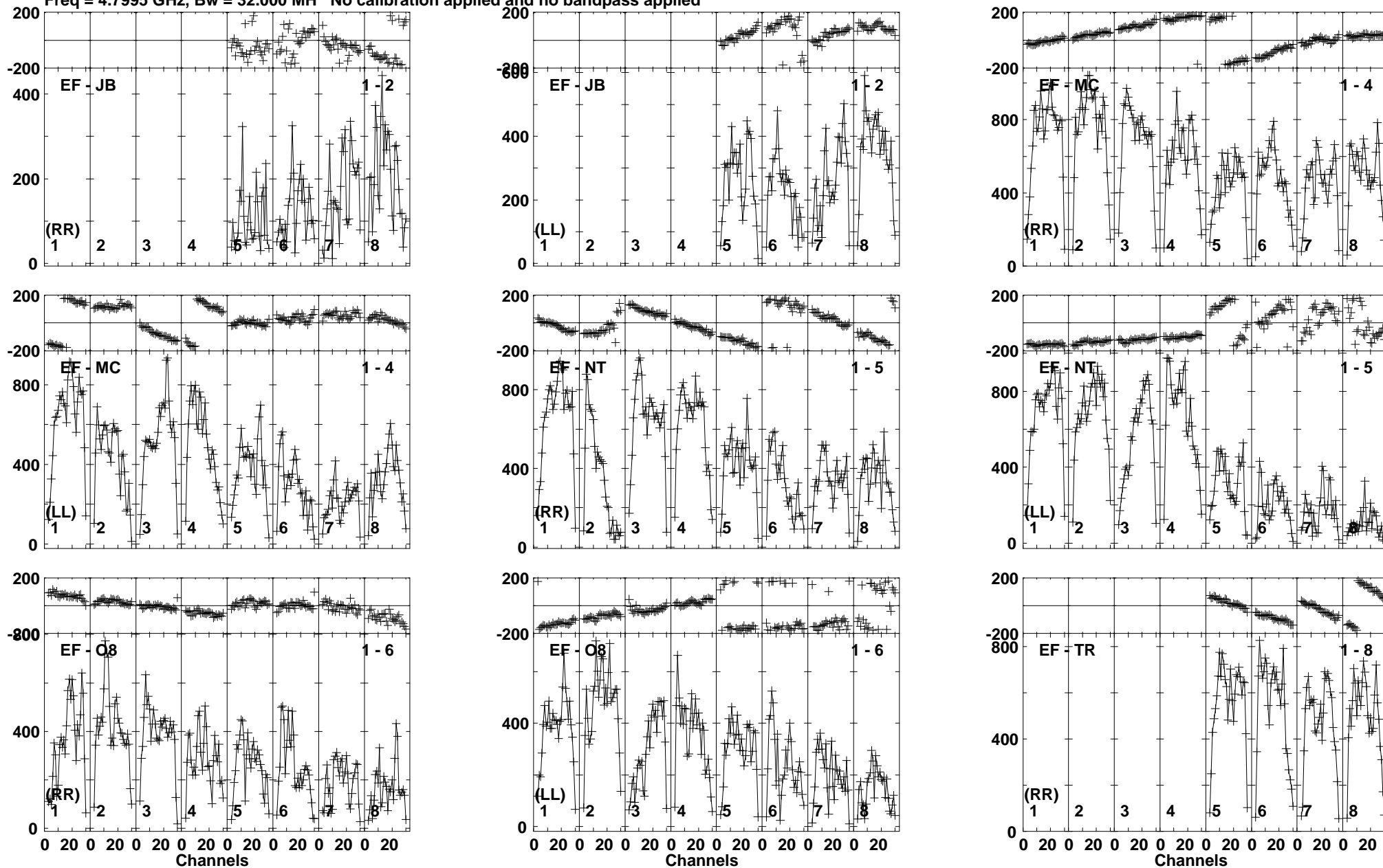
Lower frame: Micro Ampl Jy Top frame: Phas deg Vector averaged cross-power spectrum Baseline: EF (01) - JB (02) Timerange: 00/23:27:11 to 00/23:28:09
