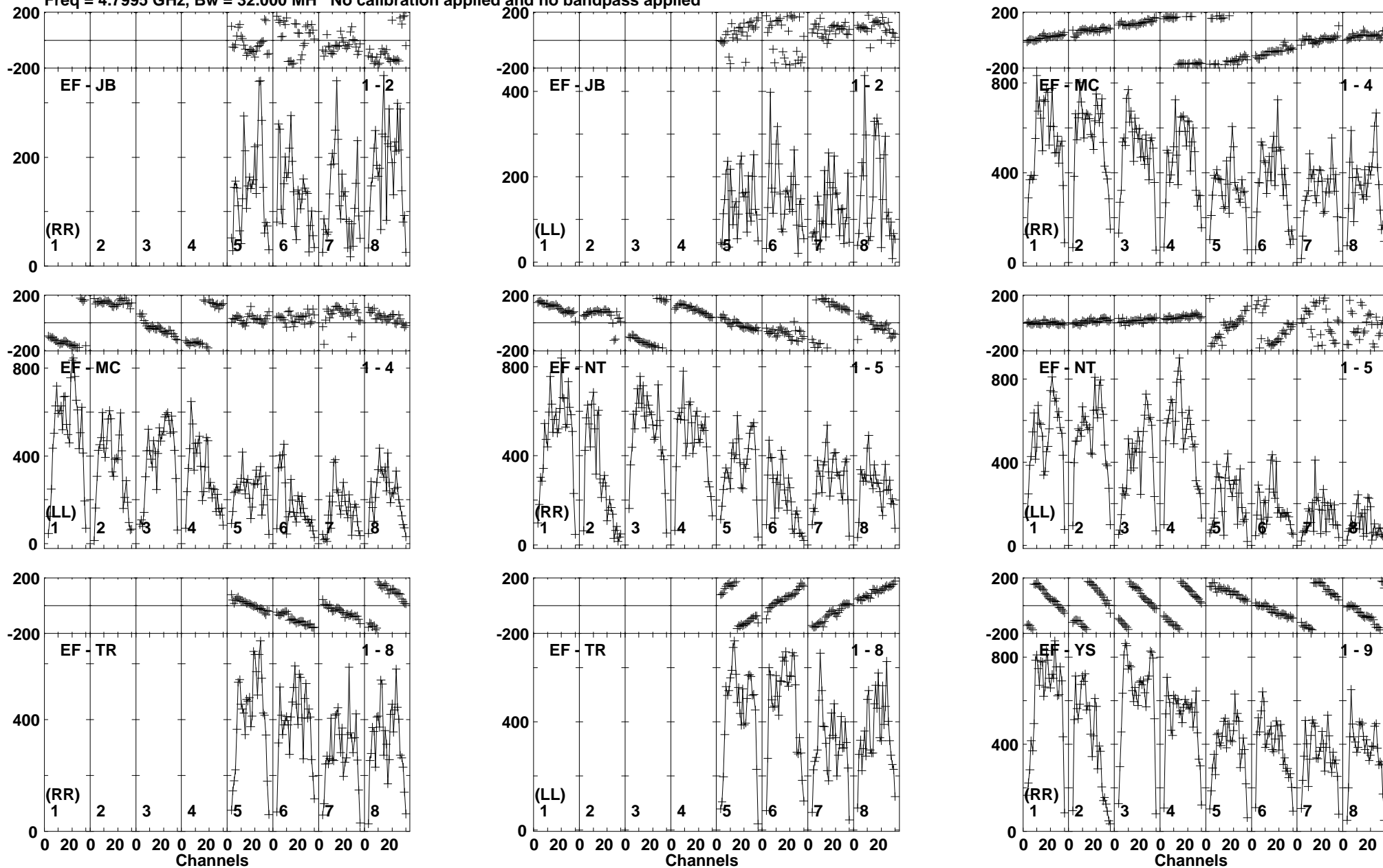
Lower frame: Micro Ampl Jy Top frame: Phas deg Vector averaged cross-power spectrum Baseline: EF (01) - JB (02) Timerange: 00/21:30:51 to 00/21:31:49
