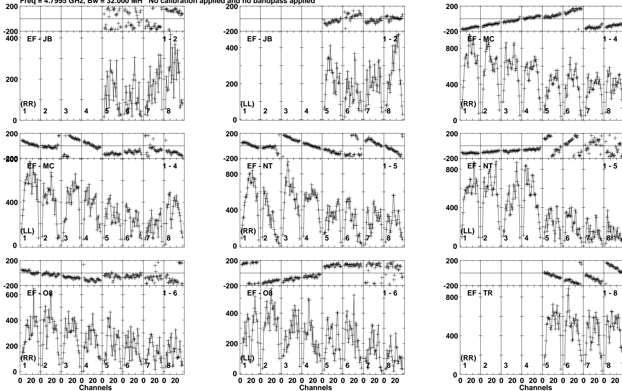
Lower frame: Micro Ampl Jy Top frame: Phas deg Vector averaged cross-power spectrum Baseline: EF (01) - JB (02) Timerange: 00:22:55:01 to 00:22:56:29
