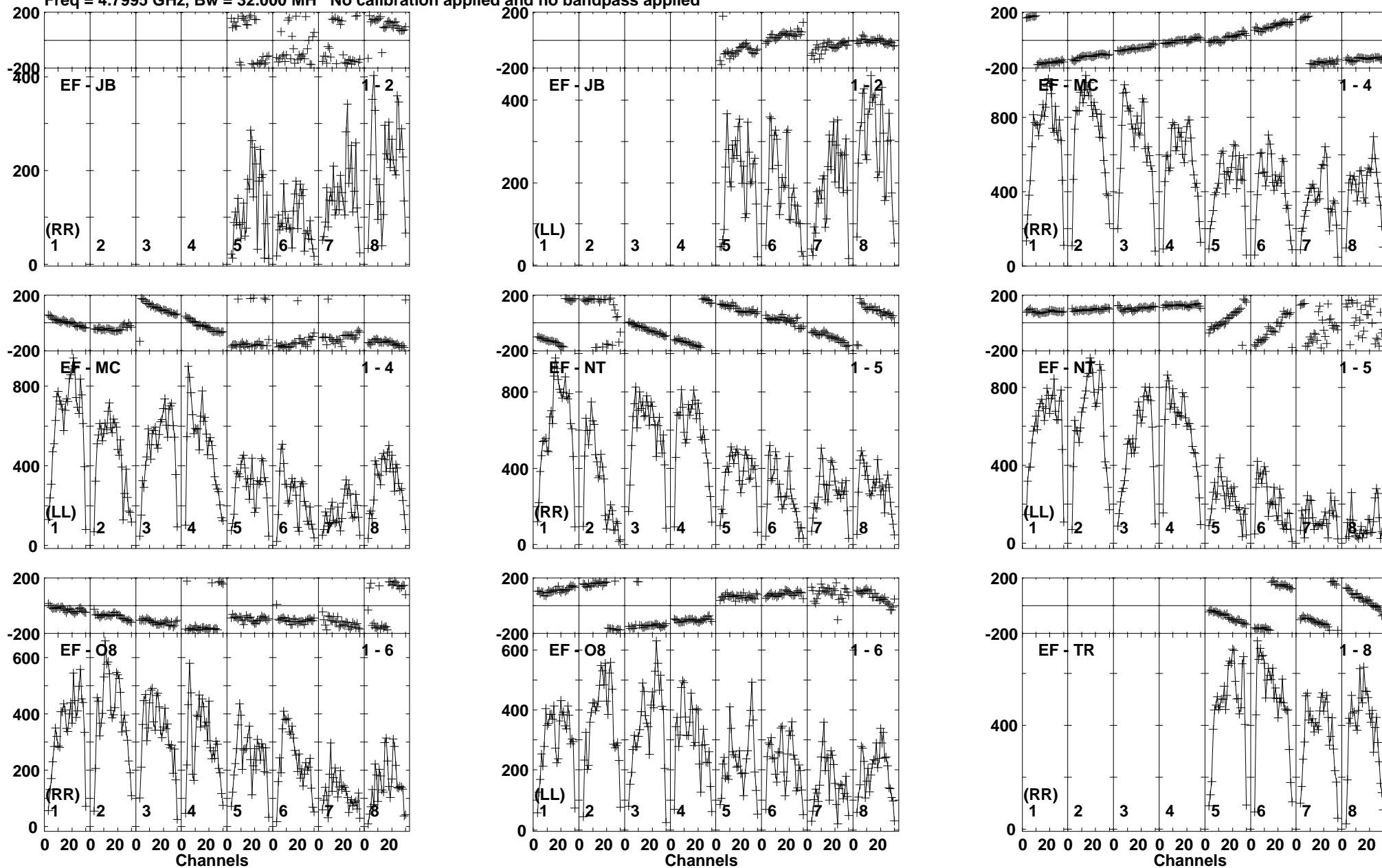
Lower frame: Micro Ampl Jy Top frame: Phas deg Vector averaged cross-power spectrum Baseline: EF (01) - JB (02) Timerange: 00/23:10:01 to 00/23:11:59
