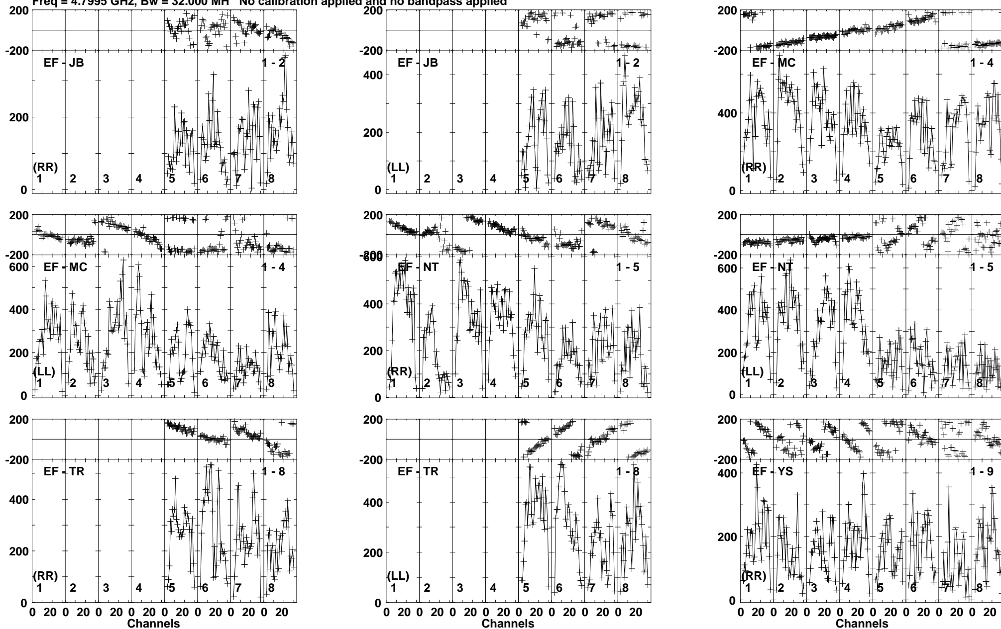
Lower frame: Micro Ampl Jy Top frame: Phas deg Vector averaged cross-power spectrum Baseline: EF (01) - JB (02) Timerange: 01/01:16:11 to 01/01:17:09
