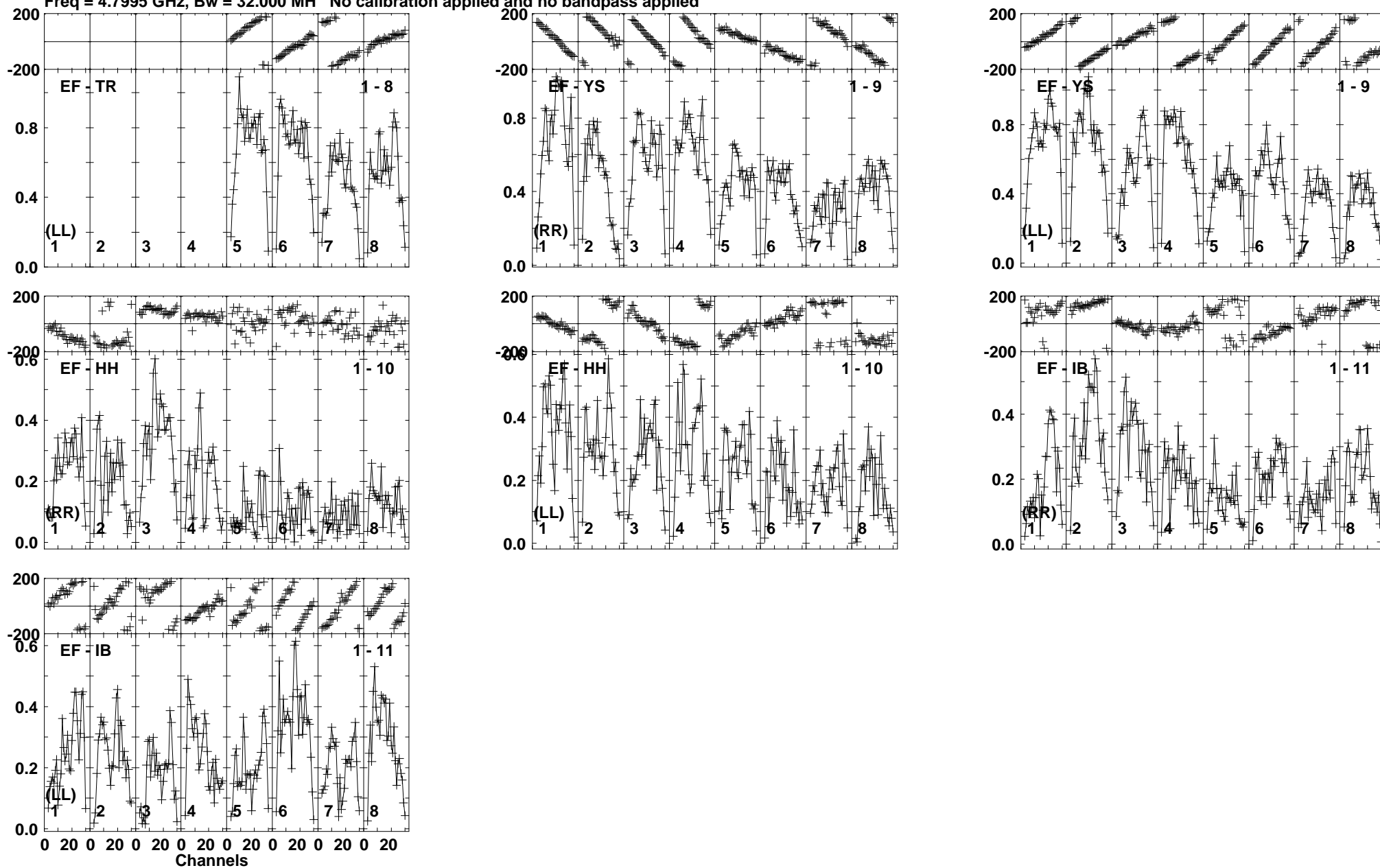
Lower frame: Milli Ampl Jy Top frame: Phas deg Vector averaged cross-power spectrum Baseline: EF (01) - TR (08) Timerange: 00/23:19:01 to 00/23:19:59
