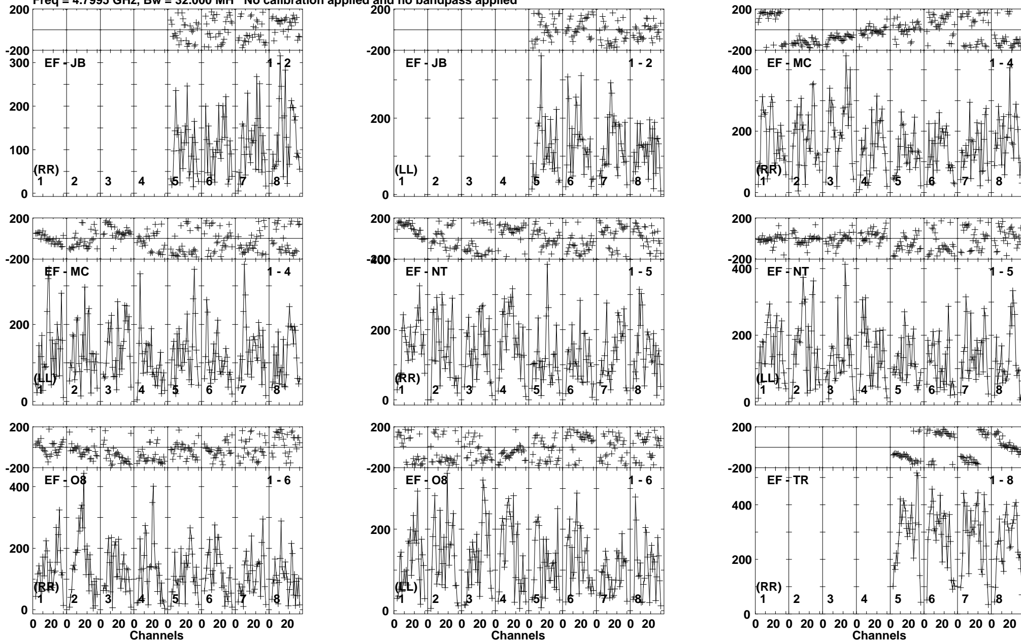
Lower frame: Micro Ampl Jy Top frame: Phas deg Vector averaged cross-power spectrum Baseline: EF (01) - JB (02) Timerange: 00:22:51:31 to 00:22:52:29
