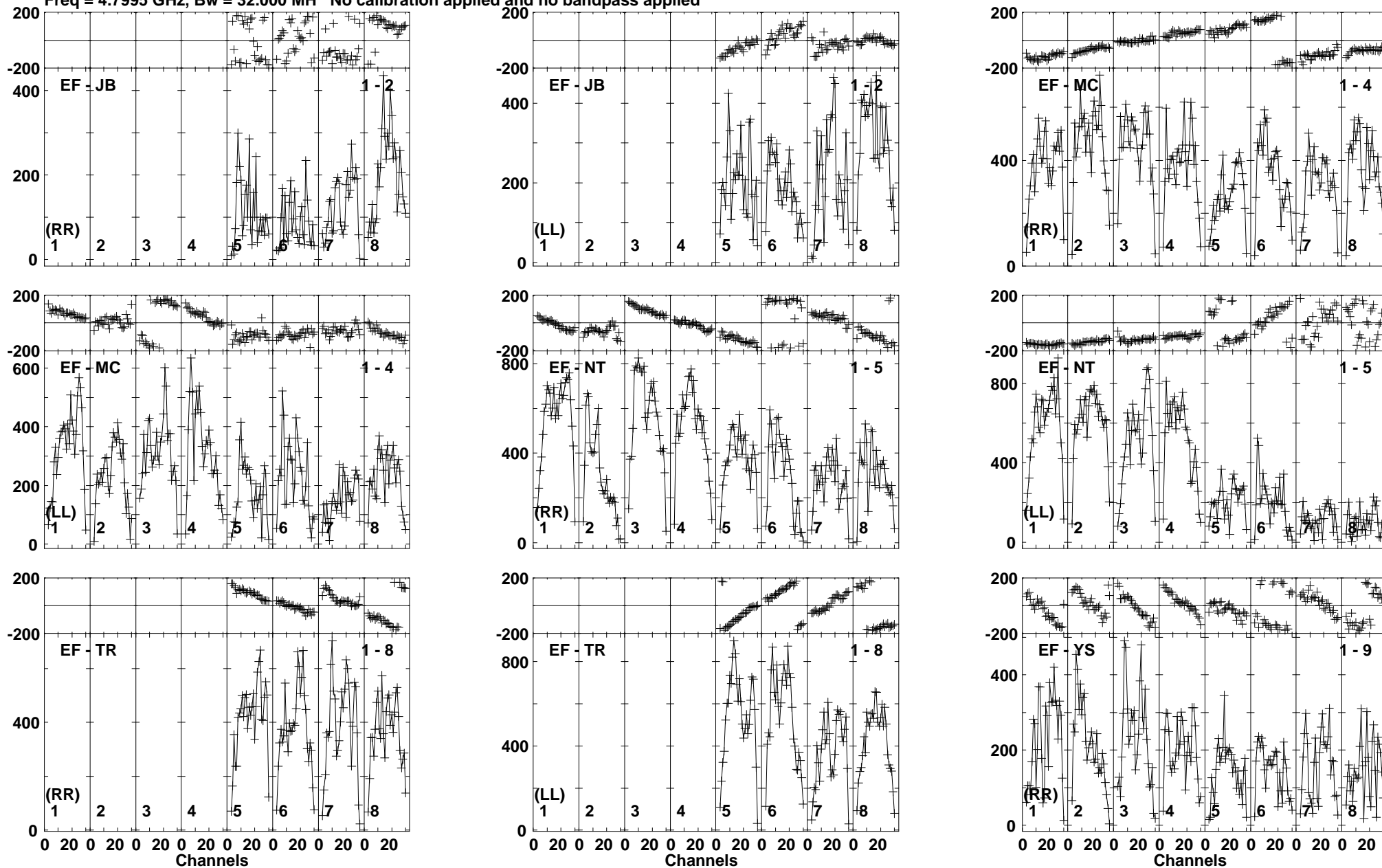
Lower frame: Micro Ampl Jy Top frame: Phas deg Vector averaged cross-power spectrum Baseline: EF (01) - JB (02) Timerange: 01/01:08:01 to 01/01:08:59
