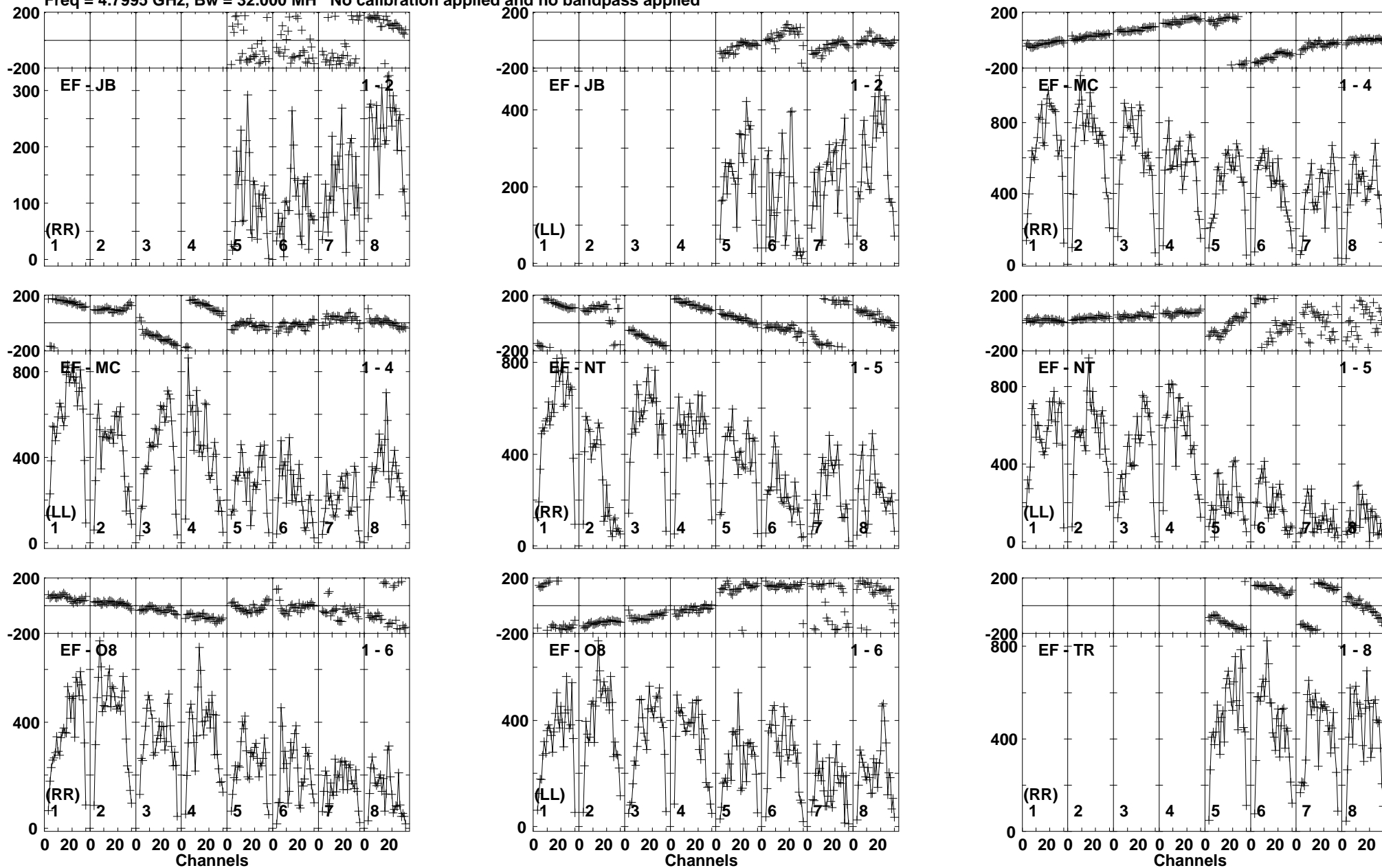
Lower frame: Micro Ampl Jy Top frame: Phas deg Vector averaged cross-power spectrum Baseline: EF (01) - JB (02) Timerange: 00/22:22:41 to 00/22:24:09
