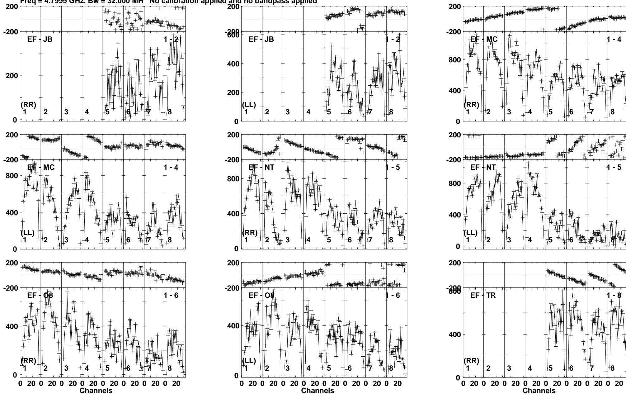
Lower frame: Micro Ampl Jy Top frame: Phas deg Vector averaged cross-power spectrum Baseline: EF (01) - JB (02) Timerange: 00:22:43:31 to 00:22:44:29
