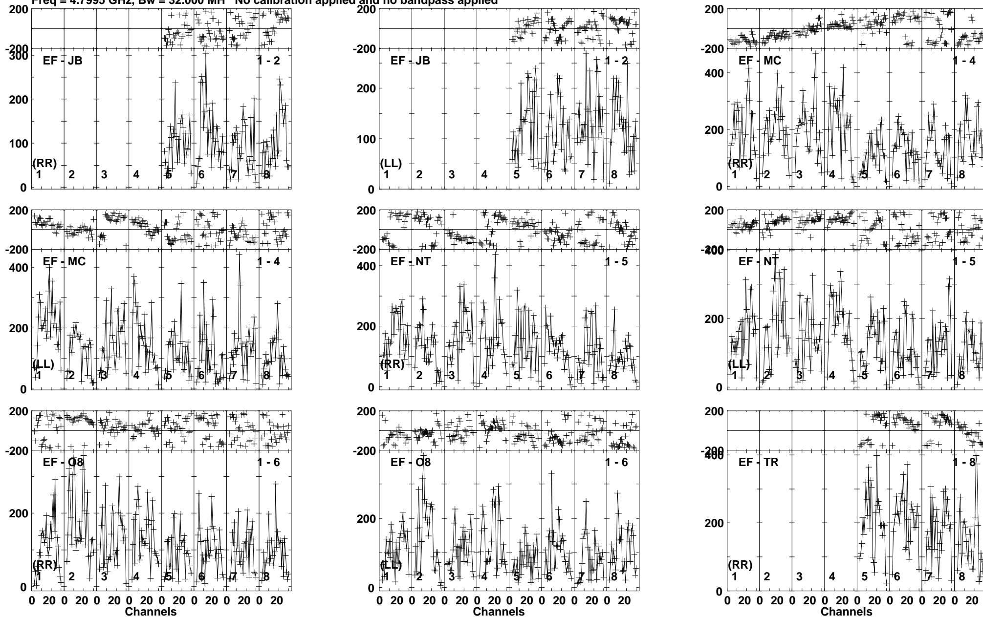
Lower frame: Micro Ampl Jy Top frame: Phas deg Vector averaged cross-power spectrum Baseline: EF (01) - JB (02) Timerange: 00/21:34:21 to 00/21:35:49
