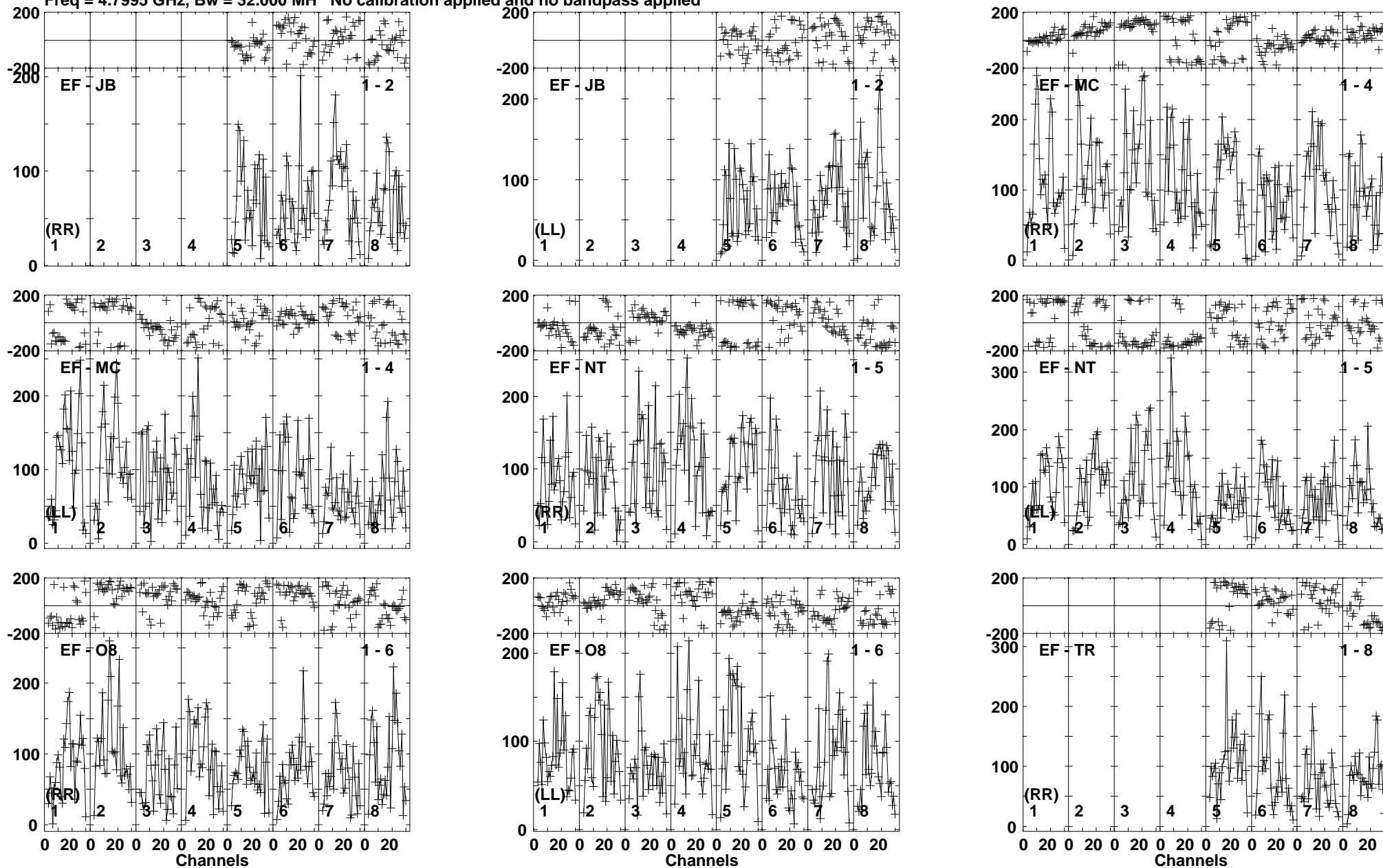
Lower frame: Micro Ampl Jy Top frame: Phas deg Vector averaged cross-power spectrum Baseline: EF (01) - JB (02) Timerange: 01/00:16:31 to 01/00:18:59
