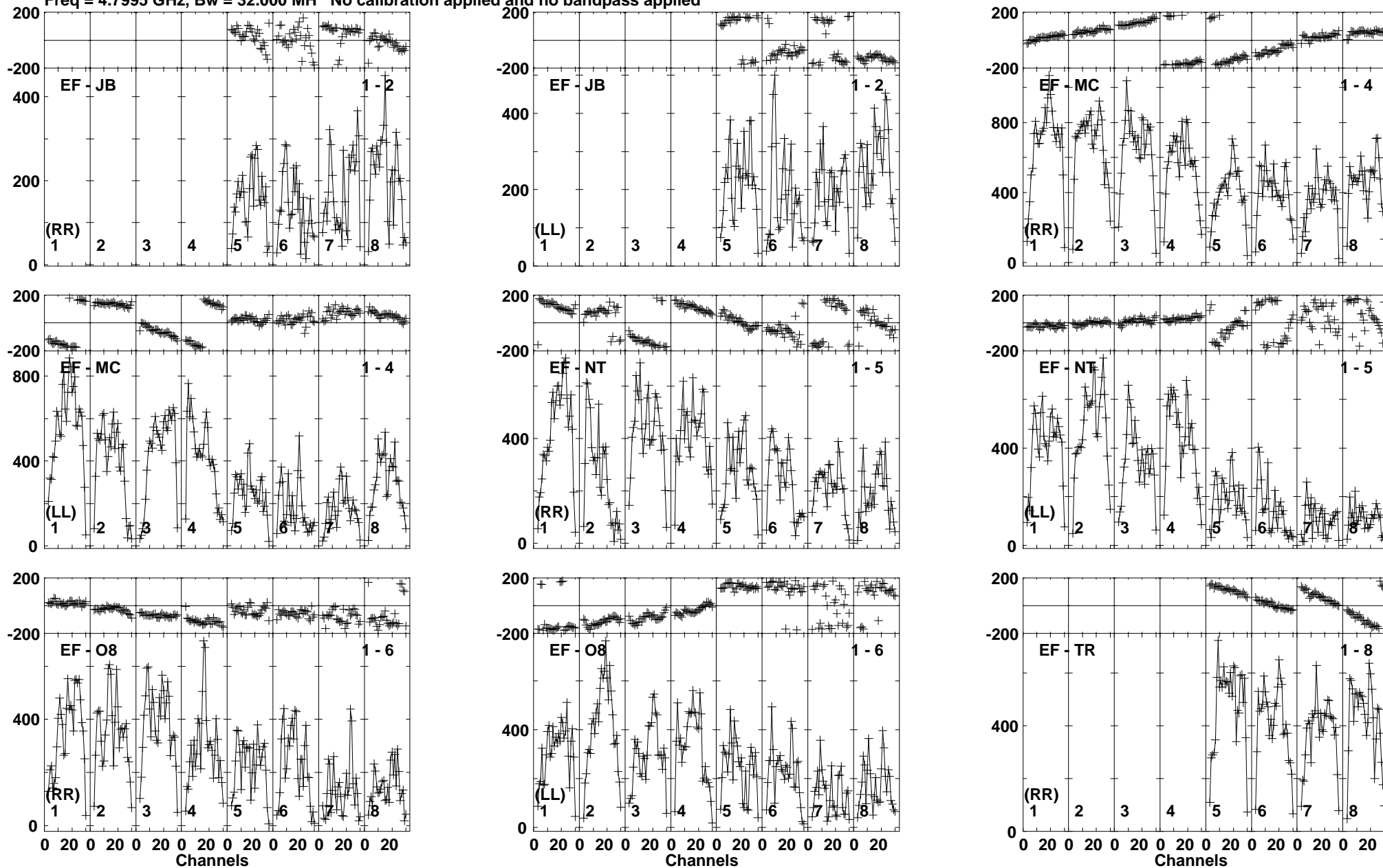
Lower frame: Micro Ampl Jy Top frame: Phas deg Vector averaged cross-power spectrum Baseline: EF (01) - JB (02) Timerange: 01/00:03:31 to 01/00:04:29
