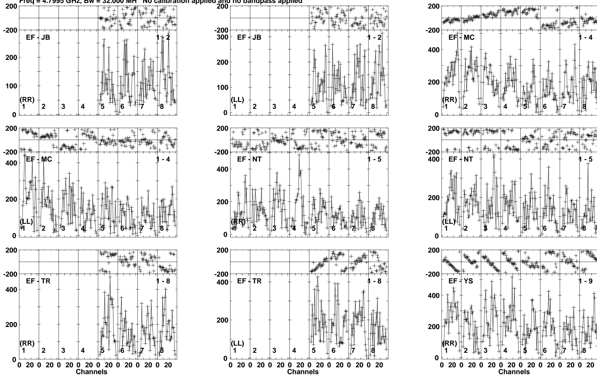
Lower frame: Micro Ampl Jy Top frame: Phas deg Vector averaged cross-power spectrum Baseline: EF (01) - JB (02) Timerange: 00/21:22:41 to 00/21:23:39
