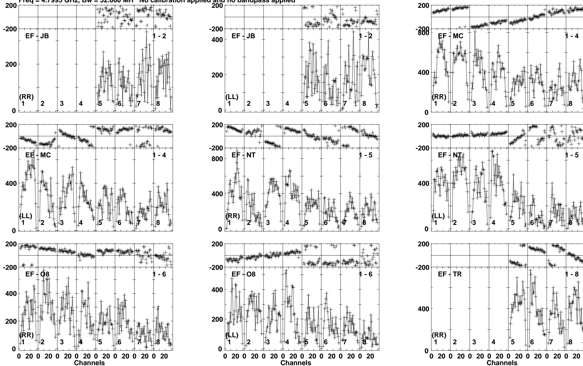
Lower frame: Micro Ampl Jy Top frame: Phas deg Vector averaged cross-power spectrum Baseline: EF (01) - JB (02) Timerange: 00/21:54:31 to 00/21:55:59
