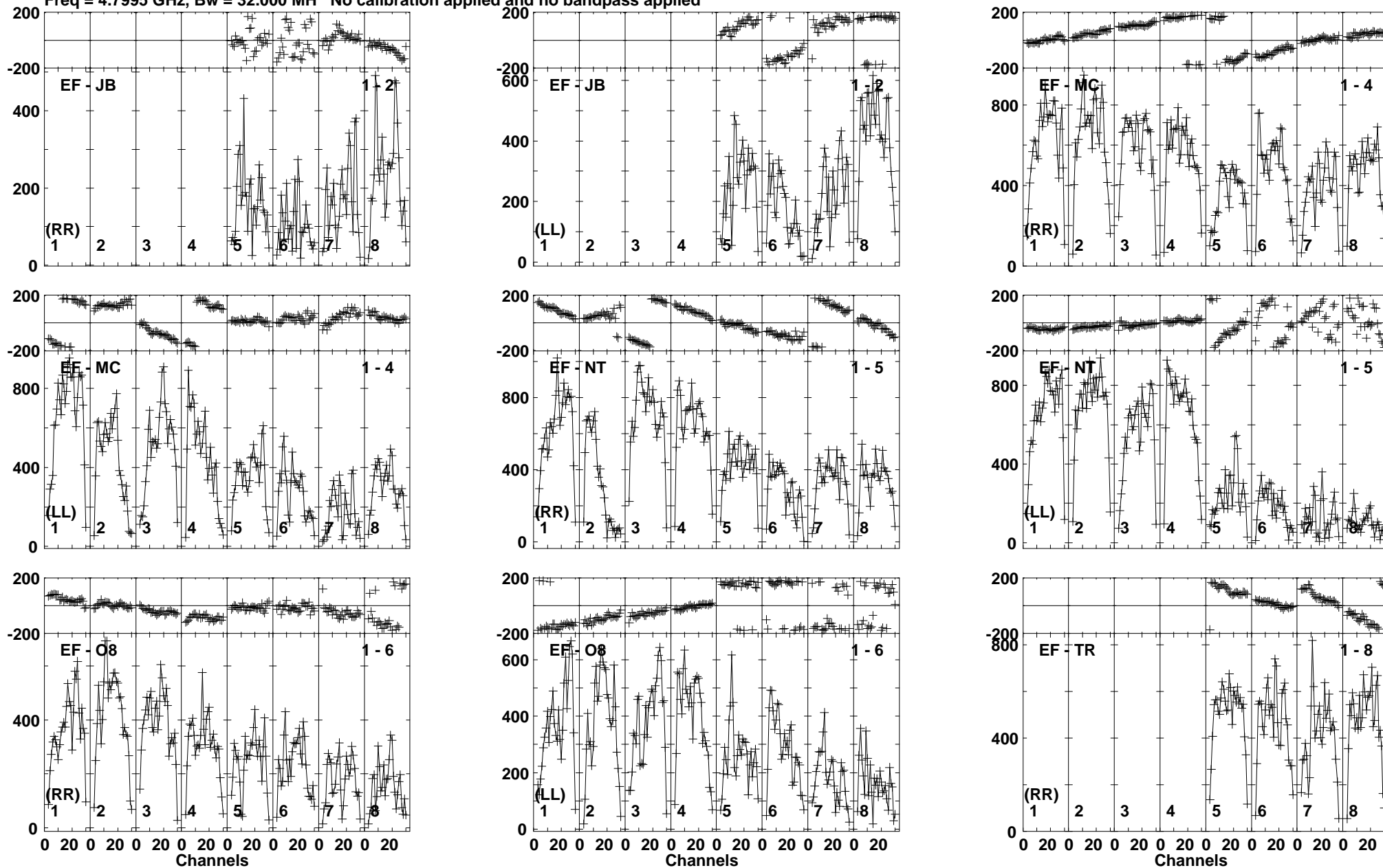
Lower frame: Micro Ampl Jy Top frame: Phas deg Vector averaged cross-power spectrum Baseline: EF (01) - JB (02) Timerange: 00/23:47:21 to 00/23:48:19
