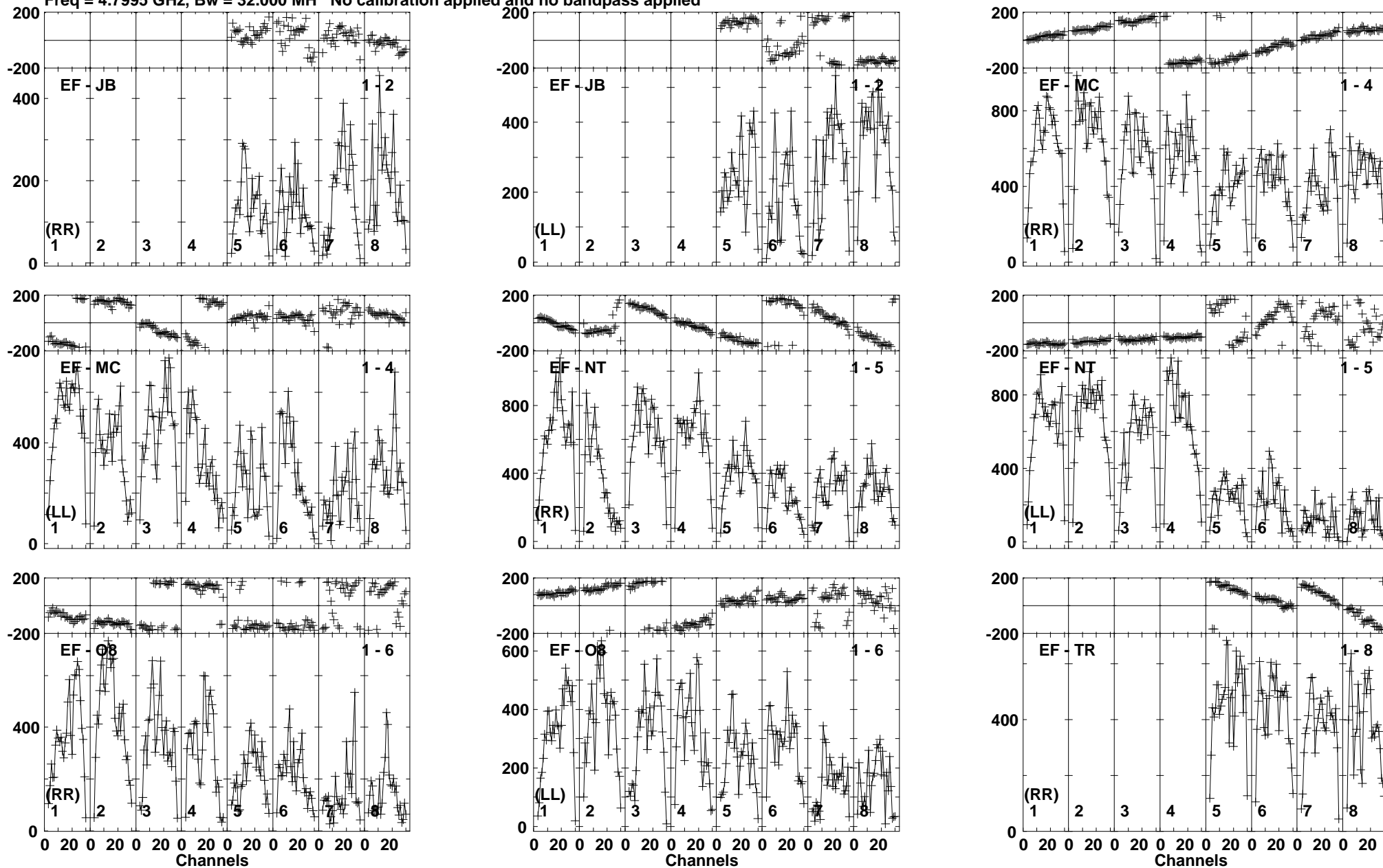
Lower frame: Micro Ampl Jy Top frame: Phas deg Vector averaged cross-power spectrum Baseline: EF (01) - JB (02) Timerange: 01/00:19:01 to 01/00:20:29
