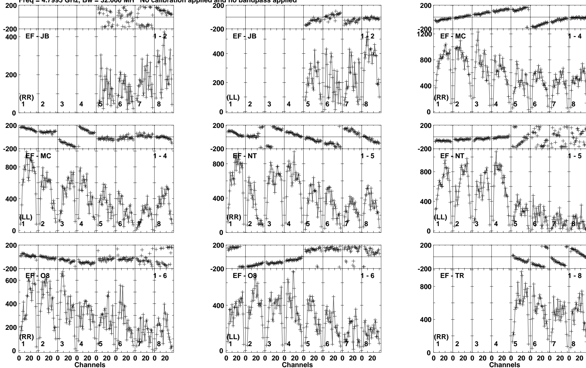
Lower frame: Micro Ampl Jy Top frame: Phas deg Vector averaged cross-power spectrum Baseline: EF (01) - JB (02) Timerange: 00/22:35:21 to 00/22:36:19
