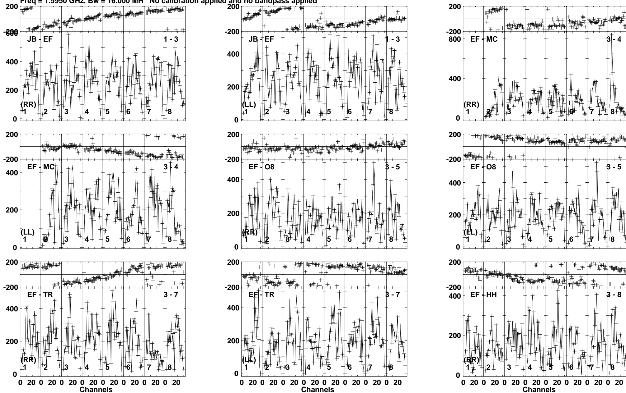
Lower frame: Micro Ampl Jy Top frame: Phas deg Vector averaged cross-power spectrum Baseline: JB (01) - EF (03) Timerange: 00/20:24:01 to 00/20:26:29
