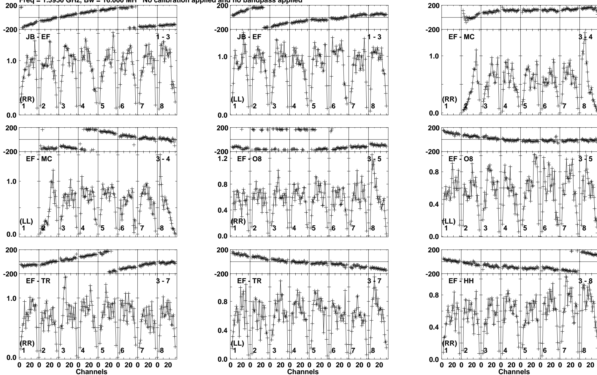
Lower frame: Milli Ampl Jy Top frame: Phas deg Vector averaged cross-power spectrum Baseline: JB (01) - EF (03) Timerange: 00/21:22:51 to 00/21:23:49
