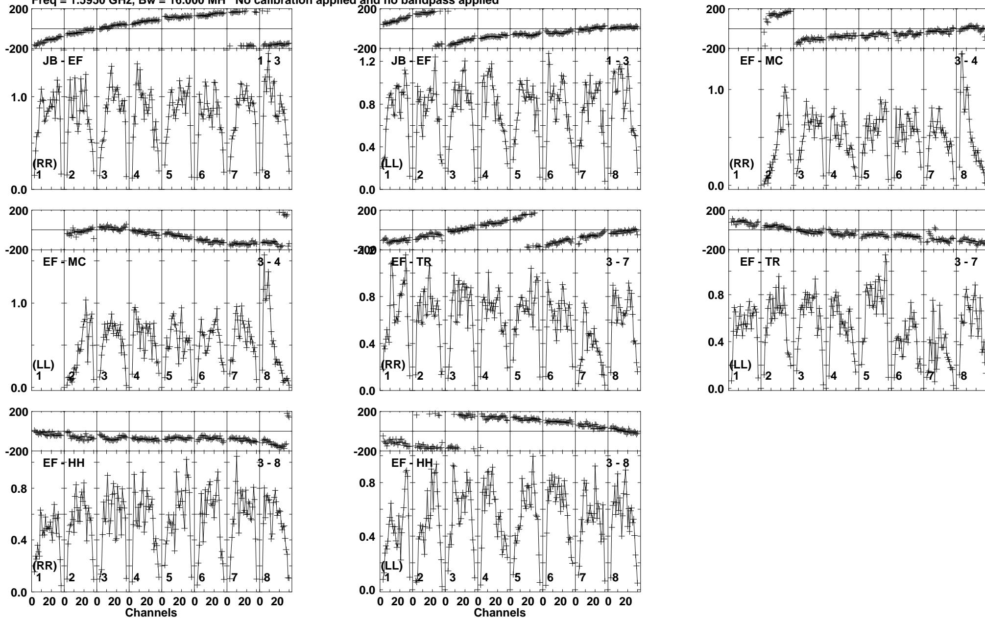
Lower frame: Milli Ampl Jy Top frame: Phas deg Vector averaged cross-power spectrum Baseline: JB (01) - EF (03) Timerange: 00:22:18:51 to 00:22:20:19
