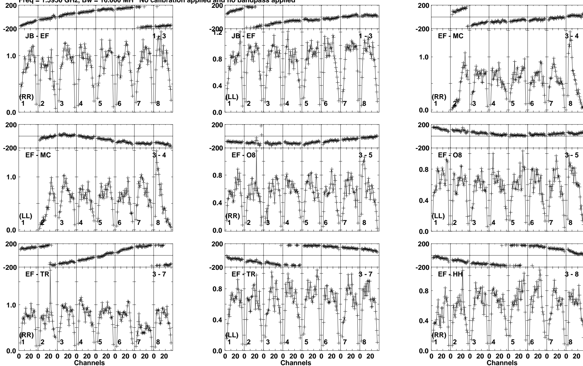
Lower frame: Milli Ampl Jy Top frame: Phas deg Vector averaged cross-power spectrum Baseline: JB (01) - EF (03) Timerange: 00/20:37:31 to 00/20:39:29
