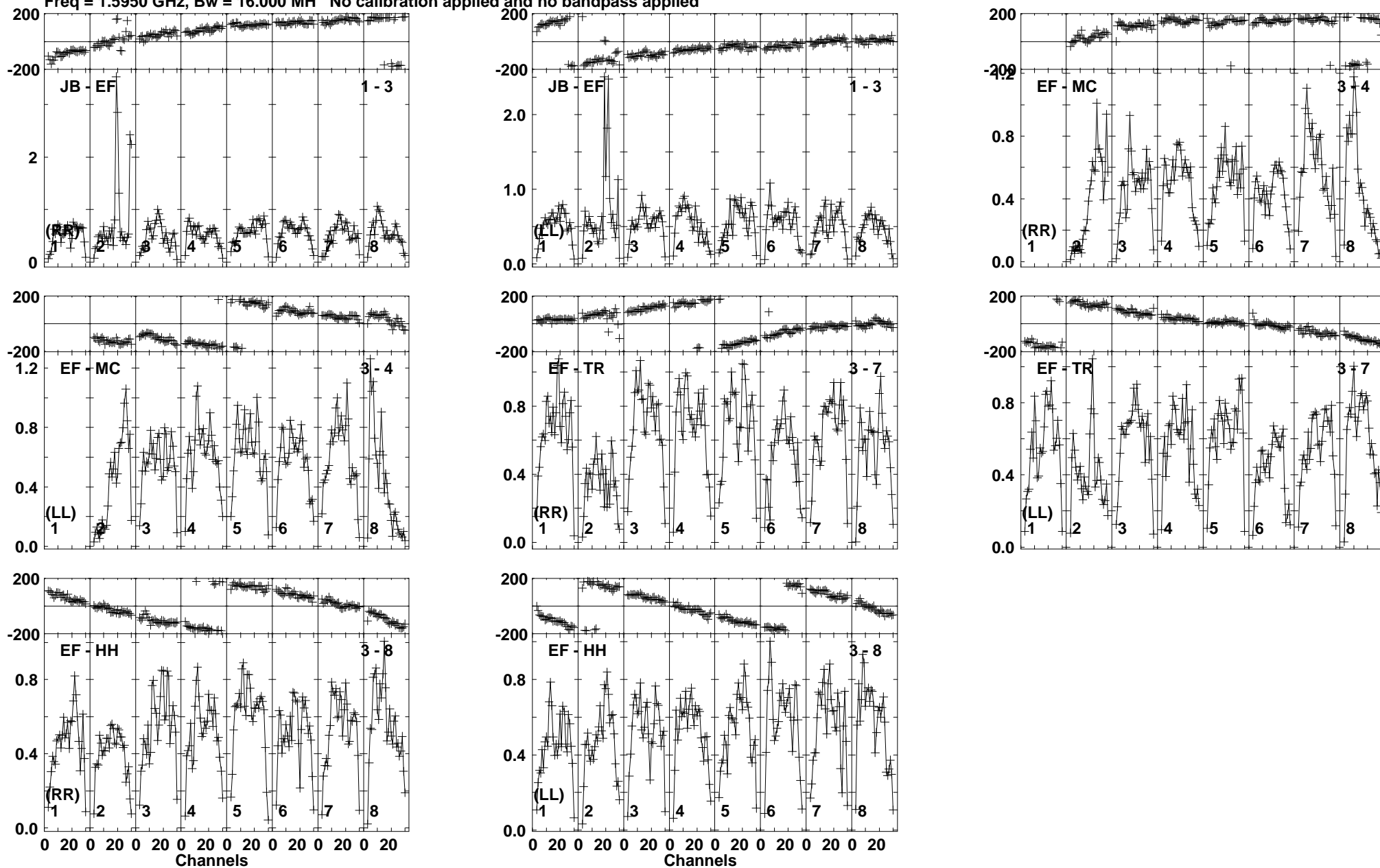
Lower frame: Milli Ampl Jy Top frame: Phas deg Vector averaged cross-power spectrum Baseline: JB (01) - EF (03) Timerange: 00:18:58:21 to 00:18:59:19
