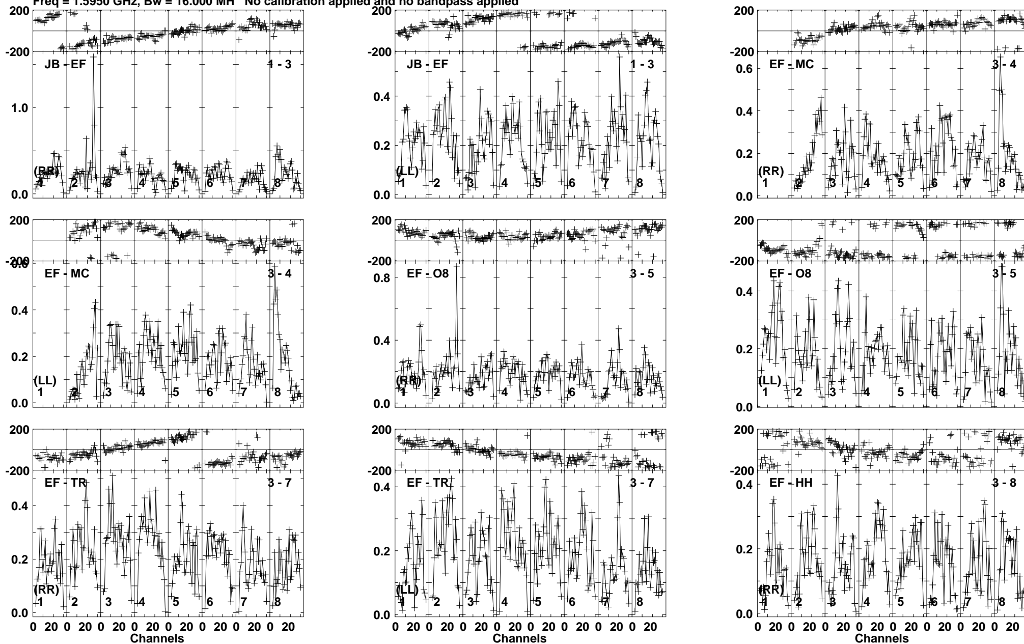
Lower frame: Milli Ampl Jy Top frame: Phas deg Vector averaged cross-power spectrum Baseline: JB (01) - EF (03) Timerange: 00/20:07:51 to 00/20:10:19
