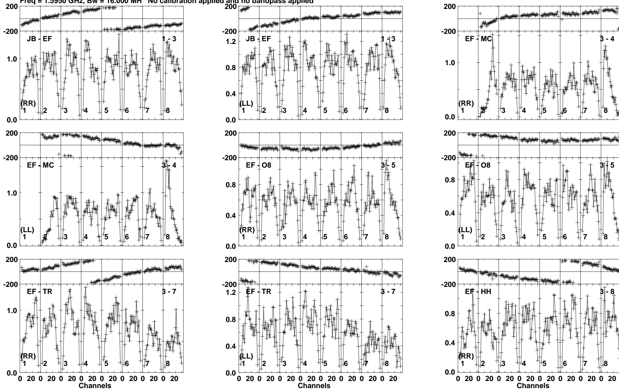
Lower frame: Milli Ampl Jy Top frame: Phas deg Vector averaged cross-power spectrum Baseline: JB (01) - EF (03) Timerange: 00/20:14:31 to 00/20:15:59
