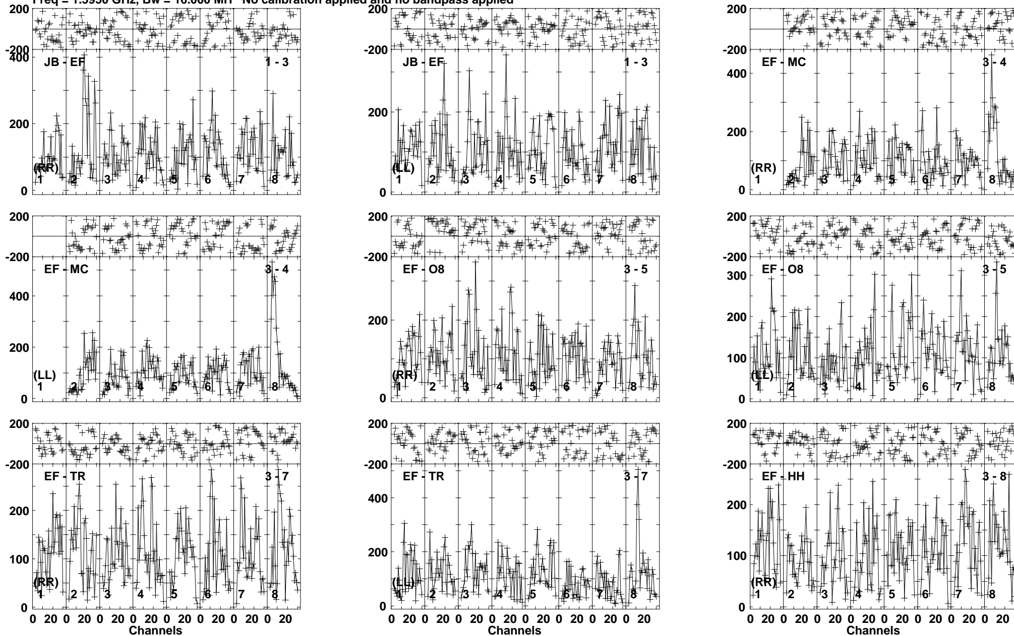
Lower frame: Micro Ampl Jy Top frame: Phas deg Vector averaged cross-power spectrum Baseline: JB (01) - EF (03) Timerange: 00/20:43:31 to 00/20:45:59
