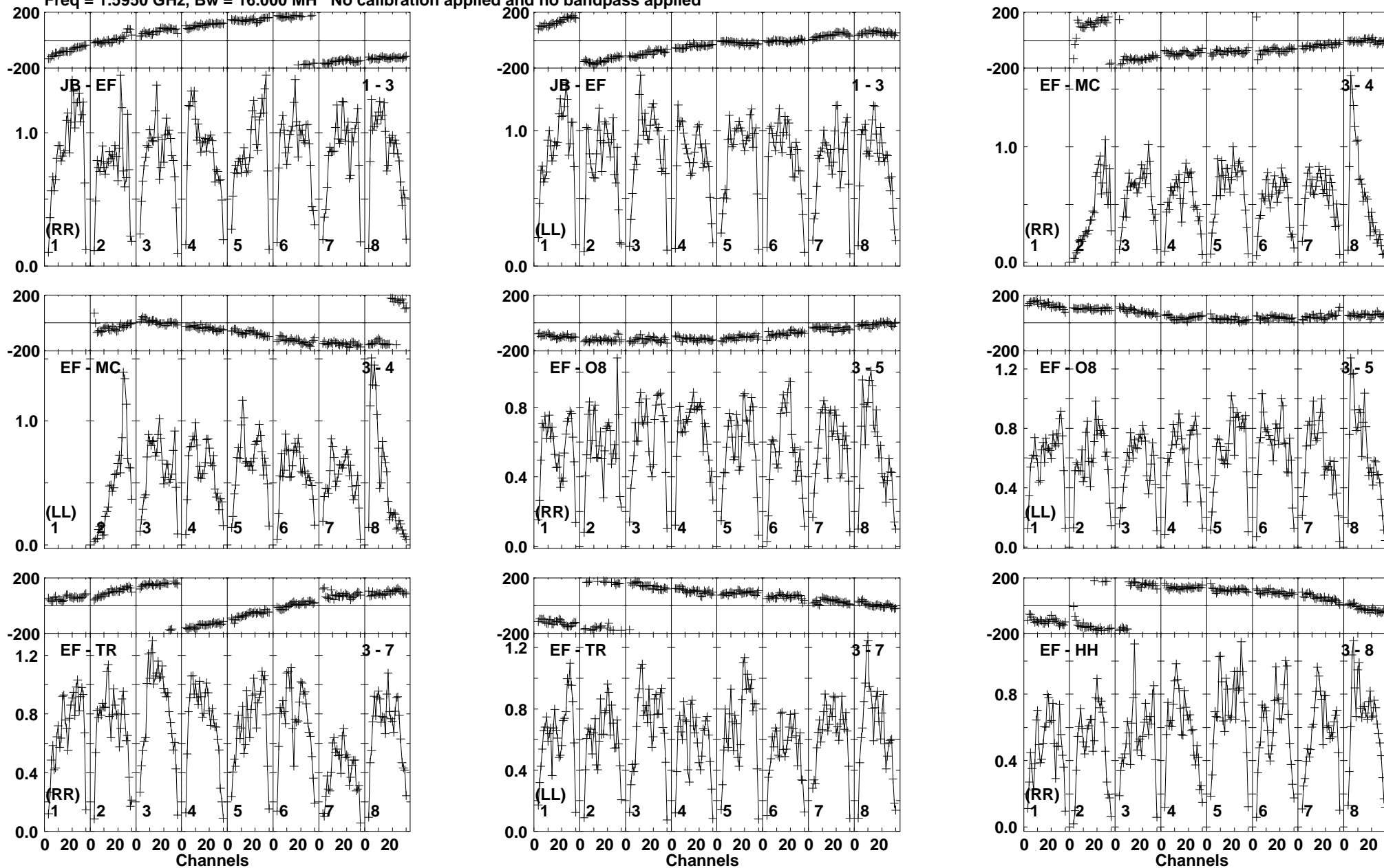
Lower frame: Milli Ampl Jy Top frame: Phas deg Vector averaged cross-power spectrum Baseline: JB (01) - EF (03) Timerange: 00/20:46:31 to 00/20:47:29
