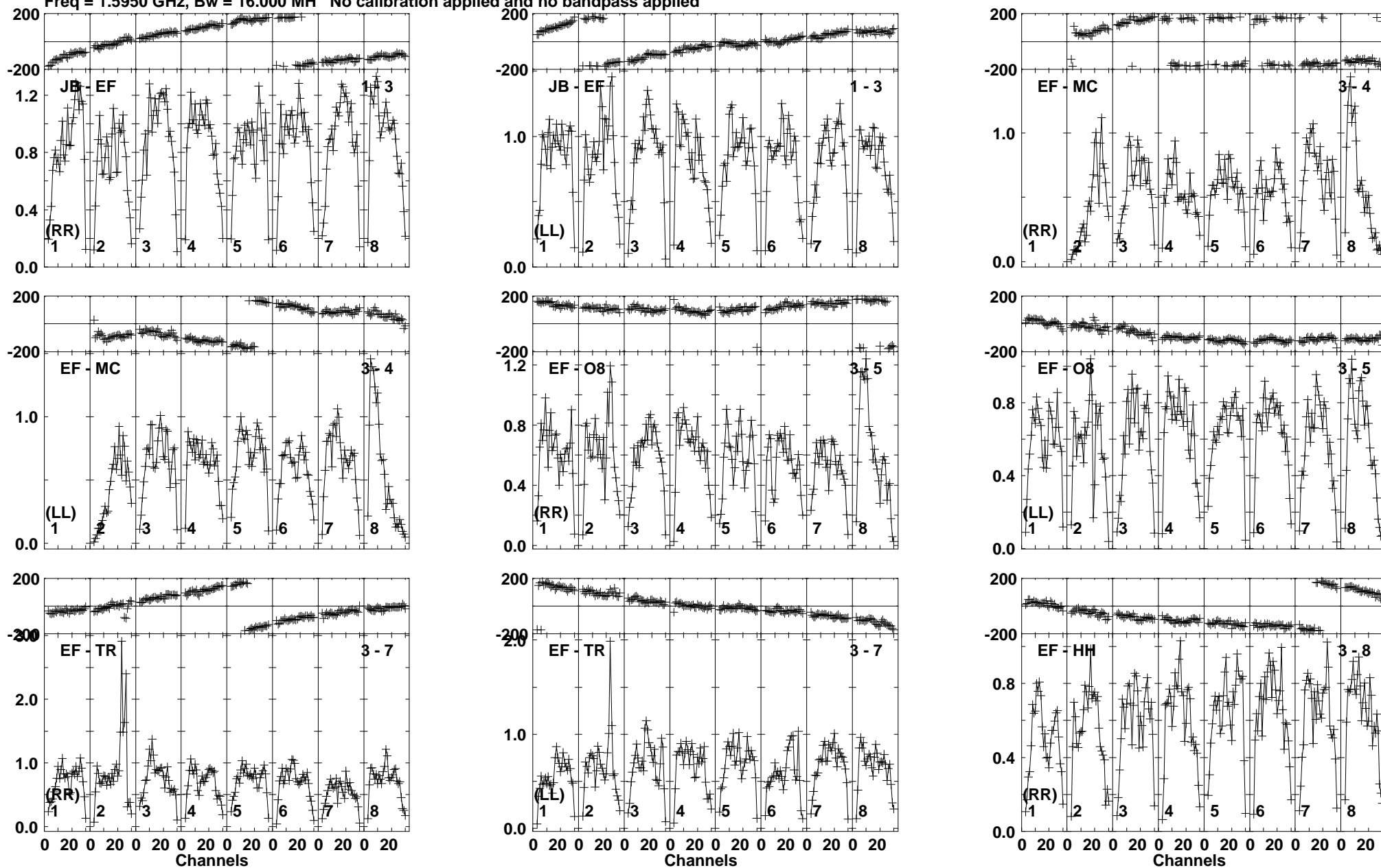
Lower frame: Milli Ampl Jy Top frame: Phas deg Vector averaged cross-power spectrum Baseline: JB (01) - EF (03) Timerange: 00/21:14:51 to 00/21:15:49
