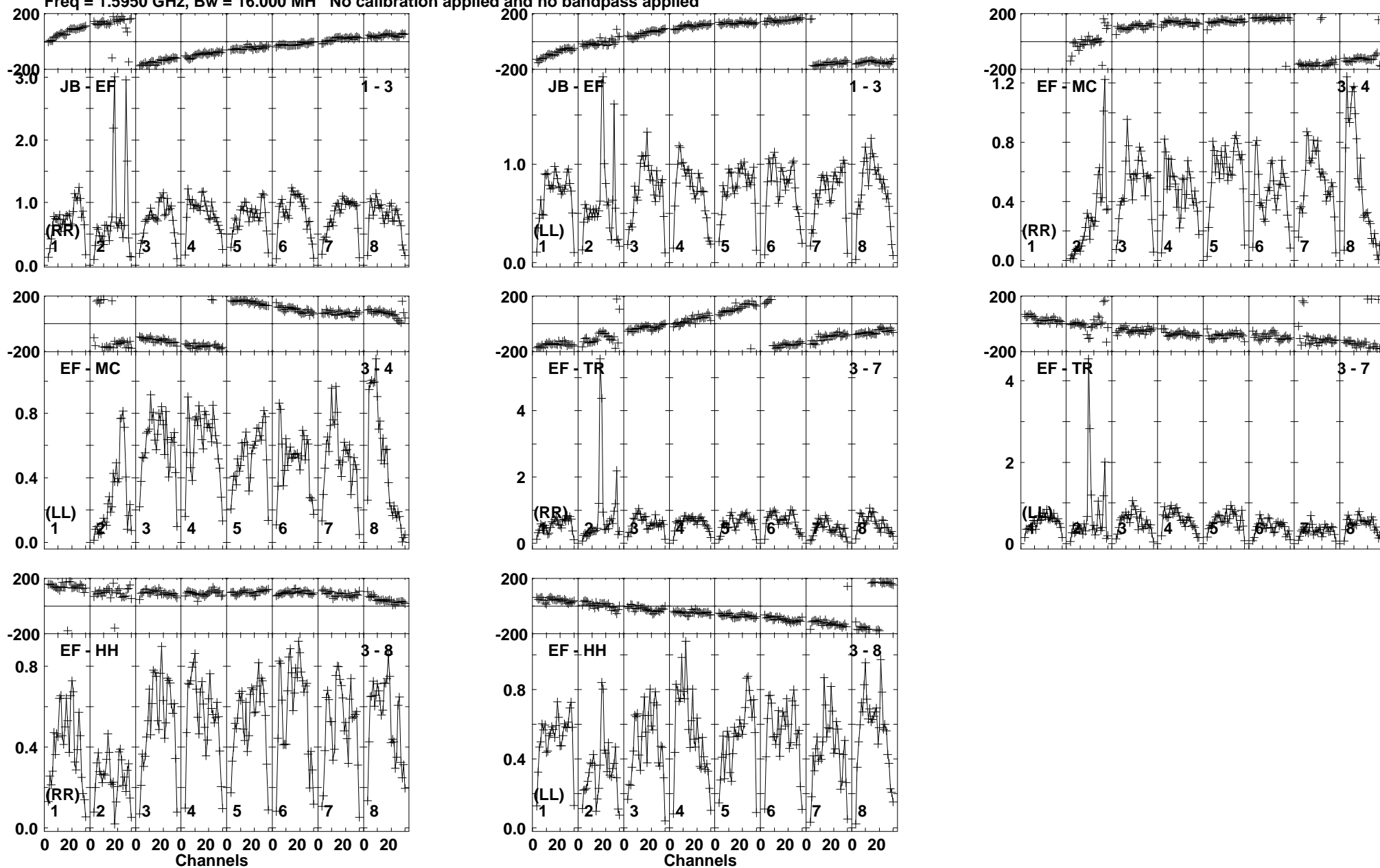
Lower frame: Milli Ampl Jy Top frame: Phas deg Vector averaged cross-power spectrum Baseline: JB (01) - EF (03) Timerange: 00/22:22:51 to 00/22:24:19
