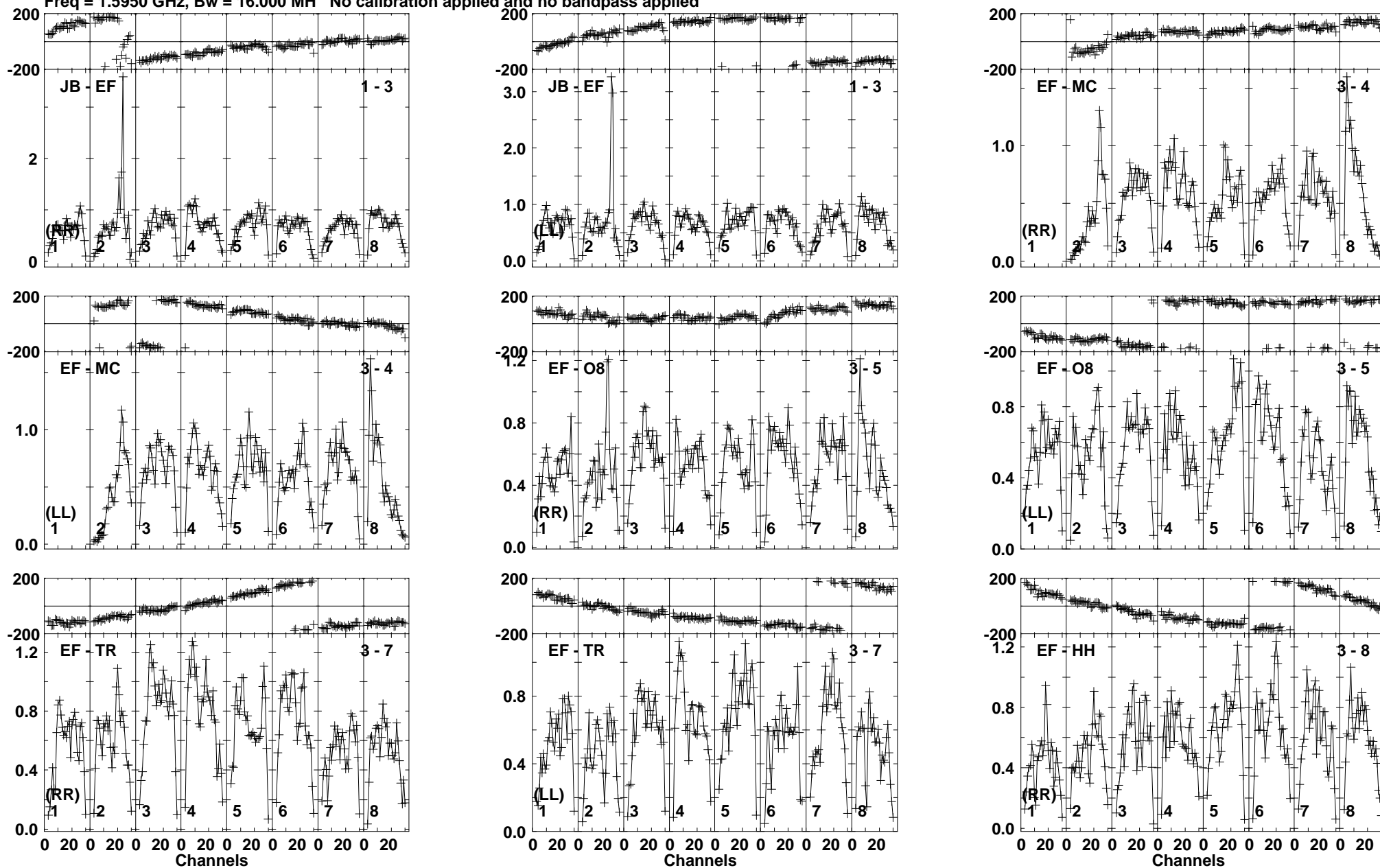
Lower frame: Milli Ampl Jy Top frame: Phas deg Vector averaged cross-power spectrum Baseline: JB (01) - EF (03) Timerange: 00/19:26:31 to 00/19:27:29
