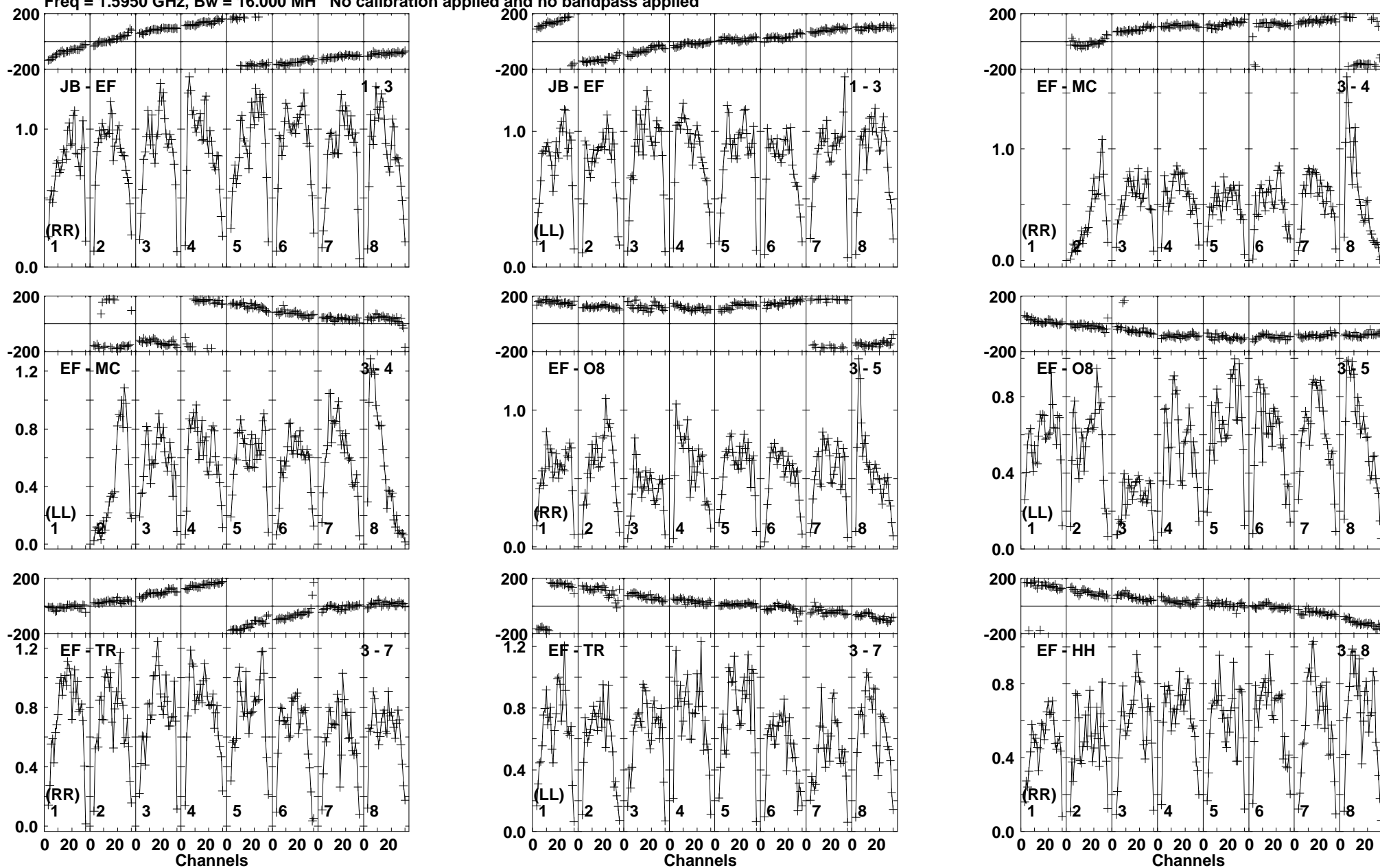
Lower frame: Milli Ampl Jy Top frame: Phas deg Vector averaged cross-power spectrum Baseline: JB (01) - EF (03) Timerange: 00/20:58:11 to 00/20:59:39
