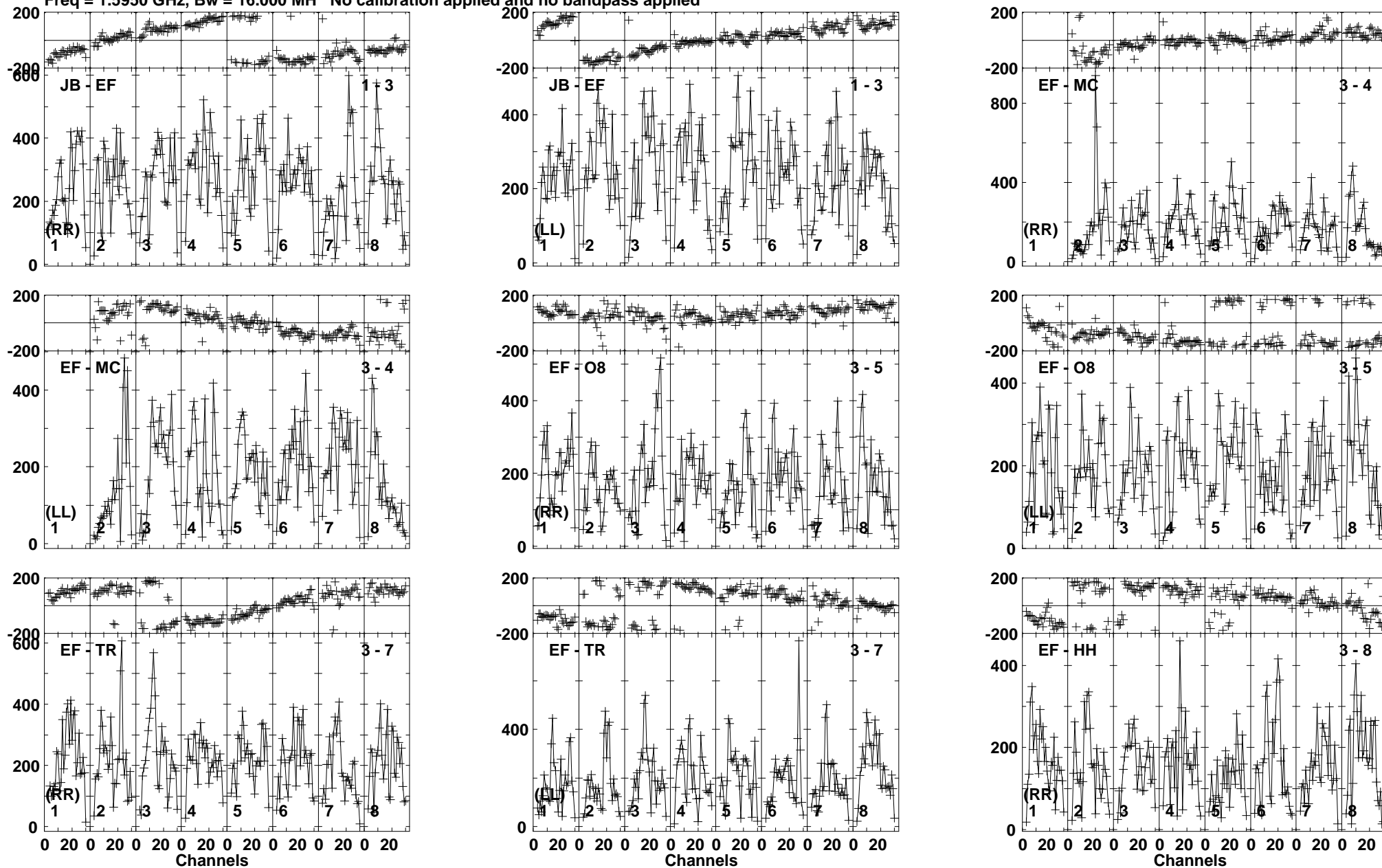
Lower frame: Micro Ampl Jy Top frame: Phas deg Vector averaged cross-power spectrum Baseline: JB (01) - EF (03) Timerange: 00/21:07:41 to 00/21:10:09
