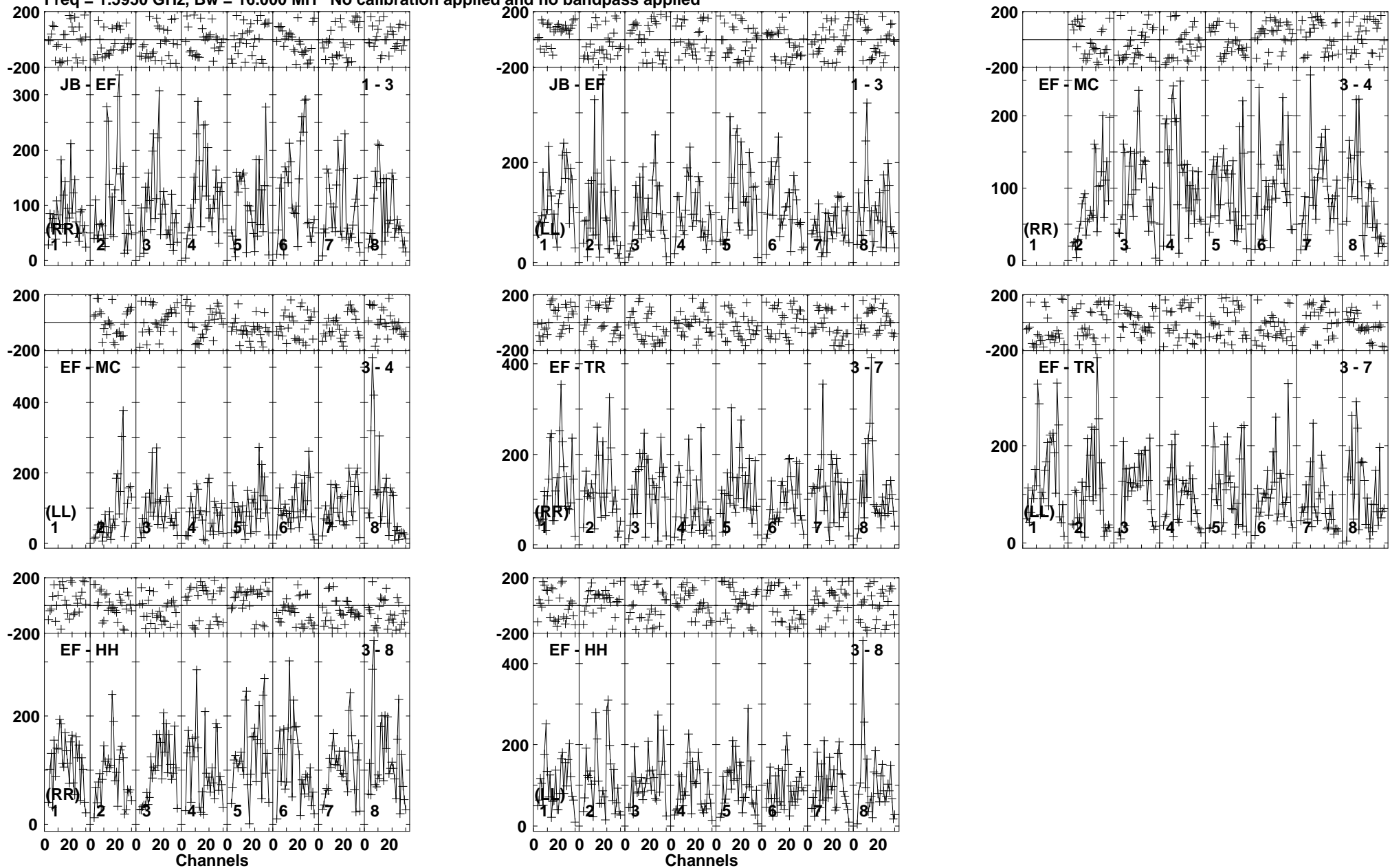
Lower frame: Micro Ampl Jy Top frame: Phas deg Vector averaged cross-power spectrum Baseline: JB (01) - EF (03) Timerange: 00/22:36:31 to 00/22:38:59
