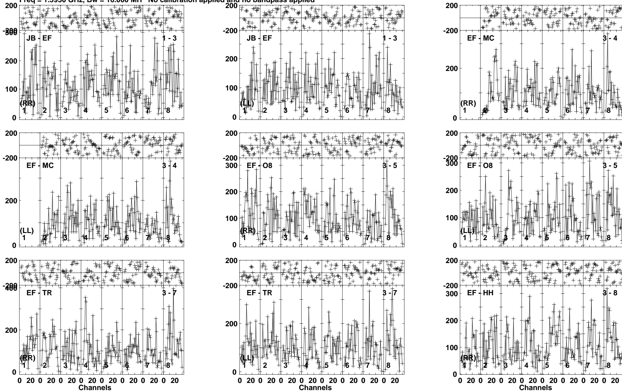
Lower frame: Micro Ampl Jy Top frame: Phas deg Vector averaged cross-power spectrum Baseline: JB (01) - EF (03) Timerange: 00:21:32:01 to 00:21:34:29
