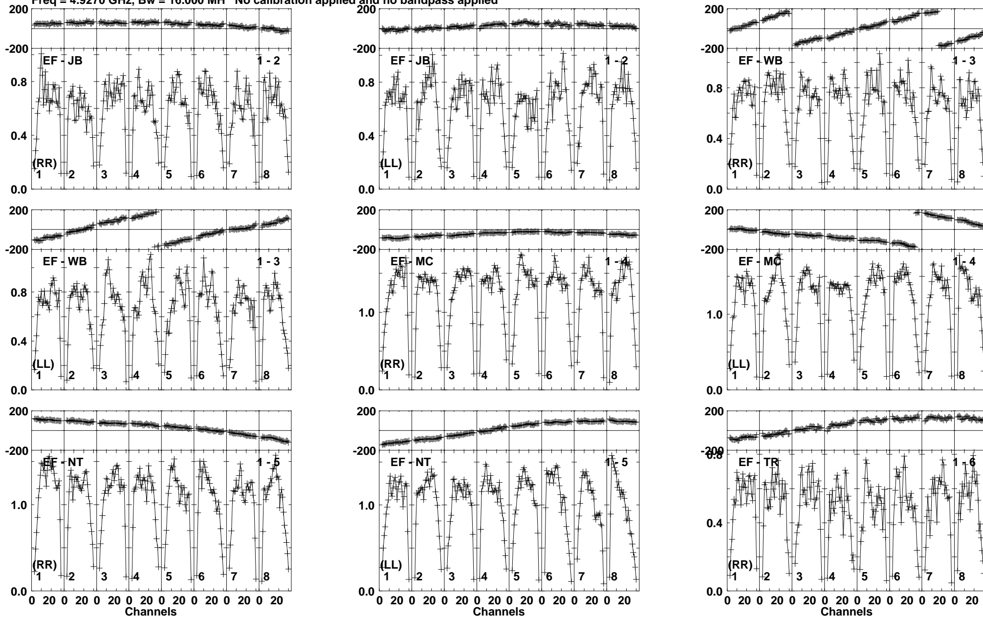
Lower frame: Milli Ampl Jy Top frame: Phas deg Vector averaged cross-power spectrum Baseline: EF (01) - JB (02) Timerange: 00/20:36:51 to 00/20:39:19
