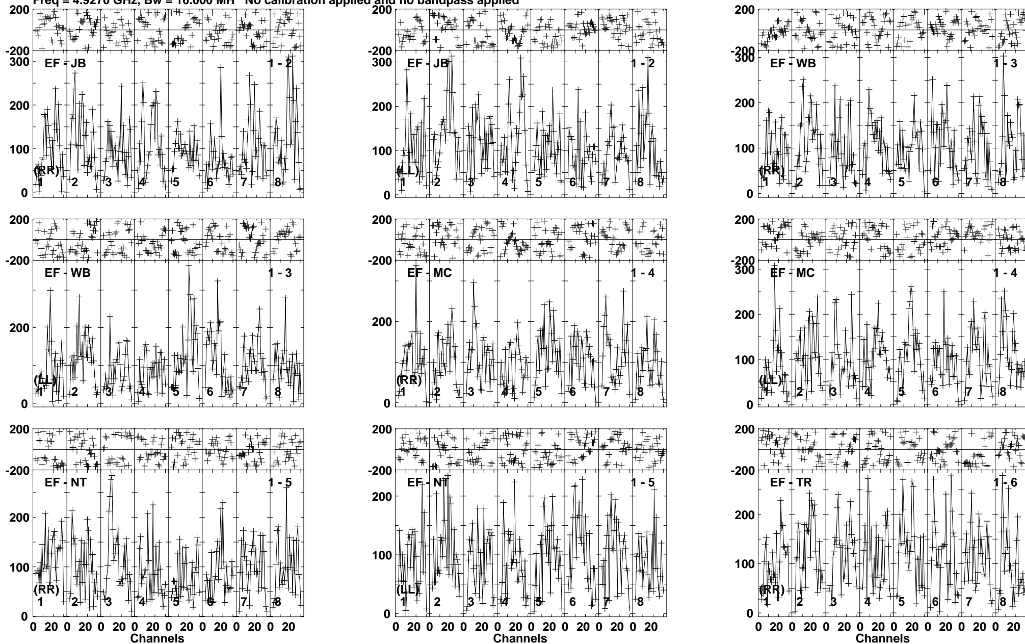
Lower frame: Micro Ampl Jy Top frame: Phas deg Vector averaged cross-power spectrum Baseline: EF (01) - JB (02) Timerange: 00/18:32:51 to 00/18:35:19
