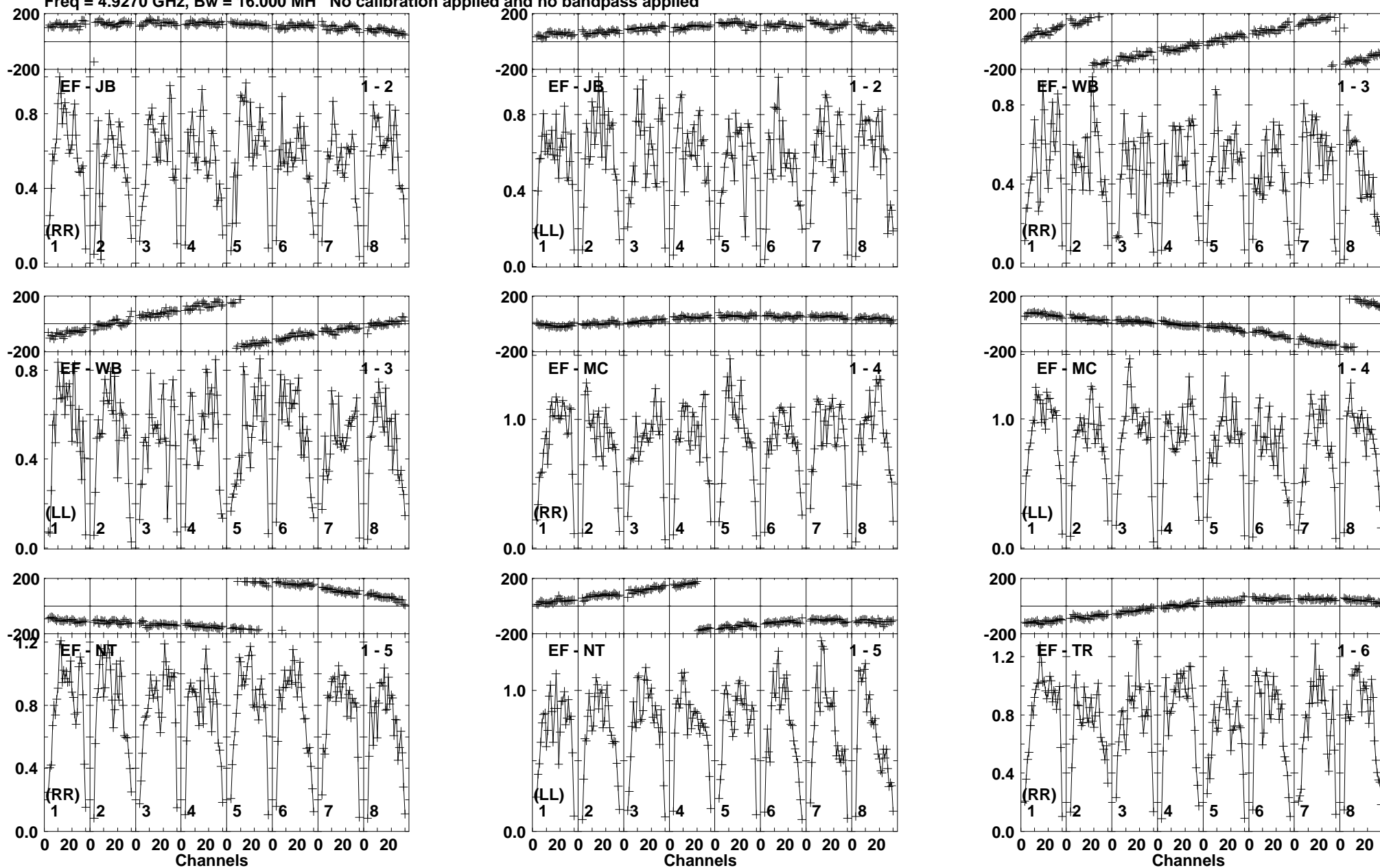
Lower frame: Milli Ampl Jy Top frame: Phas deg Vector averaged cross-power spectrum Baseline: EF (01) - JB (02) Timerange: 00/19:07:21 to 00/19:08:20
