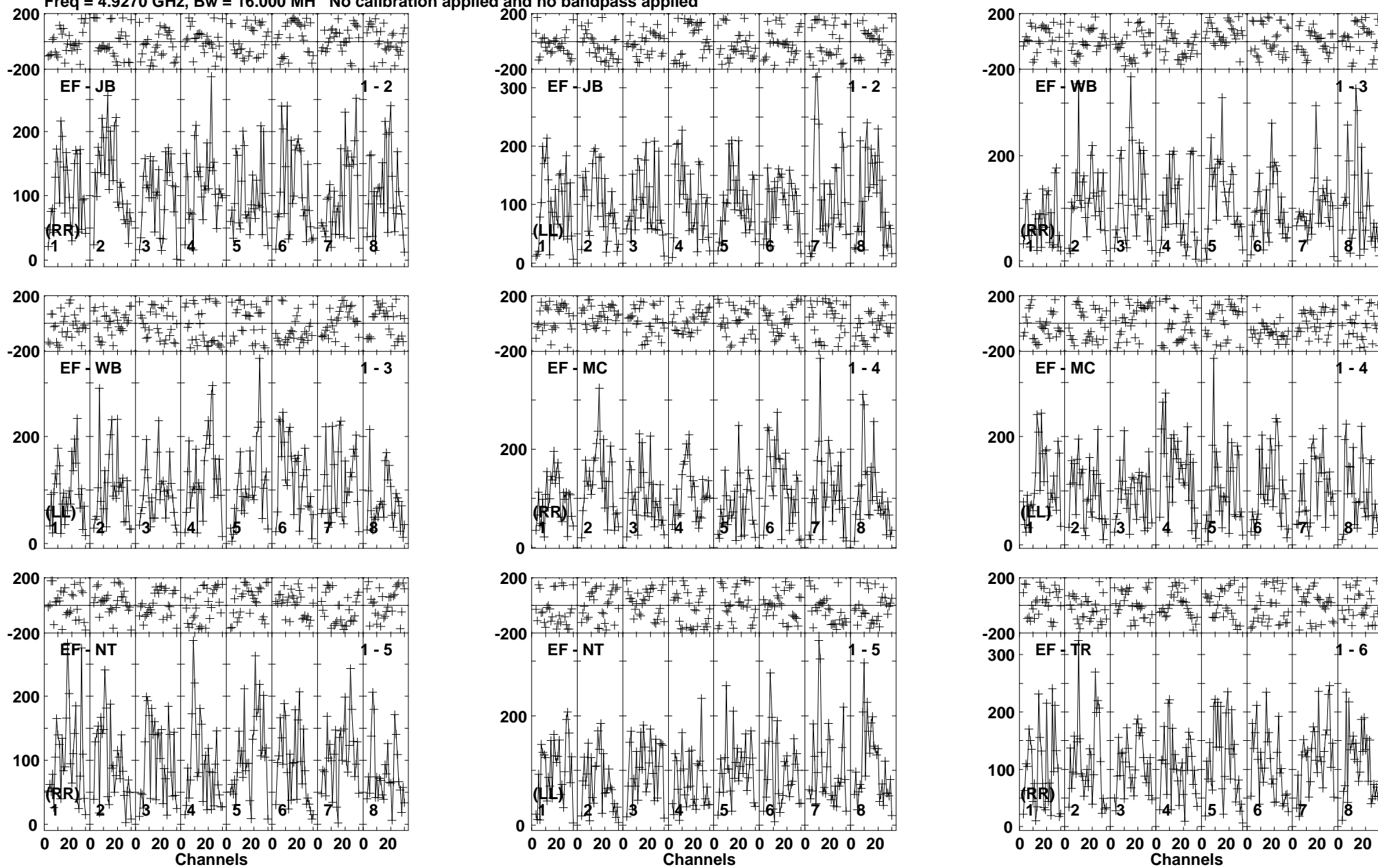
Lower frame: Micro Ampl Jy Top frame: Phas deg Vector averaged cross-power spectrum Baseline: EF (01) - JB (02) Timerange: 00/20:32:50 to 00/20:35:19
