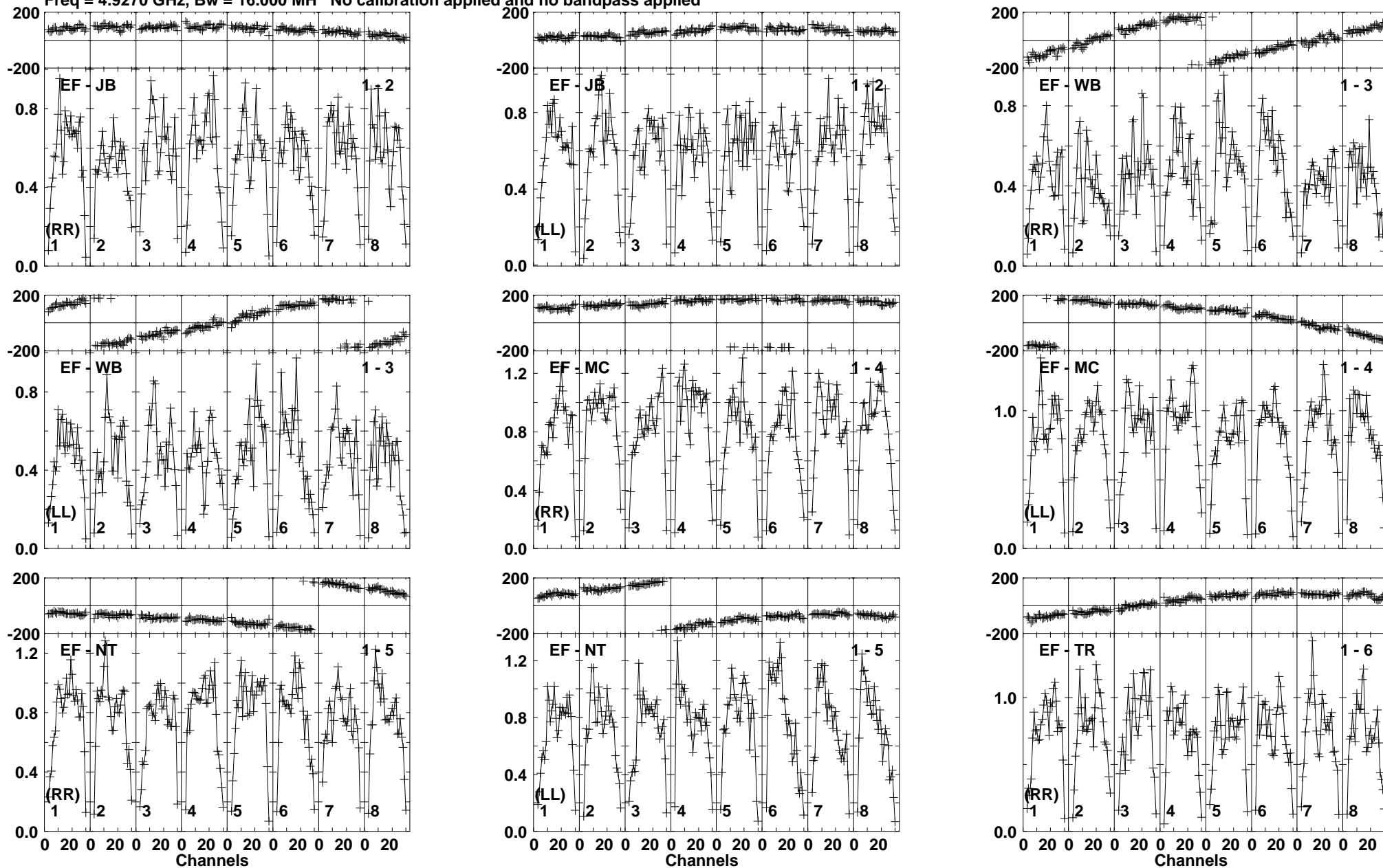
Lower frame: Milli Ampl Jy Top frame: Phas deg Vector averaged cross-power spectrum Baseline: EF (01) - JB (02) Timerange: 00:19:31:01 to 00:19:32:29
