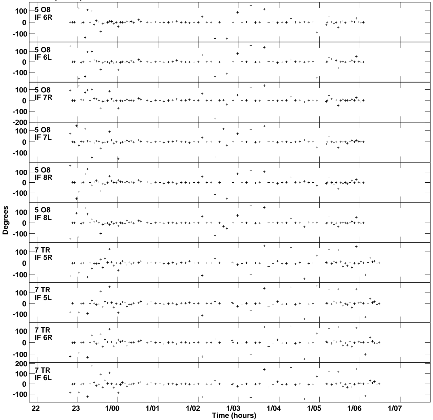
Plot file version 8 created 26-SEP-2019 11:53:40 Gain phs vs UTC time for J0257-1212.MULTI.1 SN 1 Rpol & Lpol IF 1 - 8
